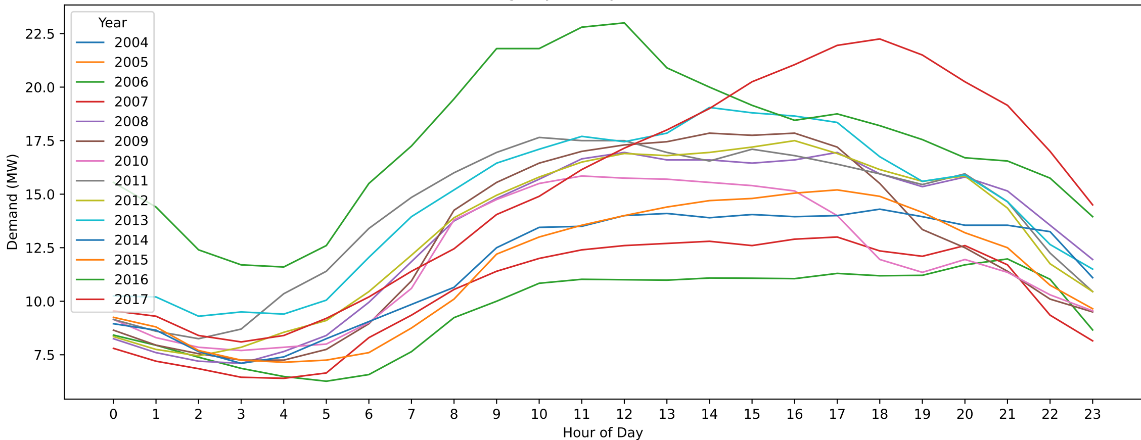
OAK — Boxing Day (Hourly Demand Across Years)
