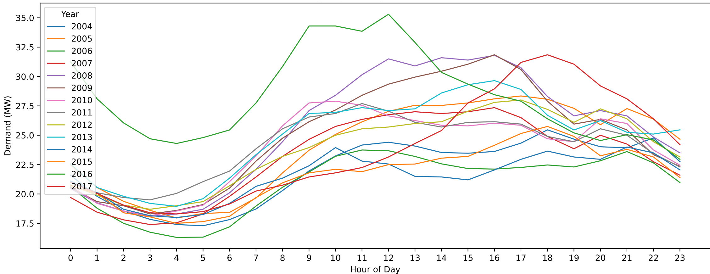
MGE — Boxing Day (Hourly Demand Across Years)
