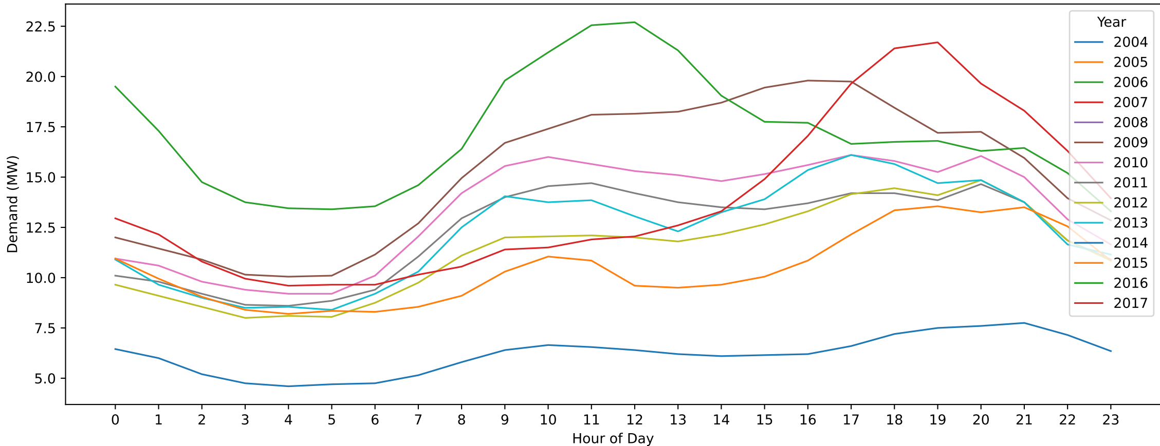
LWN — Boxing Day (Hourly Demand Across Years)
