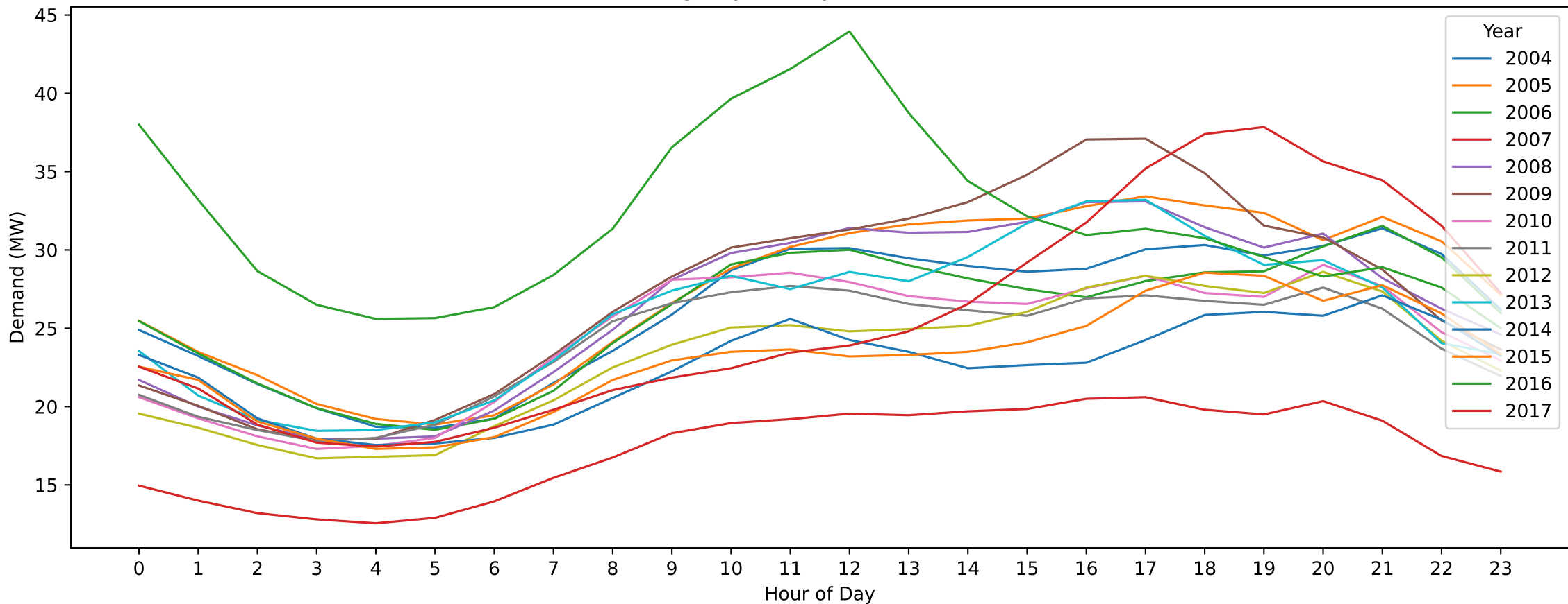
DC — Boxing Day (Hourly Demand Across Years)
