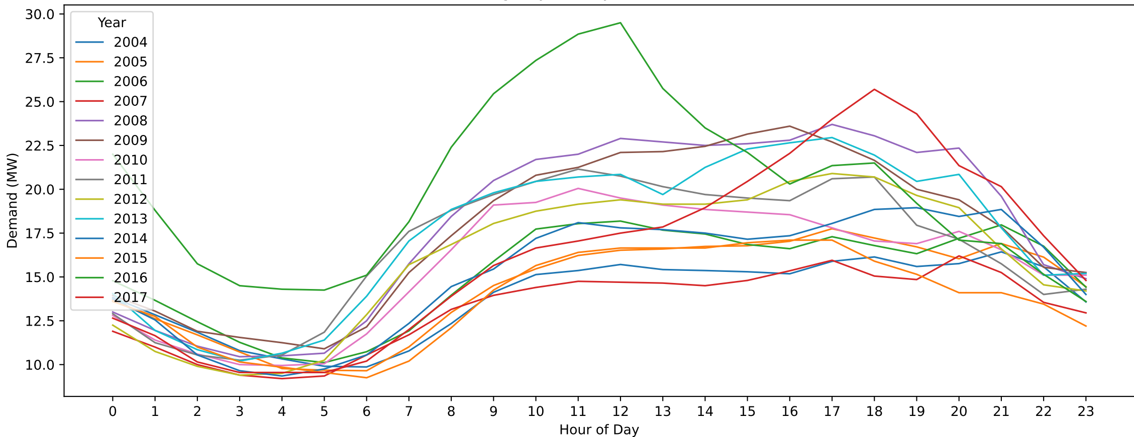
WD — Boxing Day (Hourly Demand Across Years)
