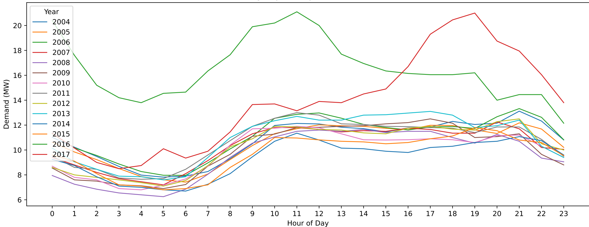
MR — Boxing Day (Hourly Demand Across Years)
