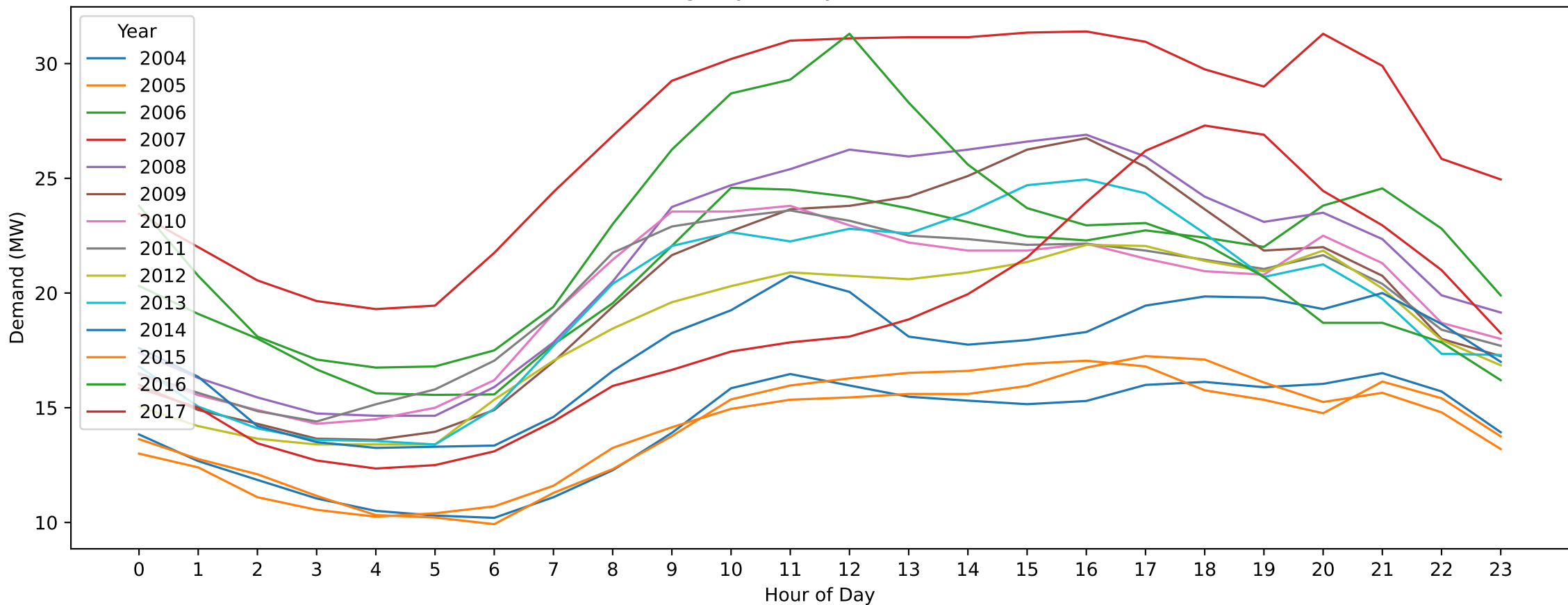
NW — Boxing Day (Hourly Demand Across Years)
