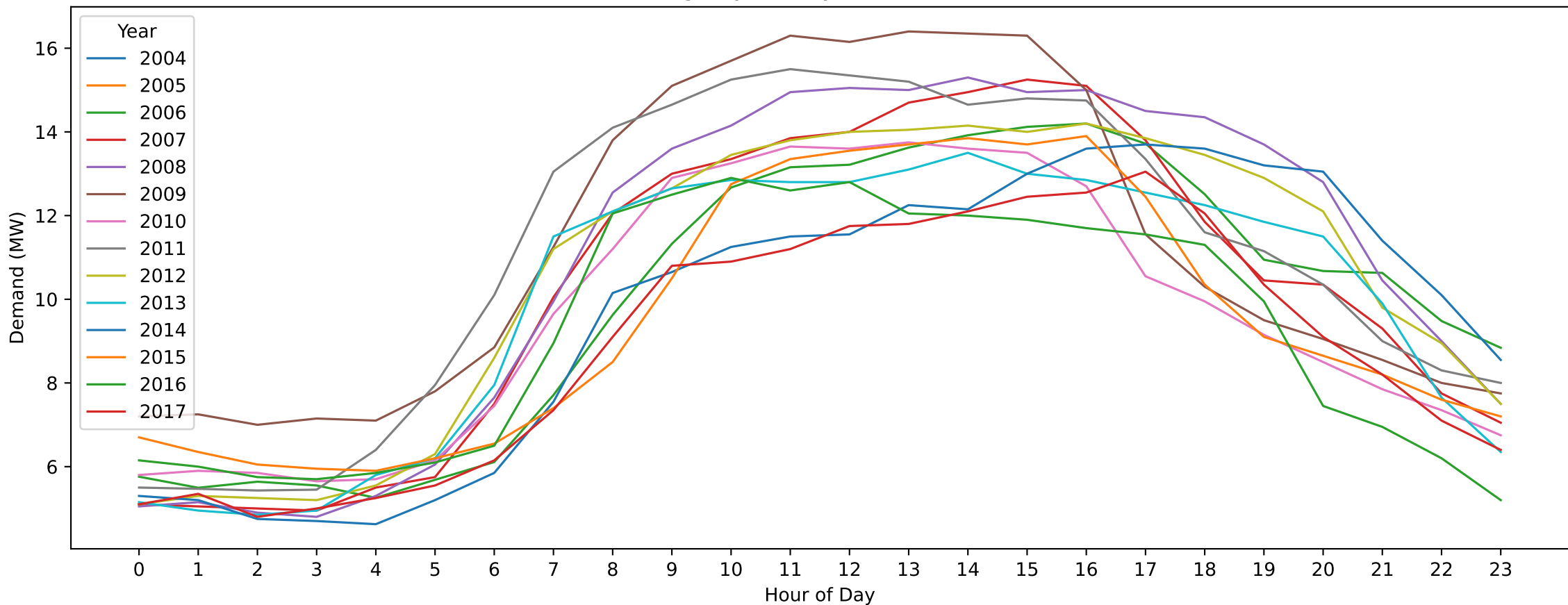
CM — Boxing Day (Hourly Demand Across Years)
