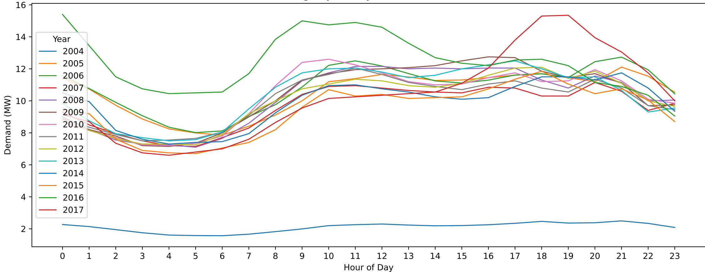
M — Boxing Day (Hourly Demand Across Years)
