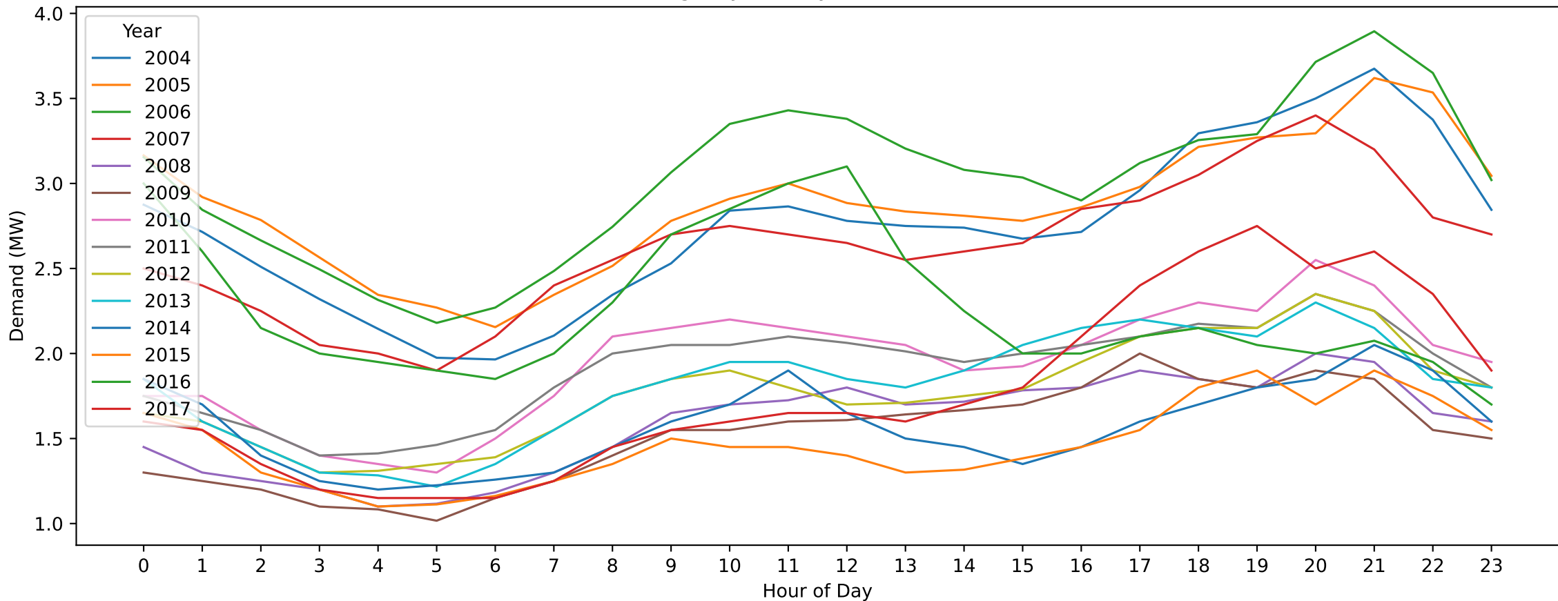
SH — Boxing Day (Hourly Demand Across Years)
