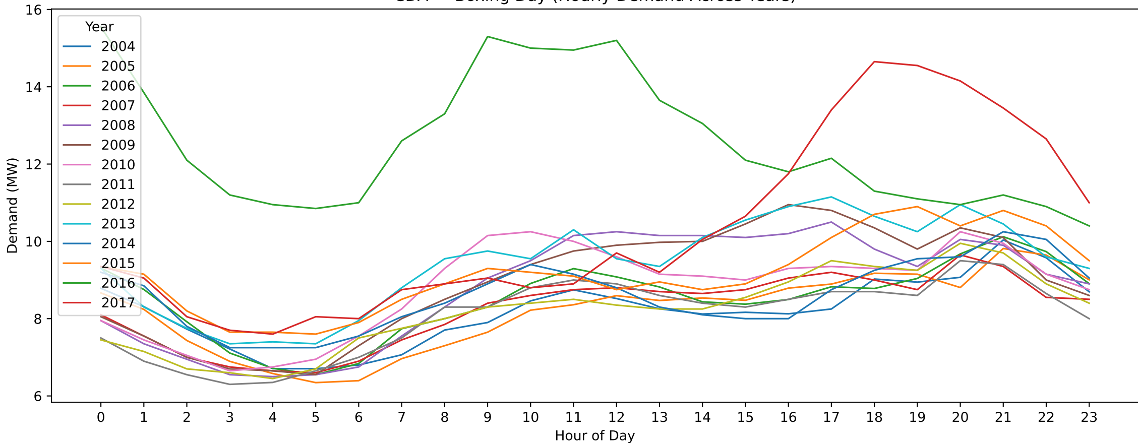
CDA — Boxing Day (Hourly Demand Across Years)
