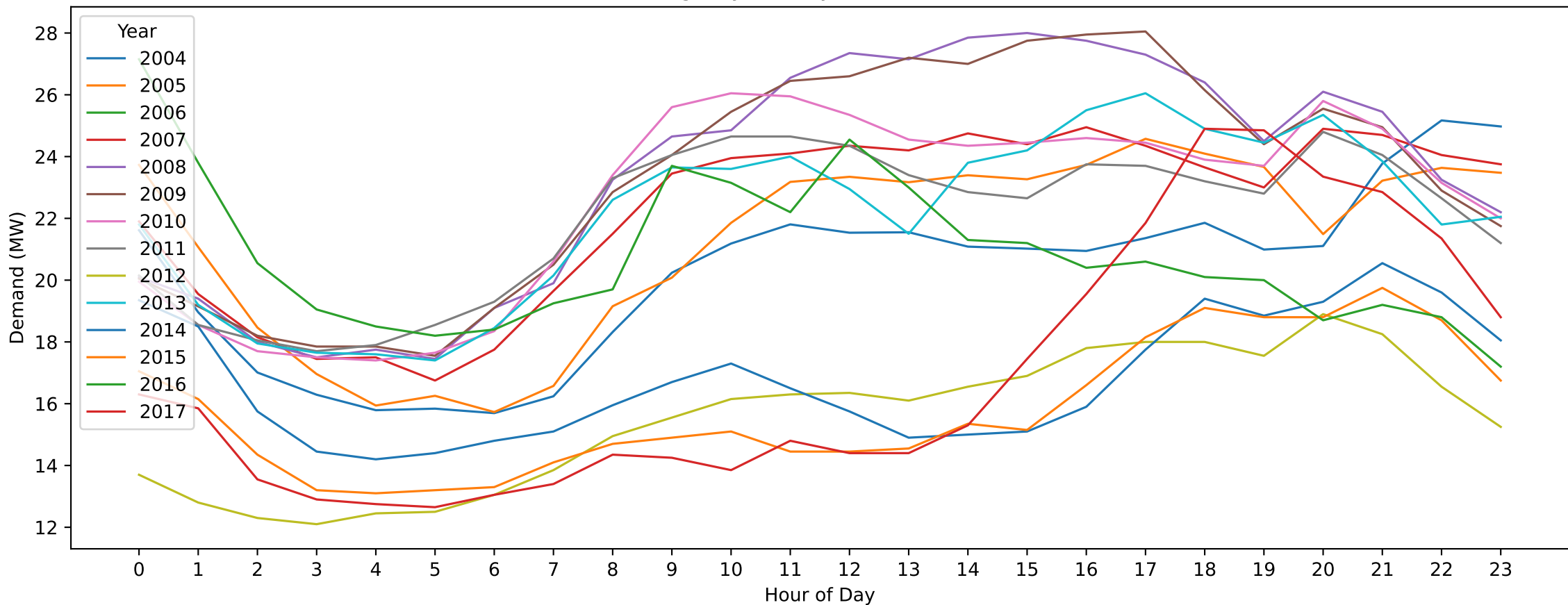
NP — Boxing Day (Hourly Demand Across Years)
