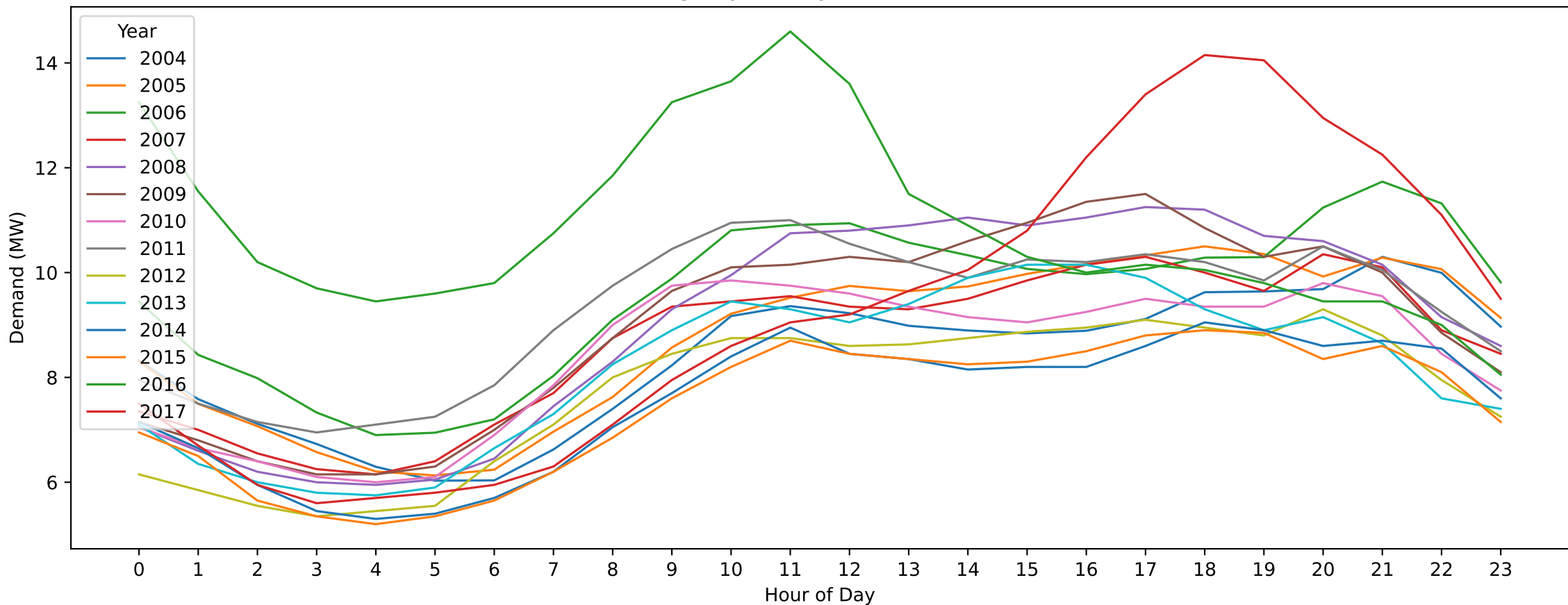
EL — Boxing Day (Hourly Demand Across Years)
