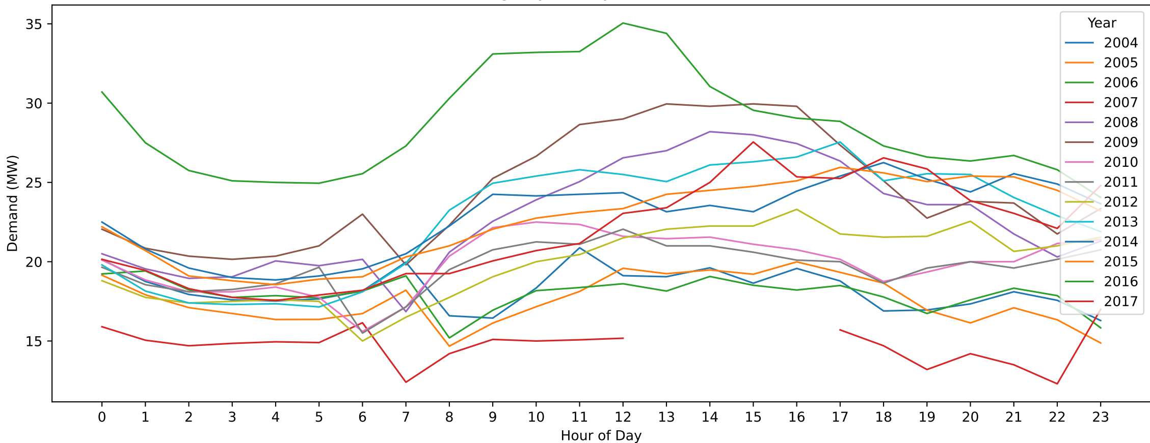
DN — Boxing Day (Hourly Demand Across Years)
