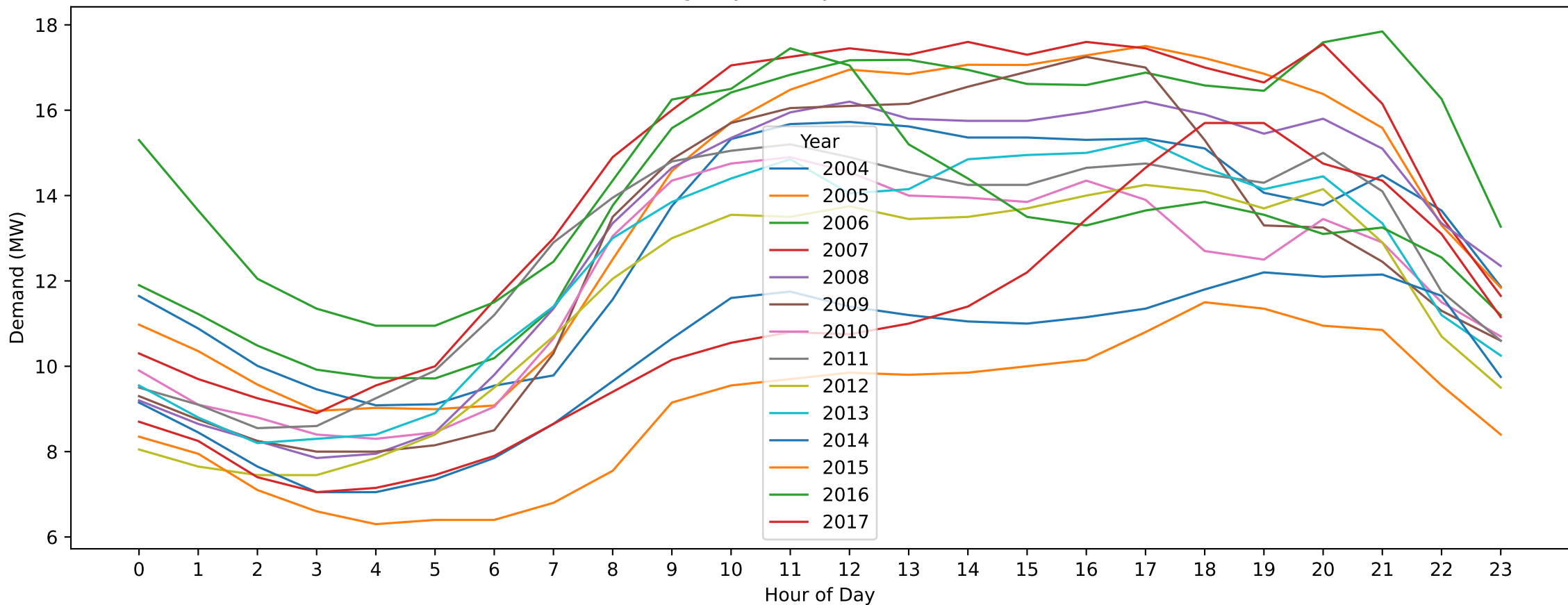
EM — Boxing Day (Hourly Demand Across Years)
