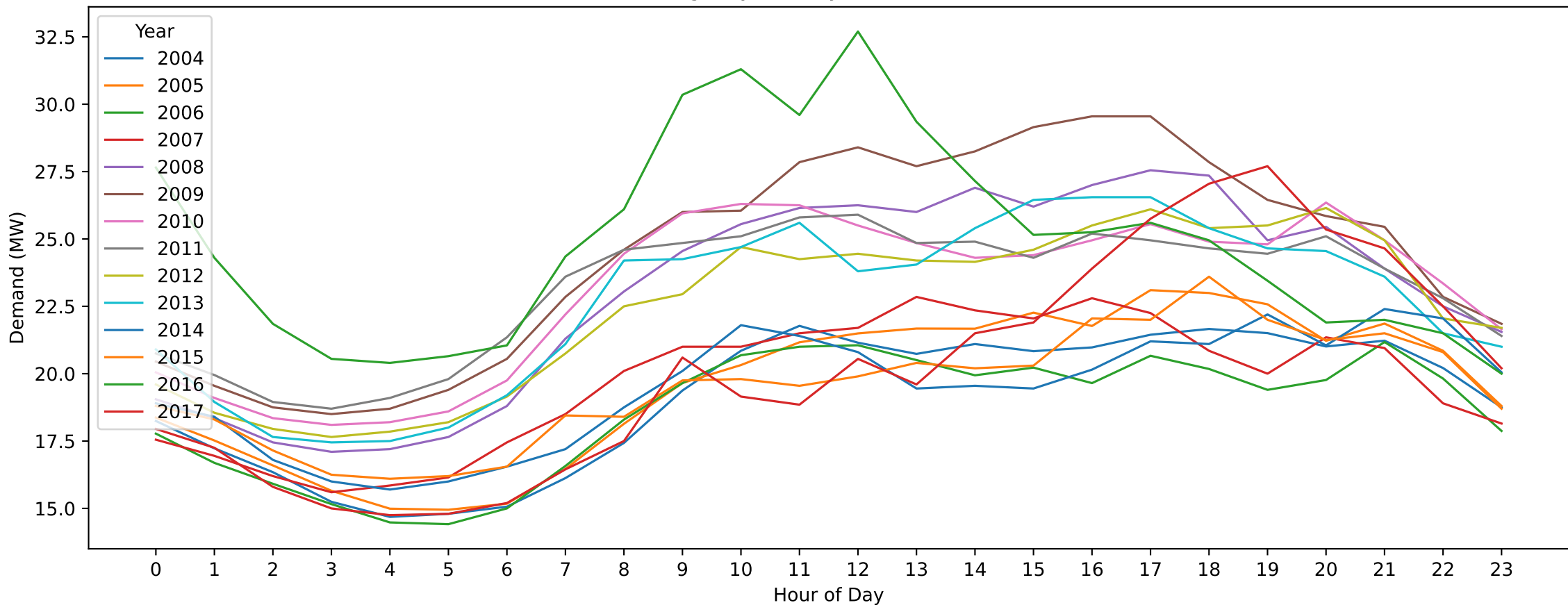
EB — Boxing Day (Hourly Demand Across Years)
