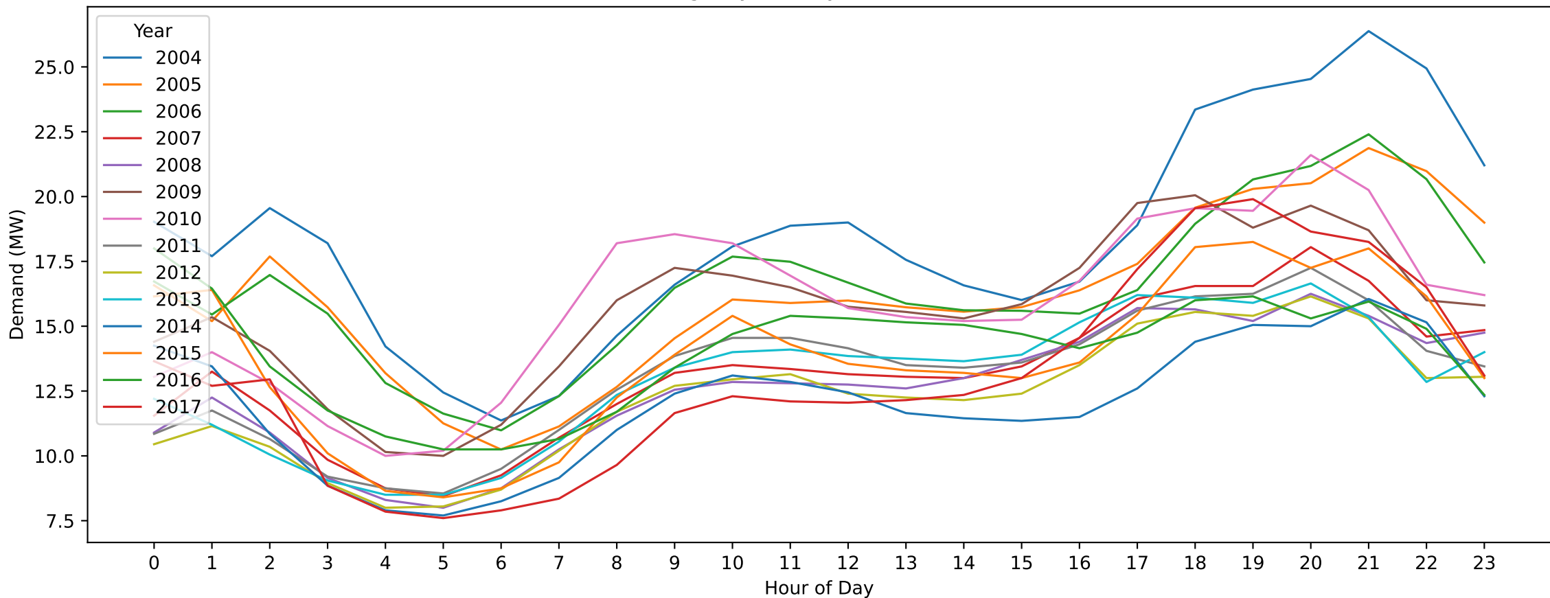
STO — Boxing Day (Hourly Demand Across Years)
