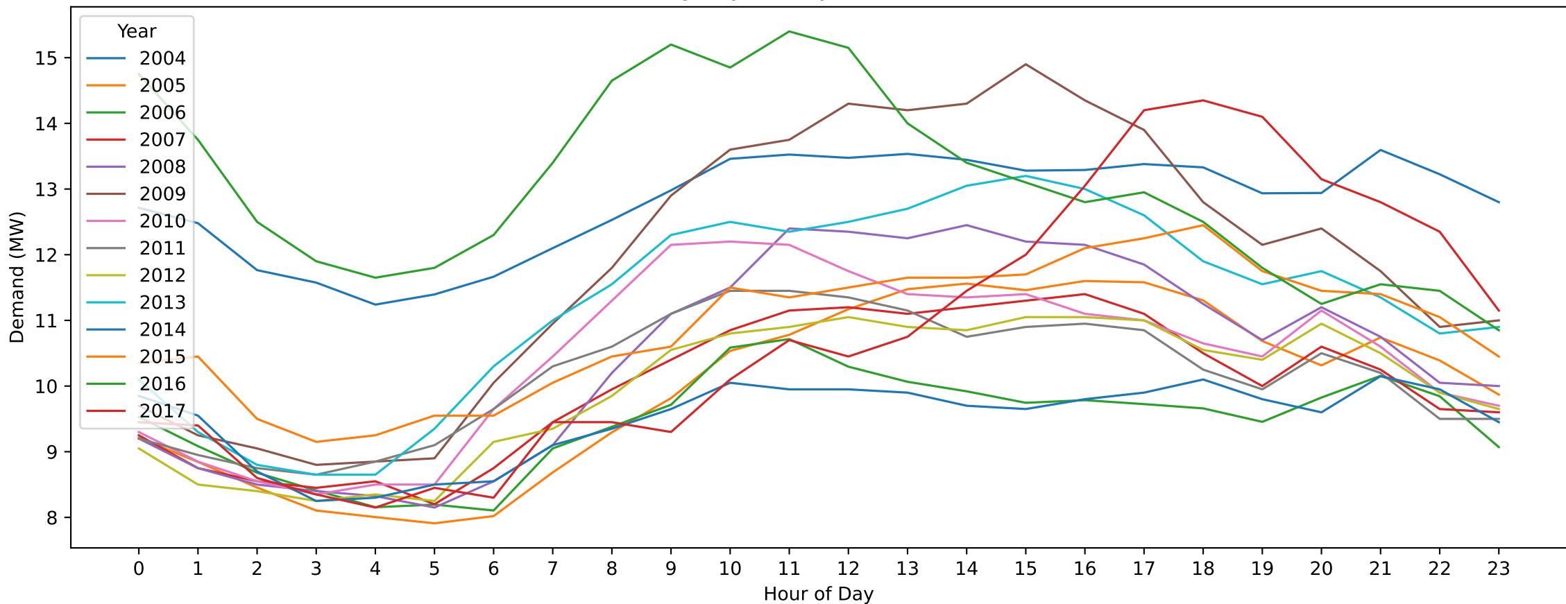
HT — Boxing Day (Hourly Demand Across Years)
