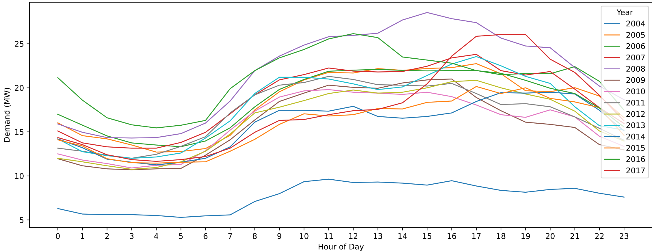
FTN — Boxing Day (Hourly Demand Across Years)
