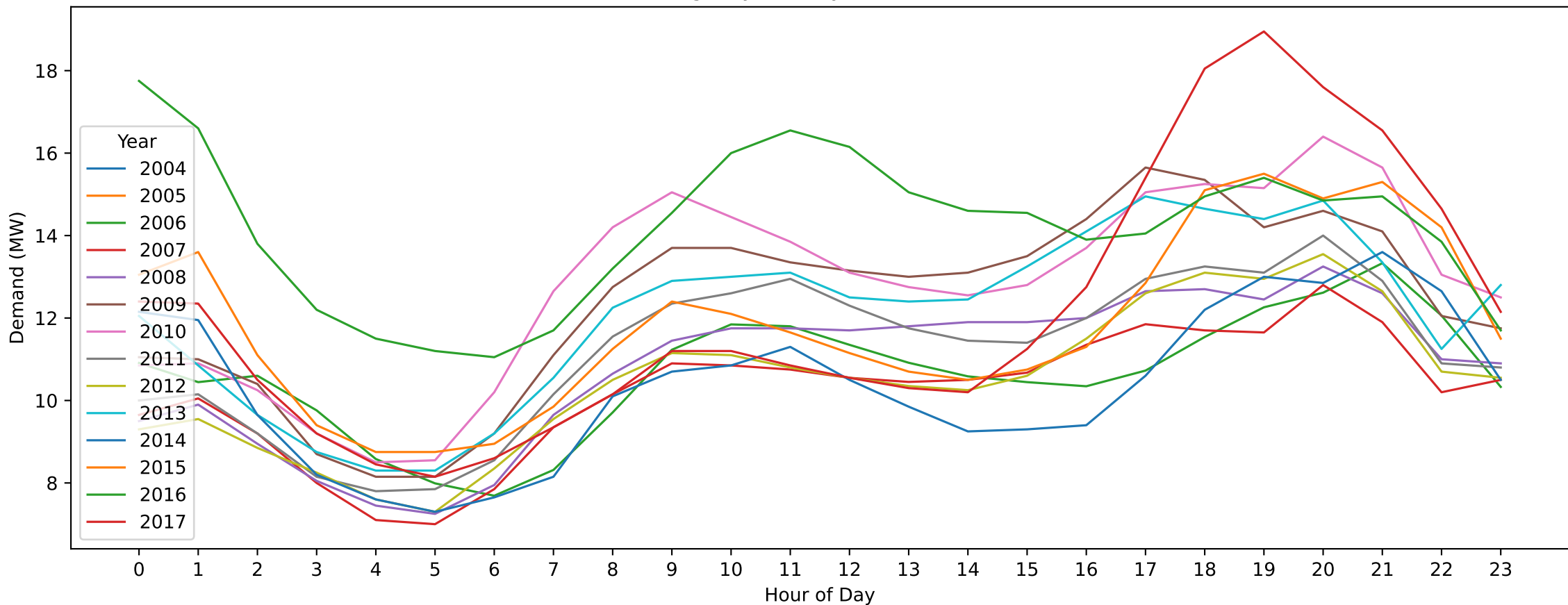
DMA — Boxing Day (Hourly Demand Across Years)
