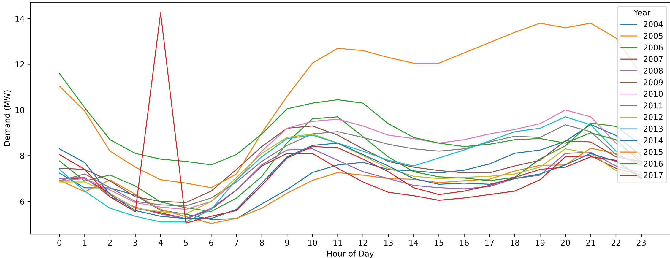
EW — Christmas Day (Hourly Demand Across Years)
