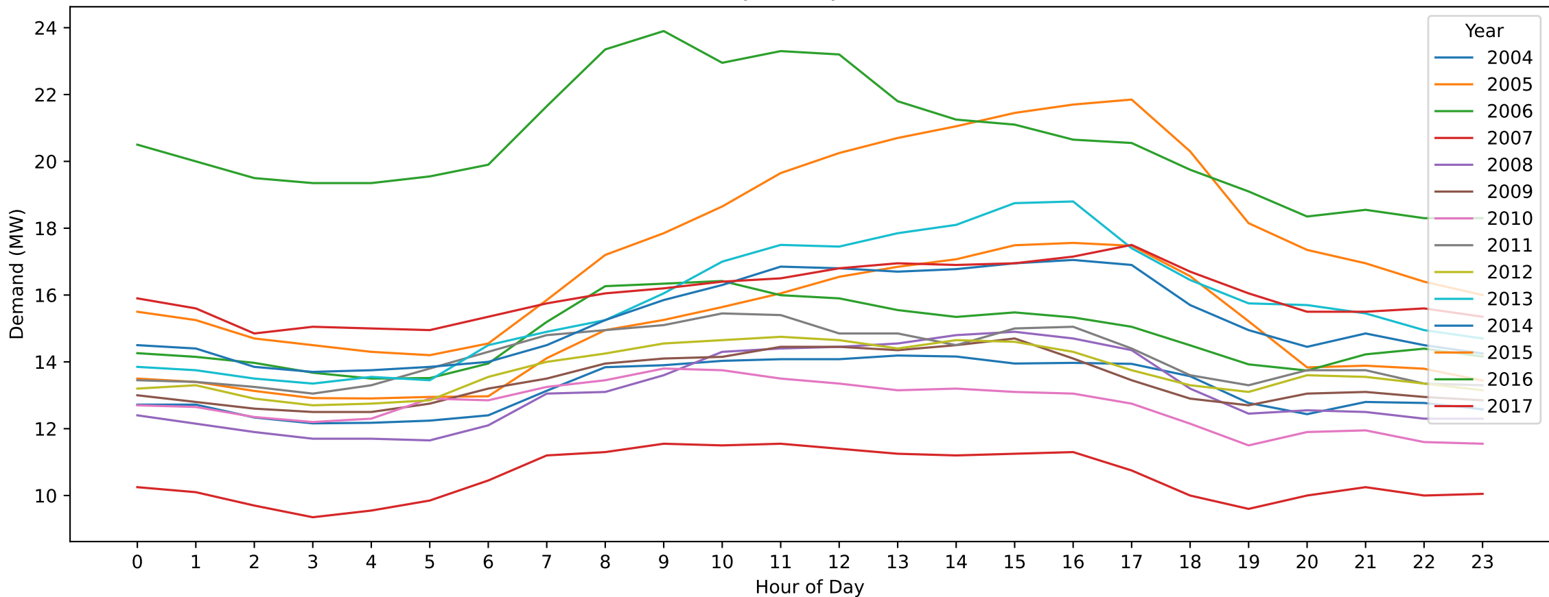
NO — Christmas Day (Hourly Demand Across Years)
