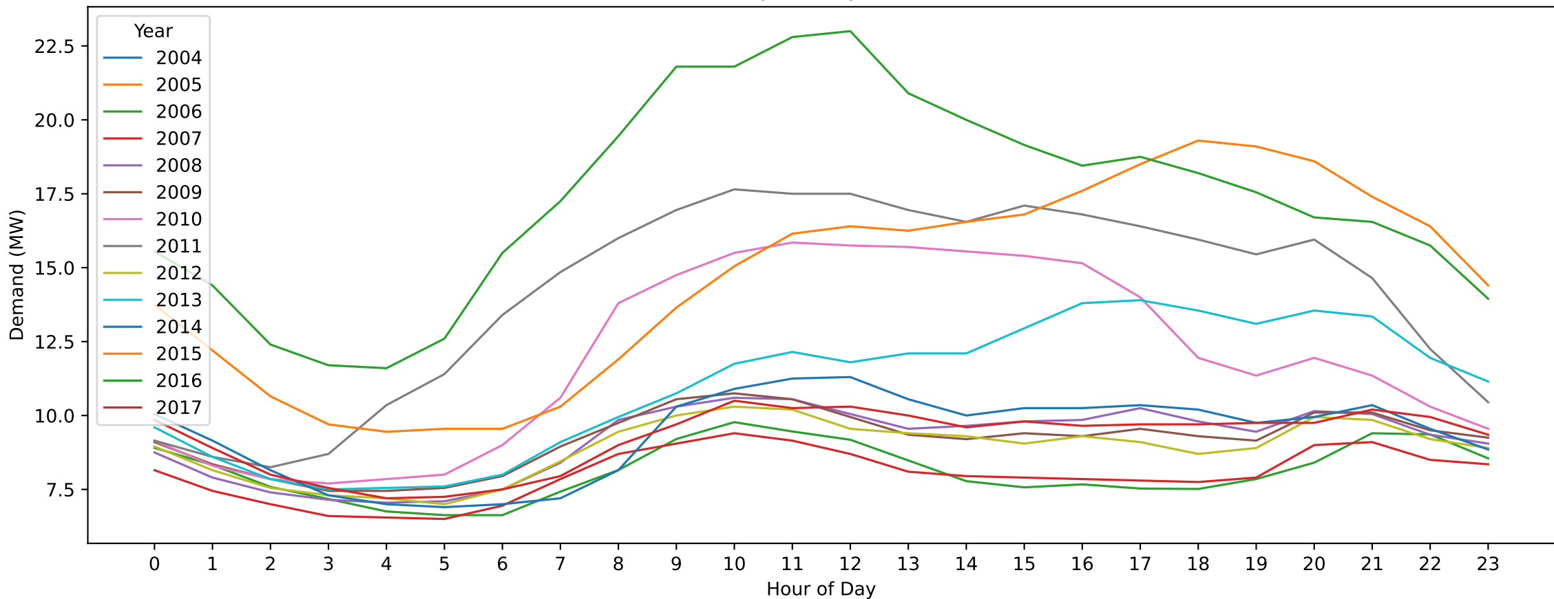
OAK — Christmas Day (Hourly Demand Across Years)
