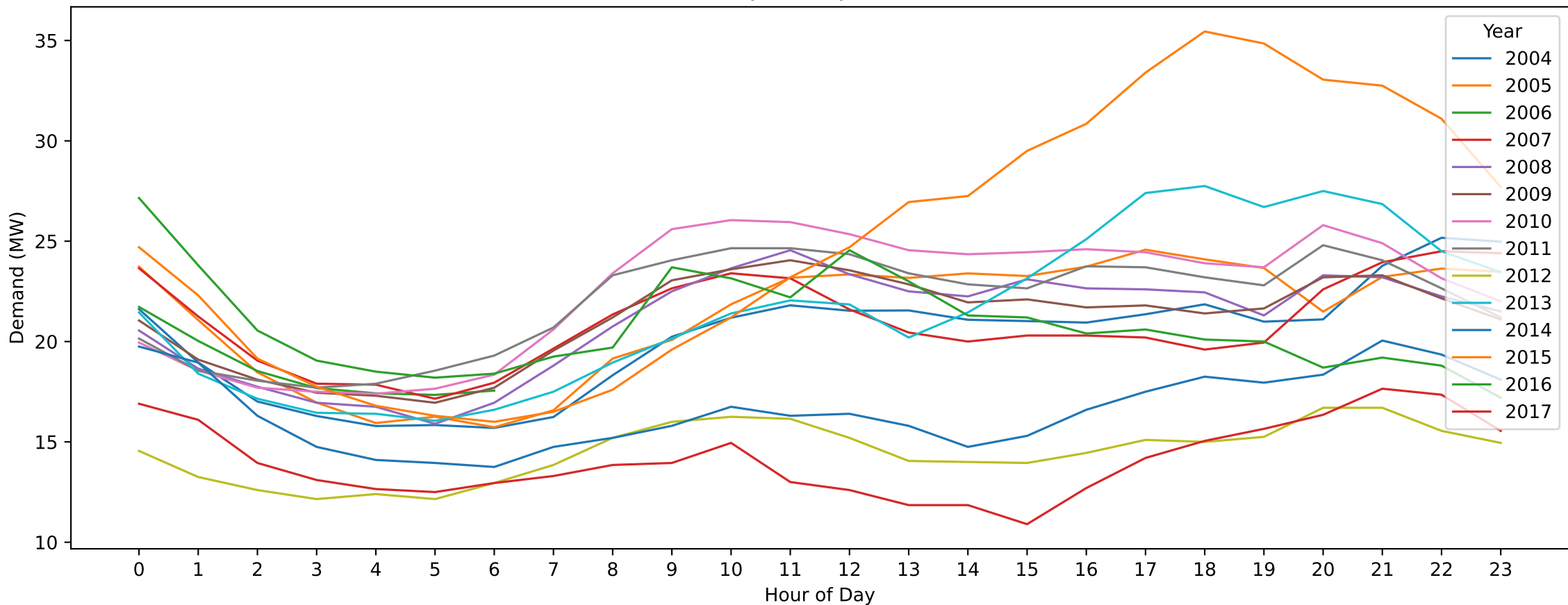
NP — Christmas Day (Hourly Demand Across Years)
