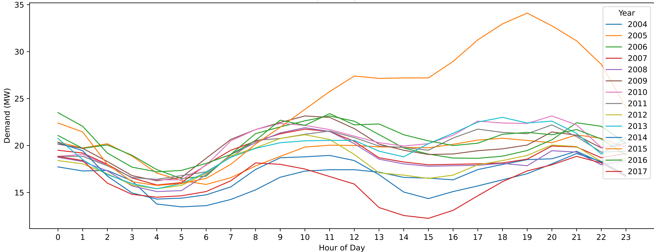
HGS — Christmas Day (Hourly Demand Across Years)
