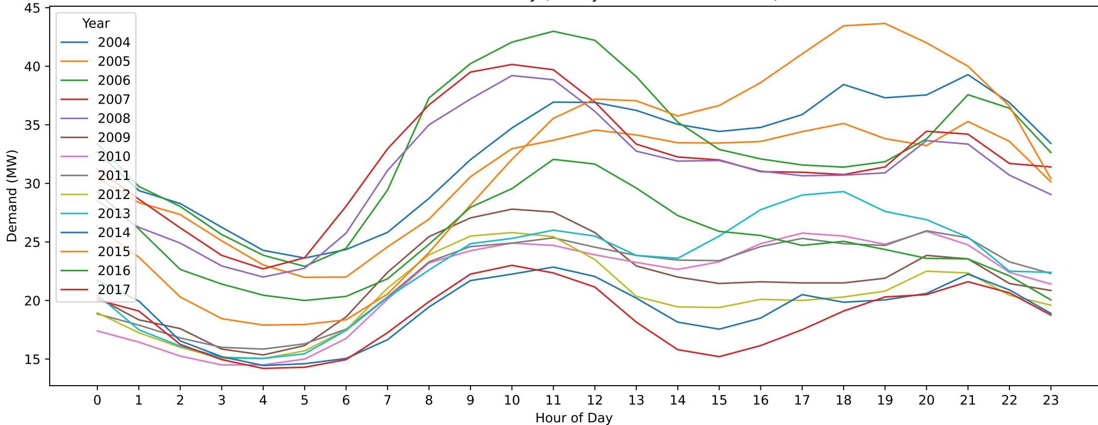
FSH — Christmas Day (Hourly Demand Across Years)
