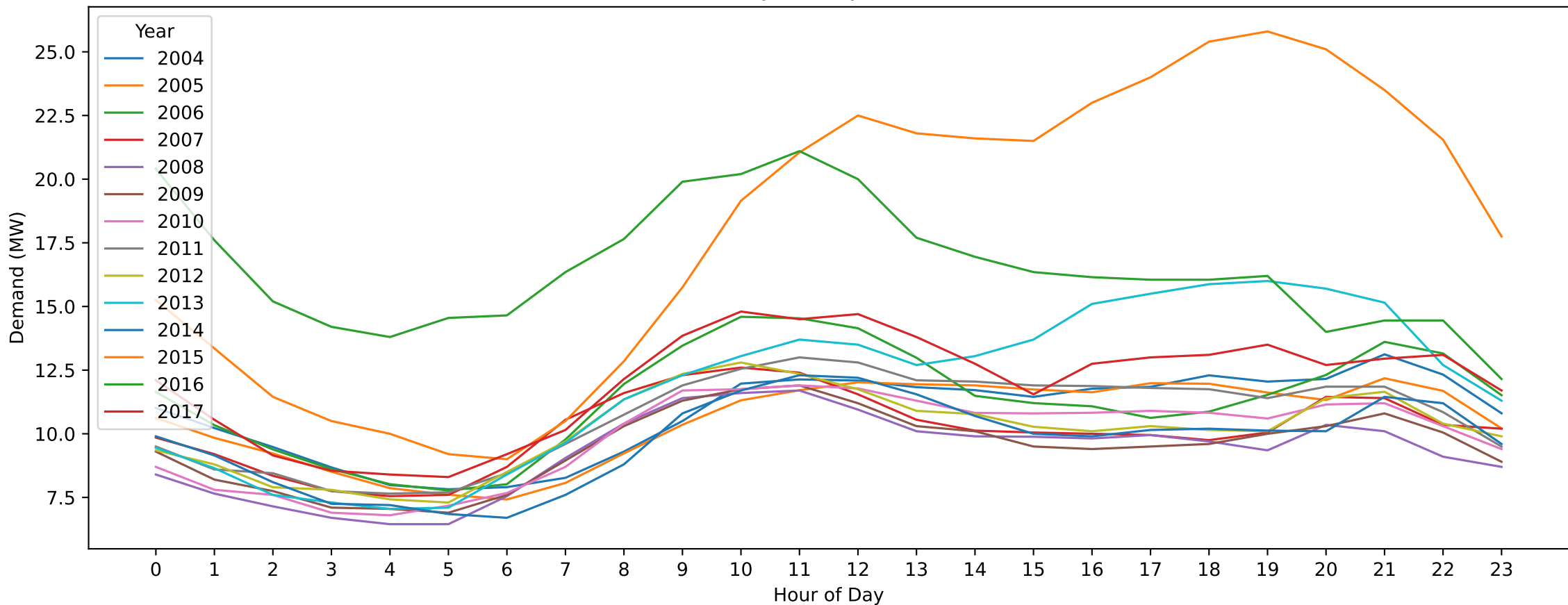
MR — Christmas Day (Hourly Demand Across Years)
