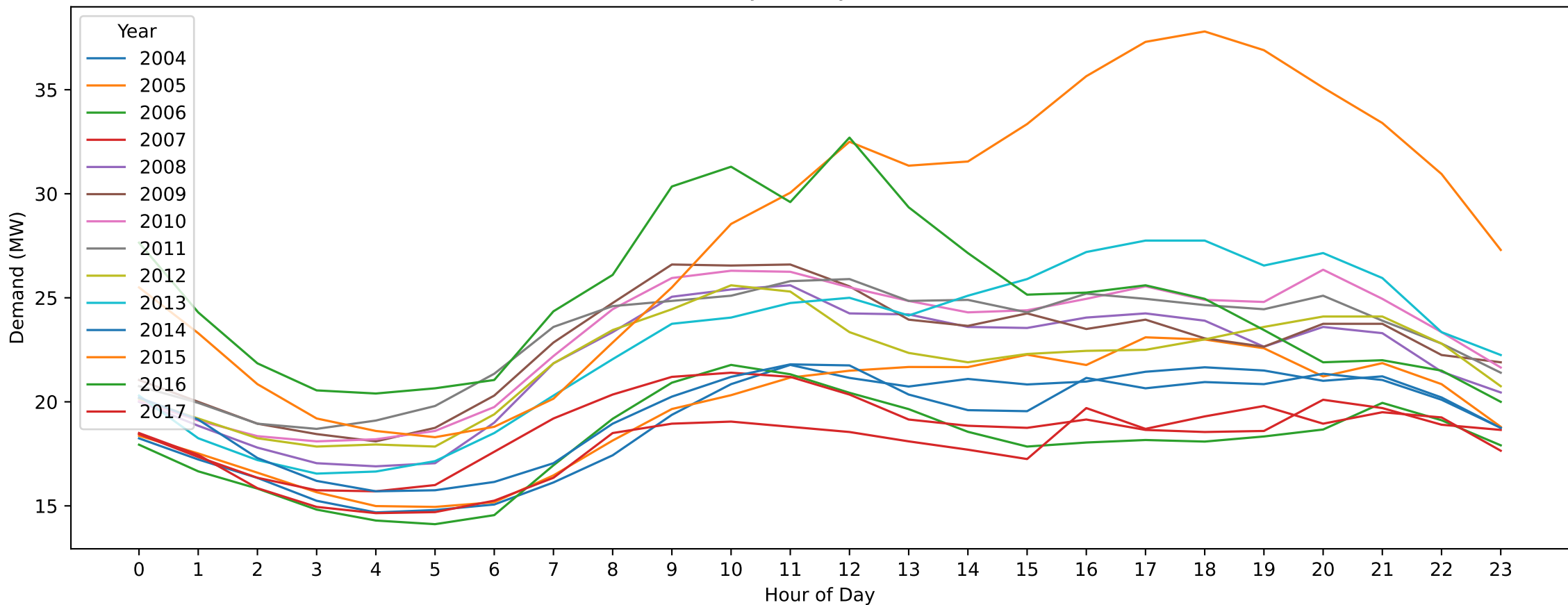
EB — Christmas Day (Hourly Demand Across Years)
