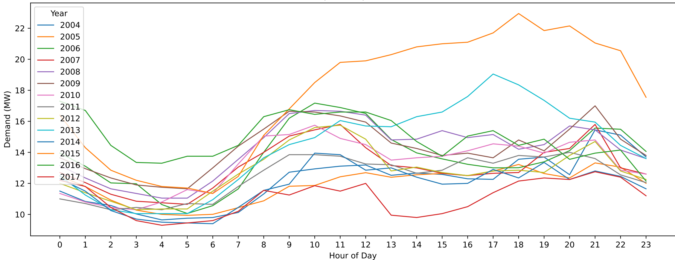
MC — Christmas Day (Hourly Demand Across Years)
