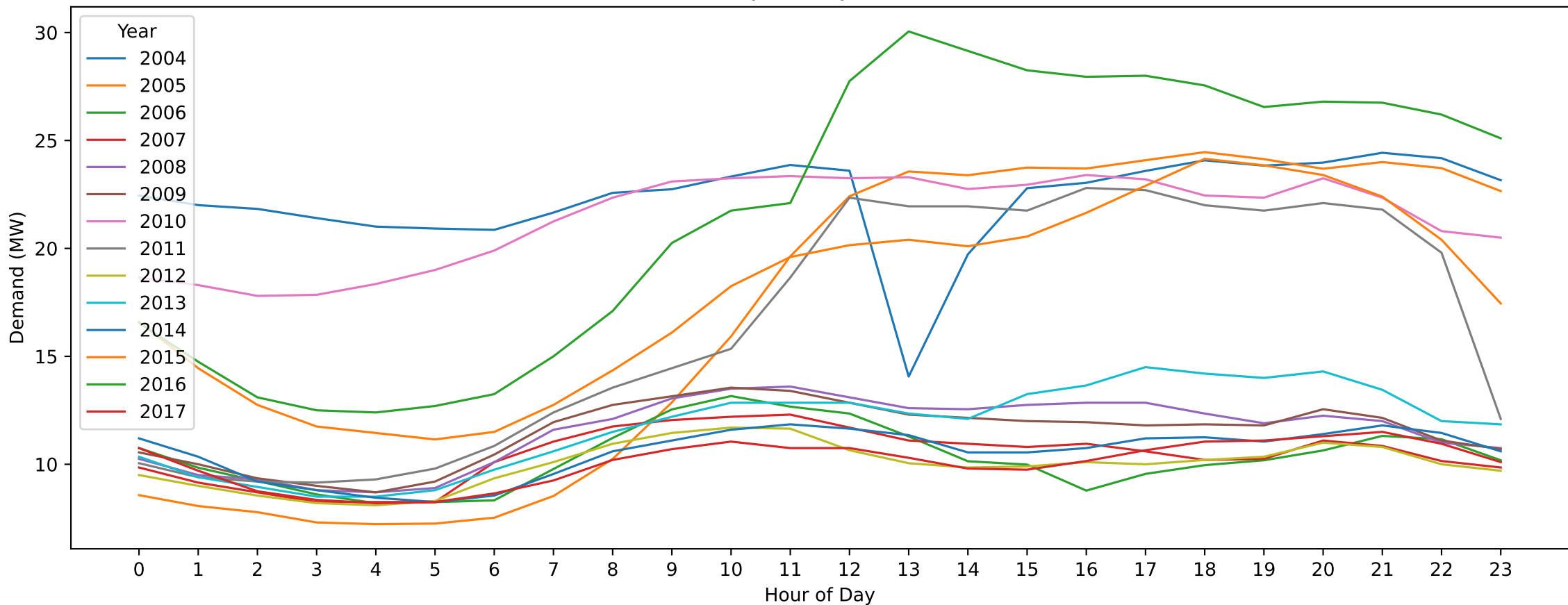
BH — Christmas Day (Hourly Demand Across Years)
