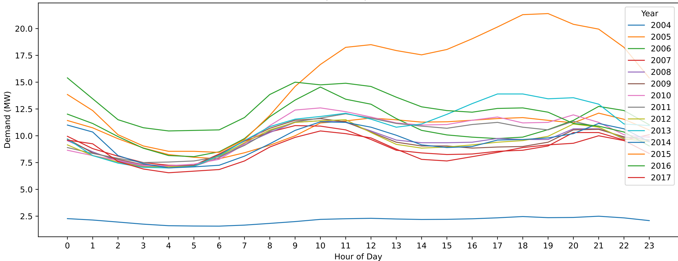
M — Christmas Day (Hourly Demand Across Years)
