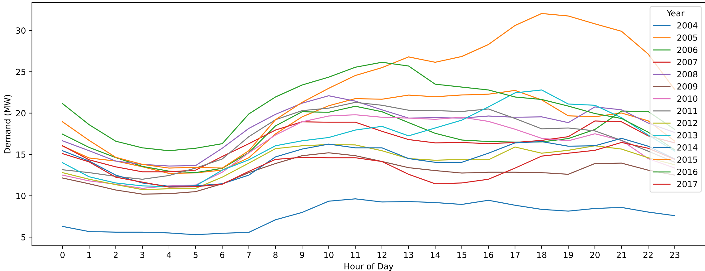
FTN — Christmas Day (Hourly Demand Across Years)
