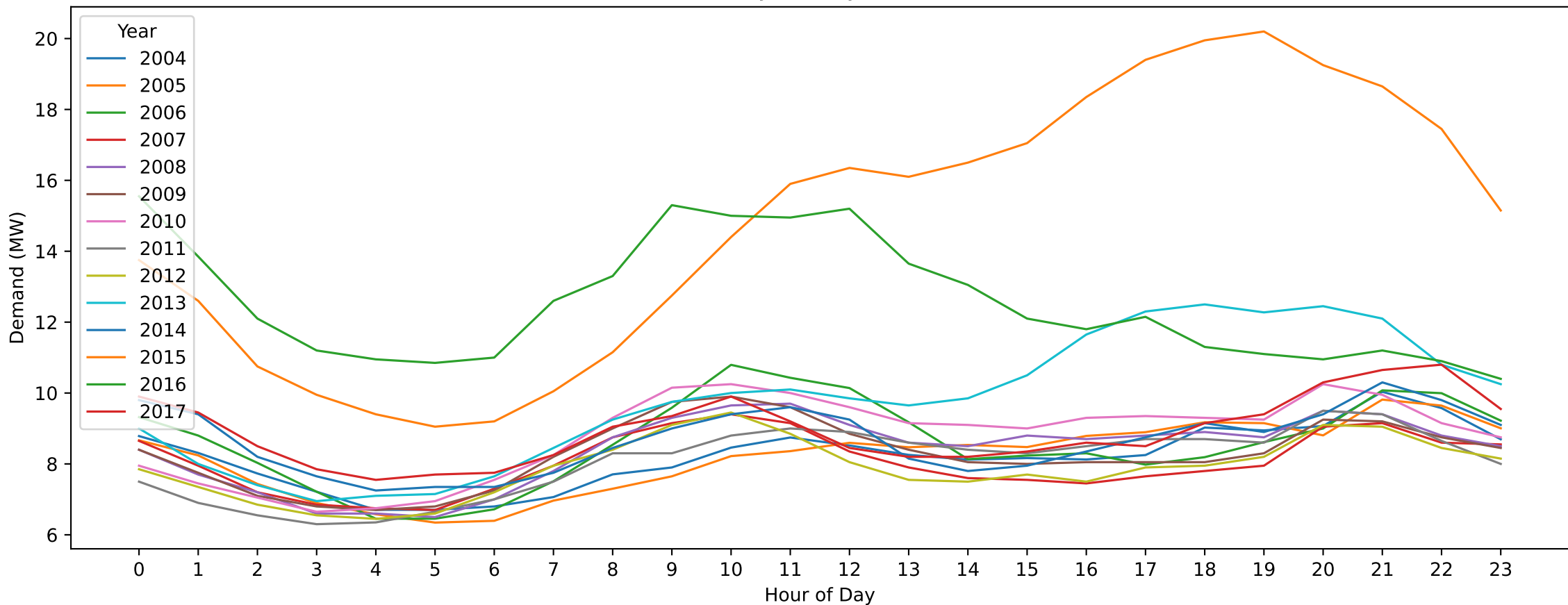
CDA — Christmas Day (Hourly Demand Across Years)
