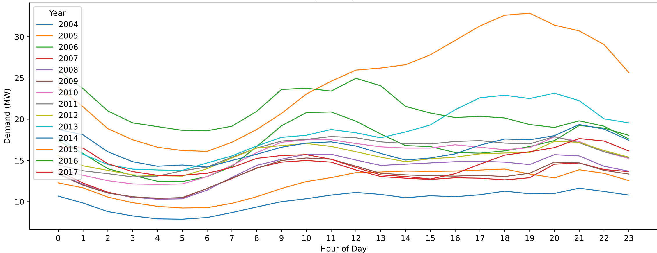
LD — Christmas Day (Hourly Demand Across Years)
