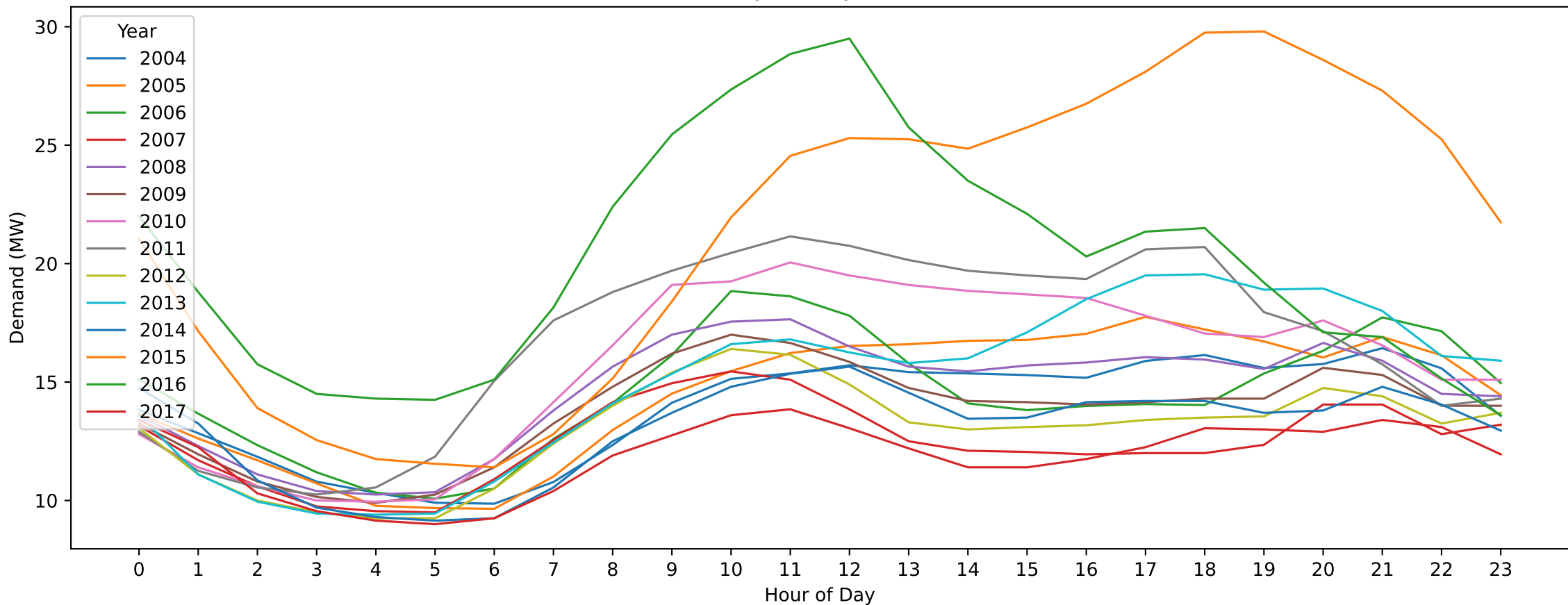
WD — Christmas Day (Hourly Demand Across Years)
