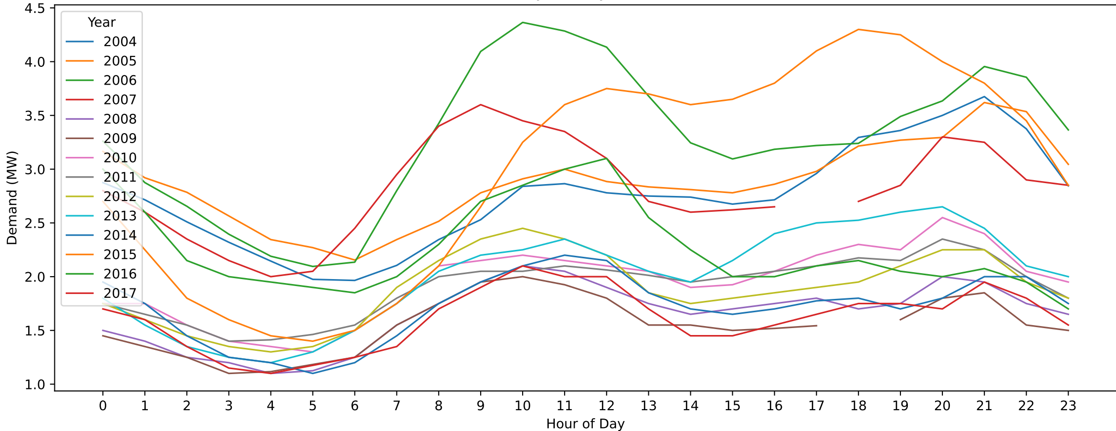
SH — Christmas Day (Hourly Demand Across Years)
