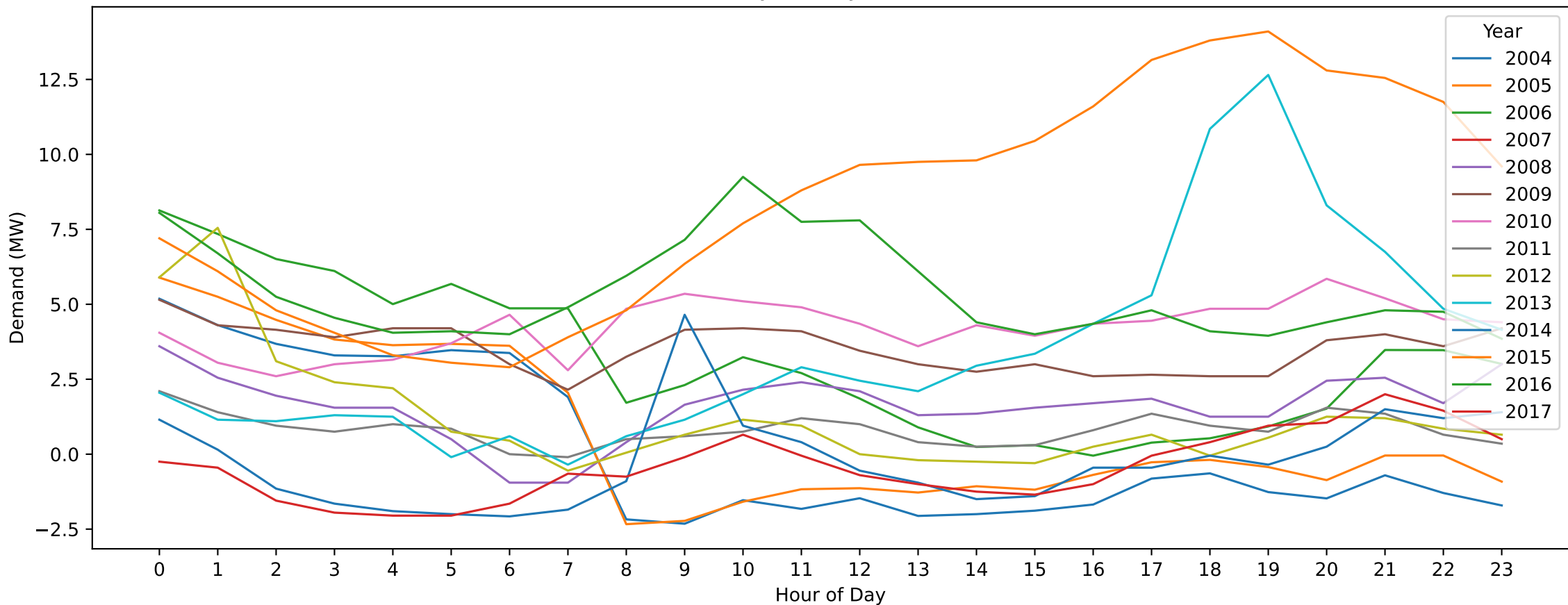
SS — Christmas Day (Hourly Demand Across Years)
