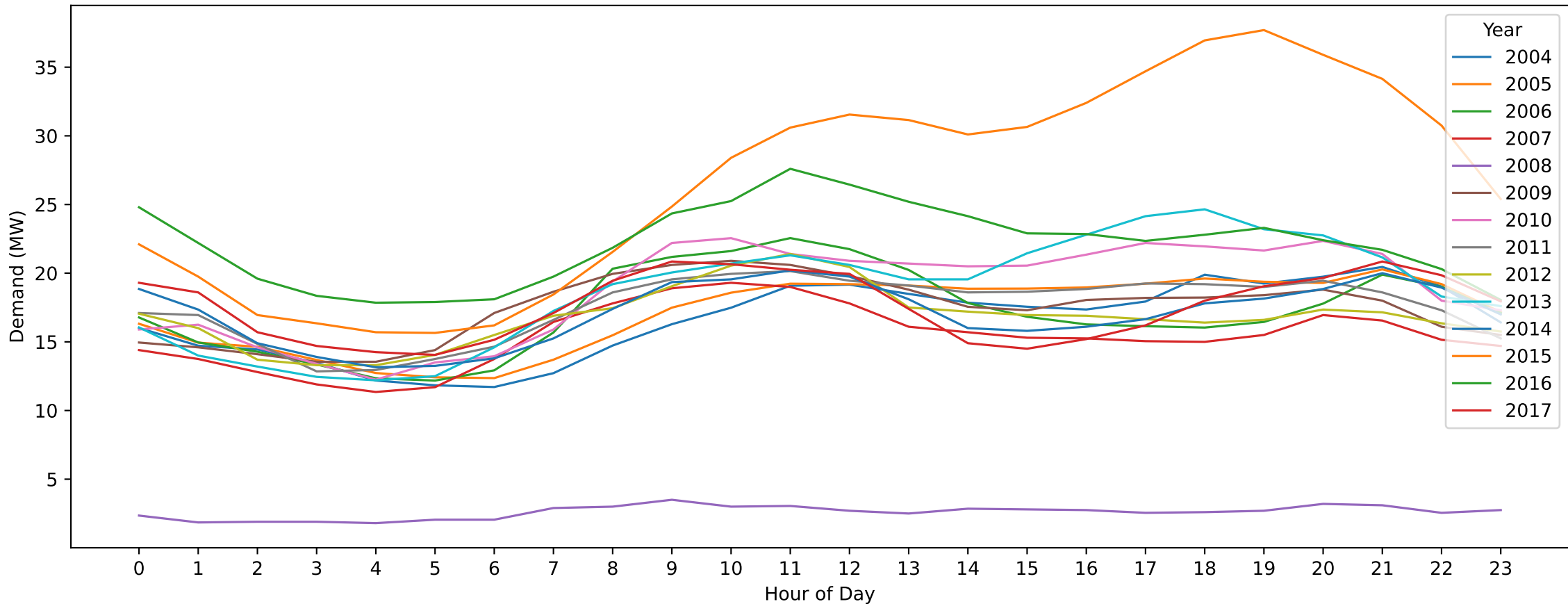
MTN — Christmas Day (Hourly Demand Across Years)
