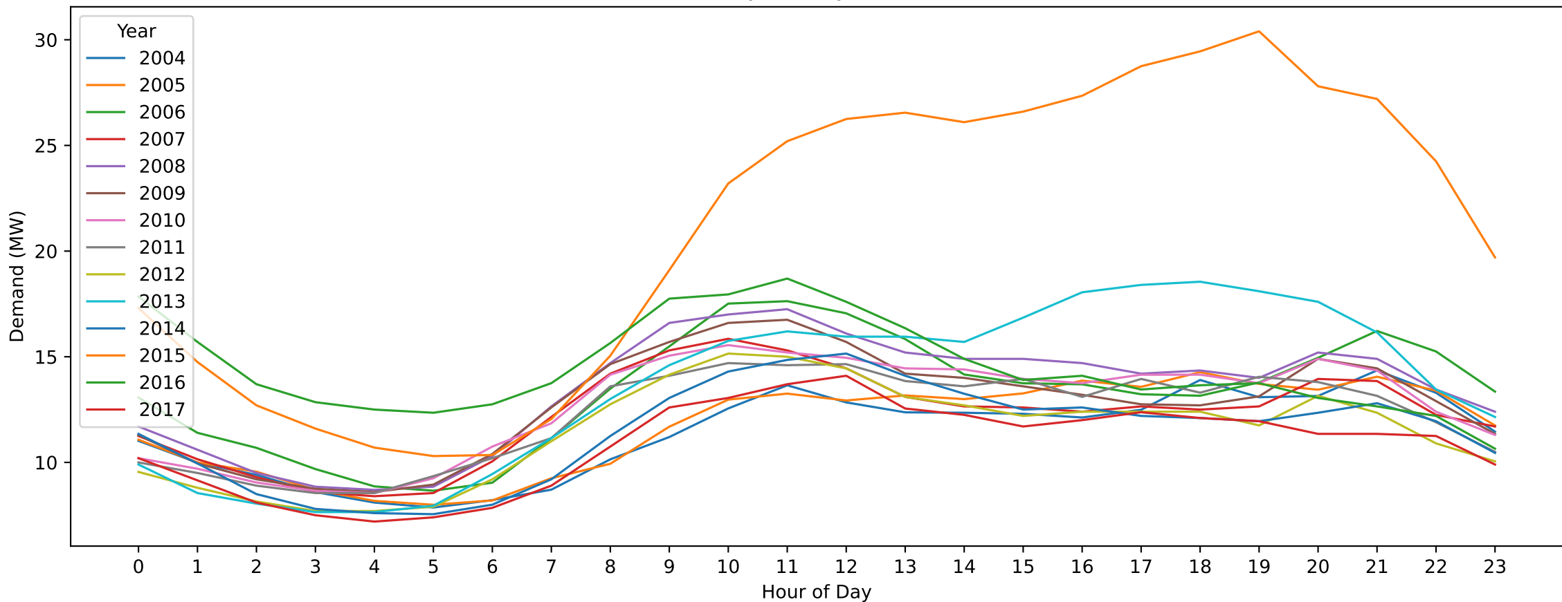
NB — Christmas Day (Hourly Demand Across Years)
