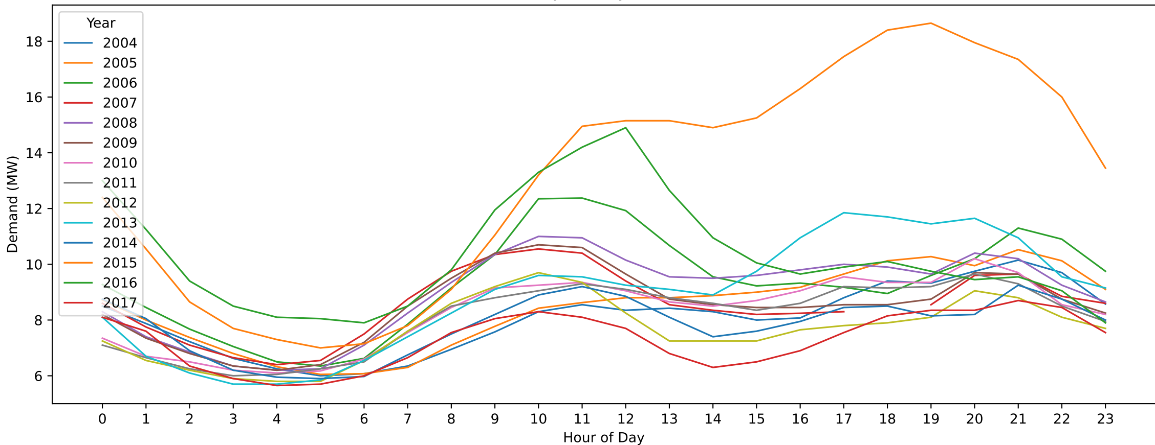
BU — Christmas Day (Hourly Demand Across Years)
