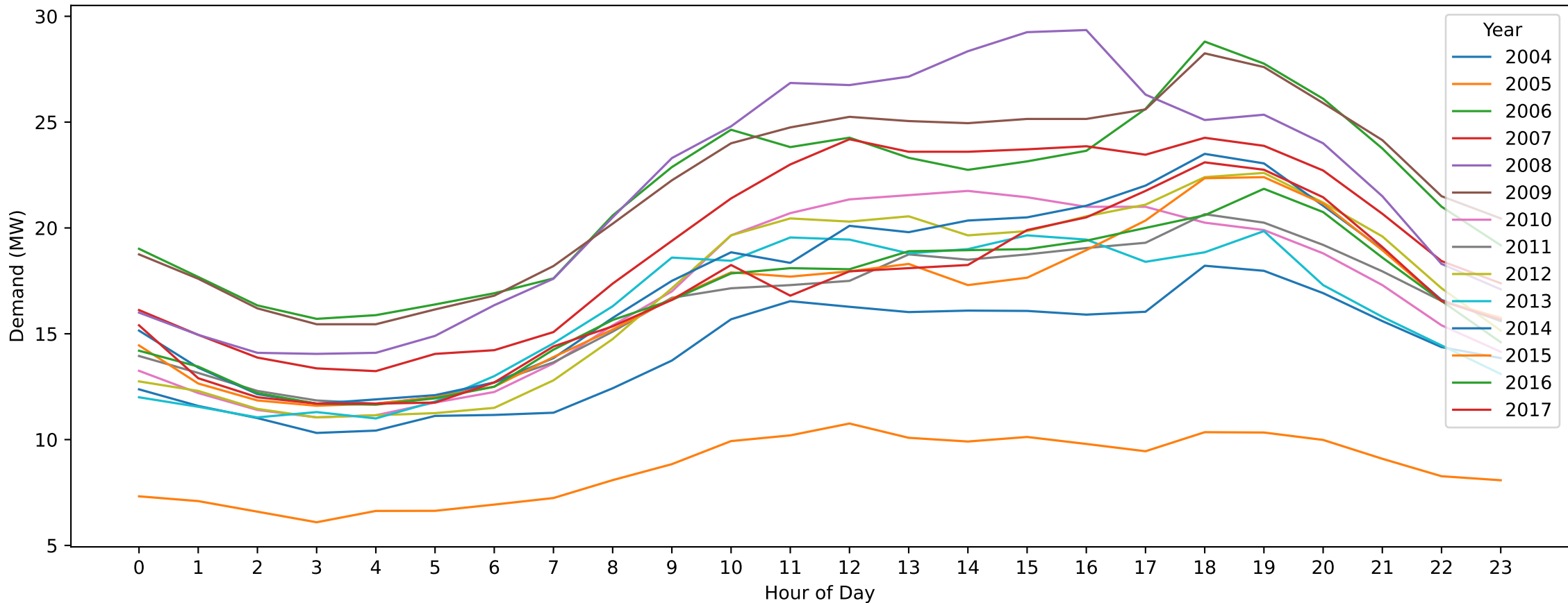
FTN — Easter Monday (Hourly Demand Across Years)
