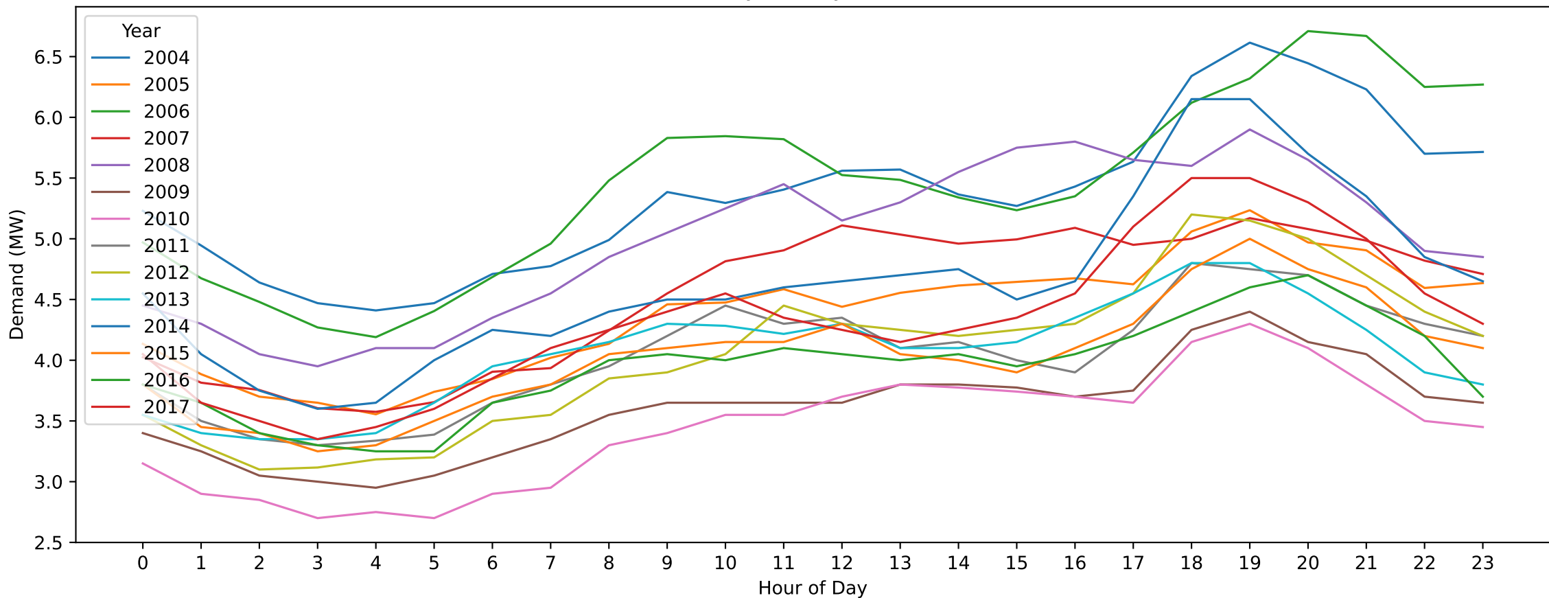
OE — Easter Monday (Hourly Demand Across Years)
