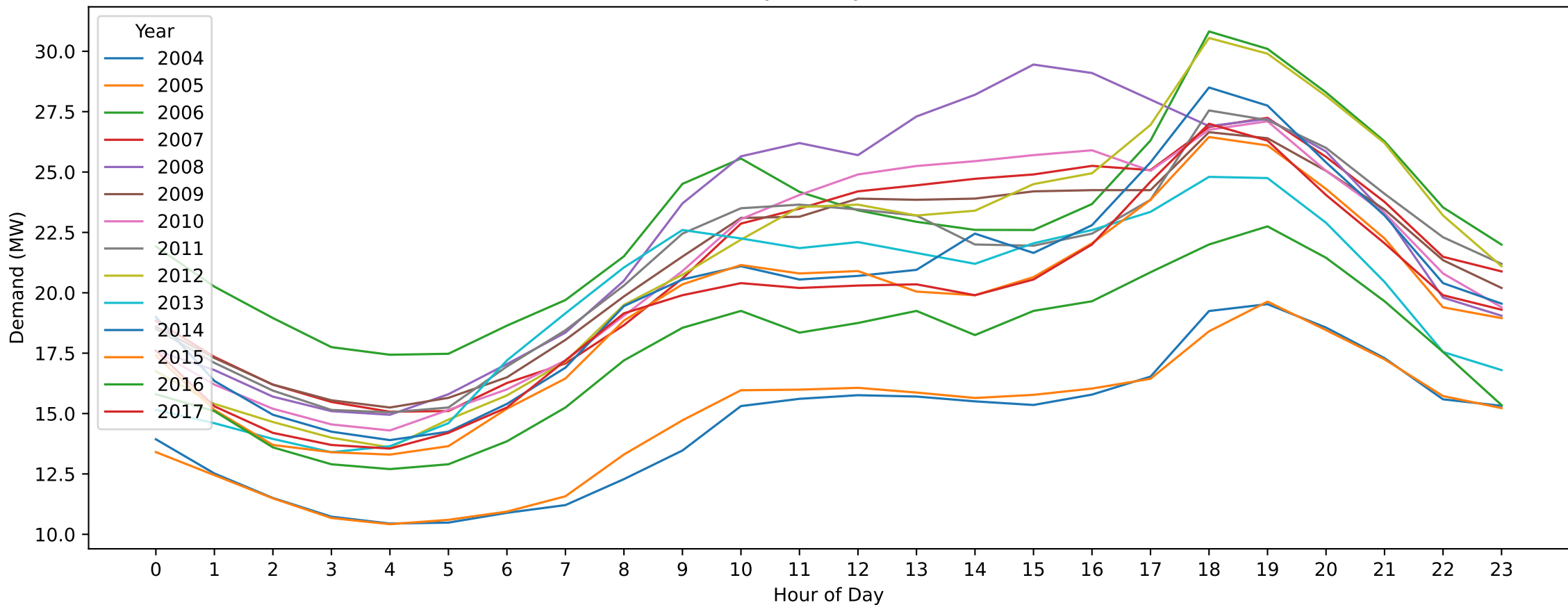
NW — Easter Monday (Hourly Demand Across Years)
