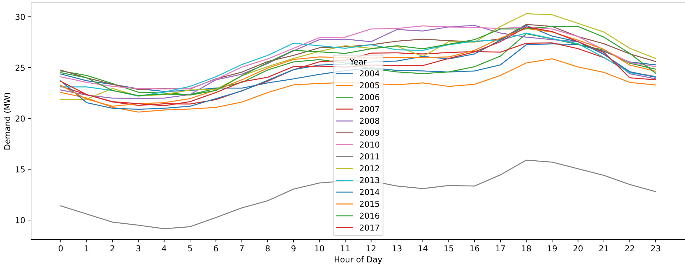
BH — Easter Monday (Hourly Demand Across Years)
