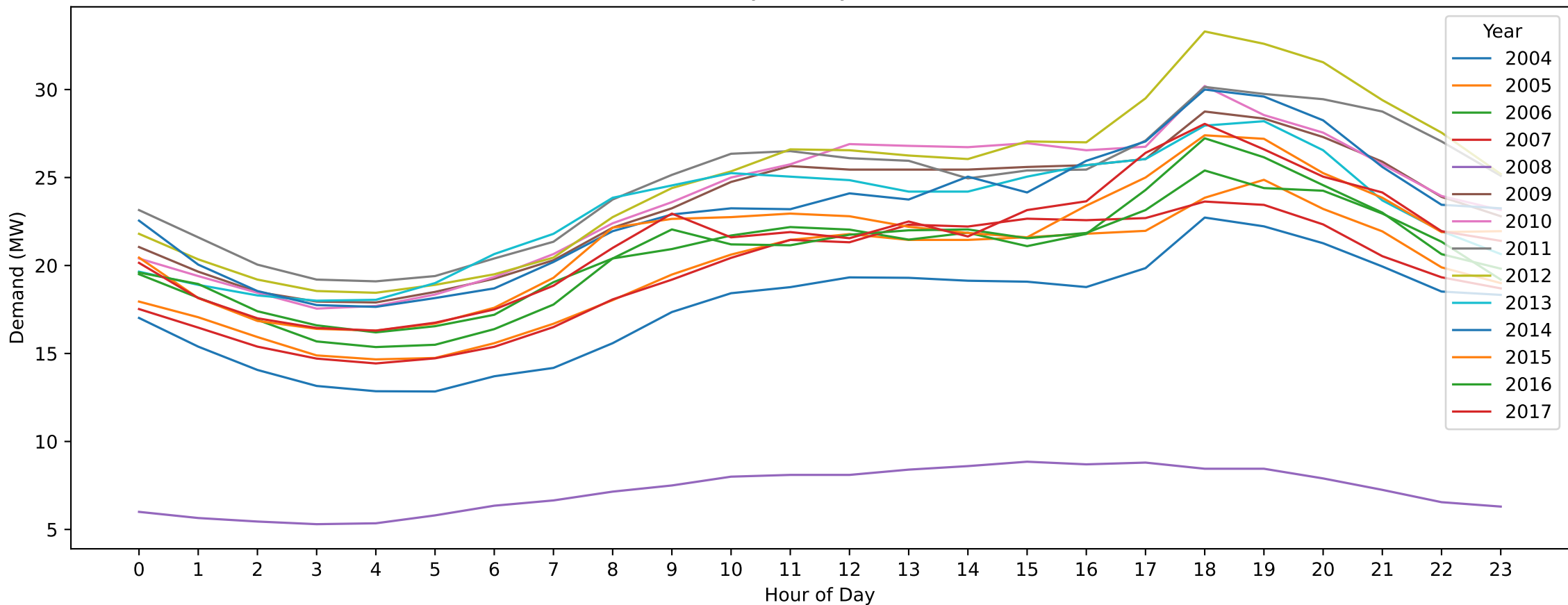
EB — Easter Monday (Hourly Demand Across Years)
