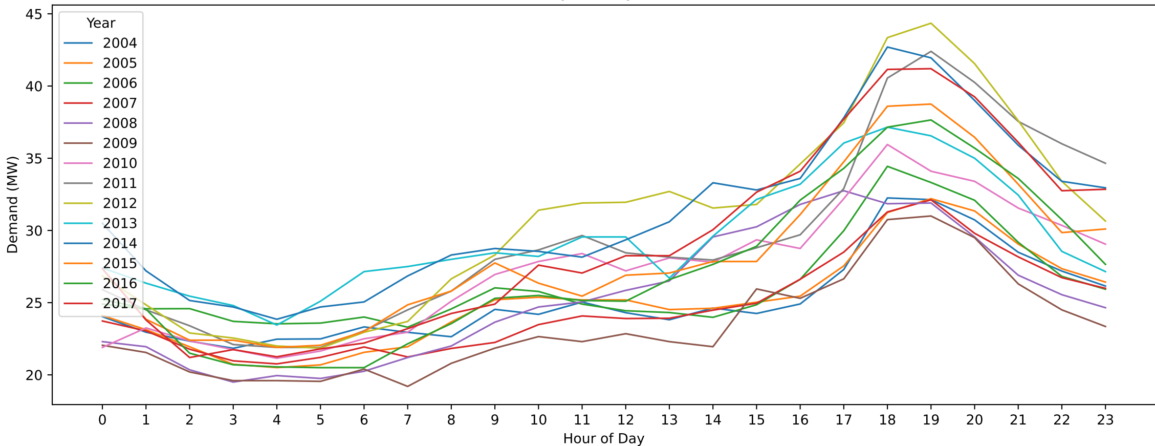
CRM — Easter Monday (Hourly Demand Across Years)
