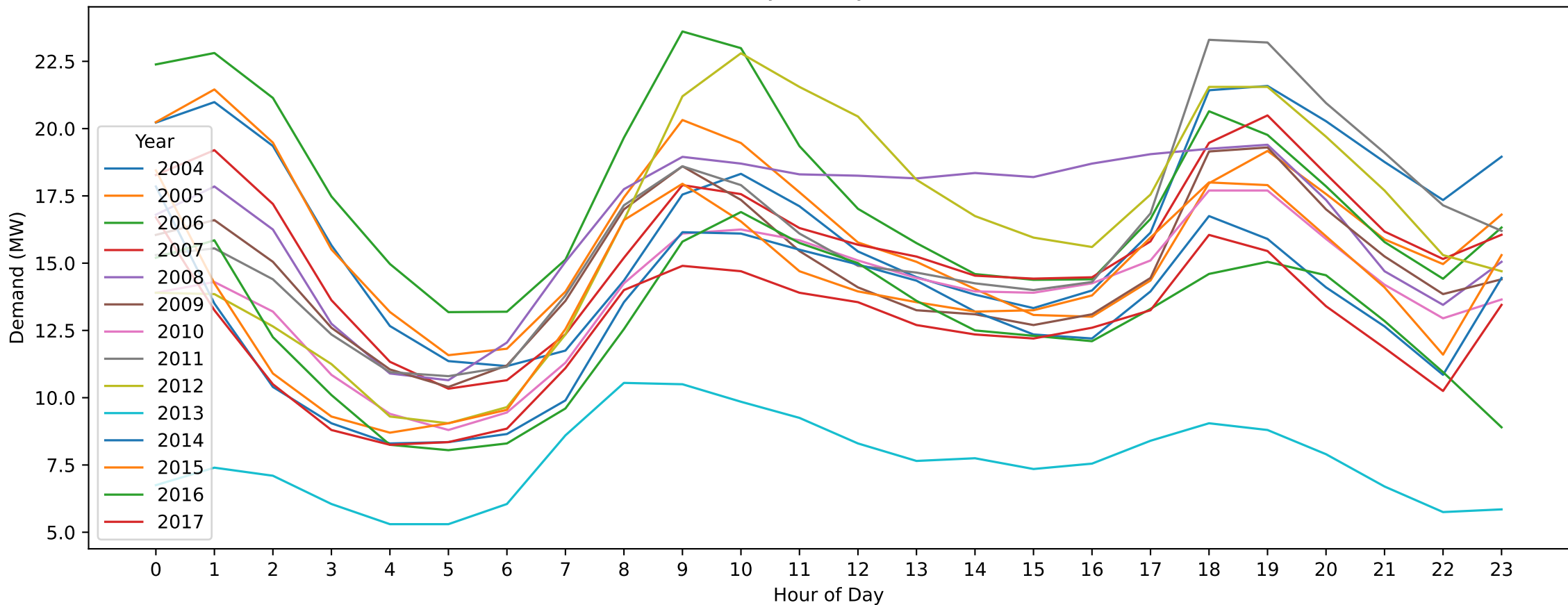
STO — Easter Monday (Hourly Demand Across Years)
