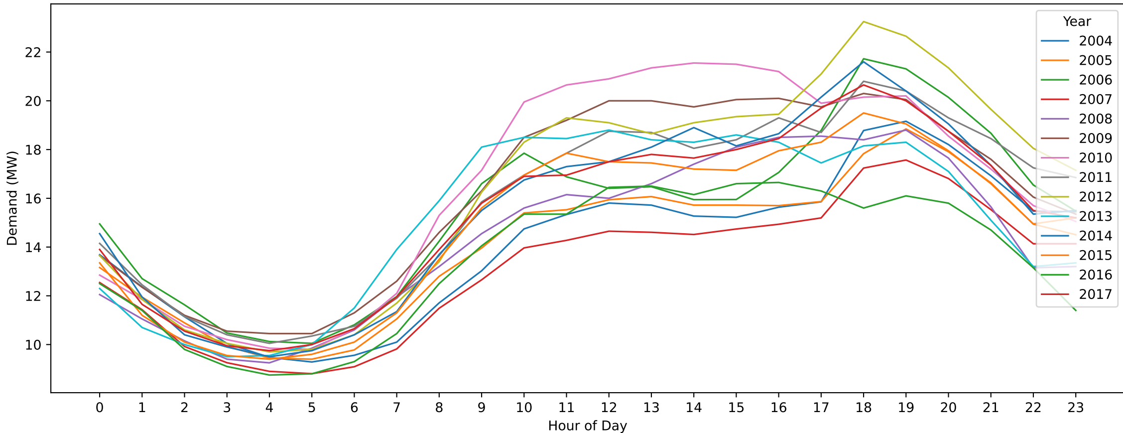
WD — Easter Monday (Hourly Demand Across Years)
