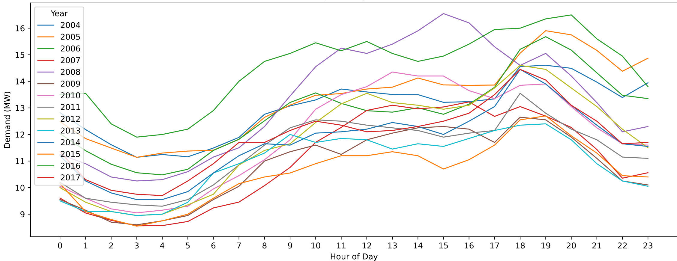
HT — Easter Monday (Hourly Demand Across Years)
