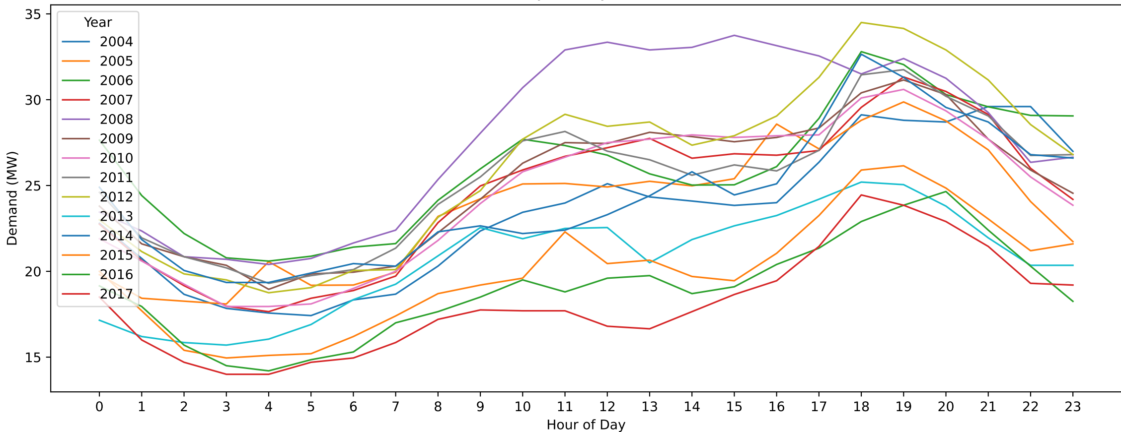
NP — Easter Monday (Hourly Demand Across Years)
