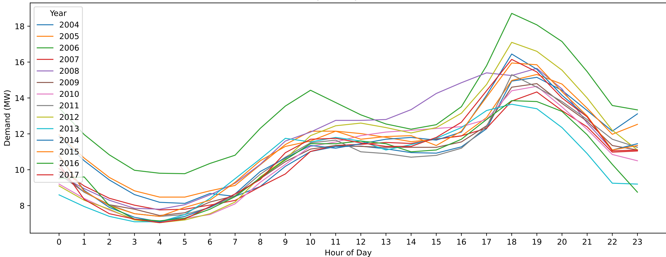
M — Easter Monday (Hourly Demand Across Years)
