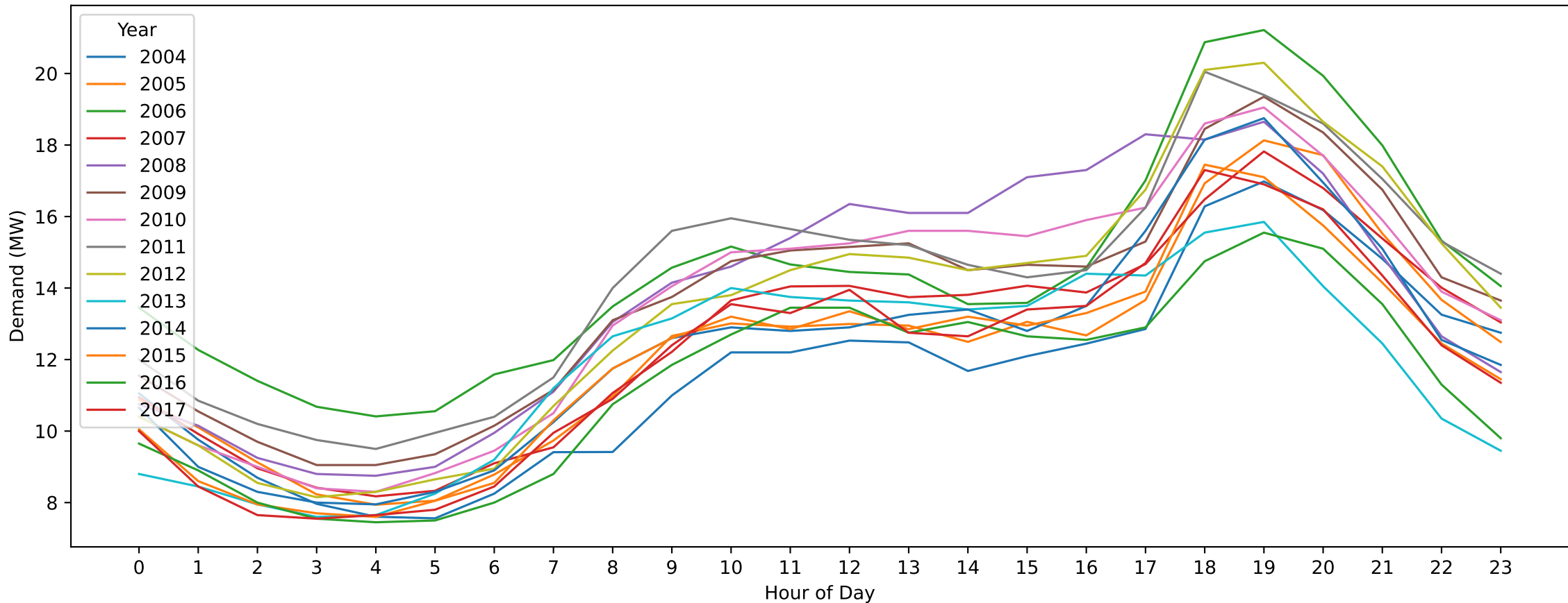
NB — Easter Monday (Hourly Demand Across Years)
