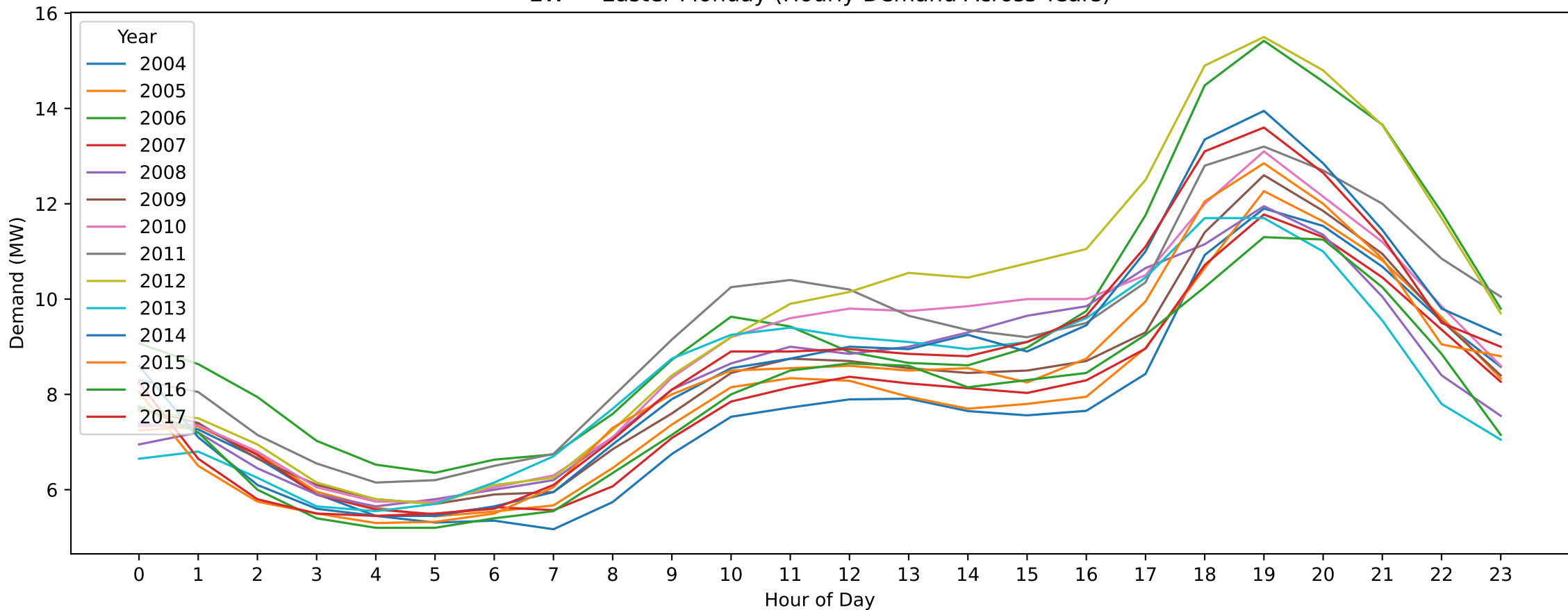
EW — Easter Monday (Hourly Demand Across Years)
