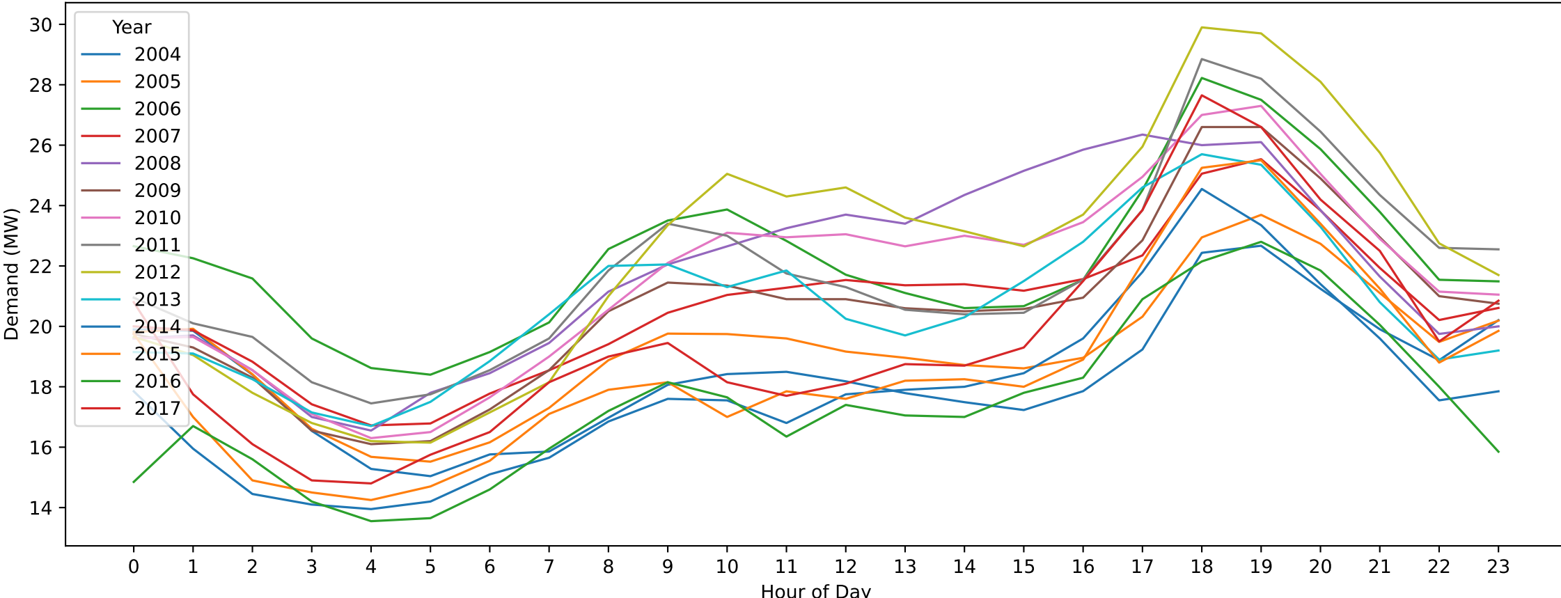
HGS — Easter Monday (Hourly Demand Across Years)
