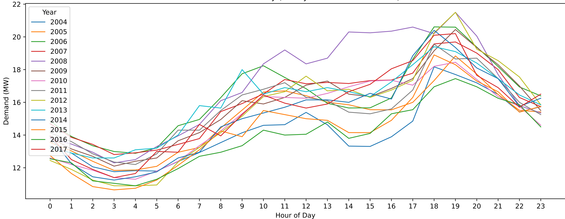
MC — Easter Monday (Hourly Demand Across Years)
