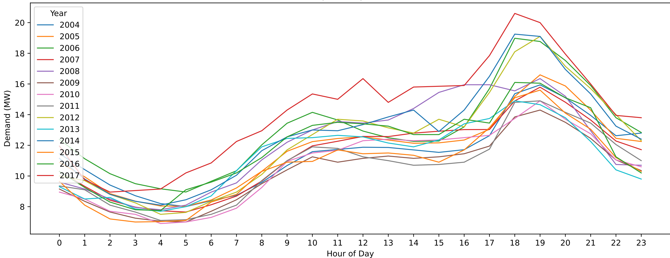
MR — Easter Monday (Hourly Demand Across Years)
