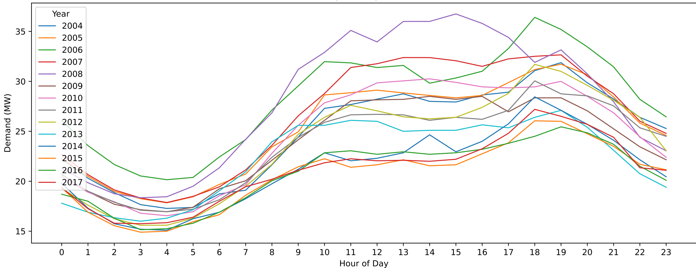
GW — Easter Monday (Hourly Demand Across Years)
