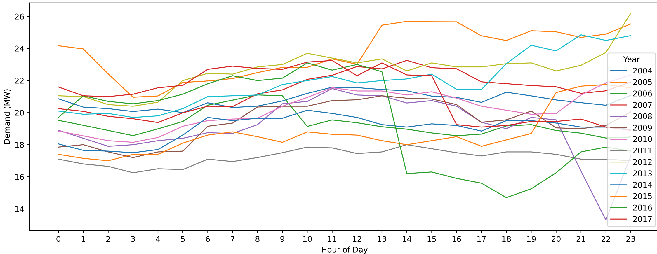
DSH — Easter Monday (Hourly Demand Across Years)
