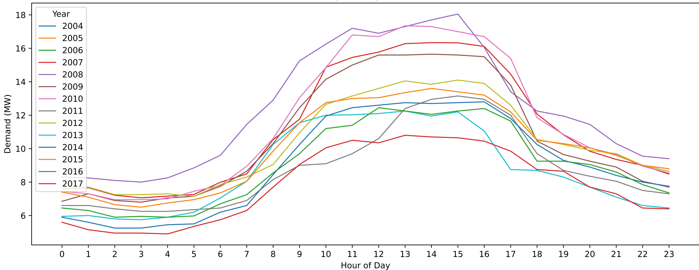
CM — Easter Monday (Hourly Demand Across Years)
