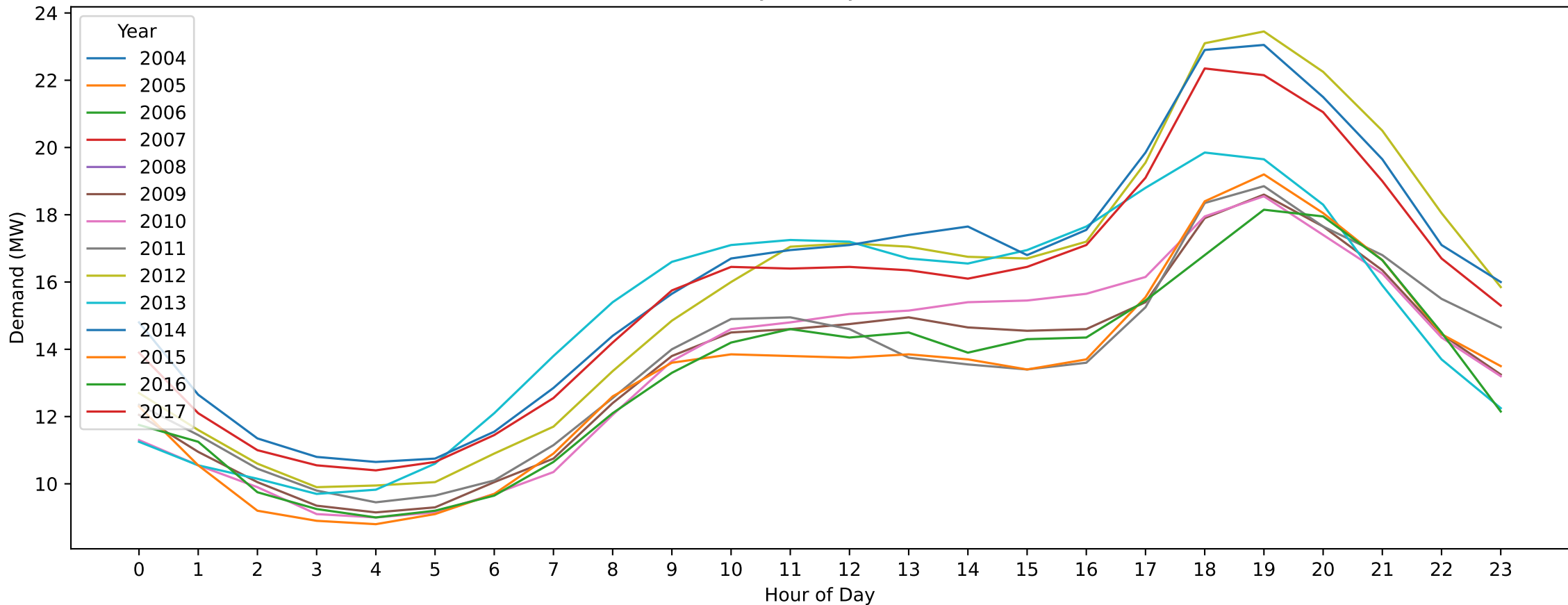
CFD — Easter Monday (Hourly Demand Across Years)
