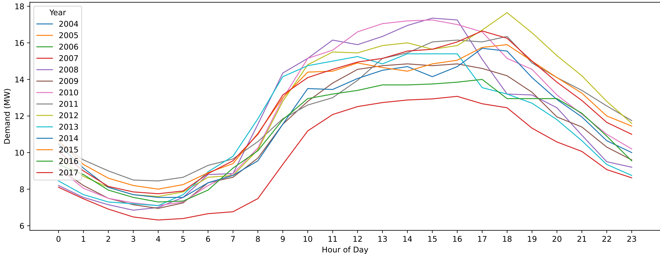
OAK — Easter Monday (Hourly Demand Across Years)
