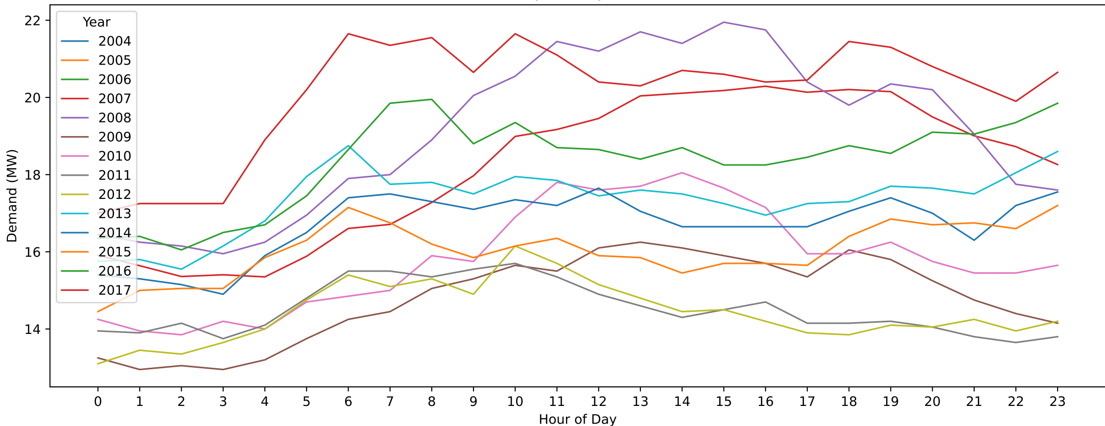
DVY — Easter Monday (Hourly Demand Across Years)
