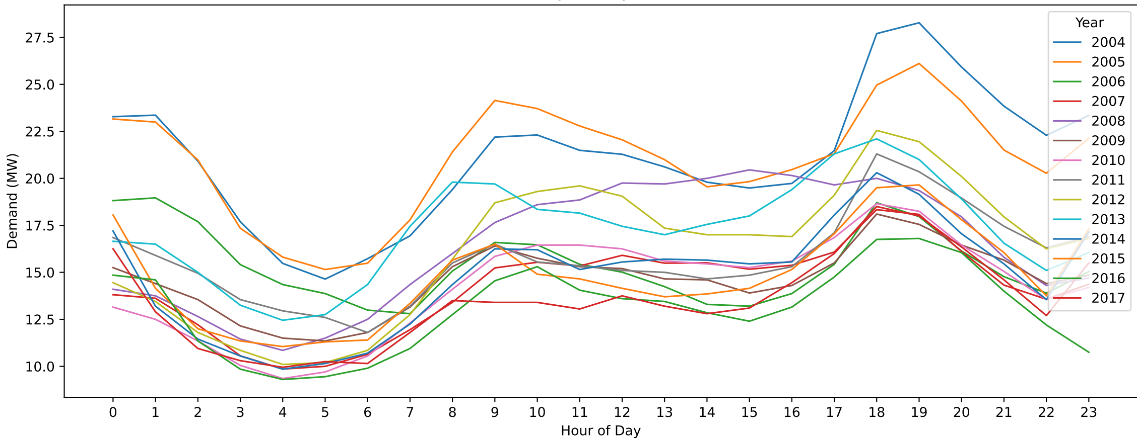
RBD — Easter Monday (Hourly Demand Across Years)
