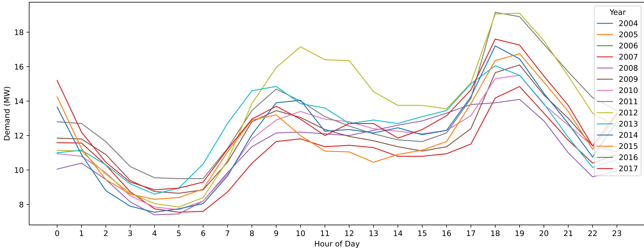
DMA — Easter Monday (Hourly Demand Across Years)
