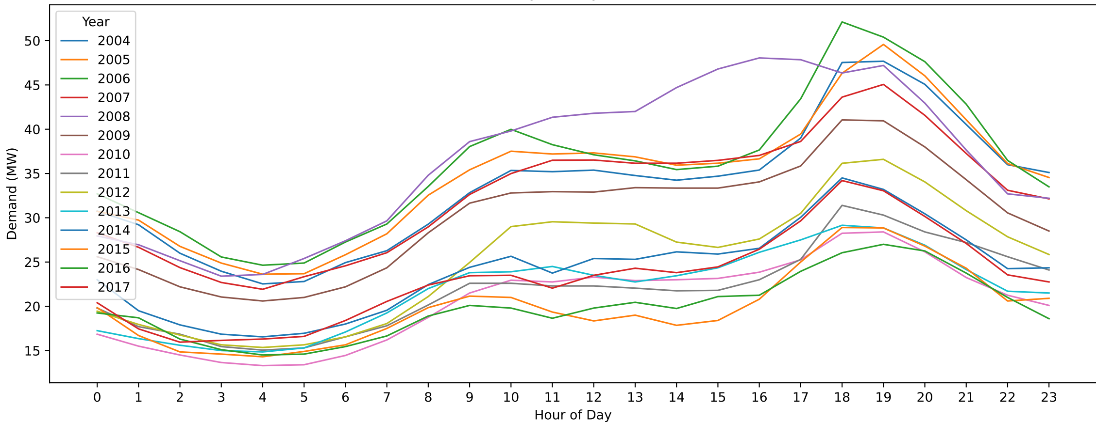
FSH — Easter Monday (Hourly Demand Across Years)
