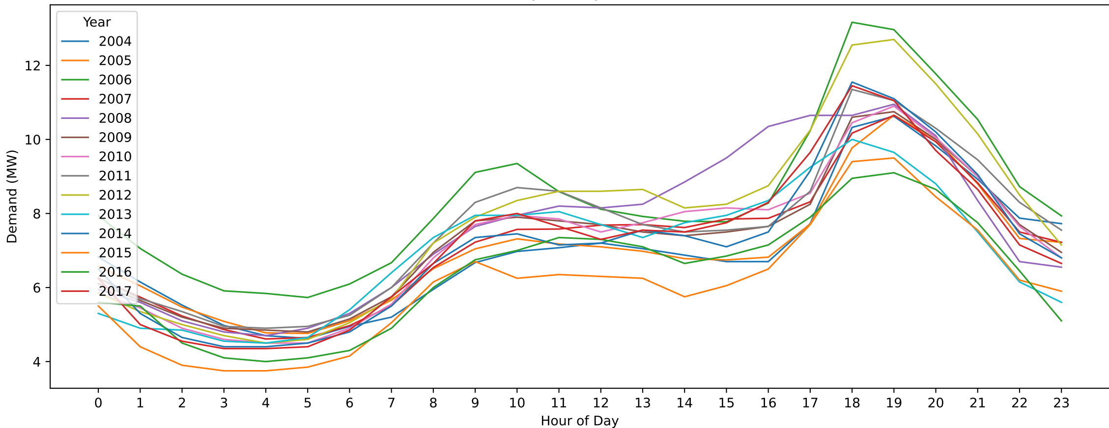
BR — Easter Monday (Hourly Demand Across Years)
