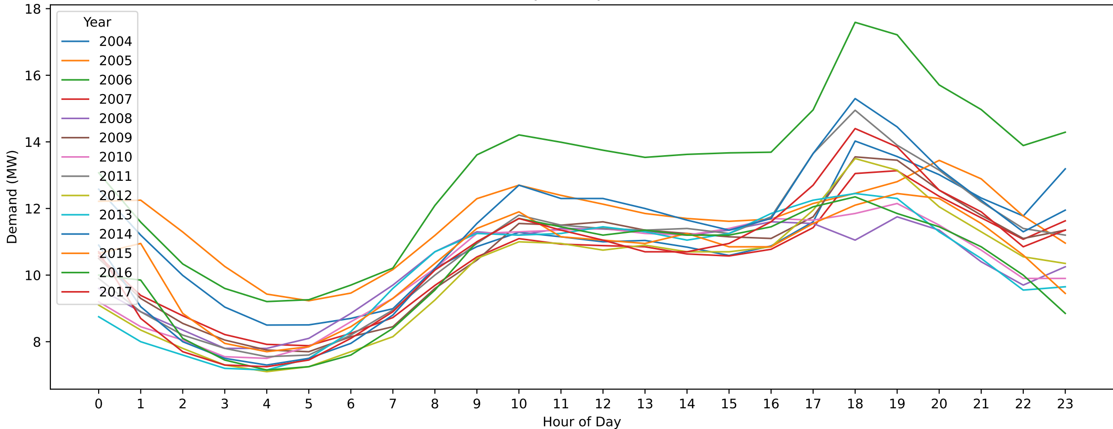
M — Easter Saturday (Hourly Demand Across Years)
