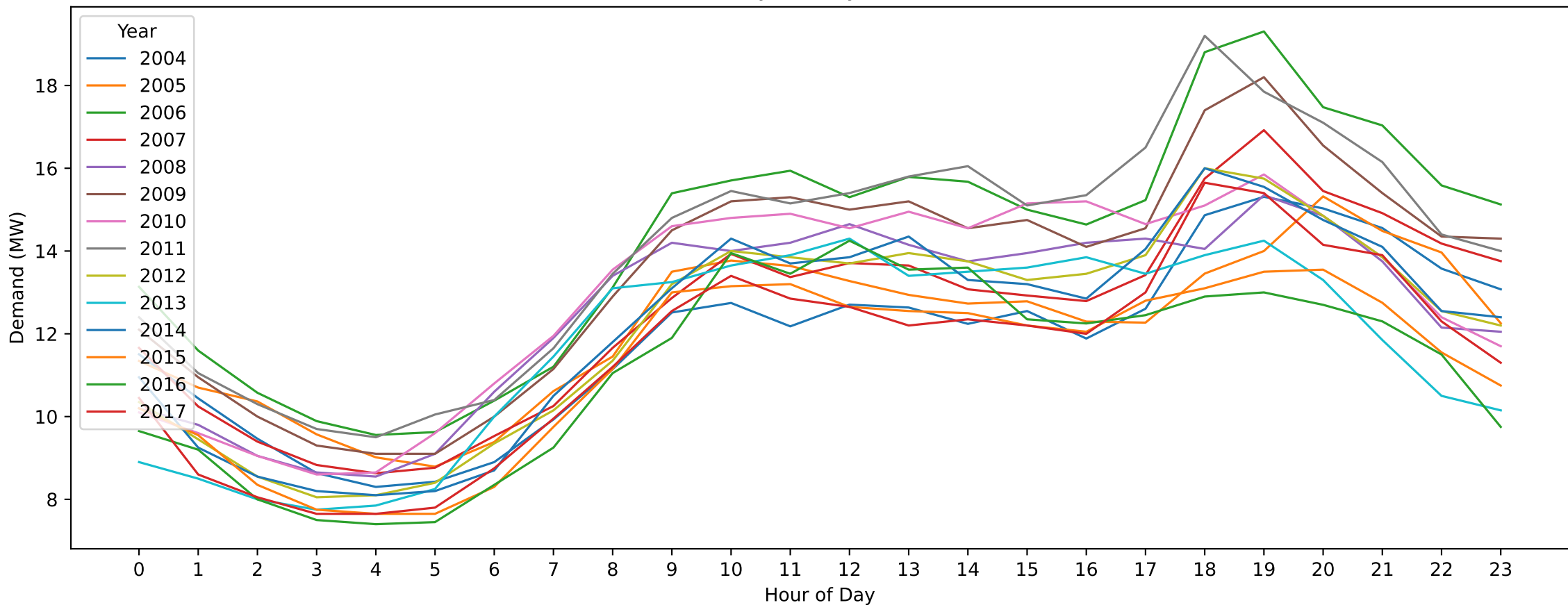
NB — Easter Saturday (Hourly Demand Across Years)
