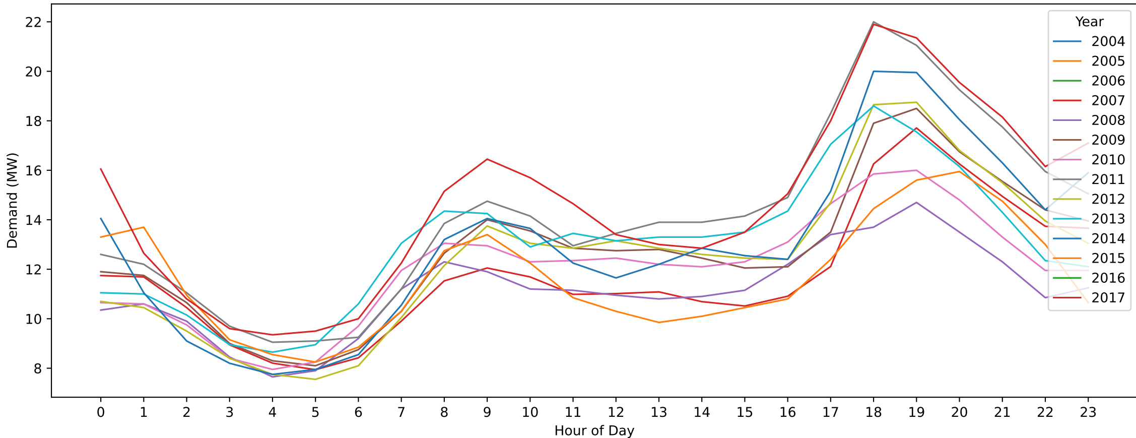
DMA — Easter Saturday (Hourly Demand Across Years)
