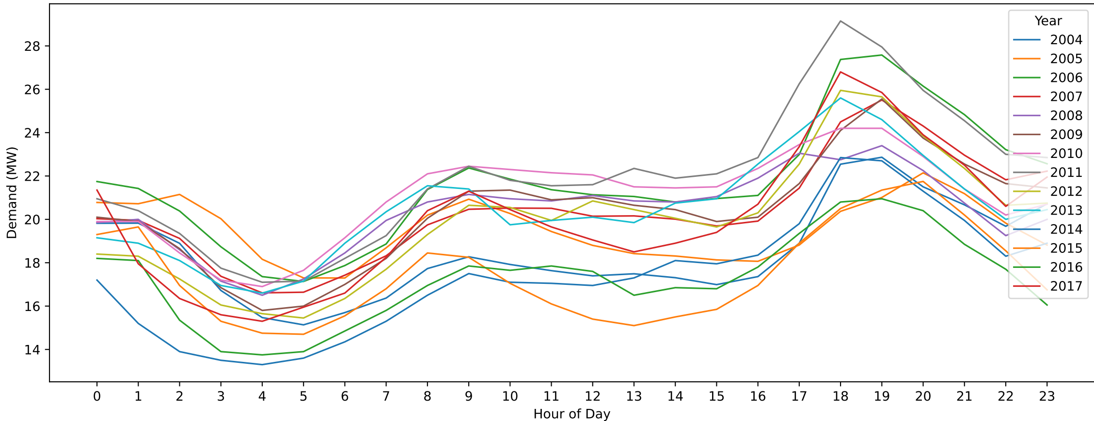
HGS — Easter Saturday (Hourly Demand Across Years)
