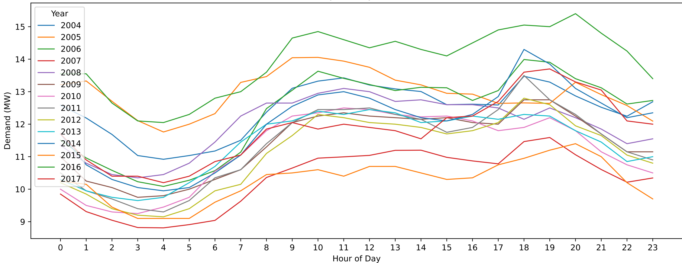
HT — Easter Saturday (Hourly Demand Across Years)
