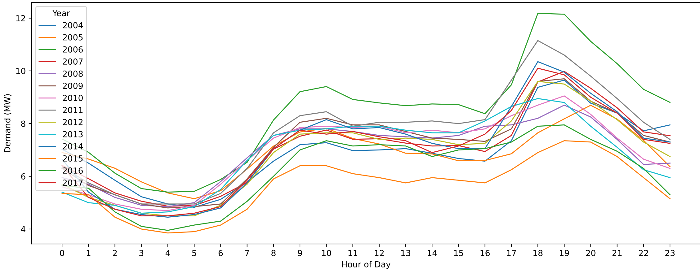
BR — Easter Saturday (Hourly Demand Across Years)
