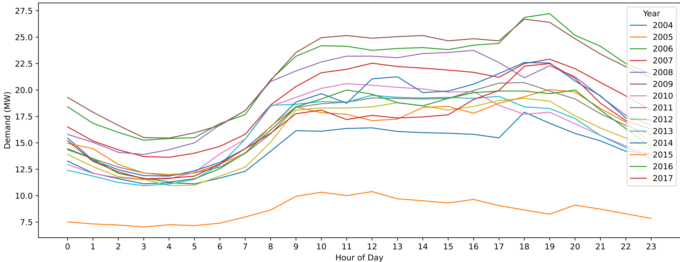
FTN — Easter Saturday (Hourly Demand Across Years)
