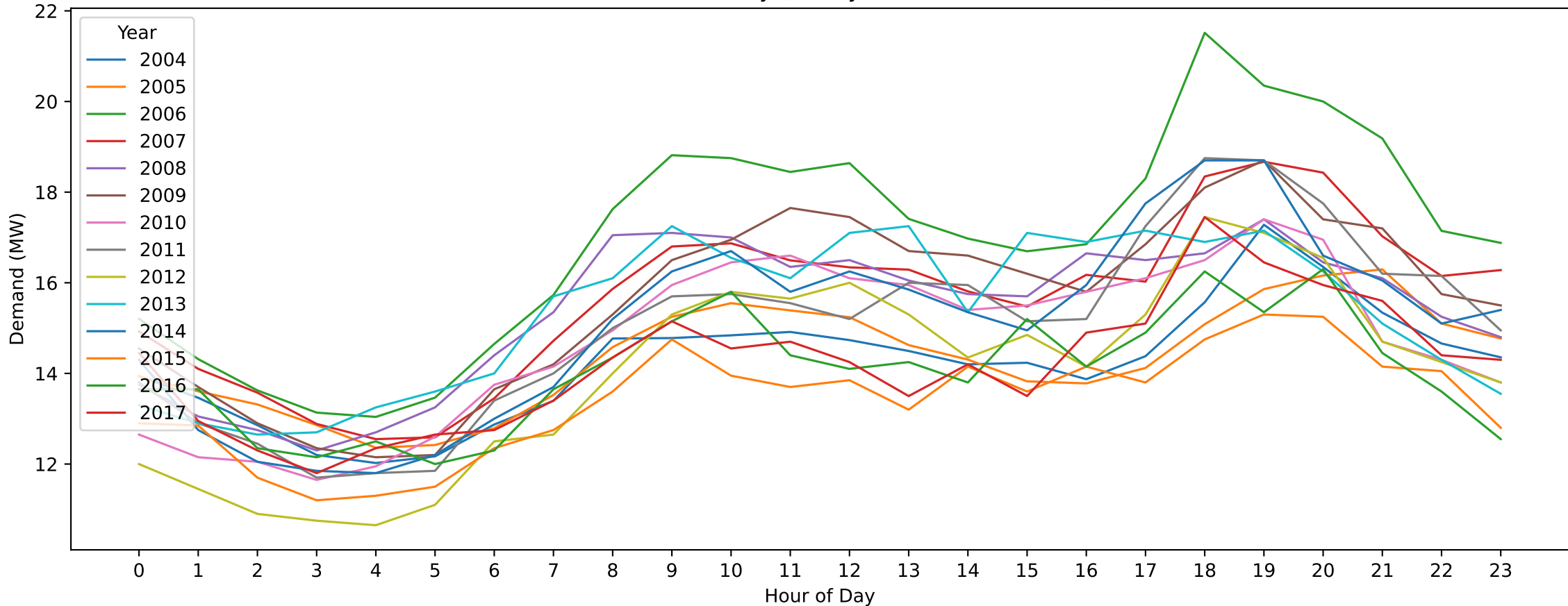
MC — Easter Saturday (Hourly Demand Across Years)
