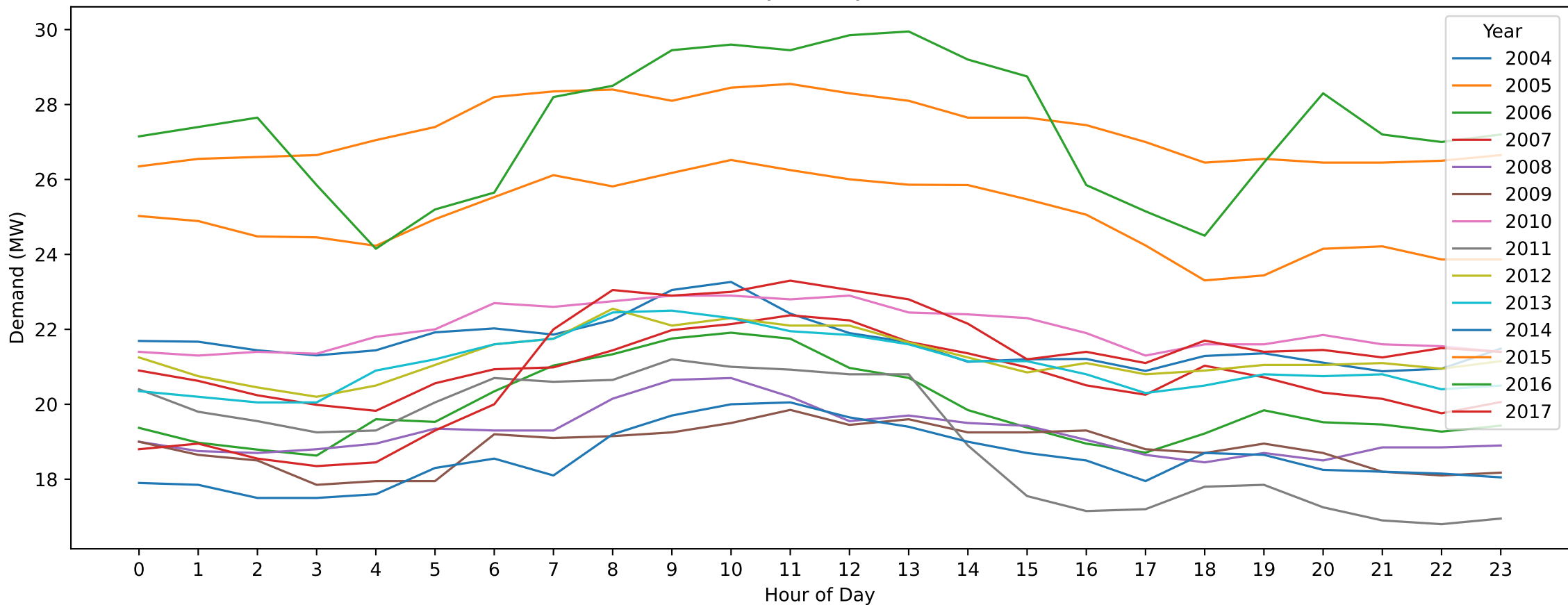
DSH — Easter Saturday (Hourly Demand Across Years)
