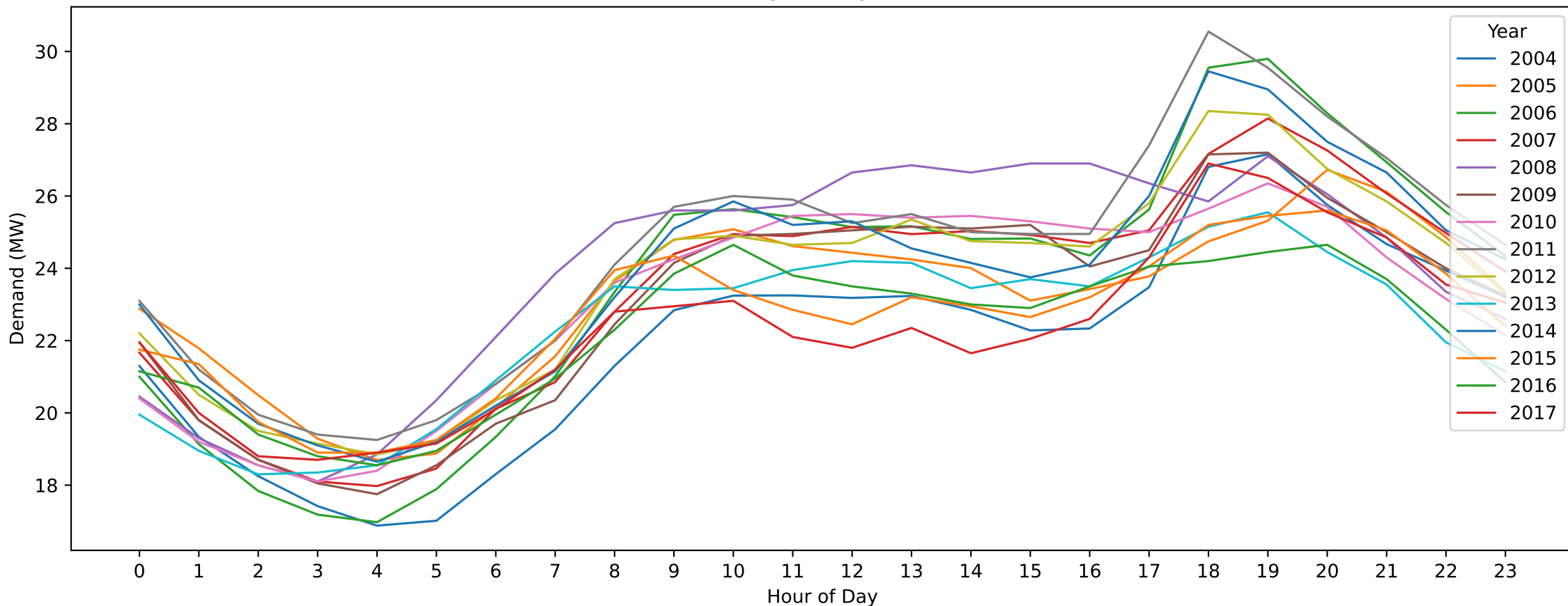
MGE — Easter Saturday (Hourly Demand Across Years)
