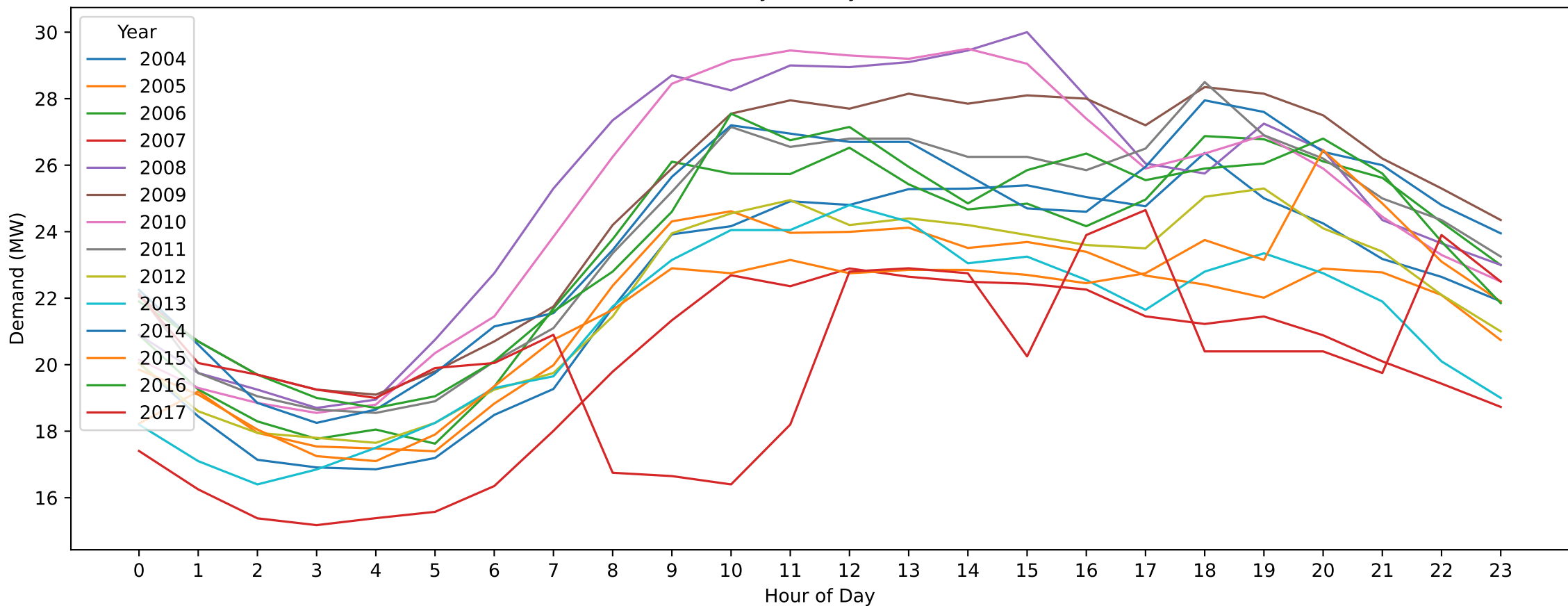
DN — Easter Saturday (Hourly Demand Across Years)
