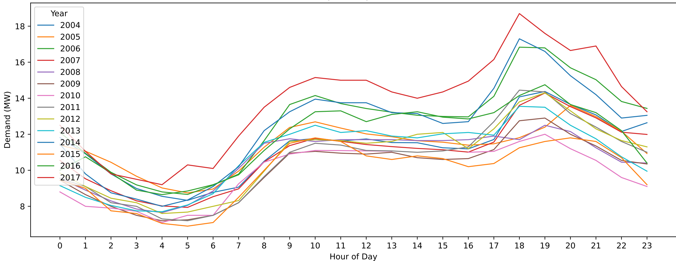
MR — Easter Saturday (Hourly Demand Across Years)
