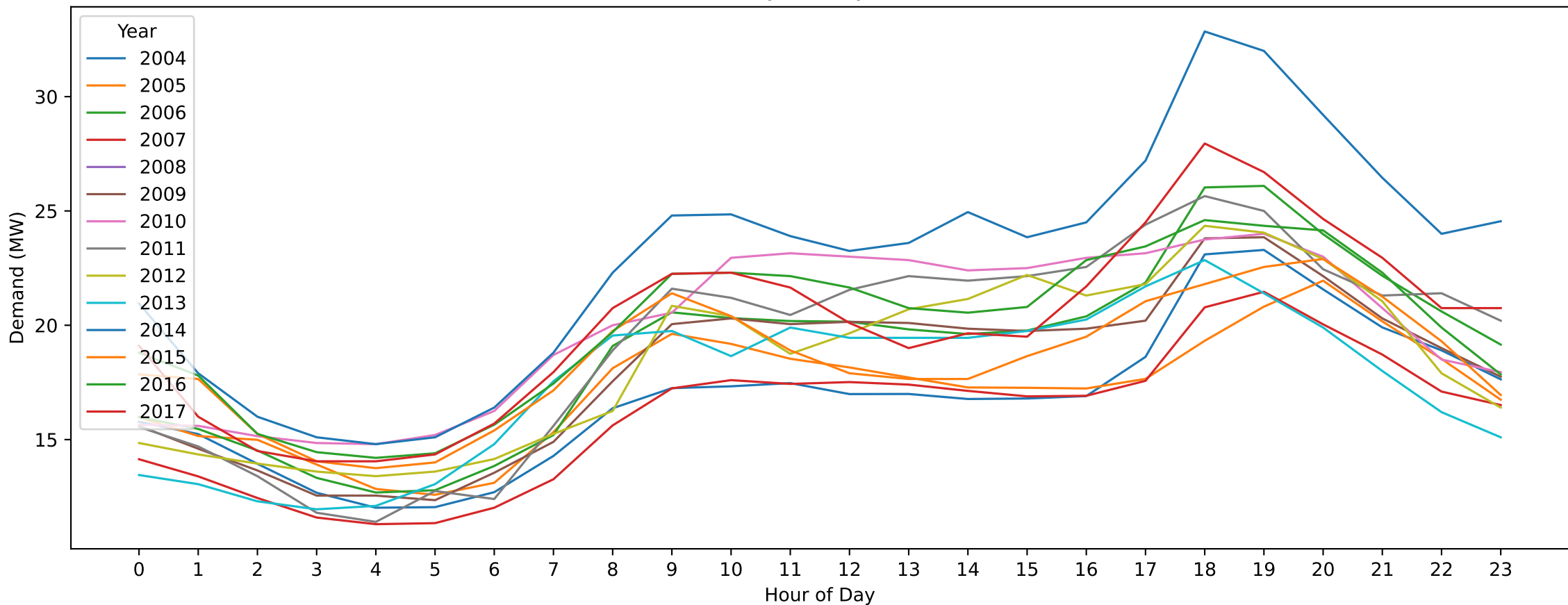
MTN — Easter Saturday (Hourly Demand Across Years)
