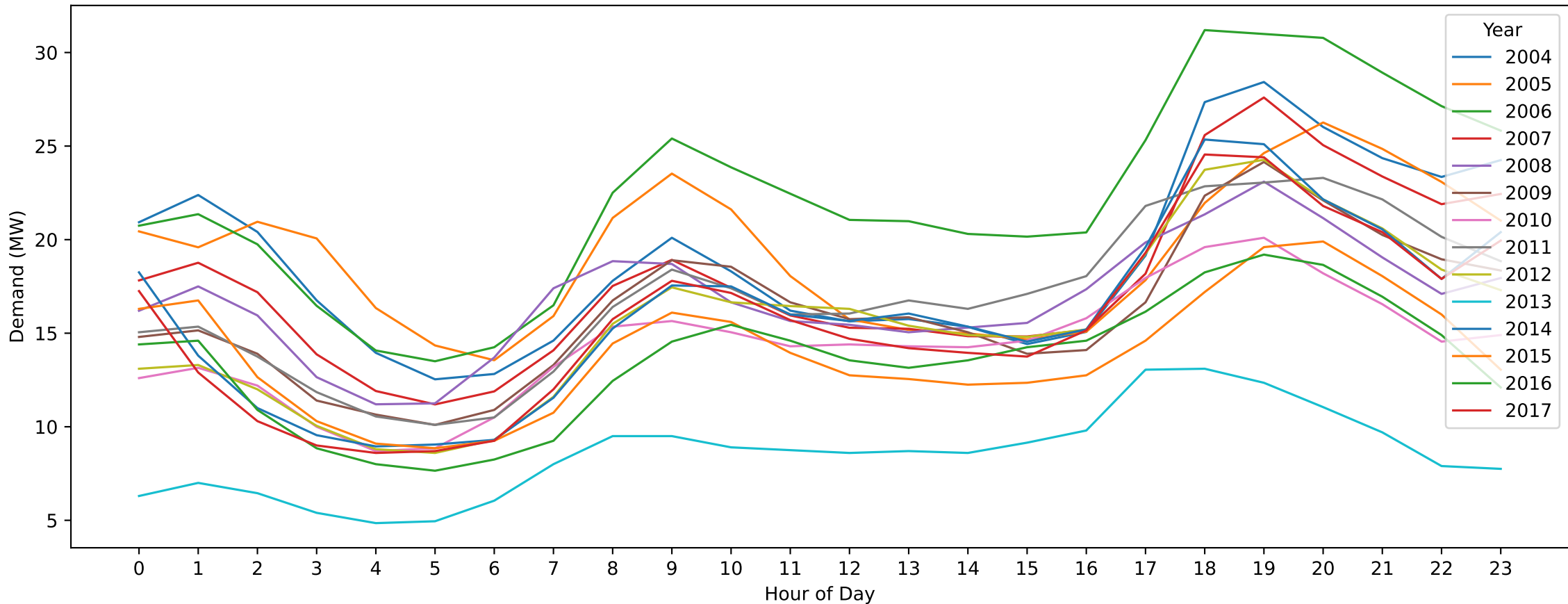
STO — Easter Saturday (Hourly Demand Across Years)
