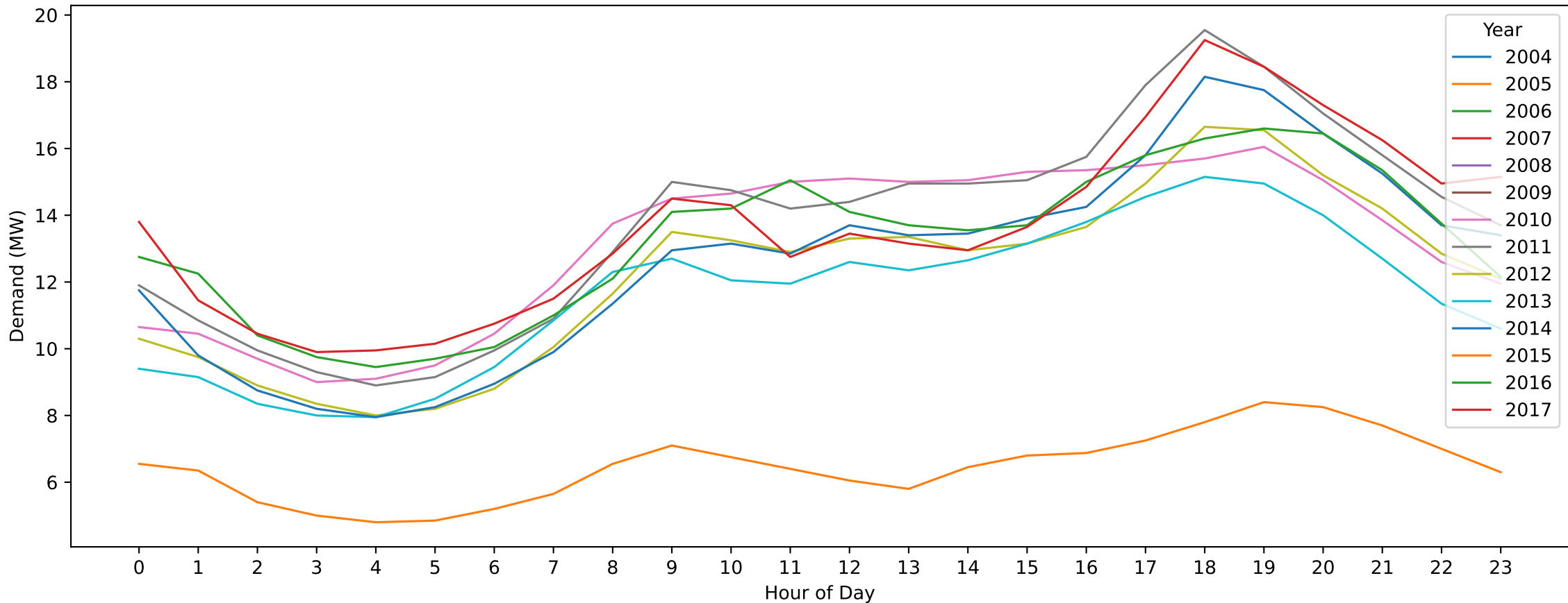
LWN — Easter Saturday (Hourly Demand Across Years)
