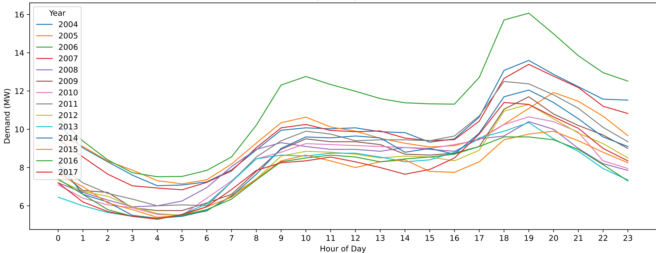
BT — Easter Saturday (Hourly Demand Across Years)
