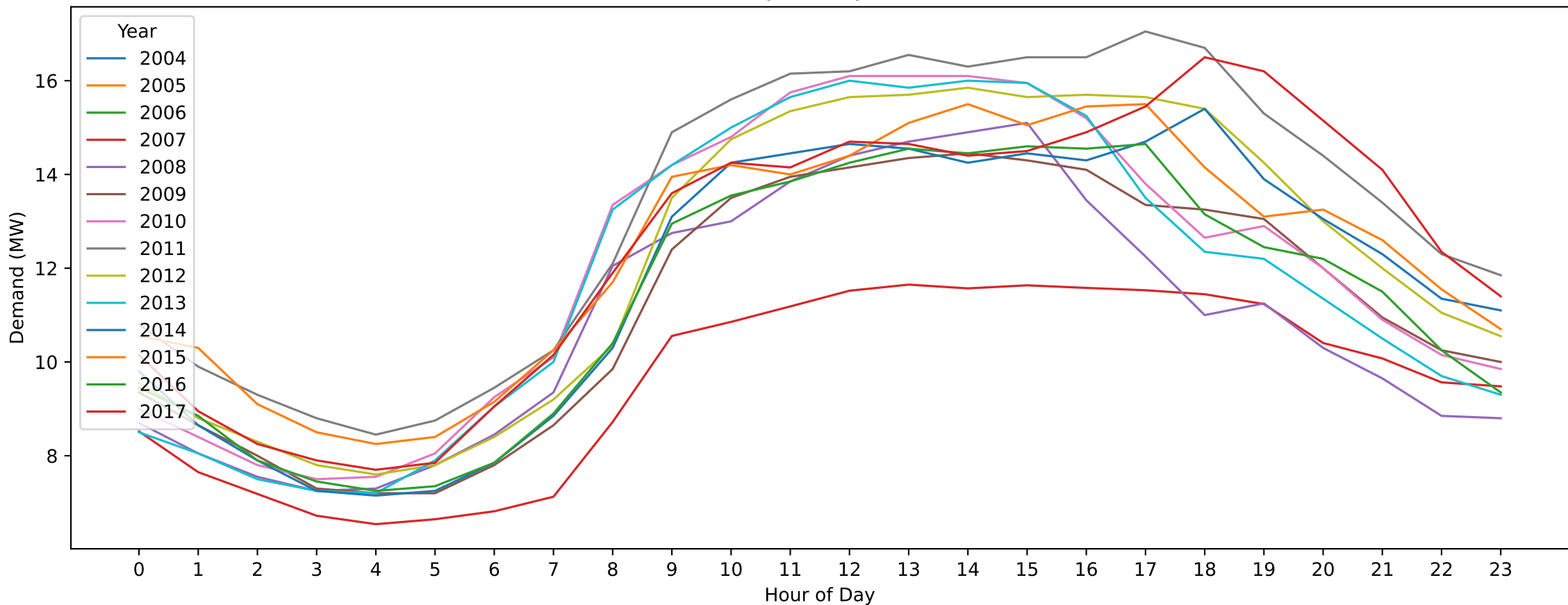
OAK — Easter Saturday (Hourly Demand Across Years)
