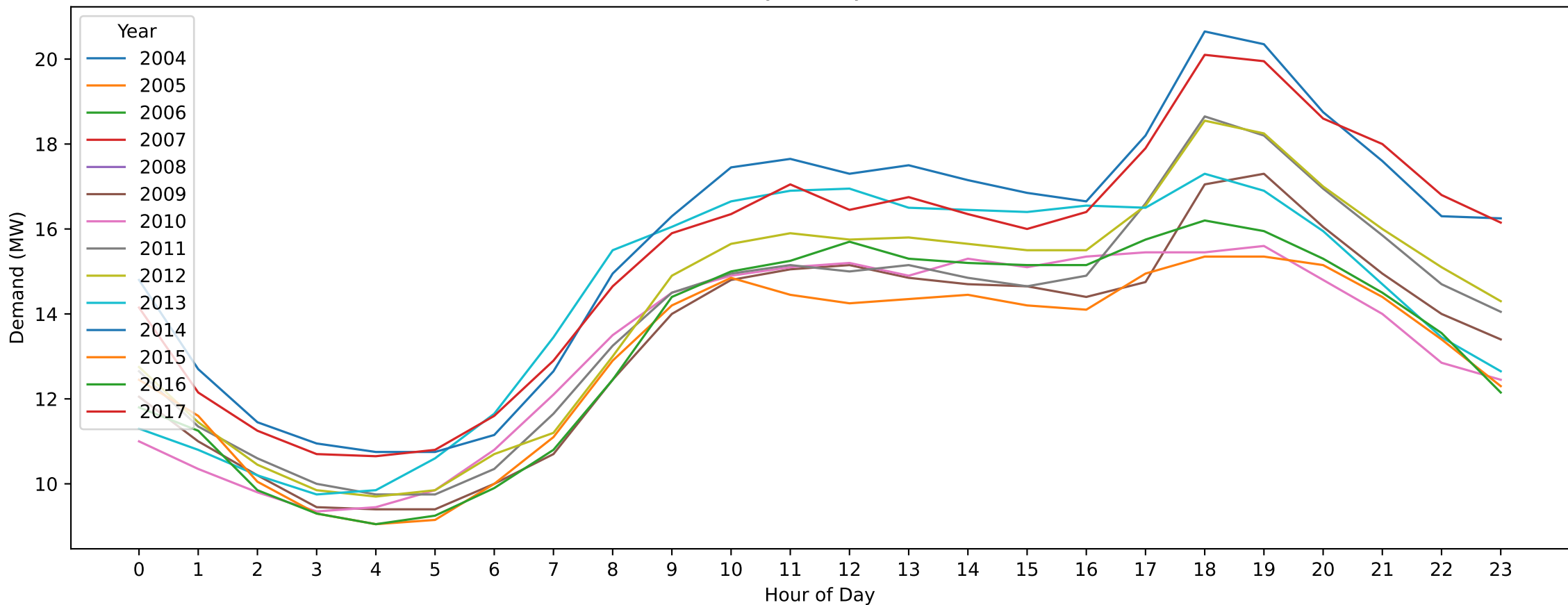
CFD — Easter Saturday (Hourly Demand Across Years)
