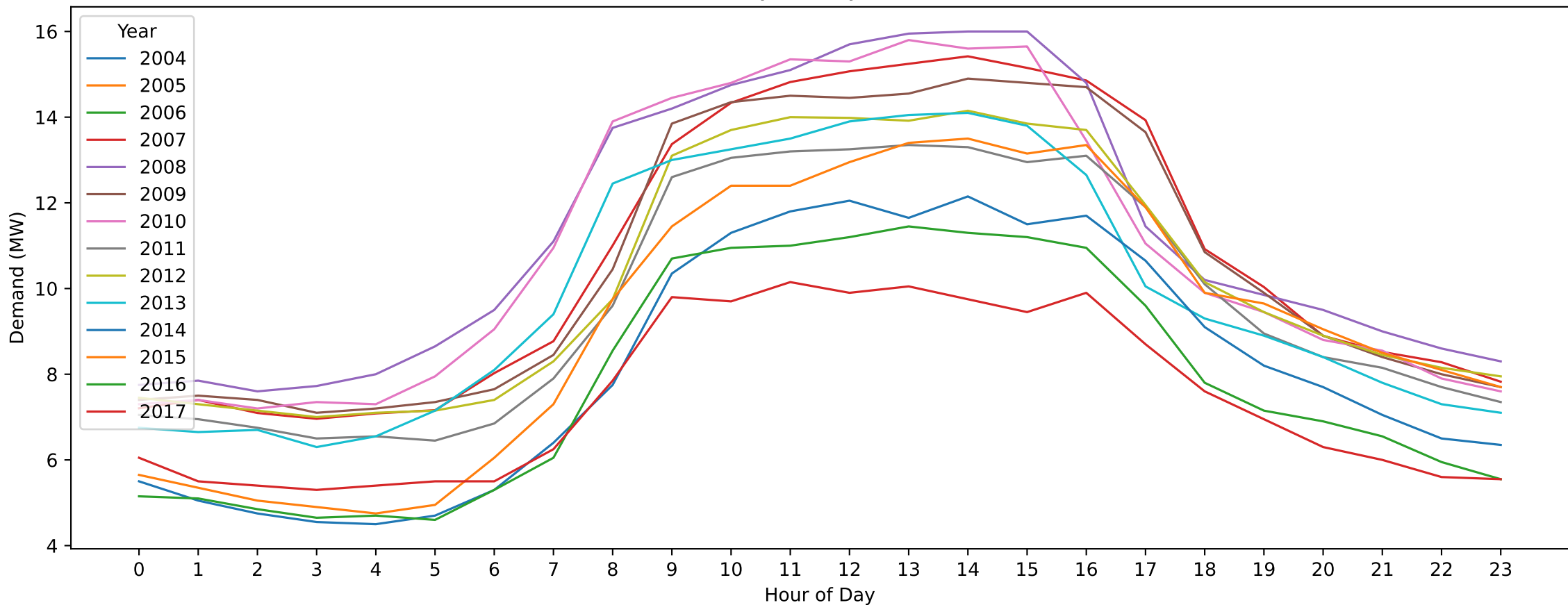
CM — Easter Saturday (Hourly Demand Across Years)
