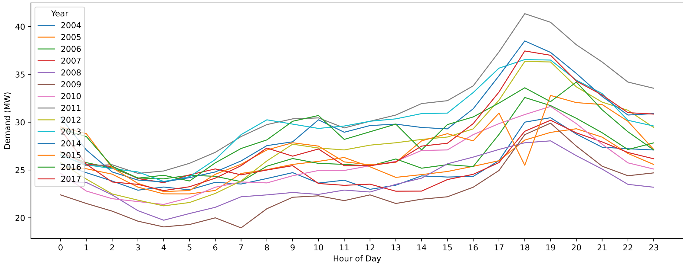
CRM — Easter Saturday (Hourly Demand Across Years)
