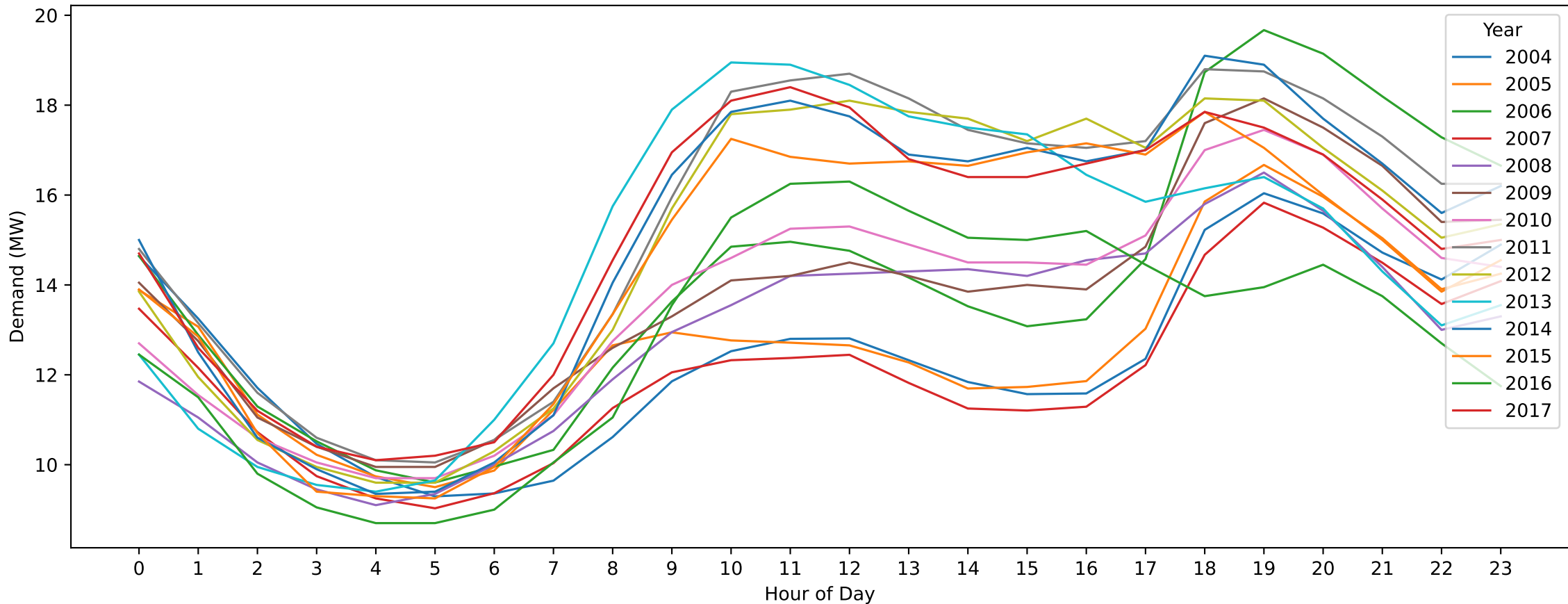
WD — Easter Sunday (Hourly Demand Across Years)
