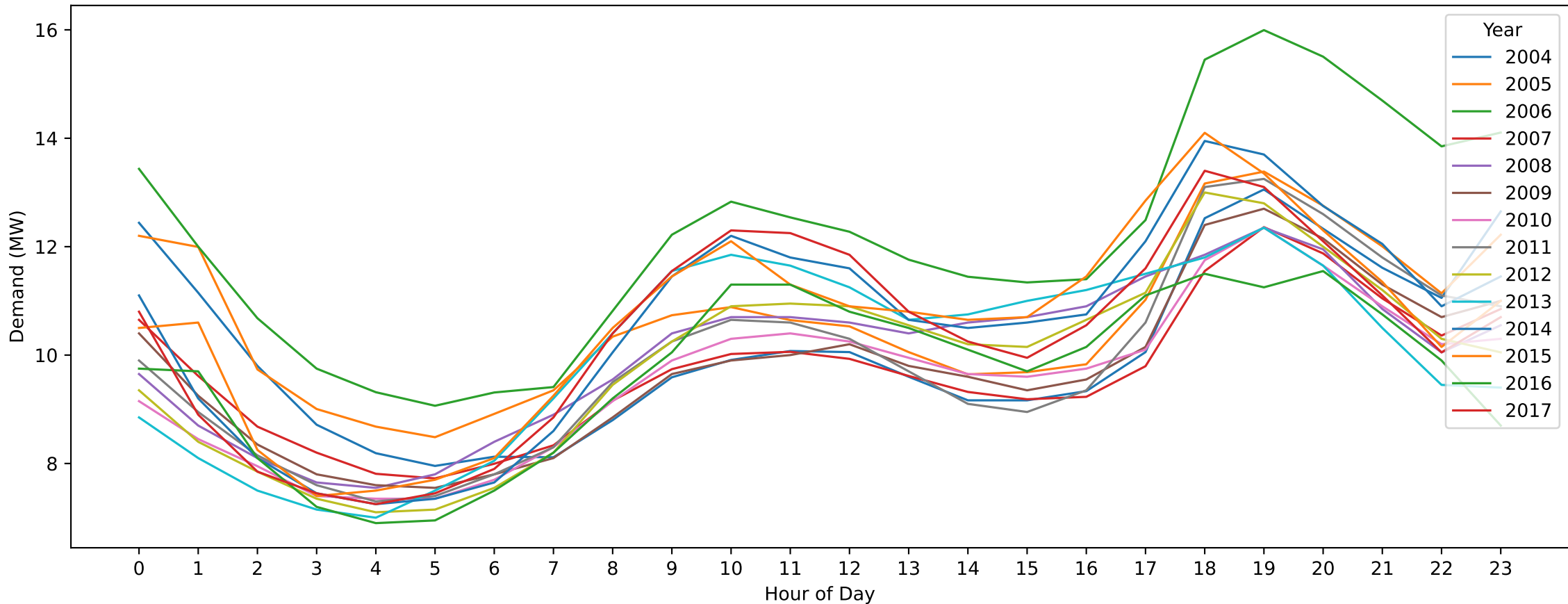
M — Easter Sunday (Hourly Demand Across Years)
