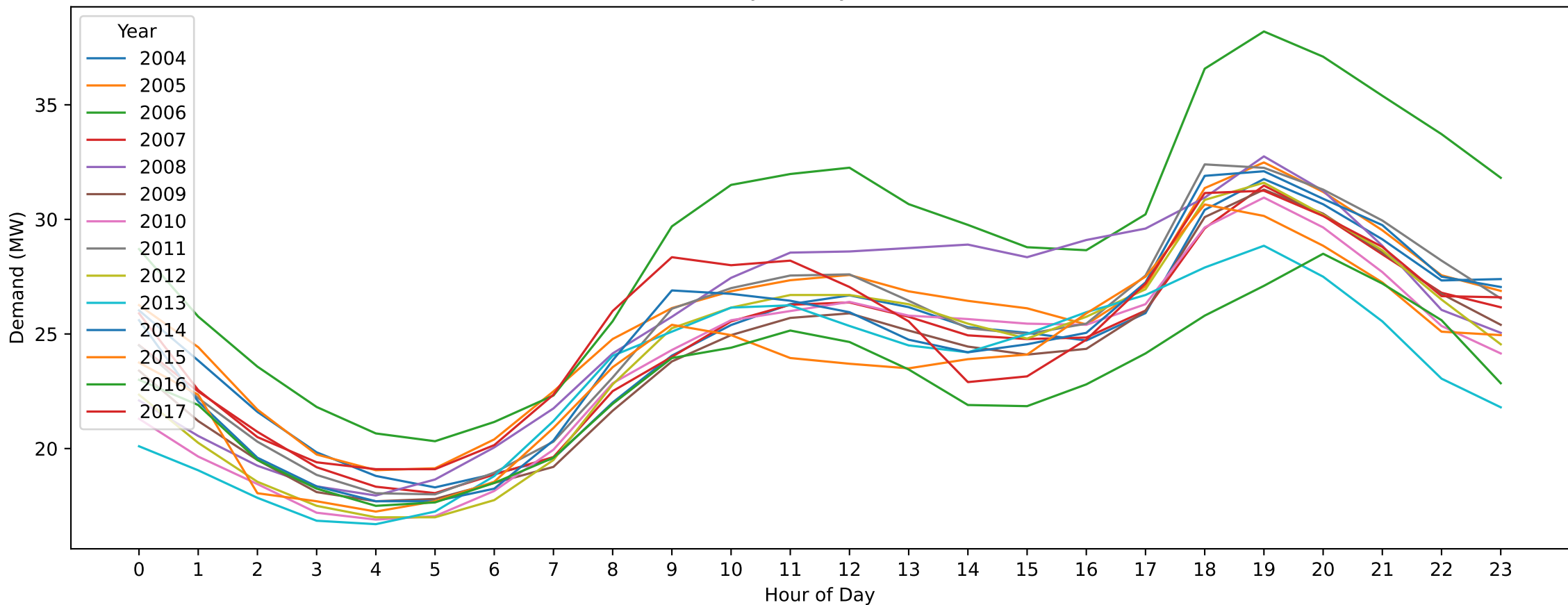
DC — Easter Sunday (Hourly Demand Across Years)
