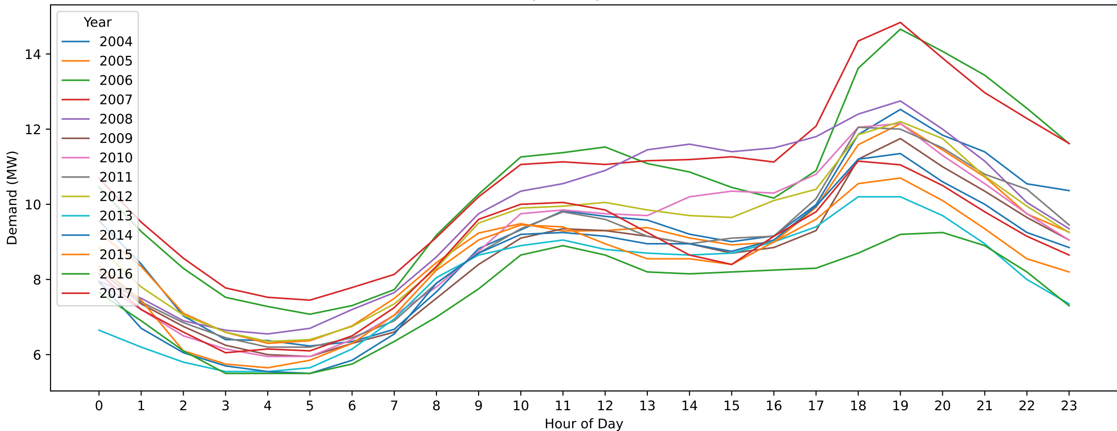
EL — Easter Sunday (Hourly Demand Across Years)
