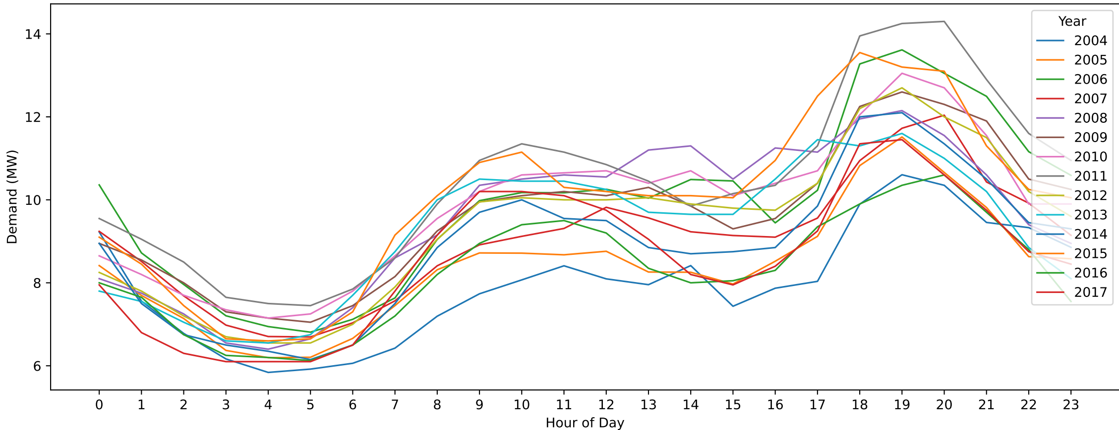
SR — Easter Sunday (Hourly Demand Across Years)
