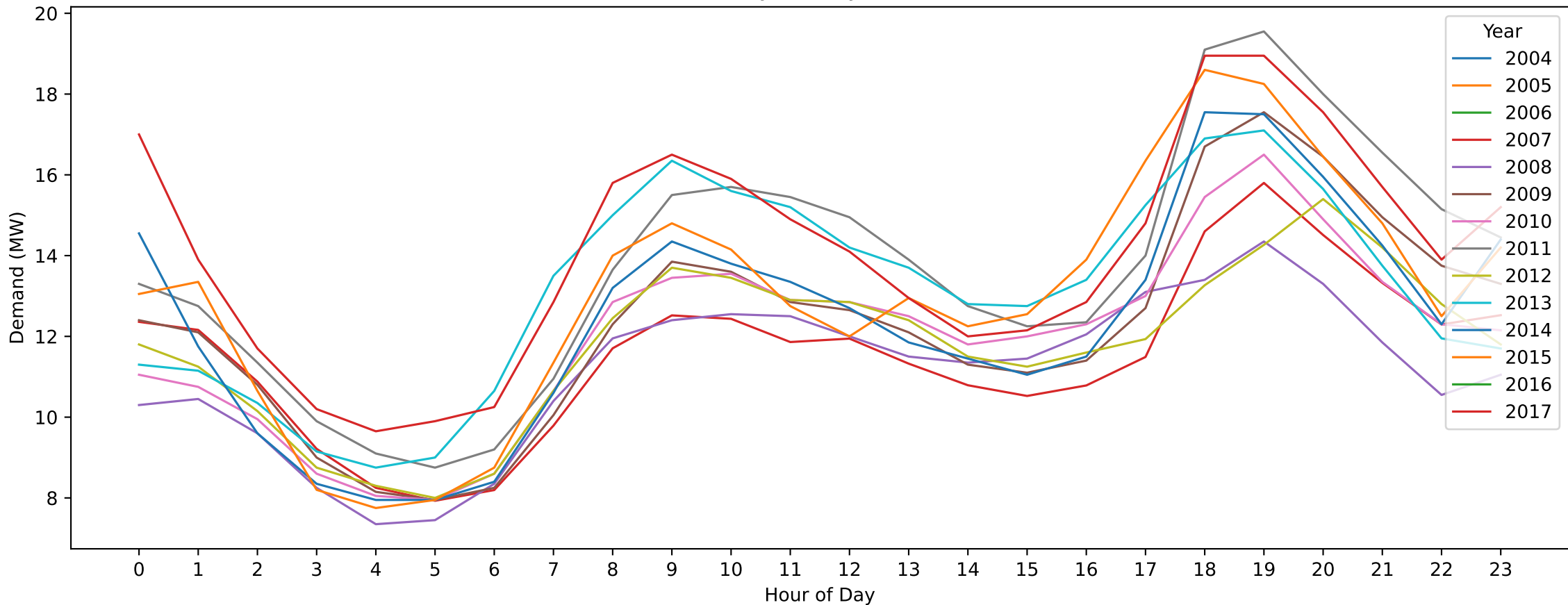
DMA — Easter Sunday (Hourly Demand Across Years)
