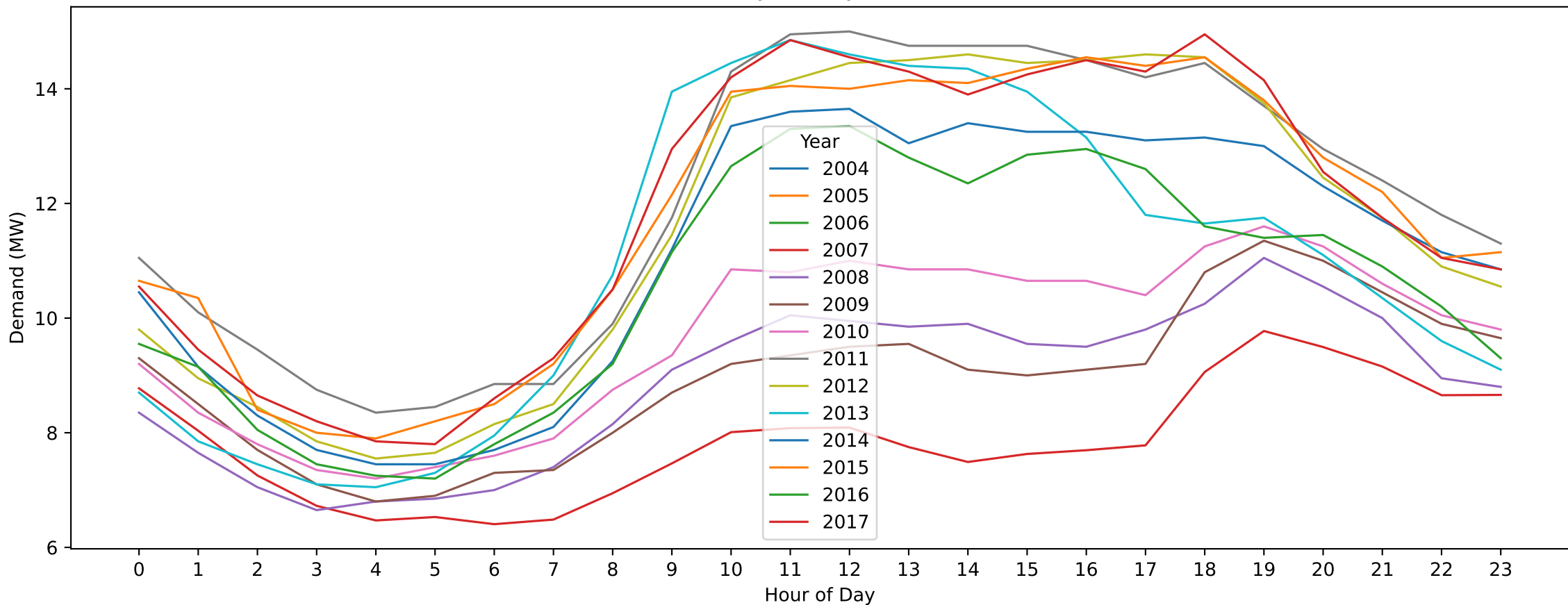
OAK — Easter Sunday (Hourly Demand Across Years)
