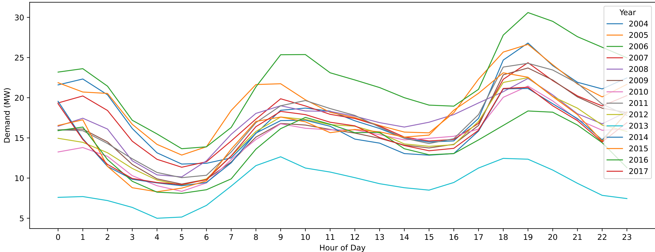
STO — Easter Sunday (Hourly Demand Across Years)
