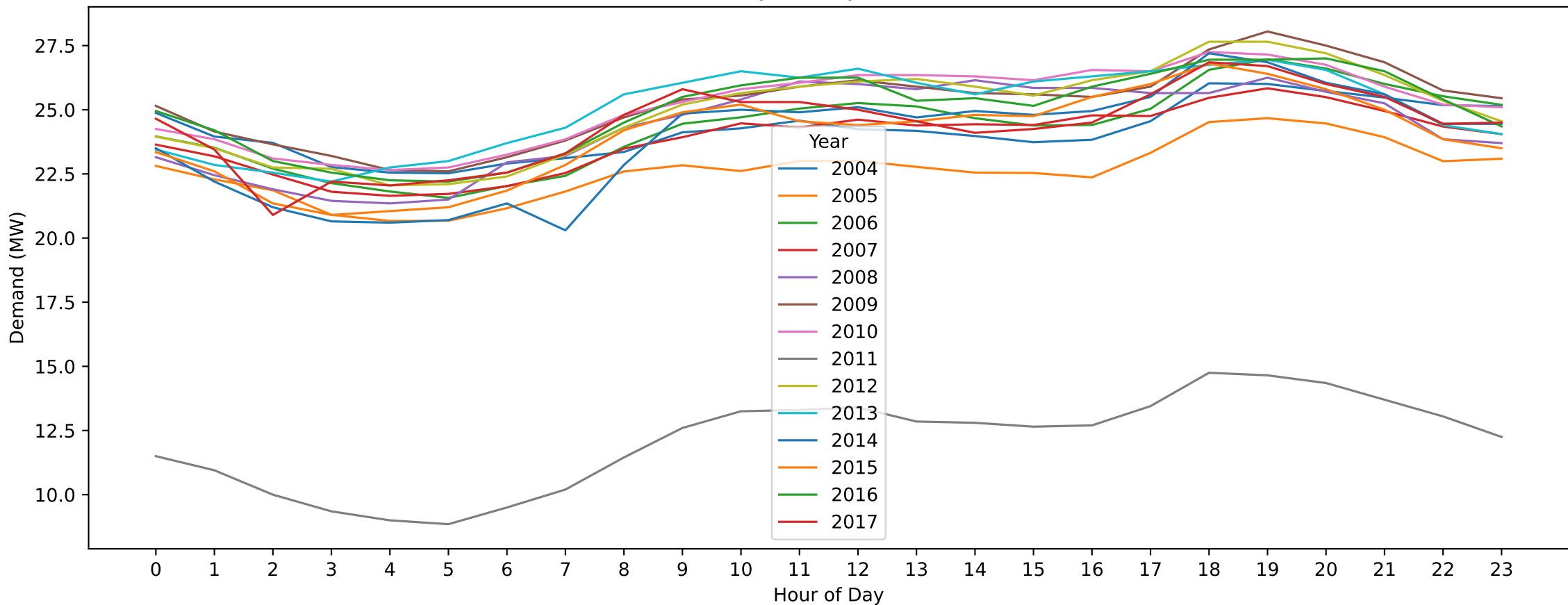
BH — Easter Sunday (Hourly Demand Across Years)
