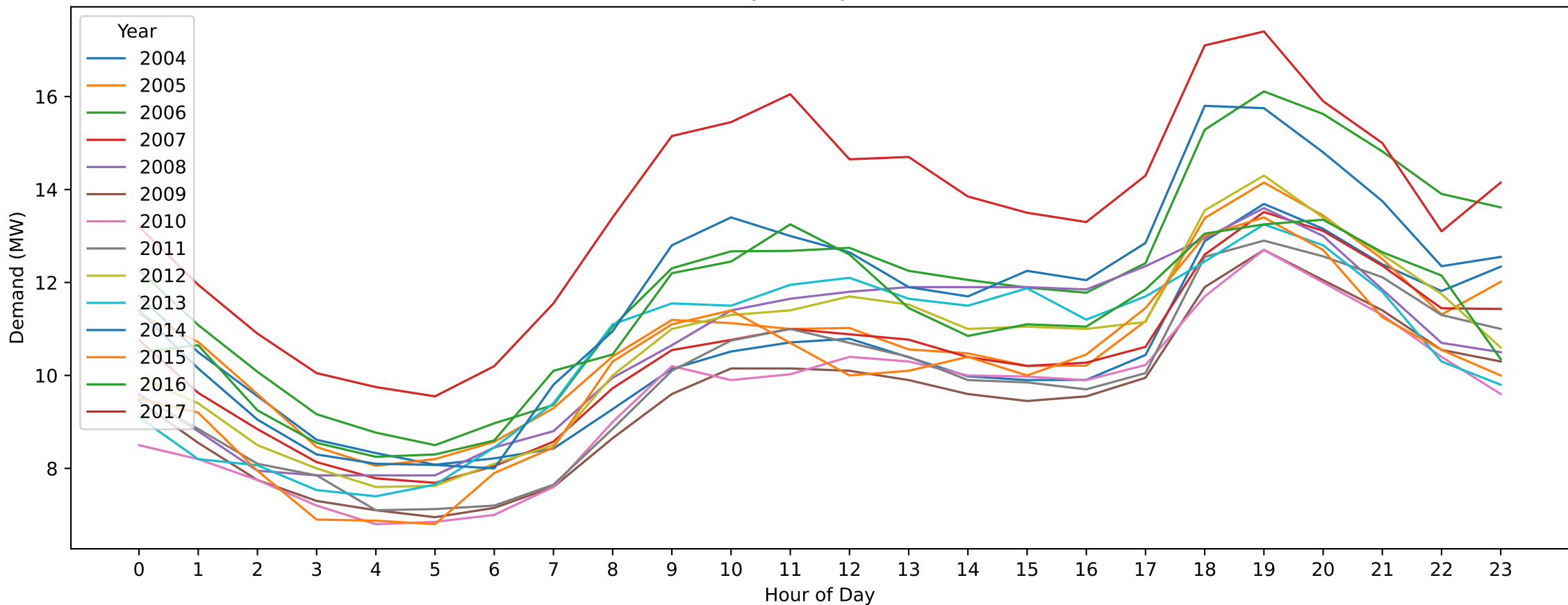
MR — Easter Sunday (Hourly Demand Across Years)
