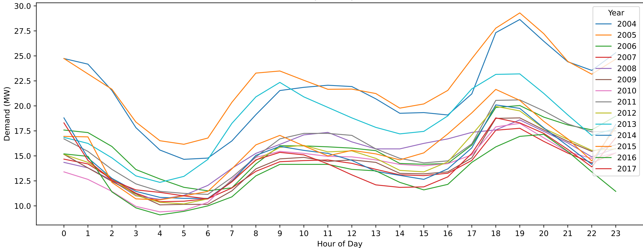
RBD — Easter Sunday (Hourly Demand Across Years)
