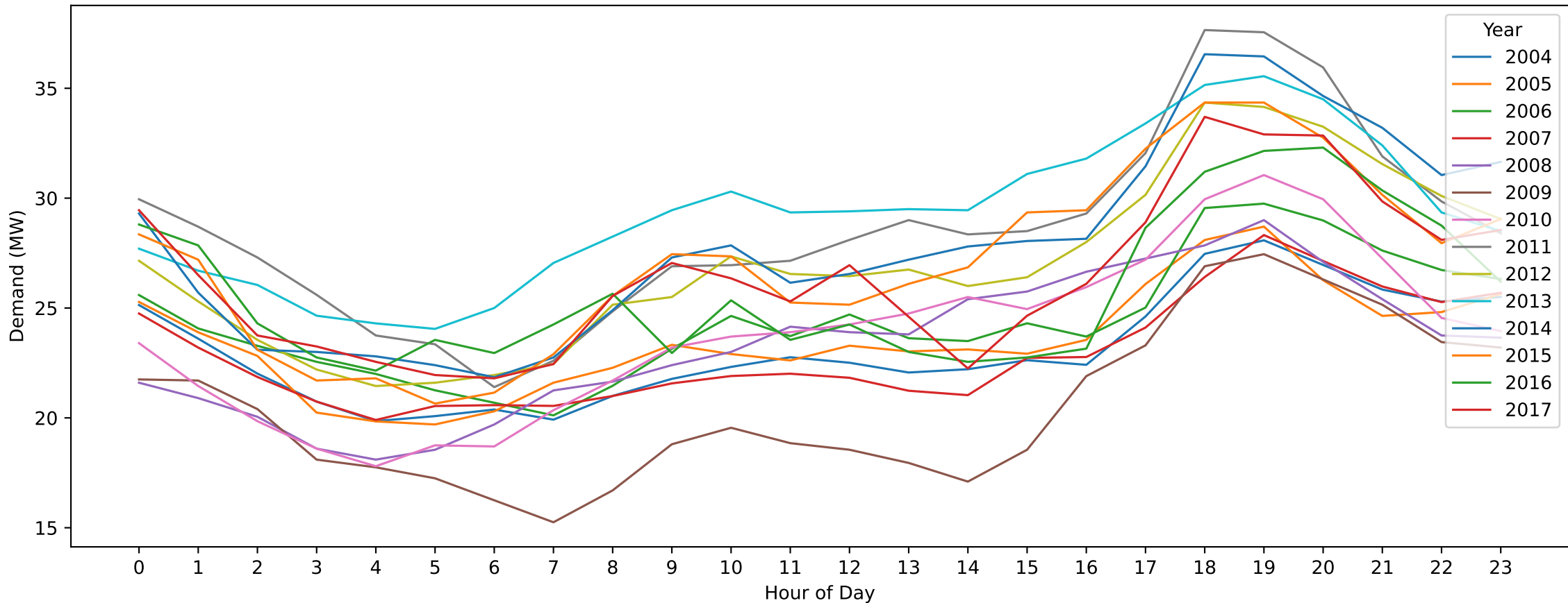
CRM — Easter Sunday (Hourly Demand Across Years)
