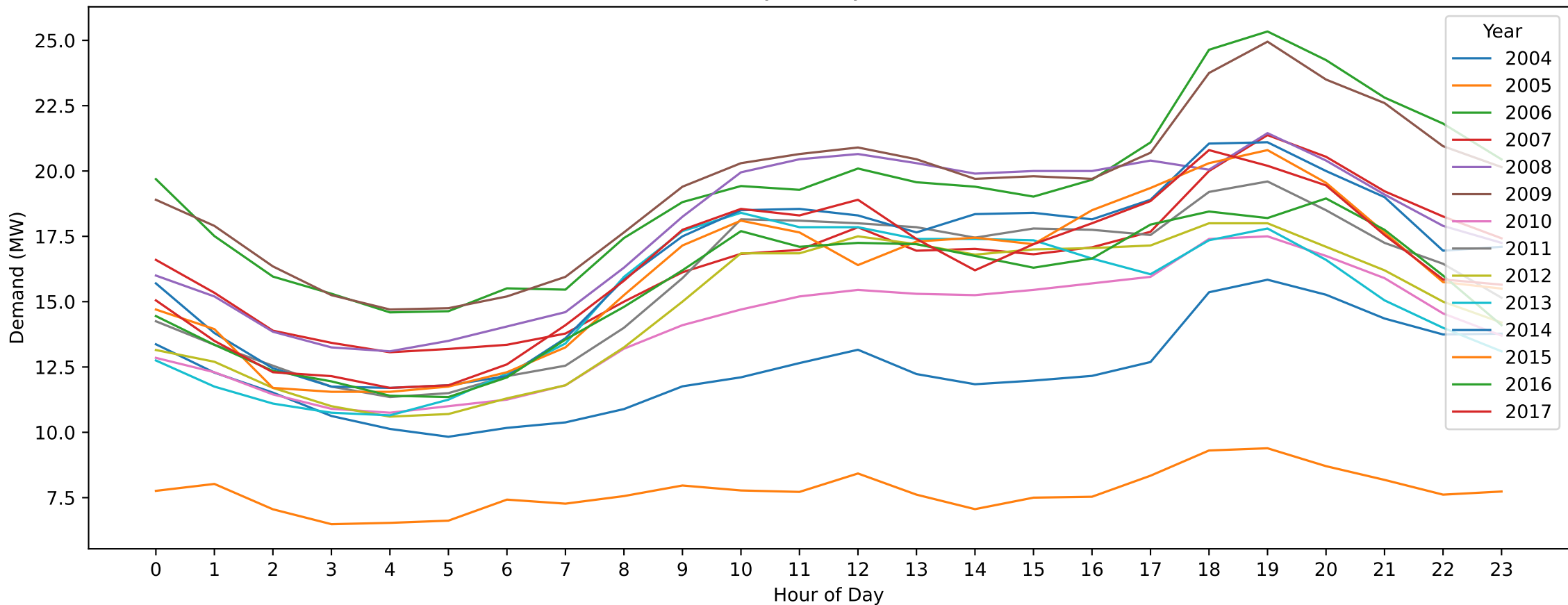
FTN — Easter Sunday (Hourly Demand Across Years)
