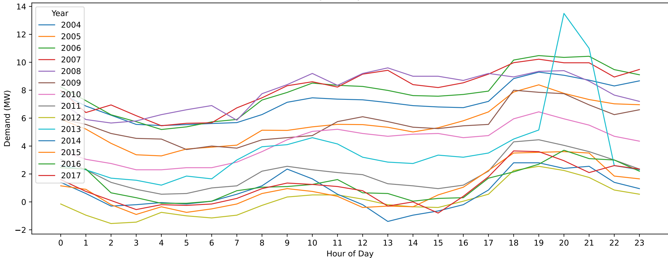
SS — Easter Sunday (Hourly Demand Across Years)
