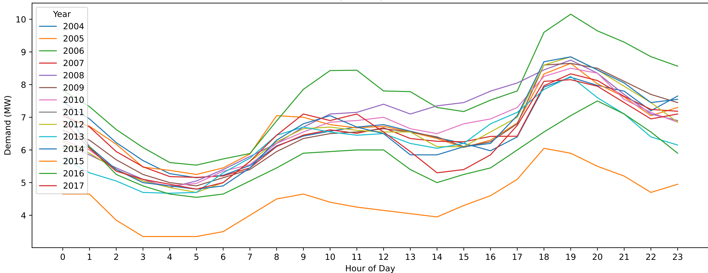
BW — Easter Sunday (Hourly Demand Across Years)
