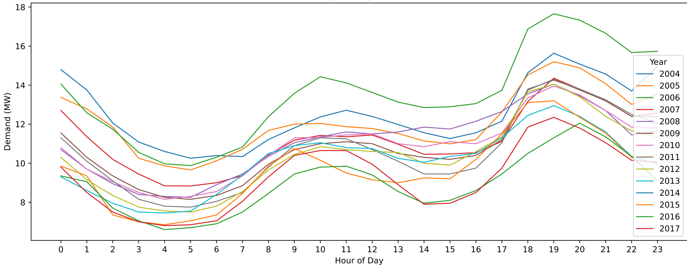
OR — Easter Sunday (Hourly Demand Across Years)
