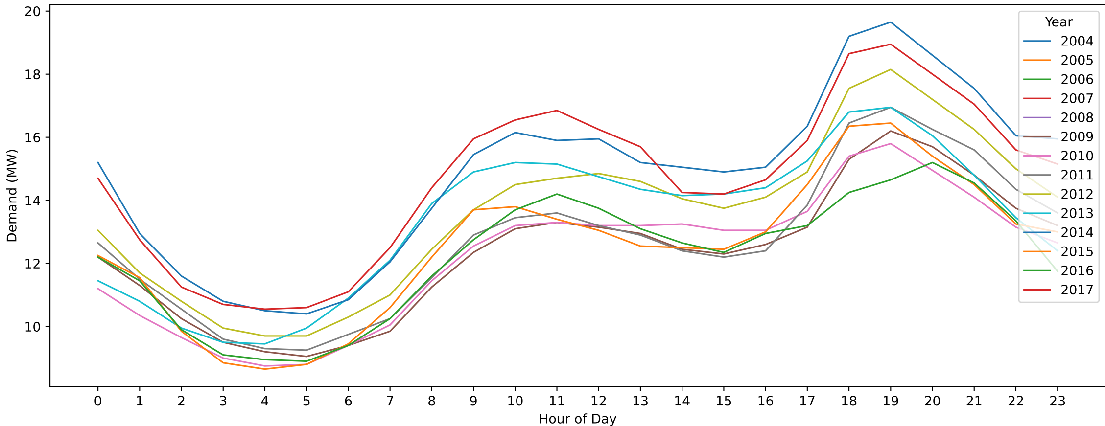
CFD — Easter Sunday (Hourly Demand Across Years)
