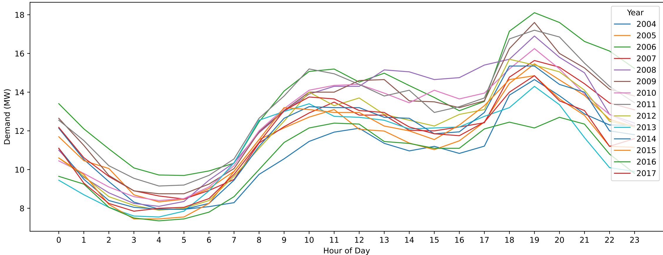
NB — Easter Sunday (Hourly Demand Across Years)
