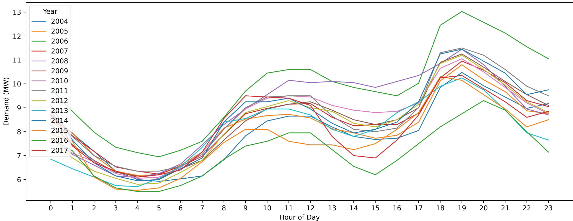
BU — Easter Sunday (Hourly Demand Across Years)
