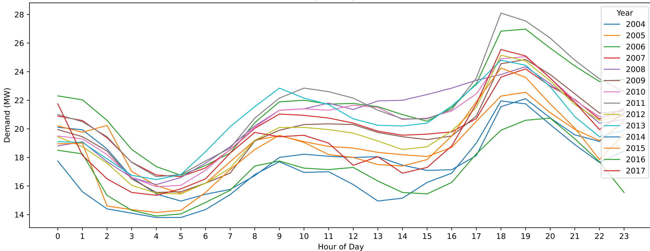
HGS — Easter Sunday (Hourly Demand Across Years)
