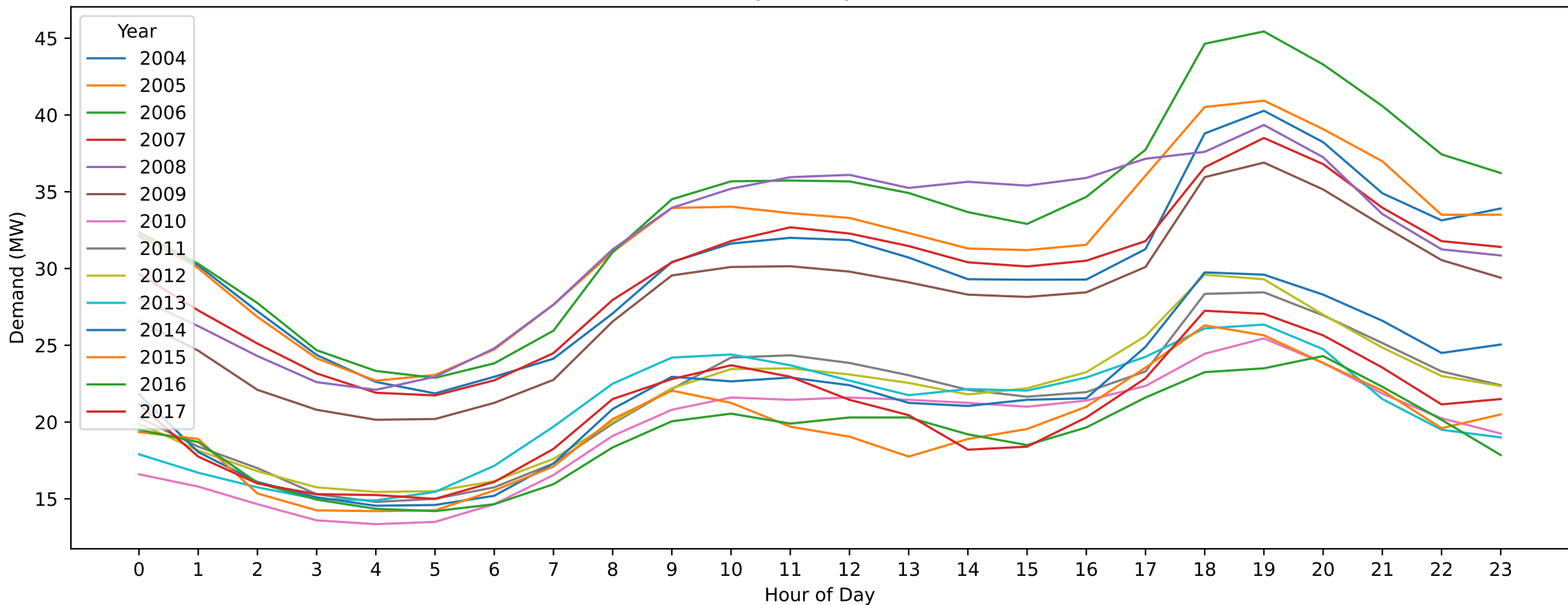
FSH — Easter Sunday (Hourly Demand Across Years)
