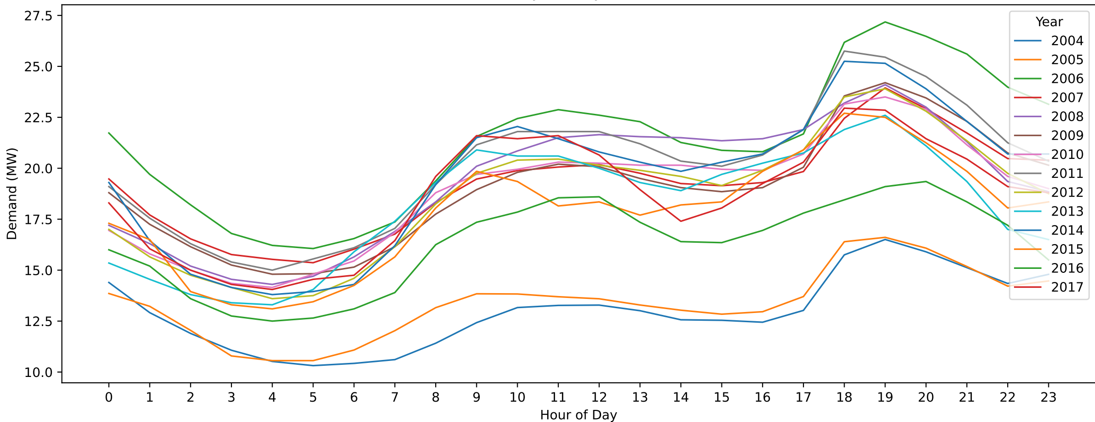
NW — Easter Sunday (Hourly Demand Across Years)
