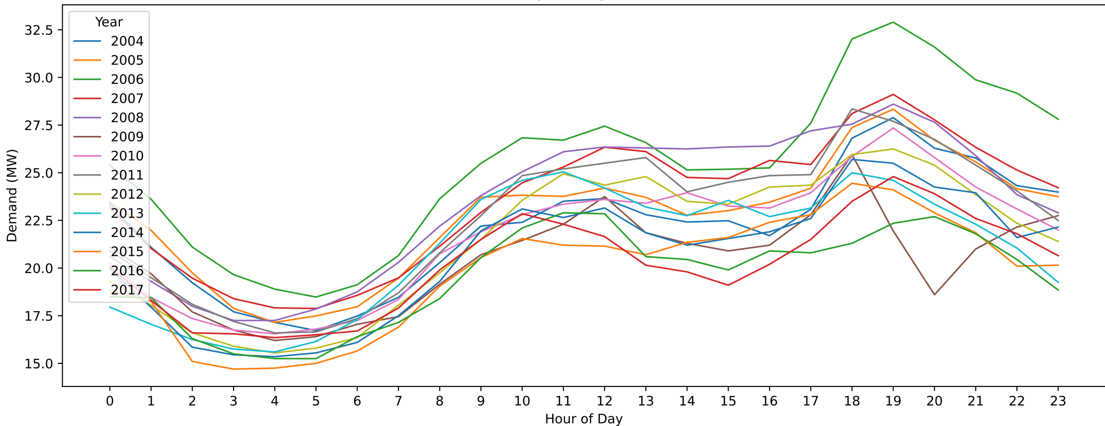
GW — Easter Sunday (Hourly Demand Across Years)
