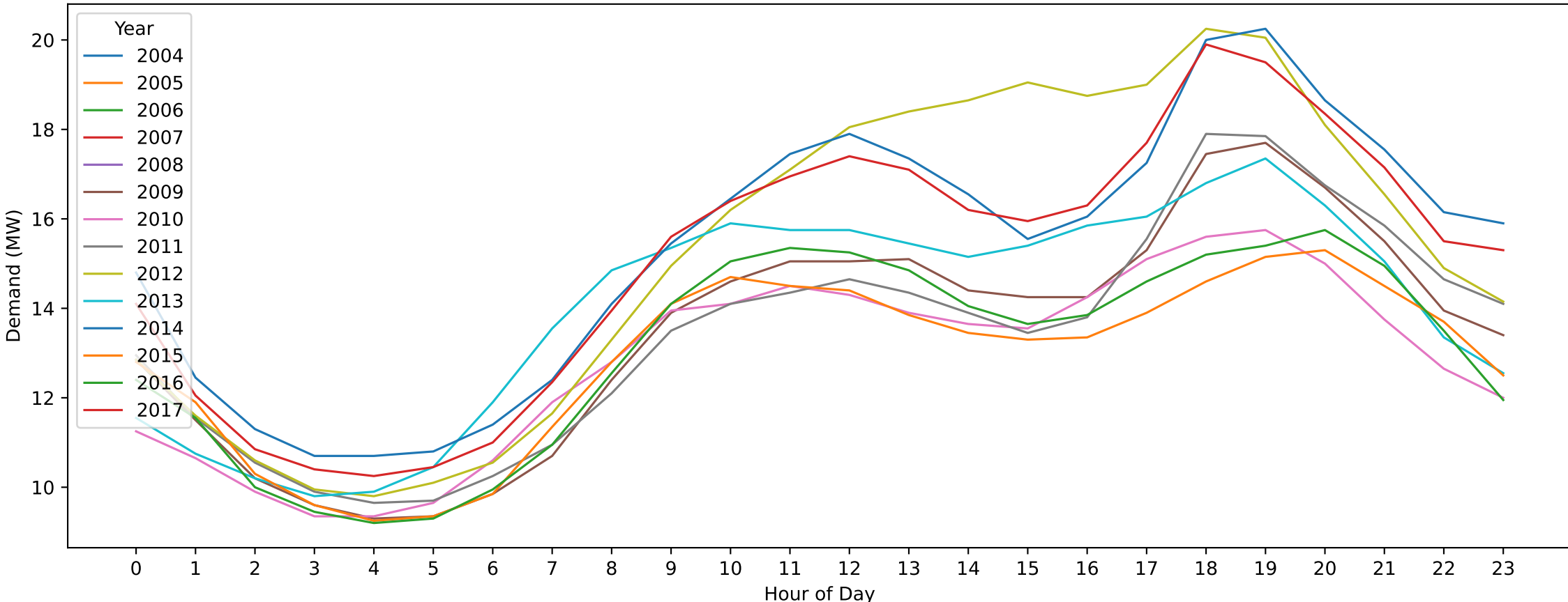
CFD — Good Friday (Hourly Demand Across Years)
