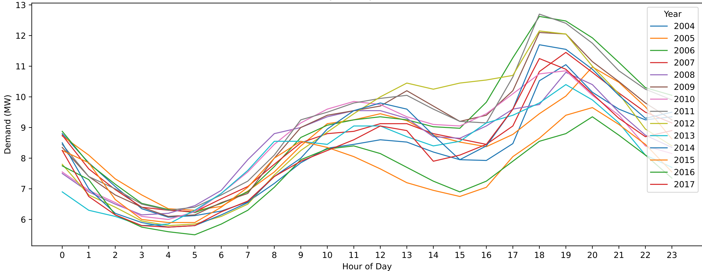
BU — Good Friday (Hourly Demand Across Years)
