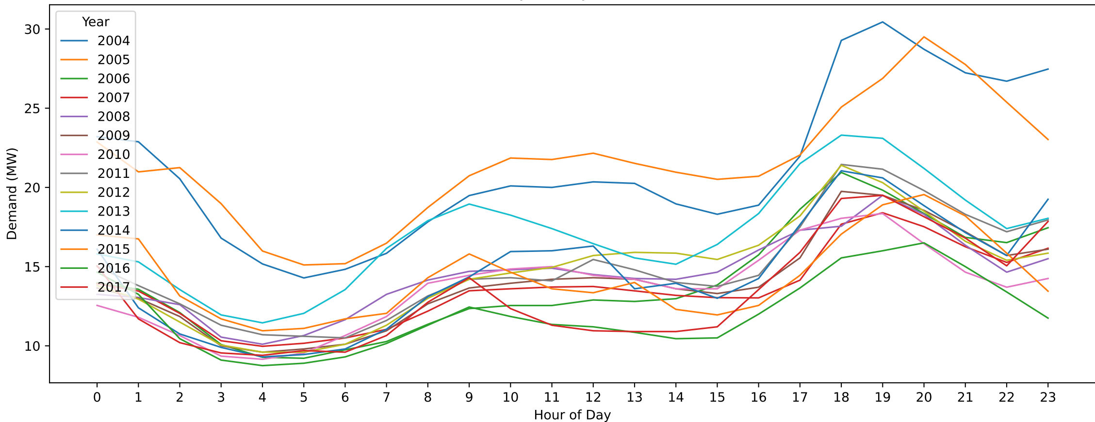
RBD — Good Friday (Hourly Demand Across Years)
