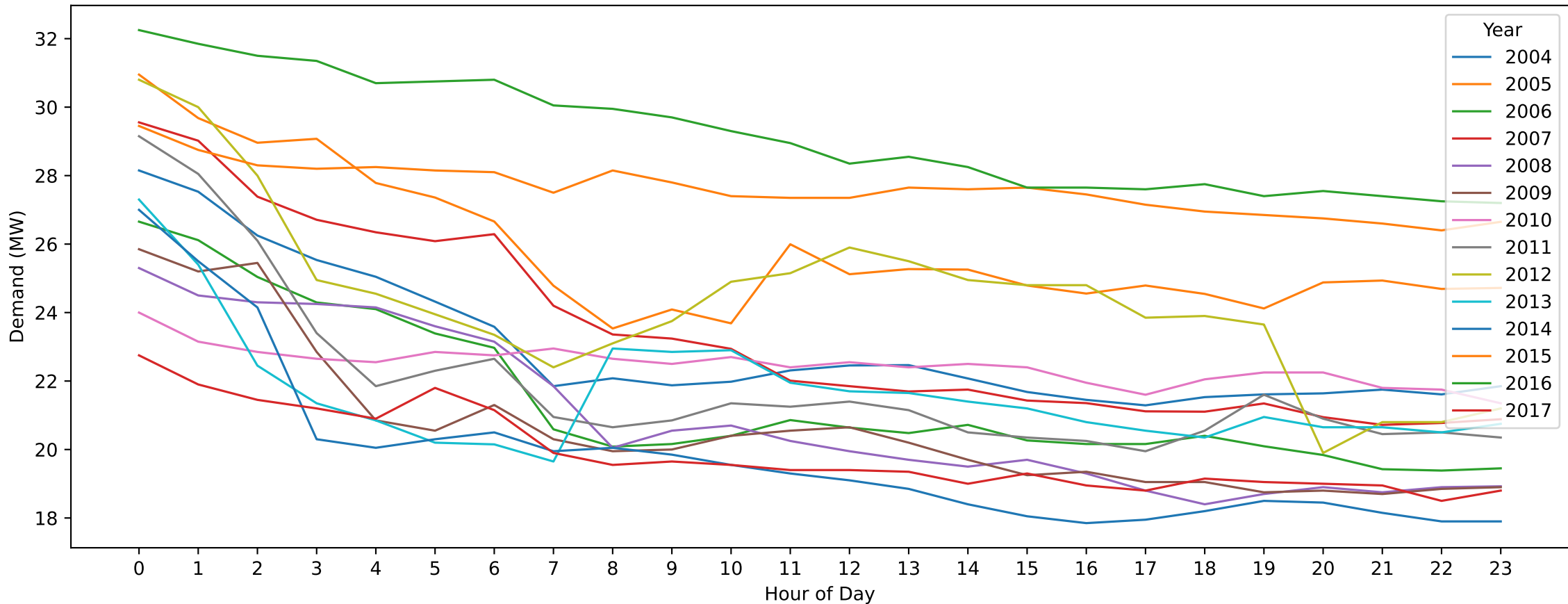
DSH — Good Friday (Hourly Demand Across Years)
