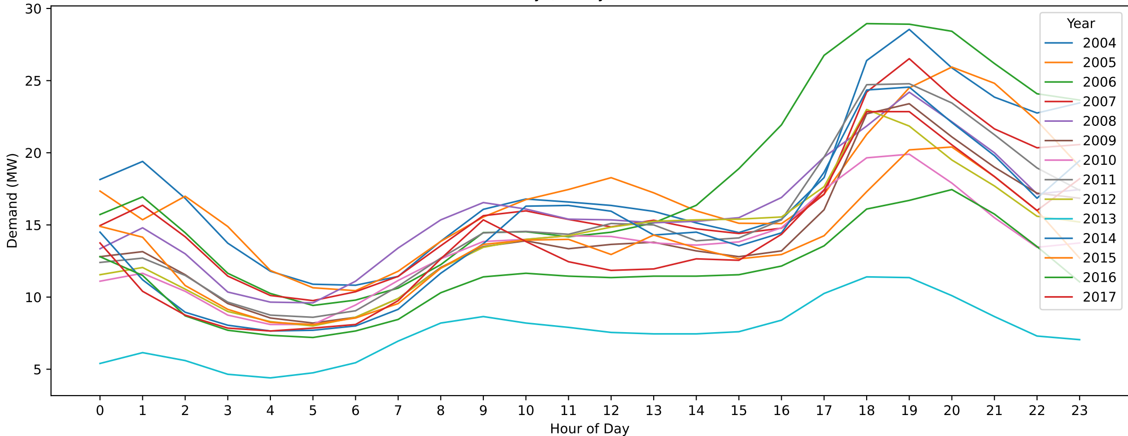
STO — Good Friday (Hourly Demand Across Years)
