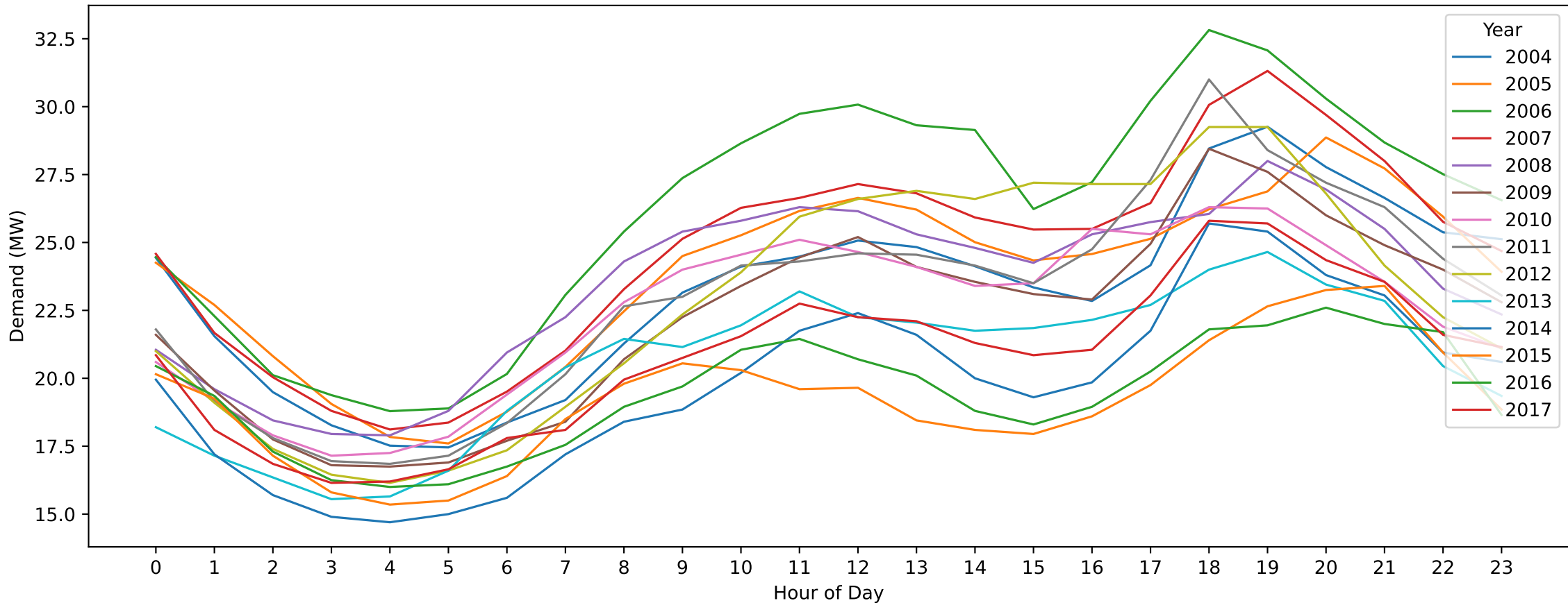
GW — Good Friday (Hourly Demand Across Years)
