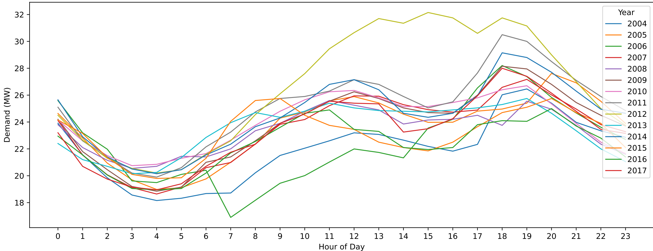
MGE — Good Friday (Hourly Demand Across Years)
