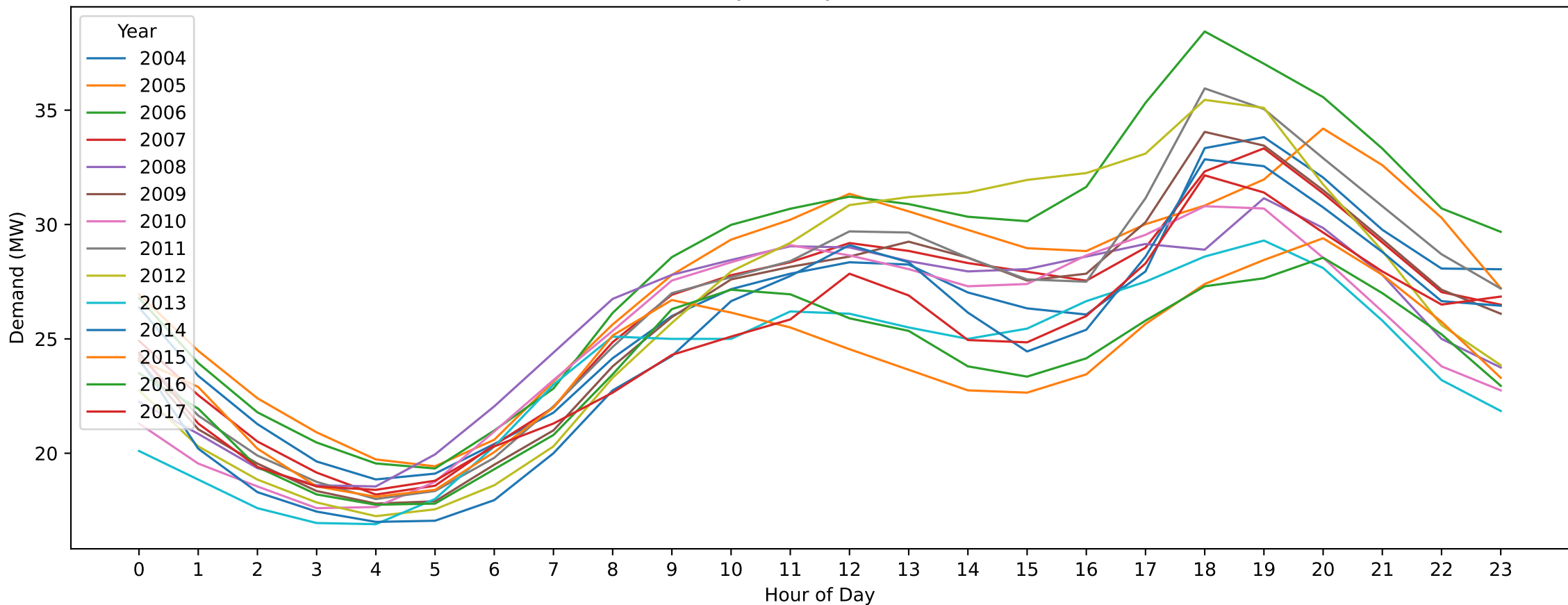
DC — Good Friday (Hourly Demand Across Years)
