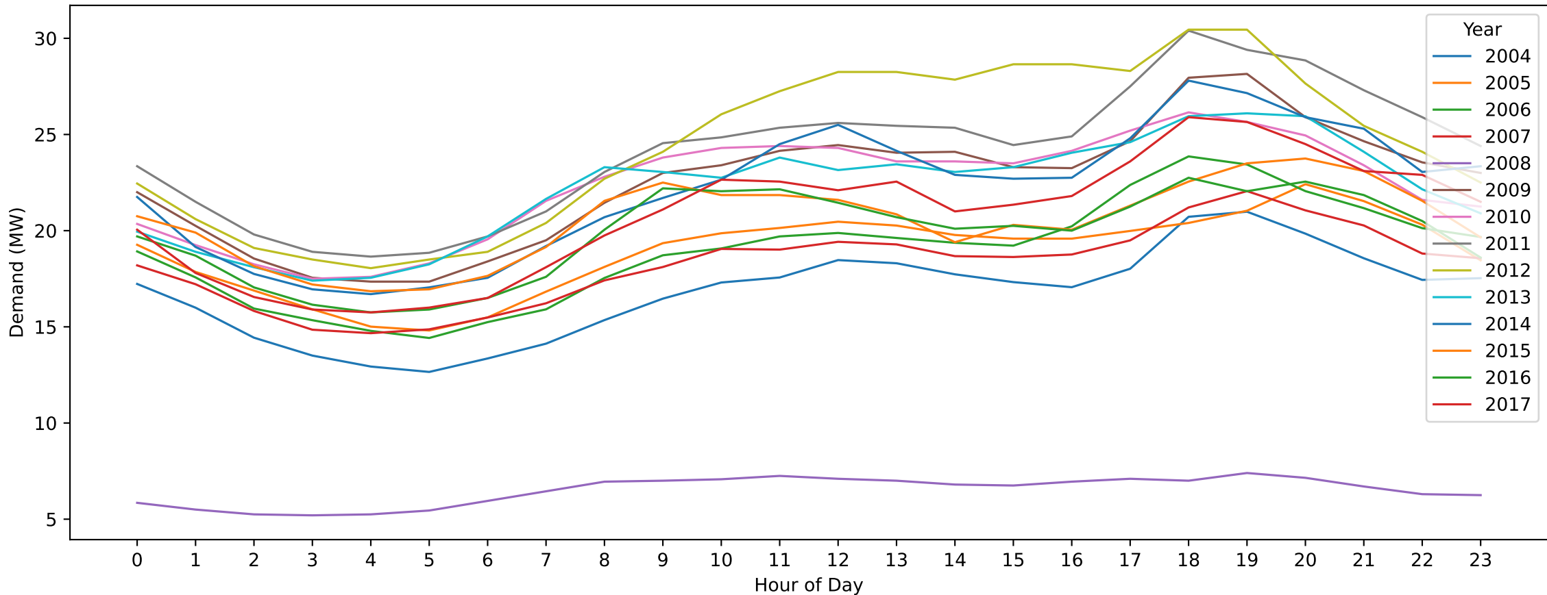
EB — Good Friday (Hourly Demand Across Years)
