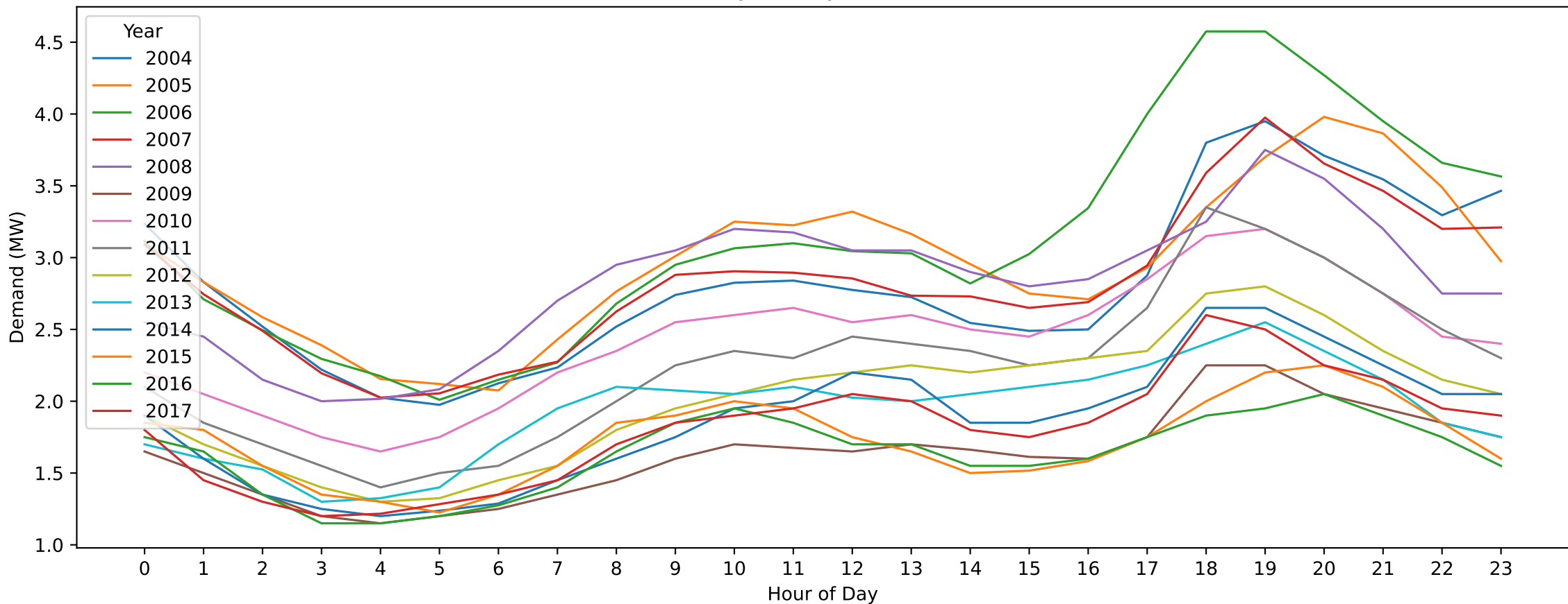
SH — Good Friday (Hourly Demand Across Years)
