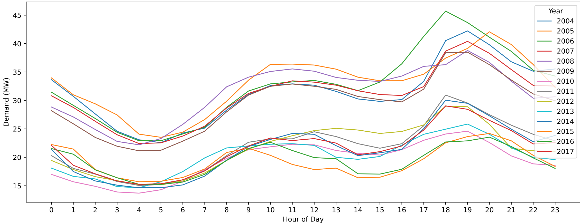
FSH — Good Friday (Hourly Demand Across Years)
