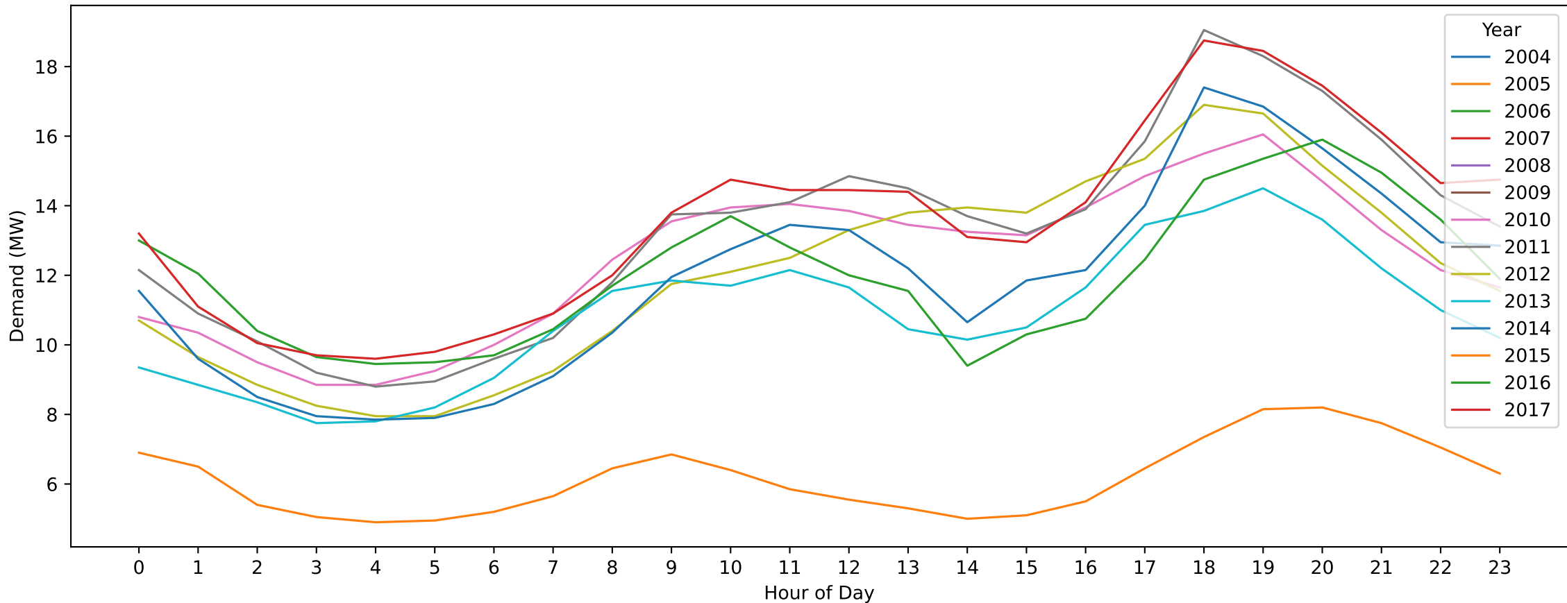
LWN — Good Friday (Hourly Demand Across Years)
