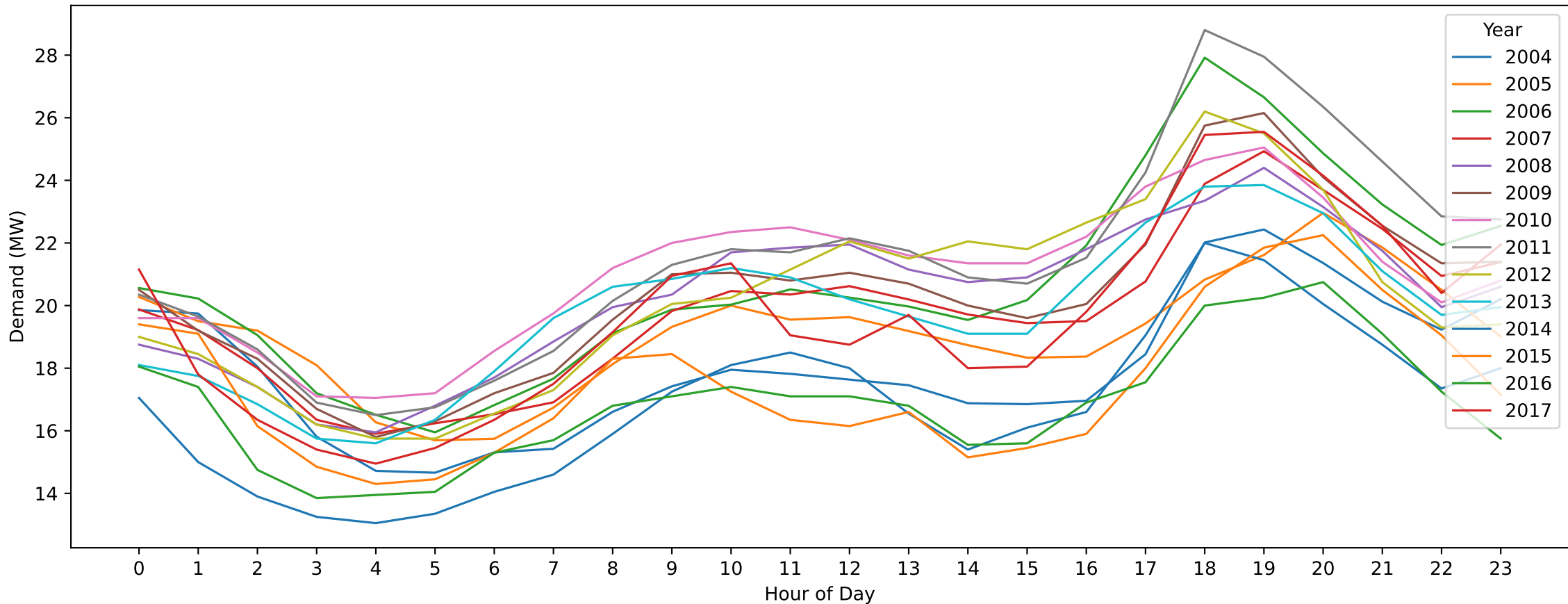
HGS — Good Friday (Hourly Demand Across Years)
