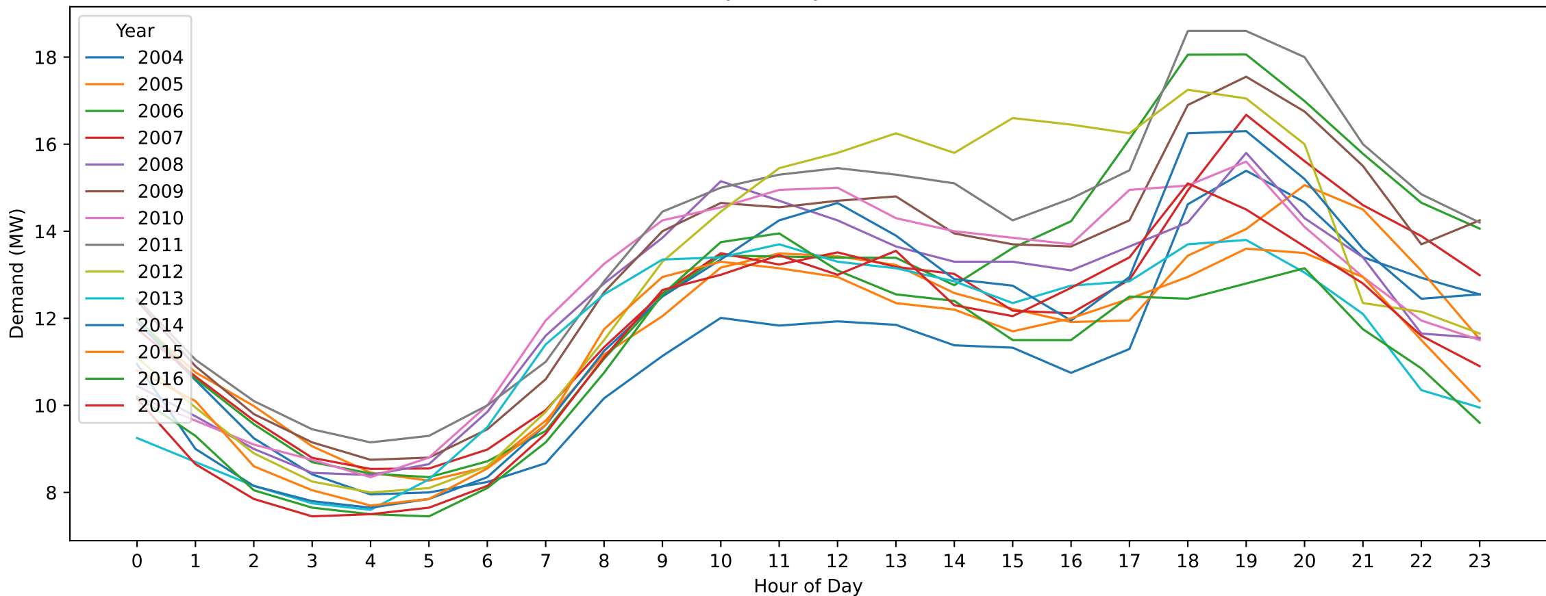
NB — Good Friday (Hourly Demand Across Years)
