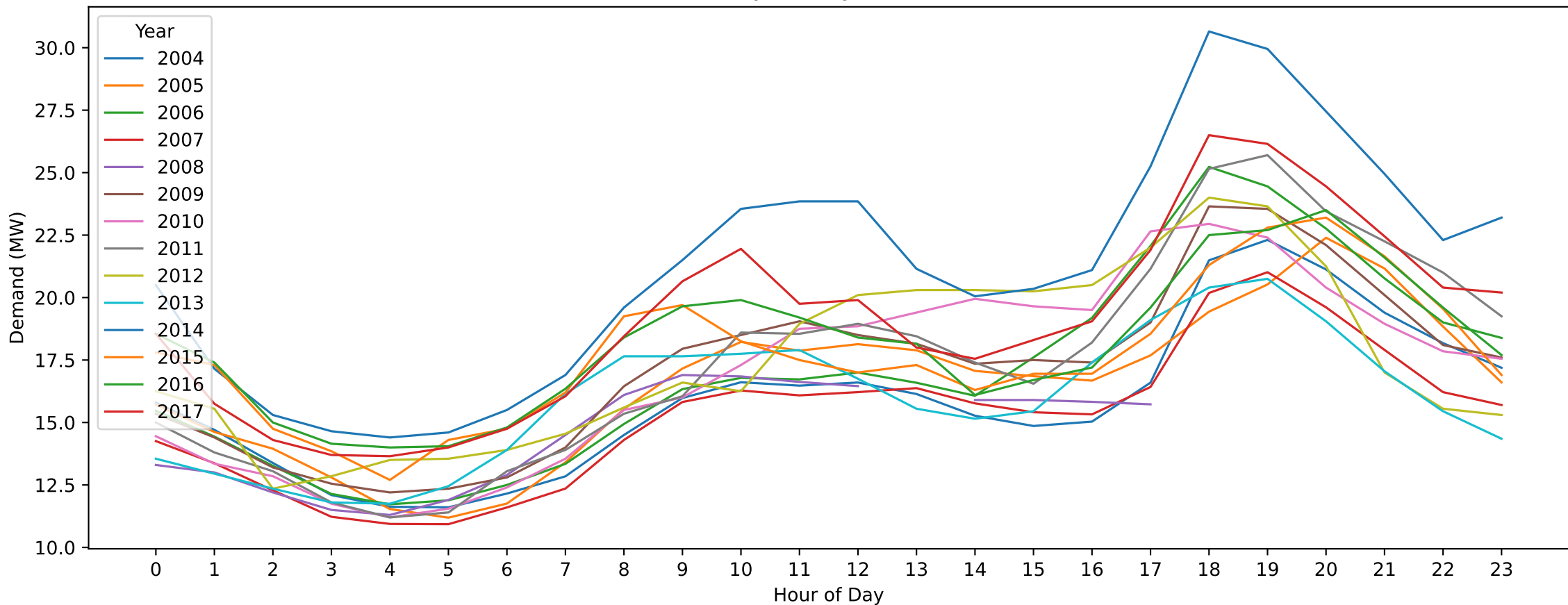
MTN — Good Friday (Hourly Demand Across Years)
