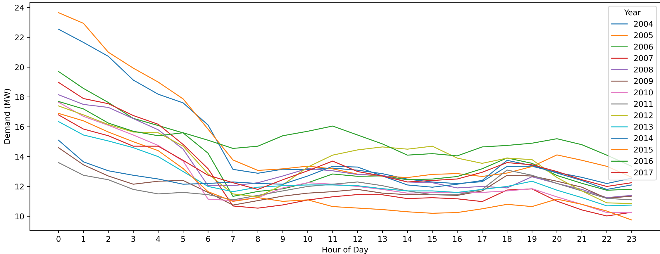
HT — Good Friday (Hourly Demand Across Years)
