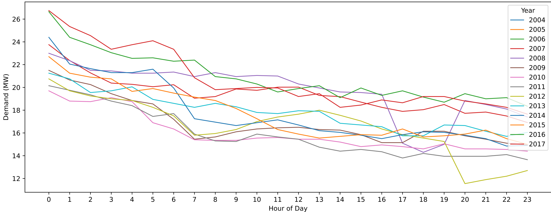
DVY — Good Friday (Hourly Demand Across Years)
