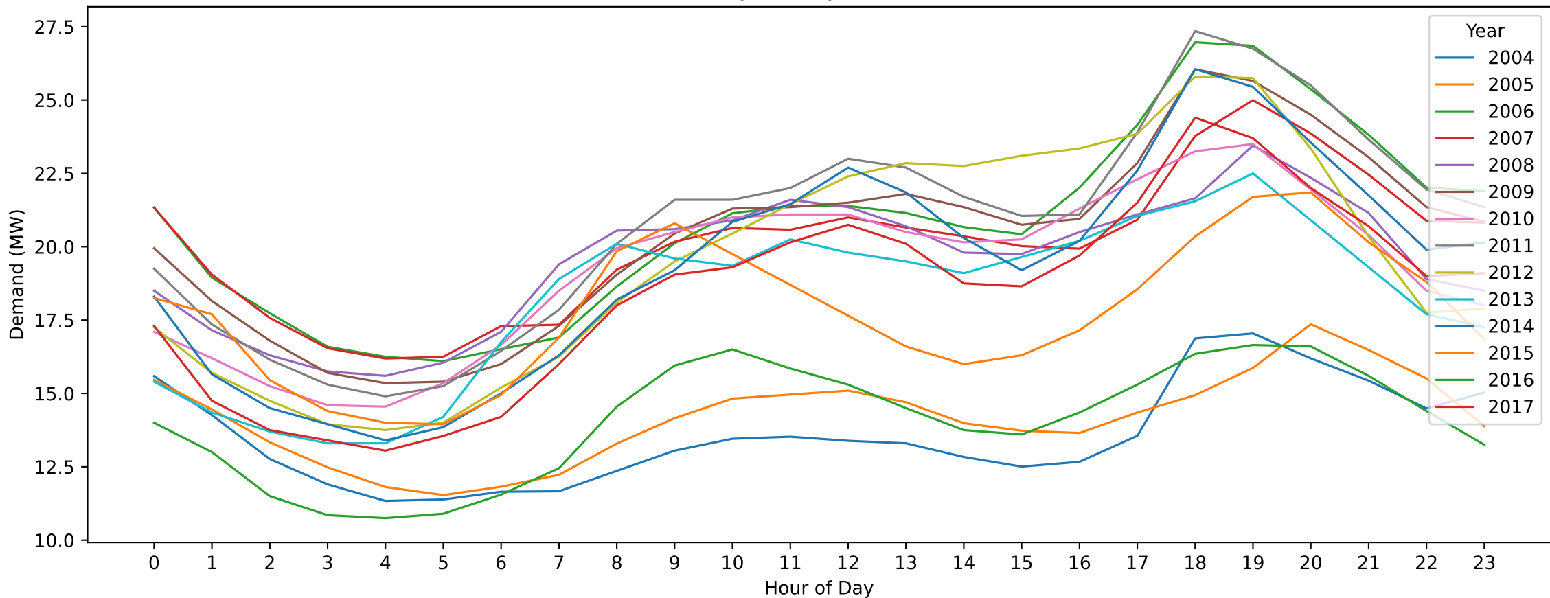
NW — Good Friday (Hourly Demand Across Years)
