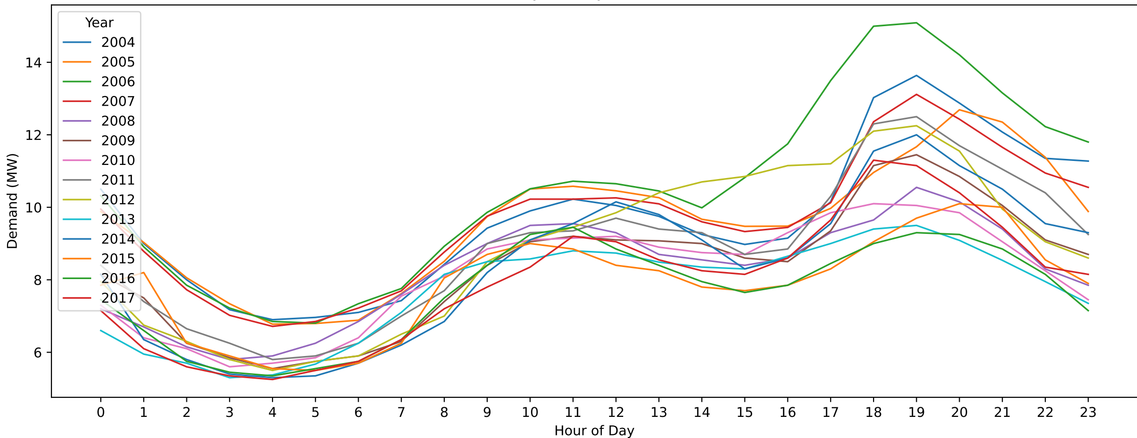
BT — Good Friday (Hourly Demand Across Years)
