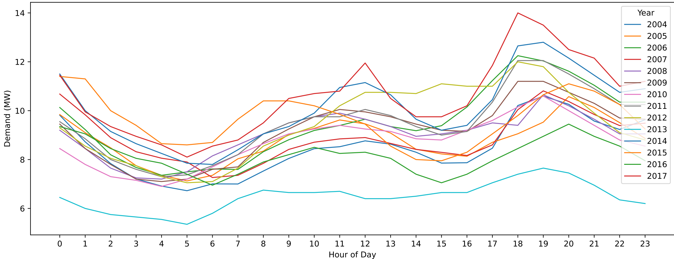
CDA — Good Friday (Hourly Demand Across Years)
