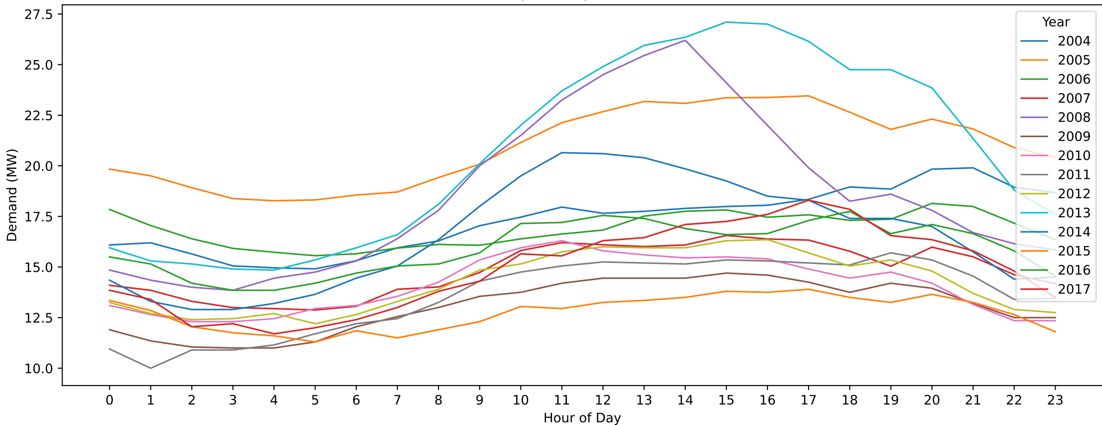
HT — Labour Day (Hourly Demand Across Years)
