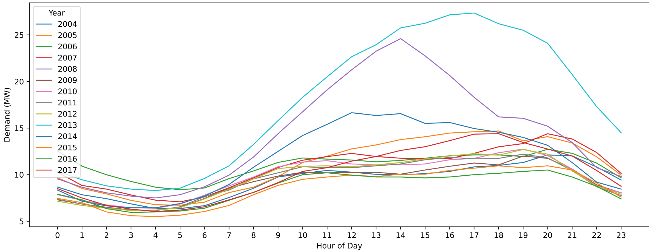
EL — Labour Day (Hourly Demand Across Years)
