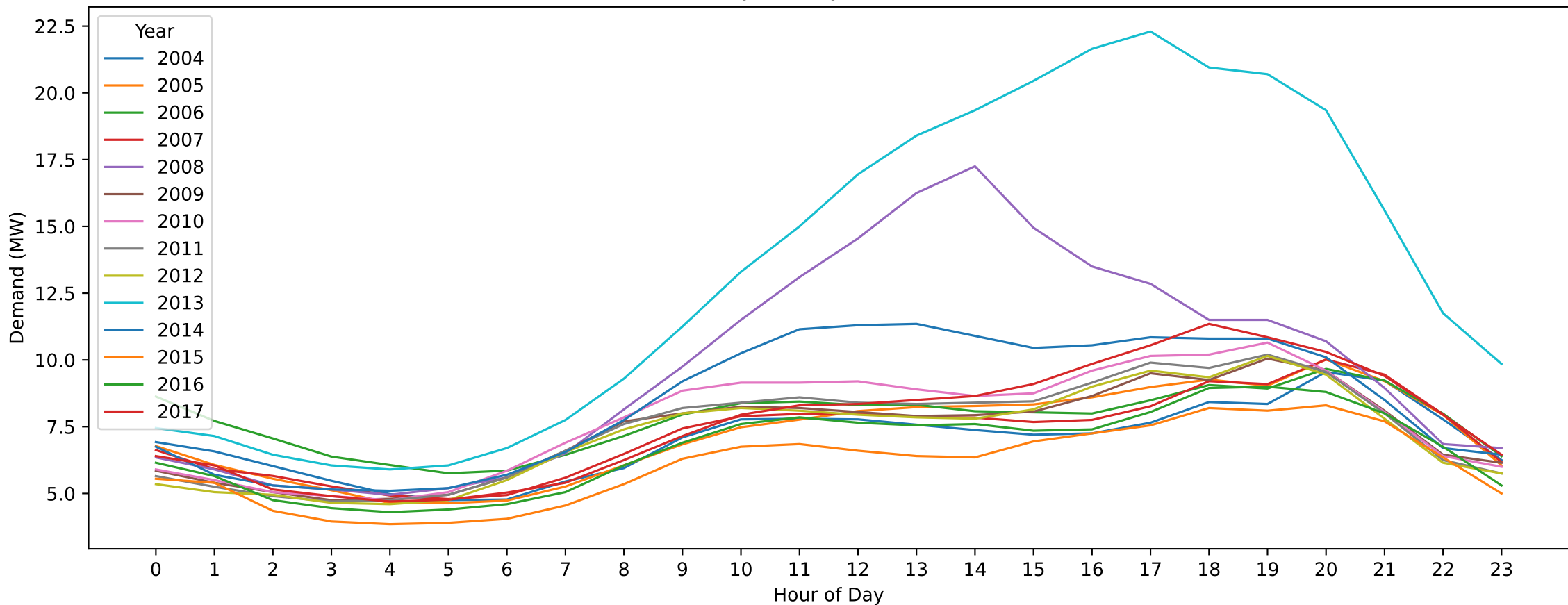
BR — Labour Day (Hourly Demand Across Years)
