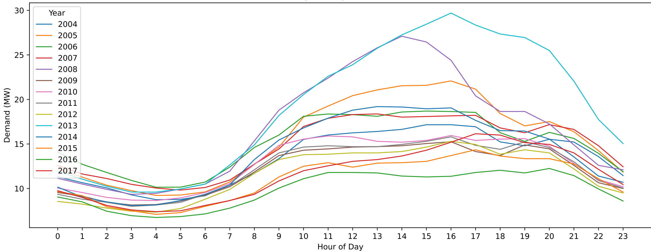
EM — Labour Day (Hourly Demand Across Years)
