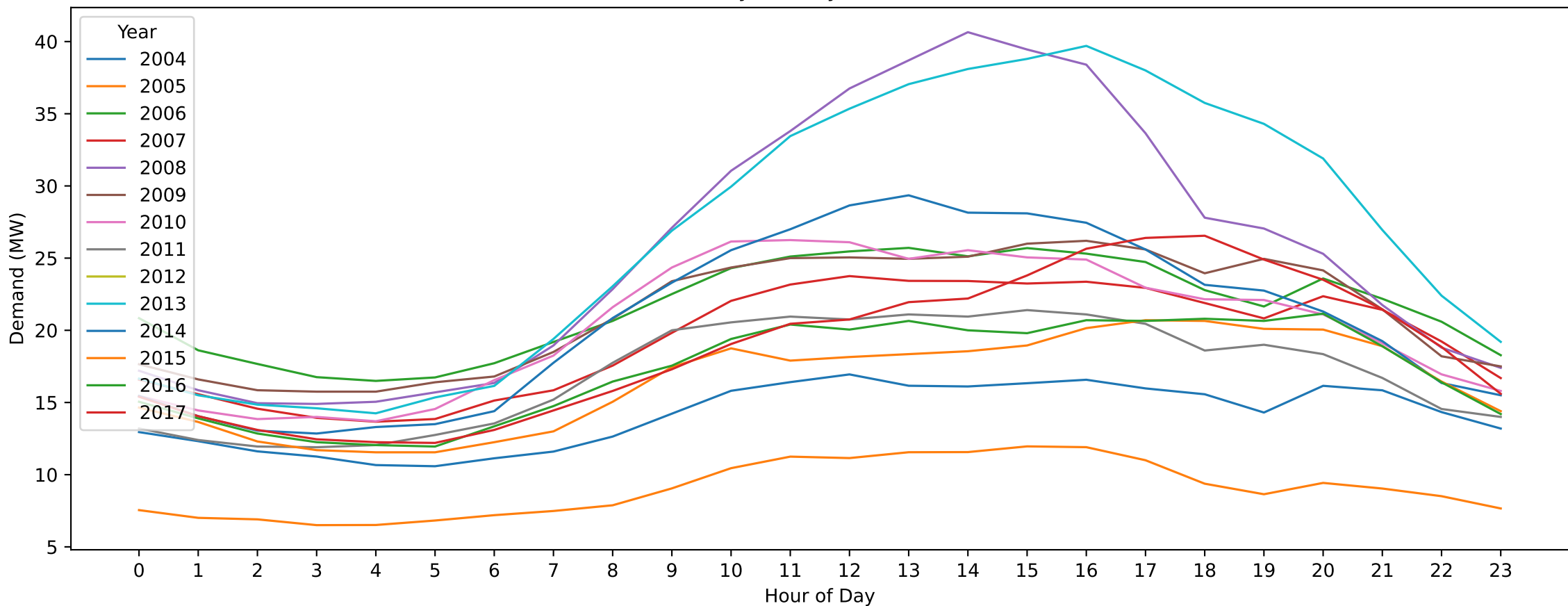
FTN — Labour Day (Hourly Demand Across Years)
