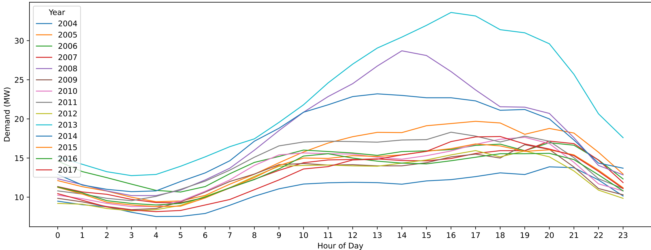
K — Labour Day (Hourly Demand Across Years)
