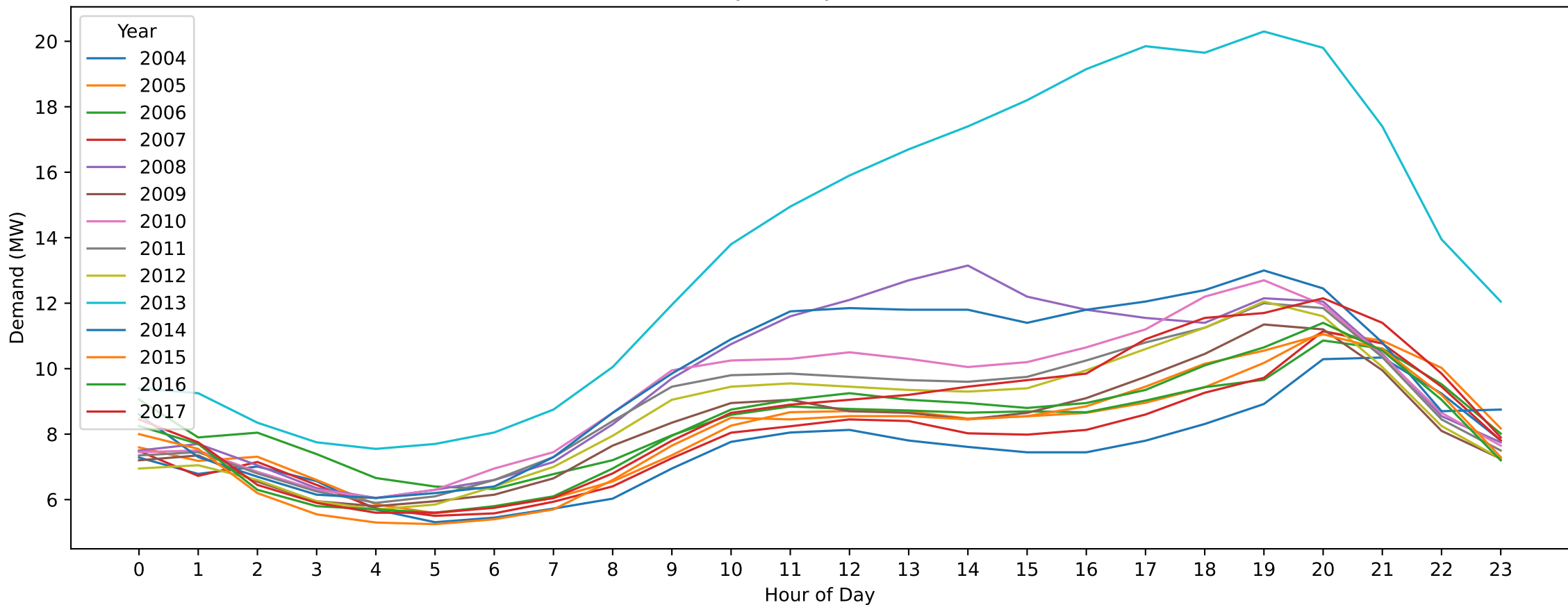
EW — Labour Day (Hourly Demand Across Years)
