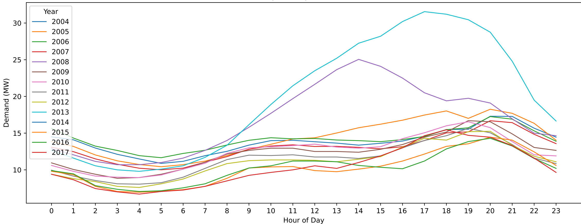
OR — Labour Day (Hourly Demand Across Years)
