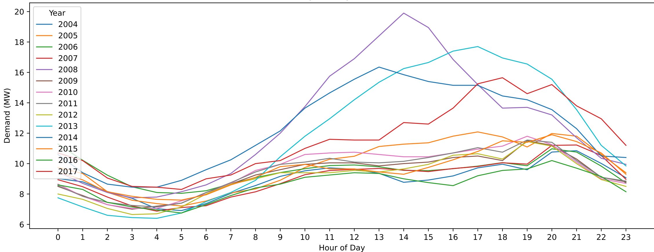
CDA — Labour Day (Hourly Demand Across Years)
