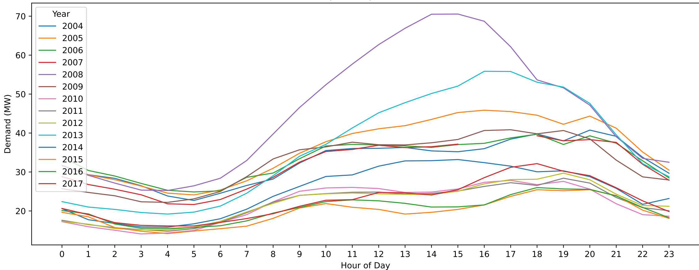
FSH — Labour Day (Hourly Demand Across Years)
