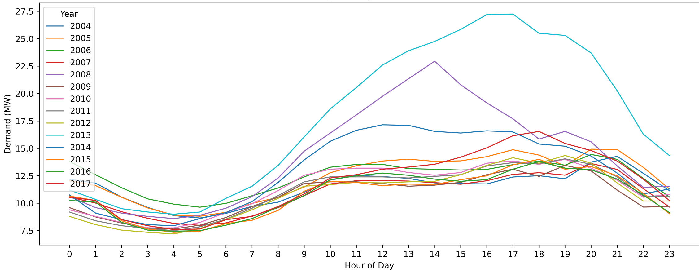
M — Labour Day (Hourly Demand Across Years)
