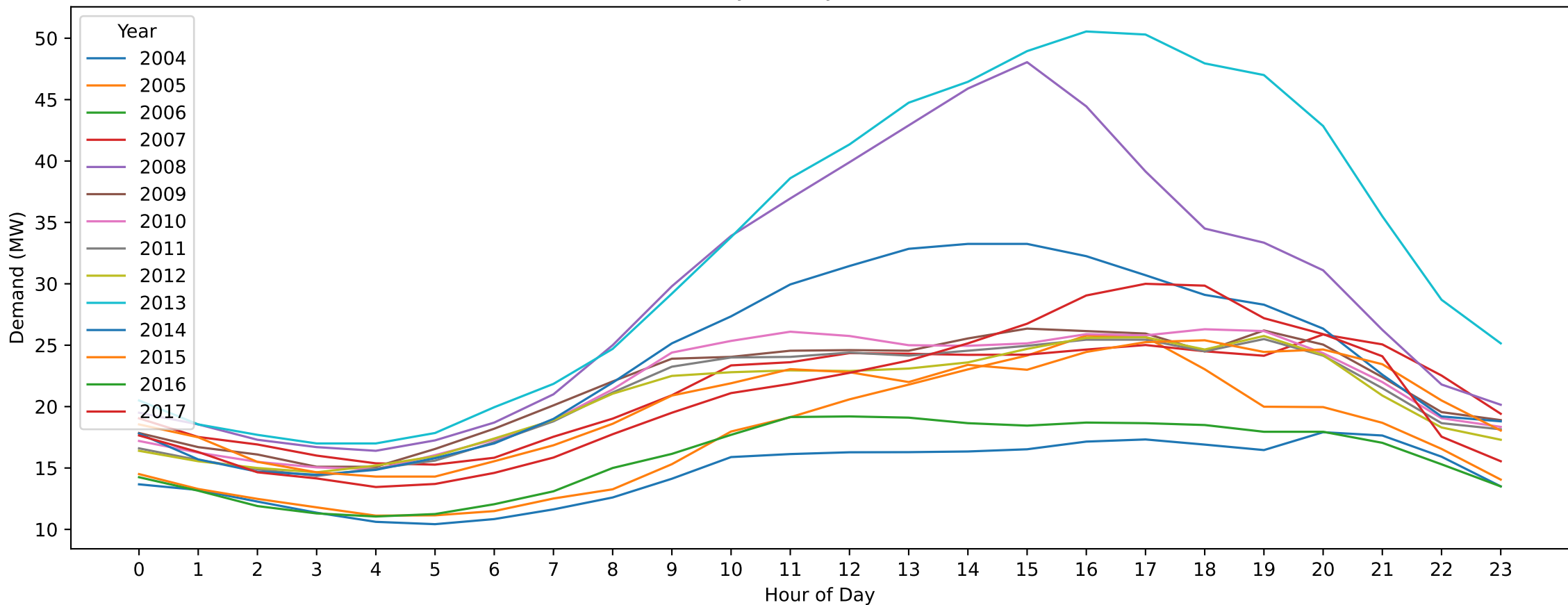
NW — Labour Day (Hourly Demand Across Years)
