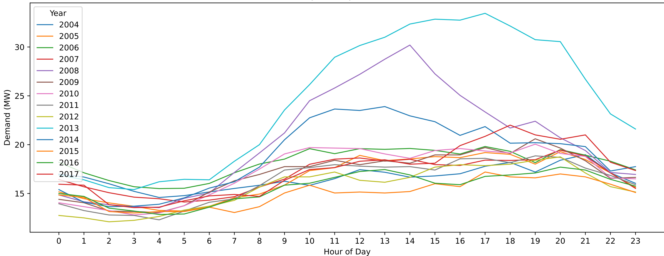
MC — Labour Day (Hourly Demand Across Years)
