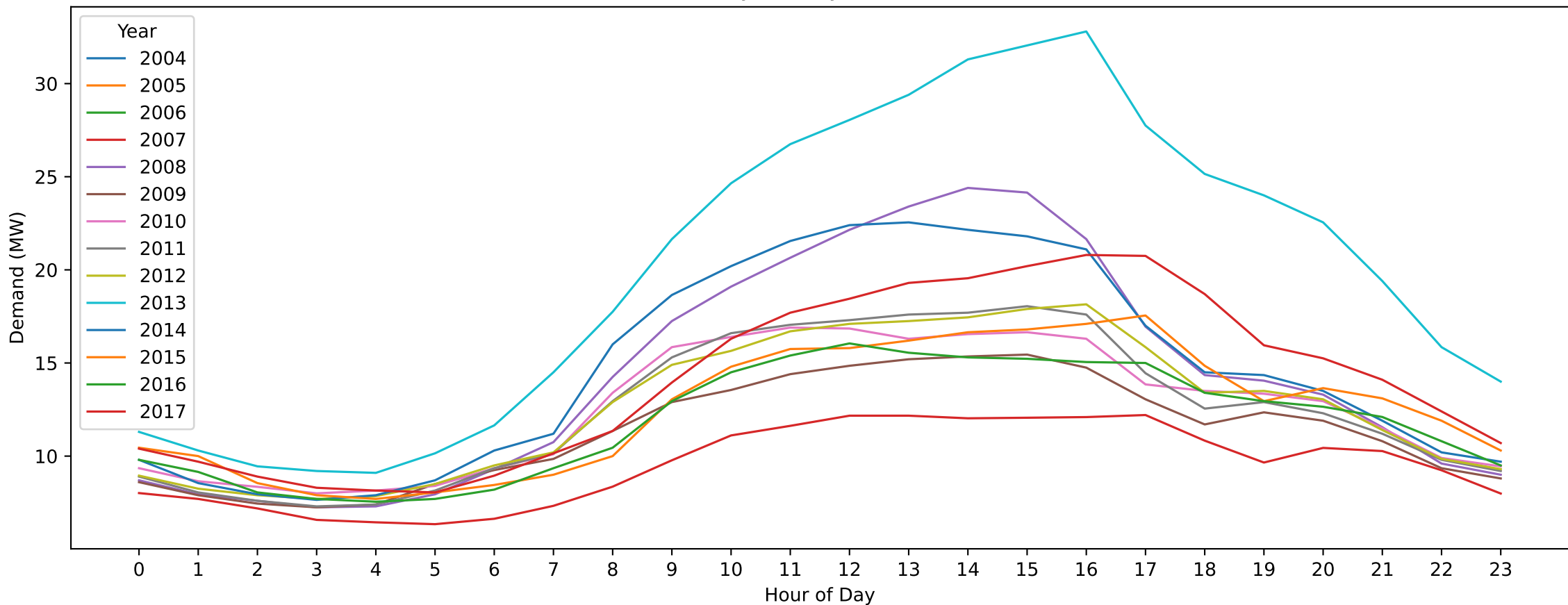
OAK — Labour Day (Hourly Demand Across Years)
