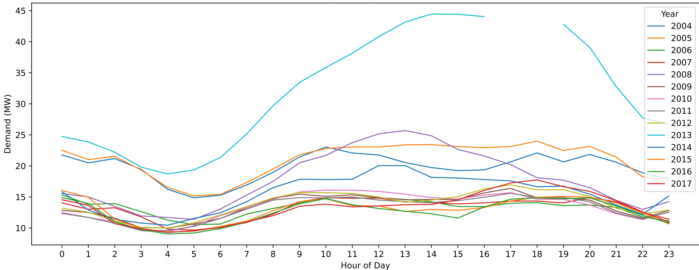
RBD — Labour Day (Hourly Demand Across Years)
