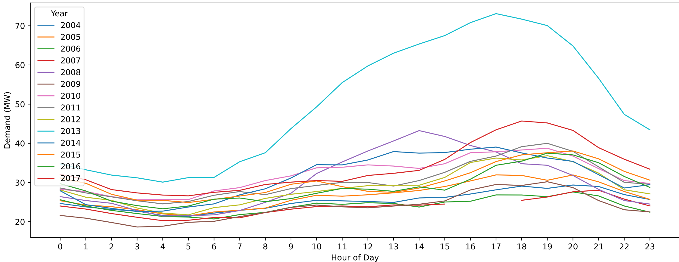
CRM — Labour Day (Hourly Demand Across Years)
