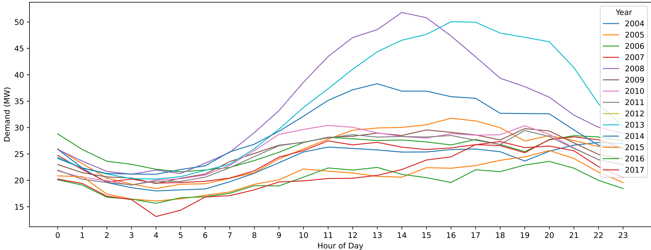
NP — Labour Day (Hourly Demand Across Years)
