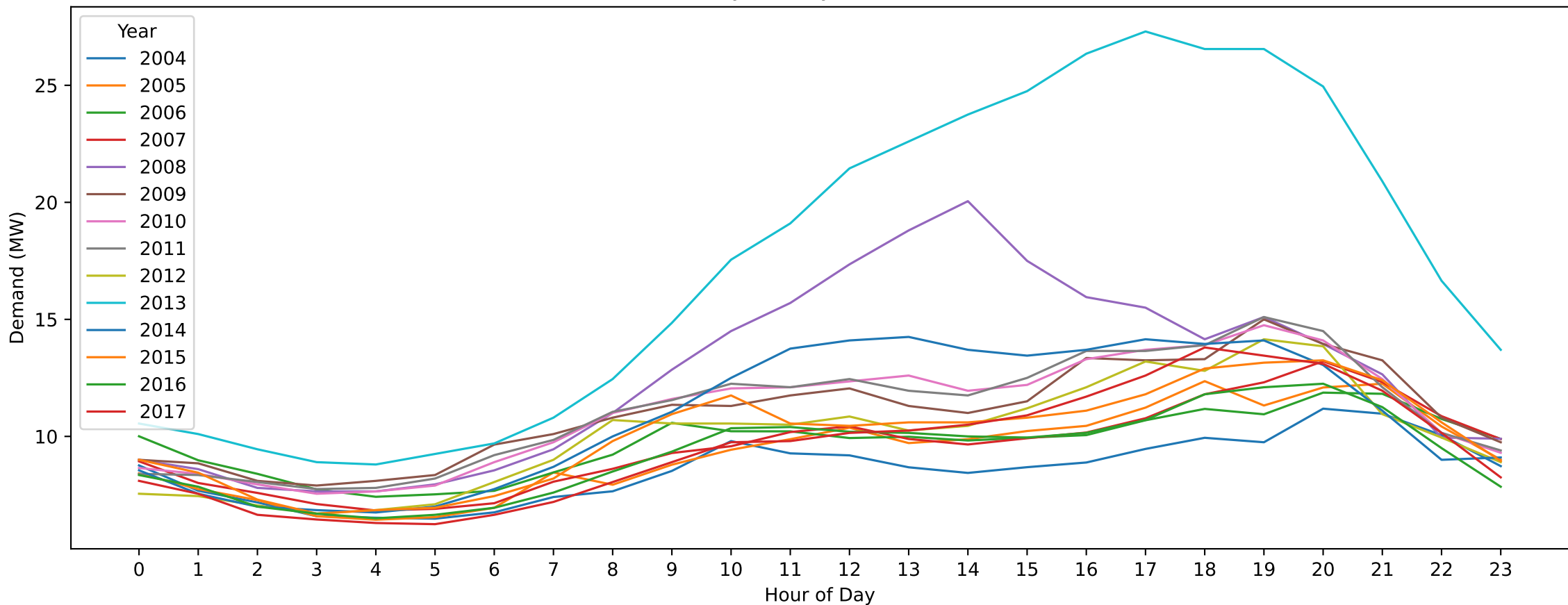
SR — Labour Day (Hourly Demand Across Years)
