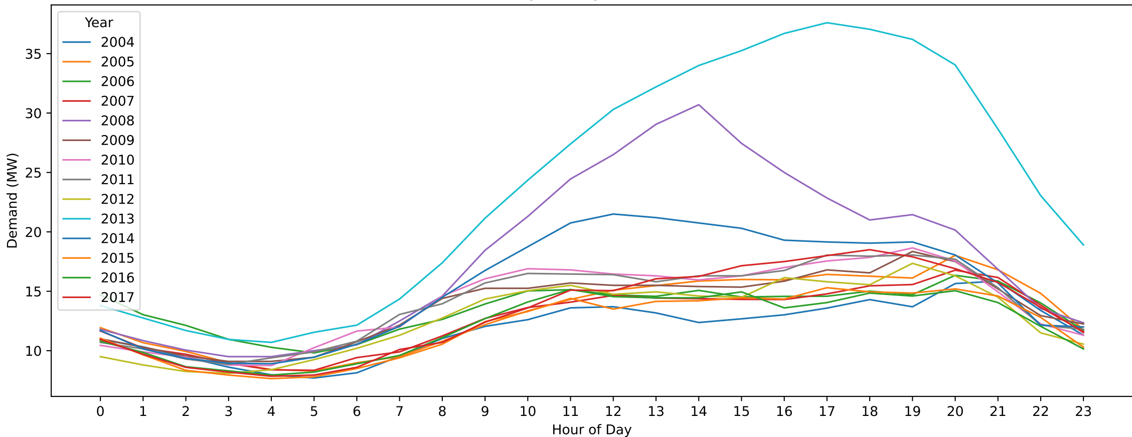
NB — Labour Day (Hourly Demand Across Years)
