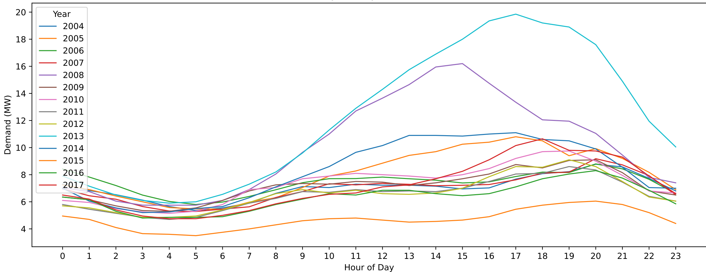
BW — Labour Day (Hourly Demand Across Years)
