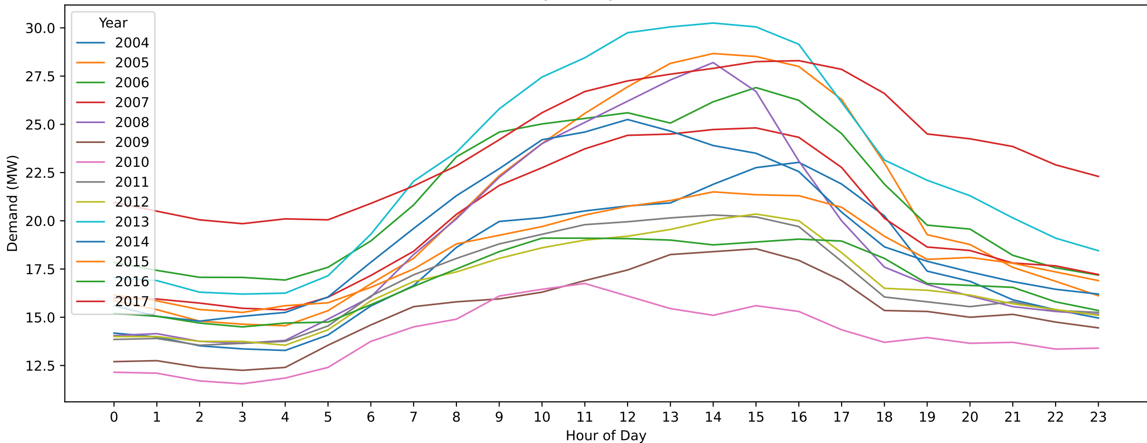
NO — Labour Day (Hourly Demand Across Years)
