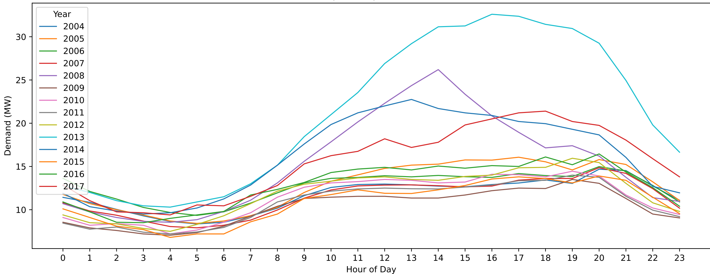
MR — Labour Day (Hourly Demand Across Years)
