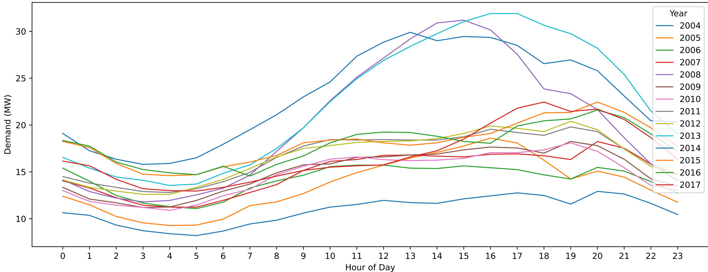
LD — Labour Day (Hourly Demand Across Years)
