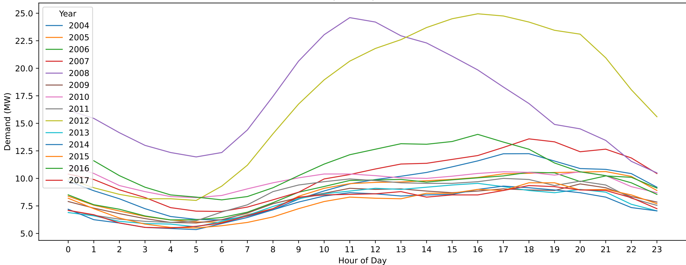
EL — New Year's Day (Hourly Demand Across Years)
