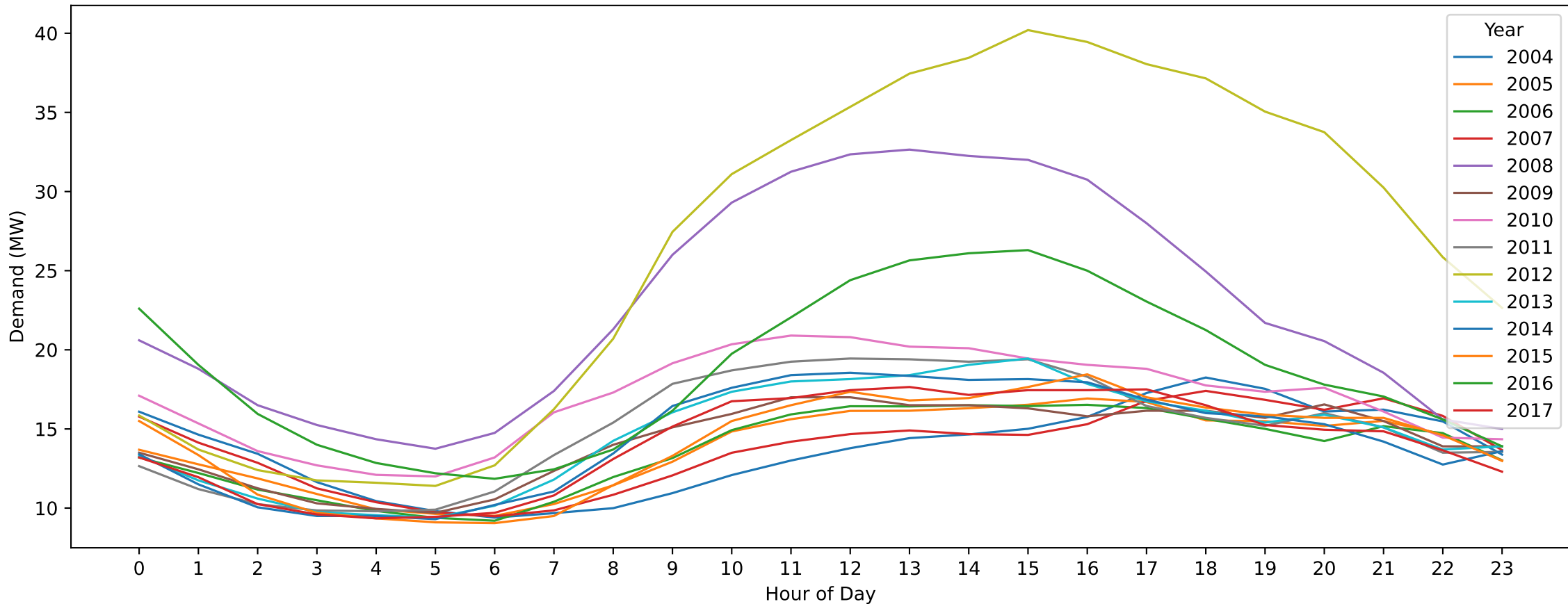
WD — New Year's Day (Hourly Demand Across Years)
