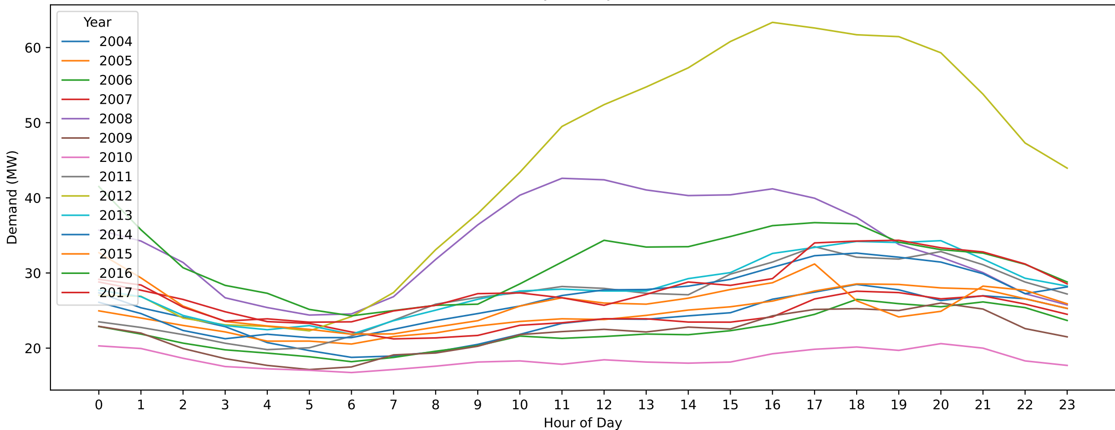
CRM — New Year's Day (Hourly Demand Across Years)
