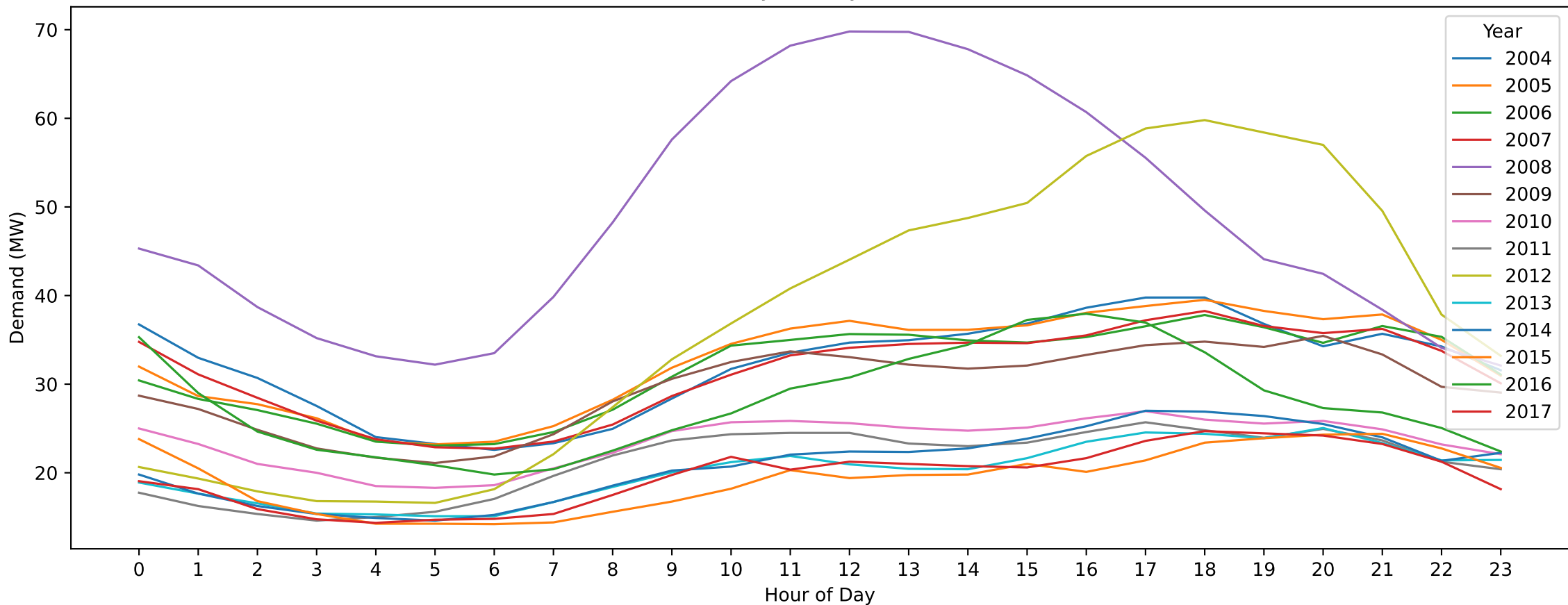
FSH — New Year's Day (Hourly Demand Across Years)
