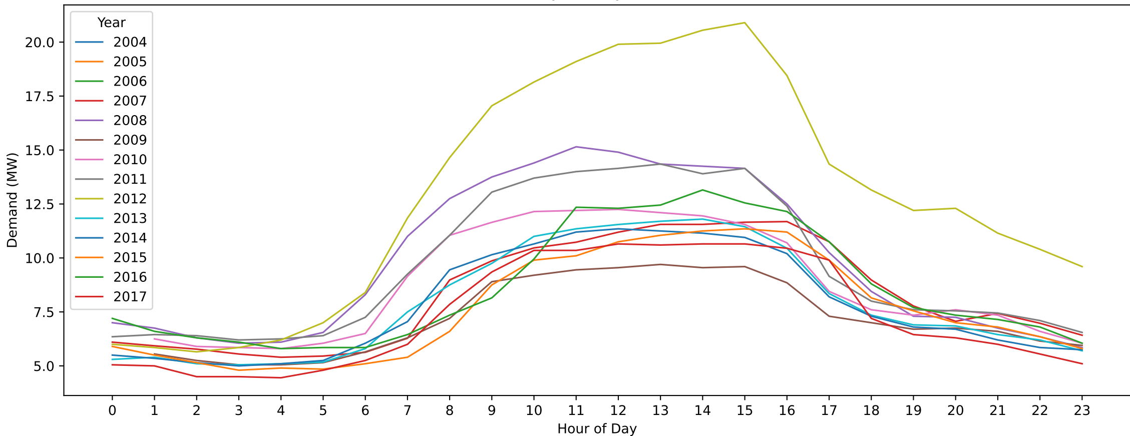
CM — New Year's Day (Hourly Demand Across Years)
