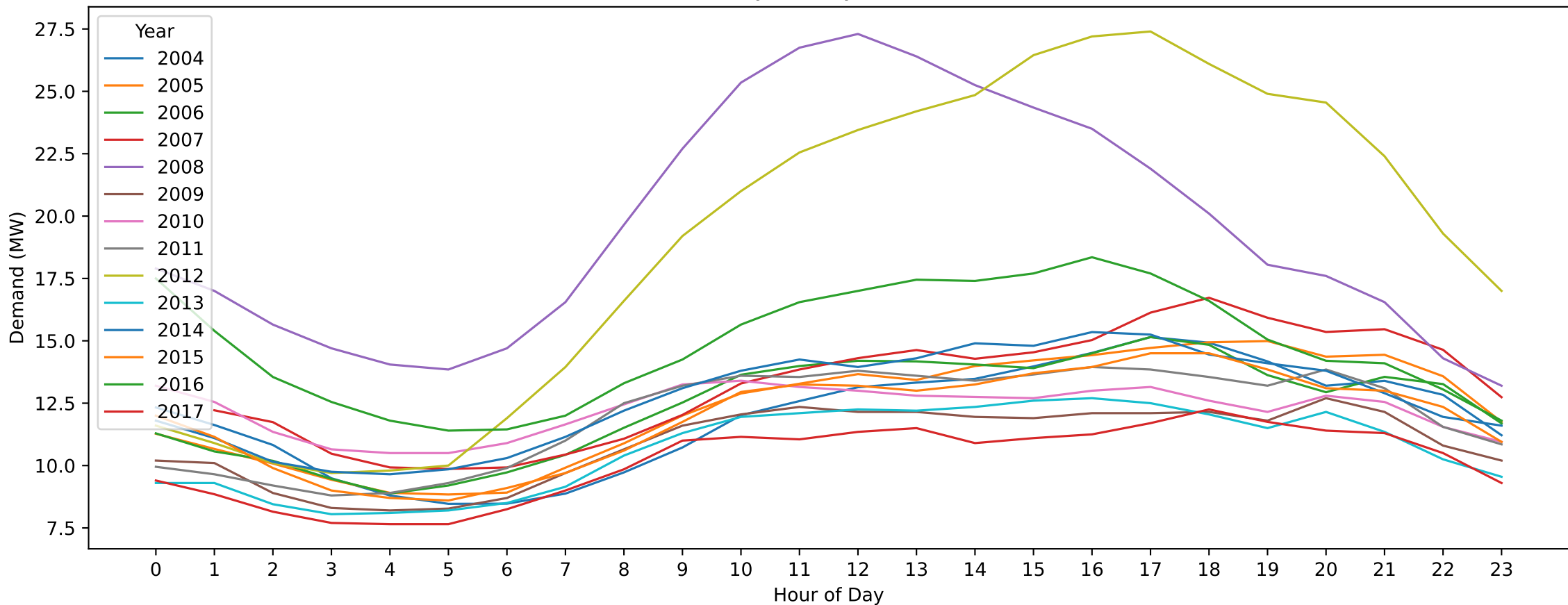
K — New Year's Day (Hourly Demand Across Years)
