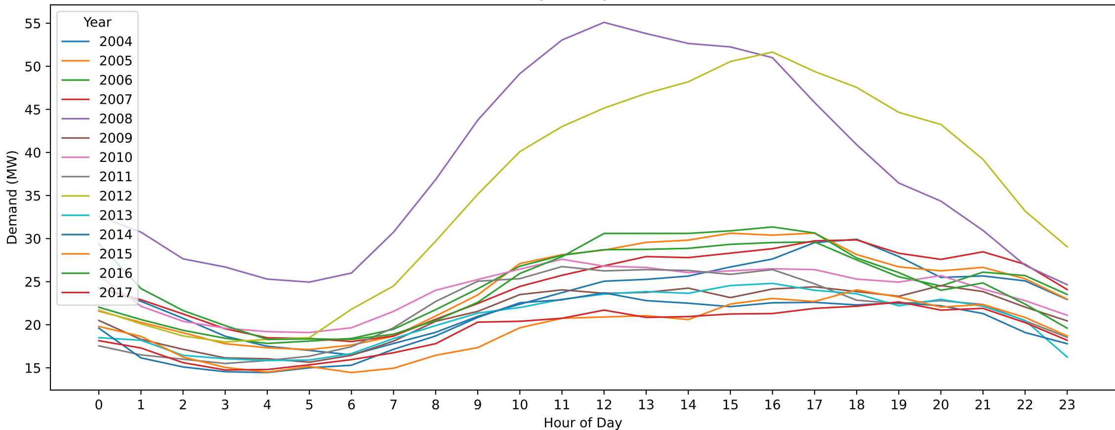
GW — New Year's Day (Hourly Demand Across Years)
