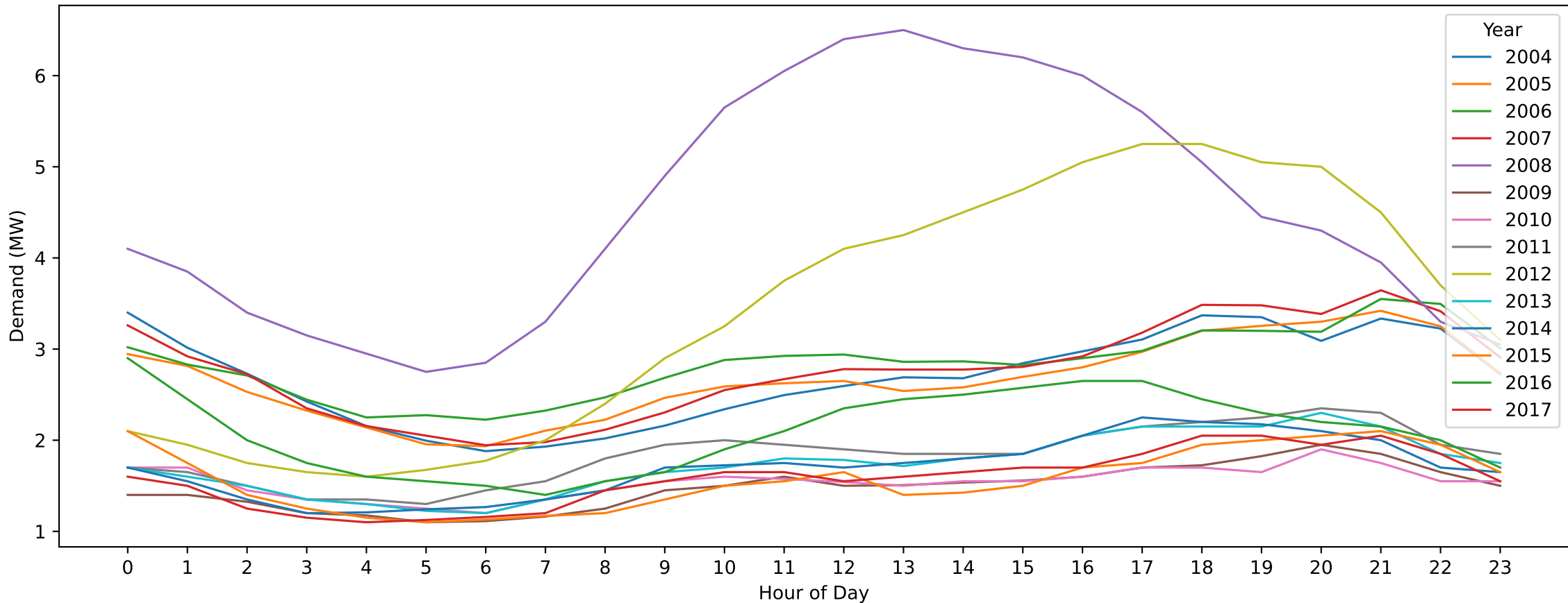
SH — New Year's Day (Hourly Demand Across Years)
