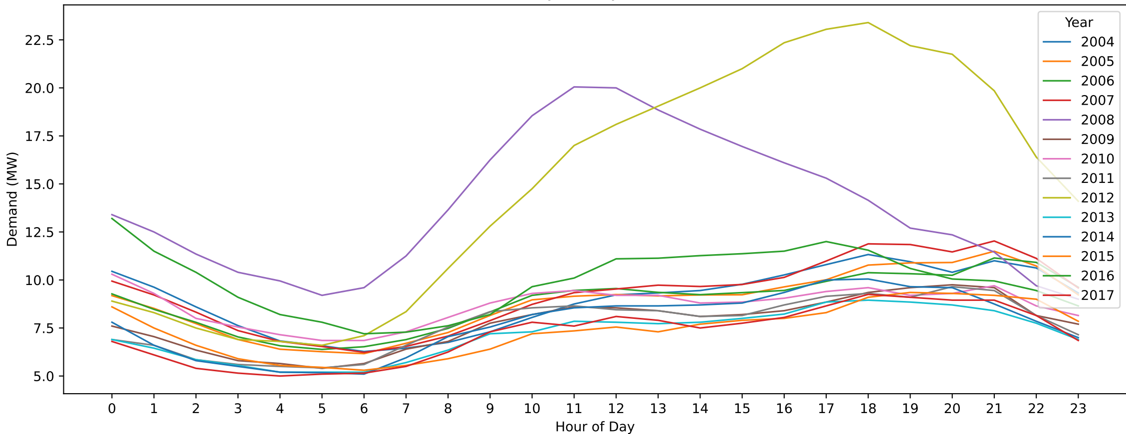
BT — New Year's Day (Hourly Demand Across Years)
