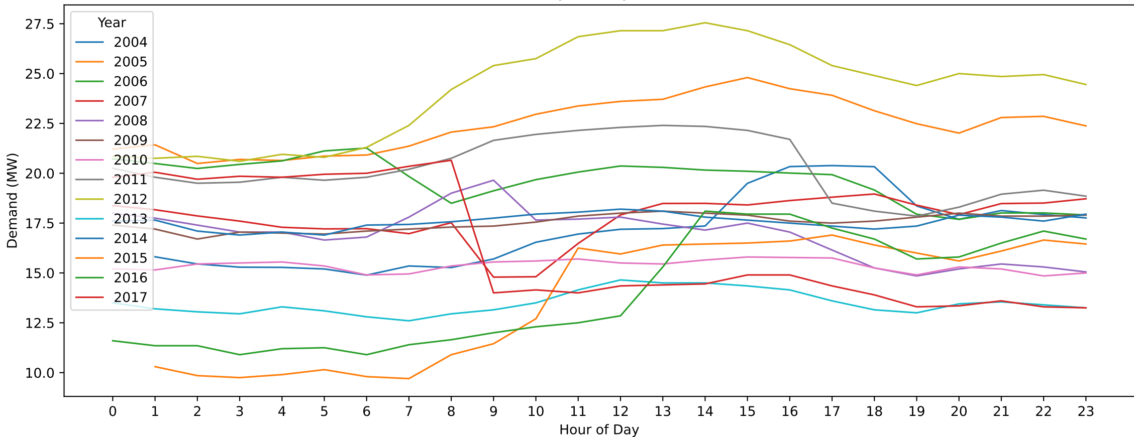
DSH — New Year's Day (Hourly Demand Across Years)
