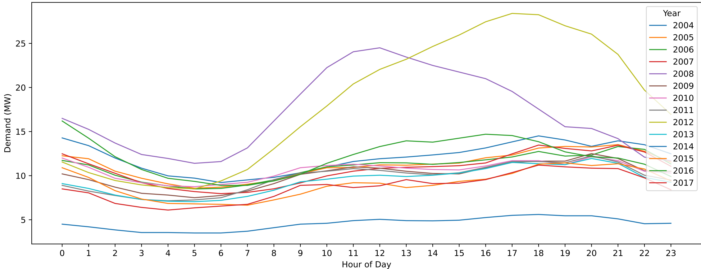
OR — New Year's Day (Hourly Demand Across Years)
