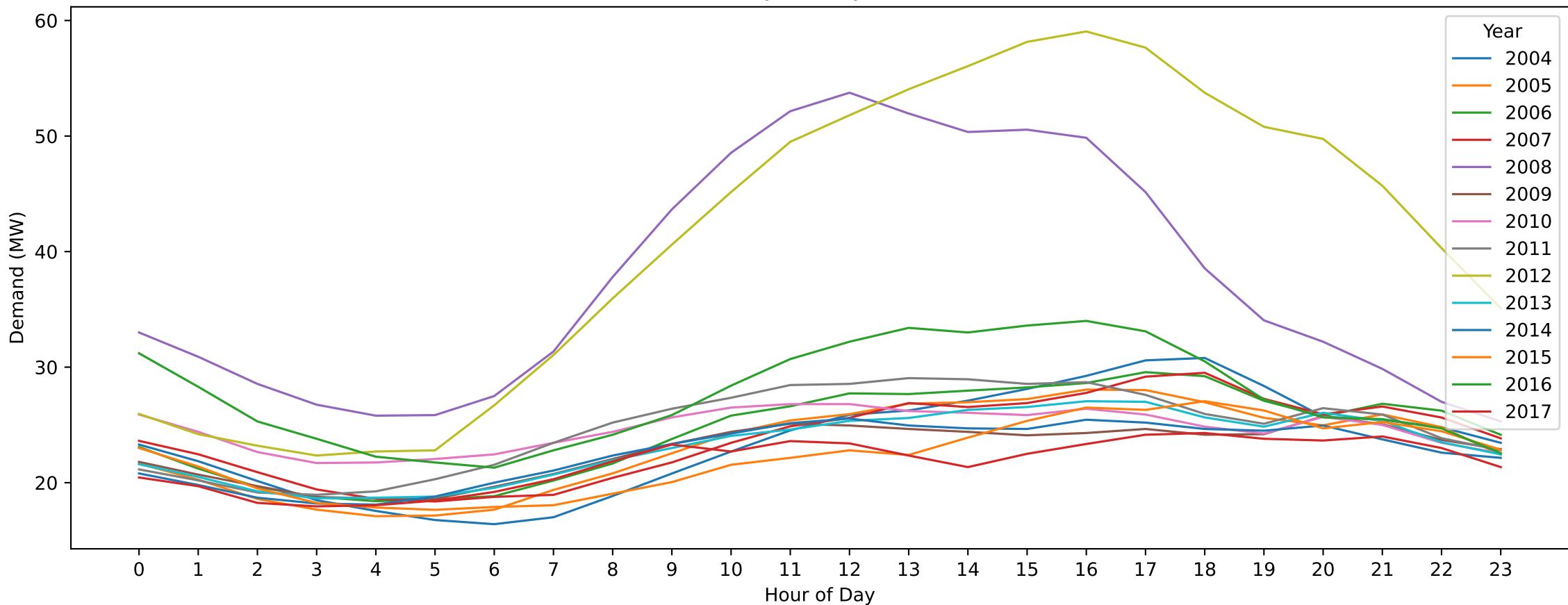
MGE — New Year's Day (Hourly Demand Across Years)
