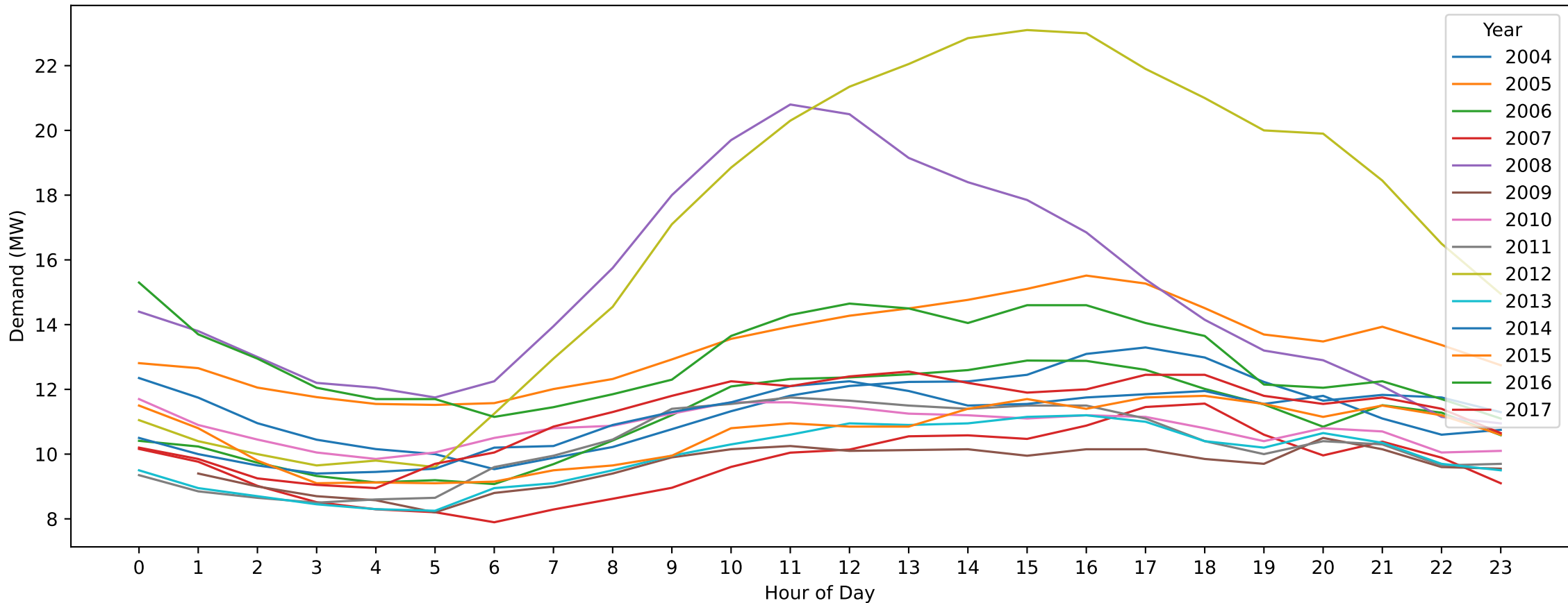
HT — New Year's Day (Hourly Demand Across Years)
