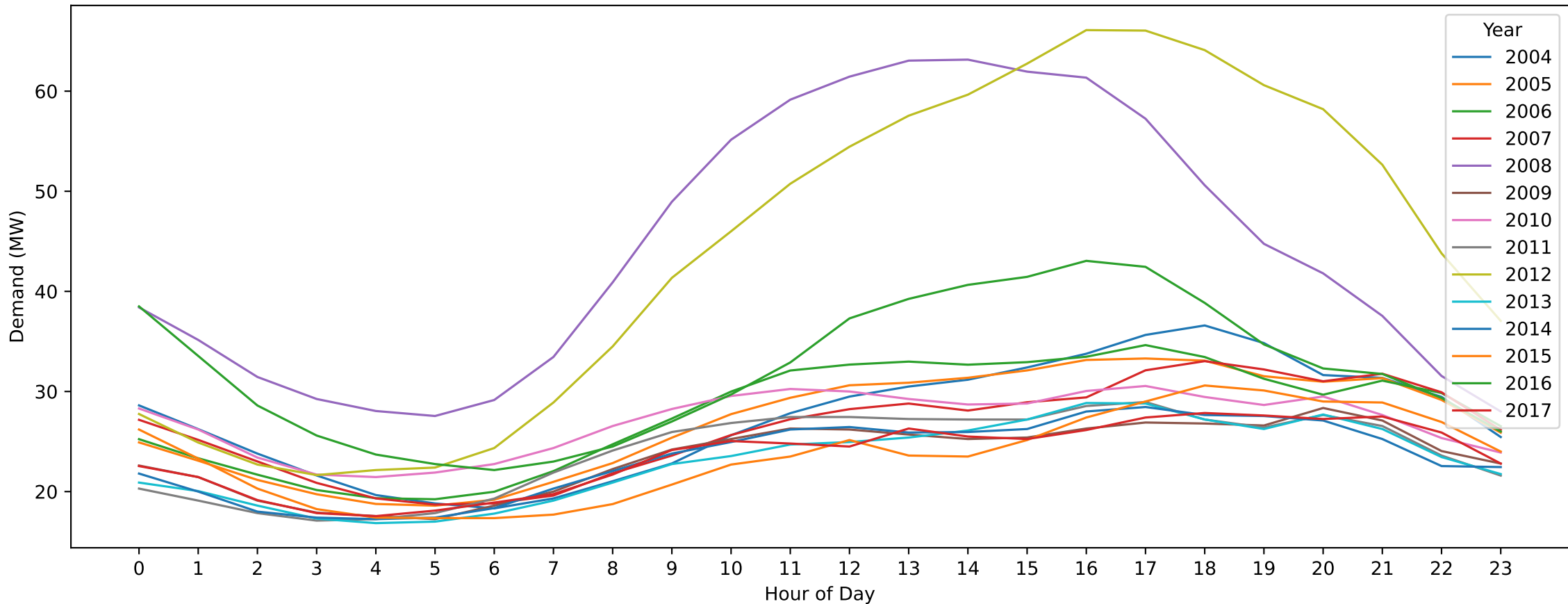
DC — New Year's Day (Hourly Demand Across Years)
