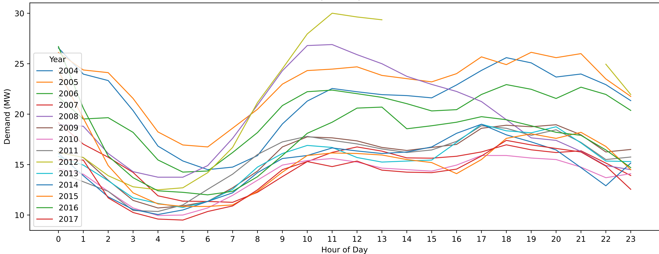
RBD — New Year's Day (Hourly Demand Across Years)
