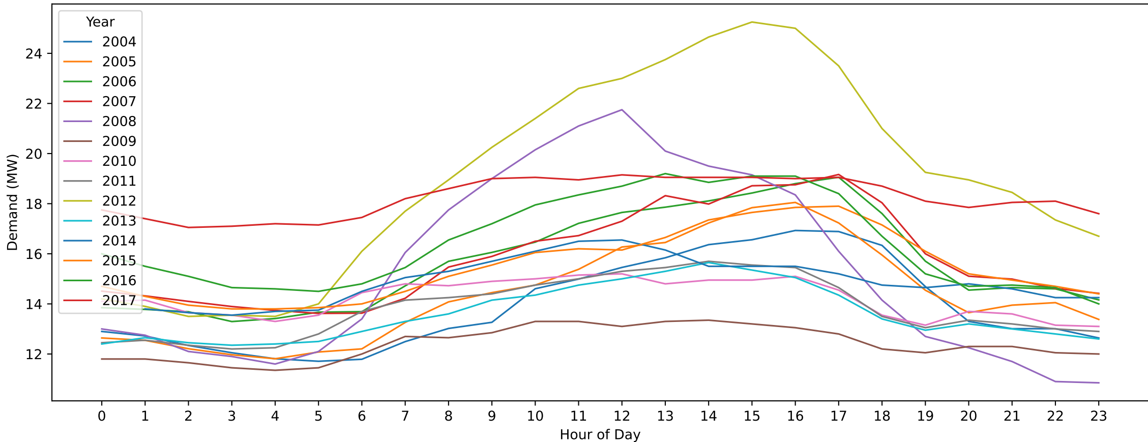
NO — New Year's Day (Hourly Demand Across Years)
