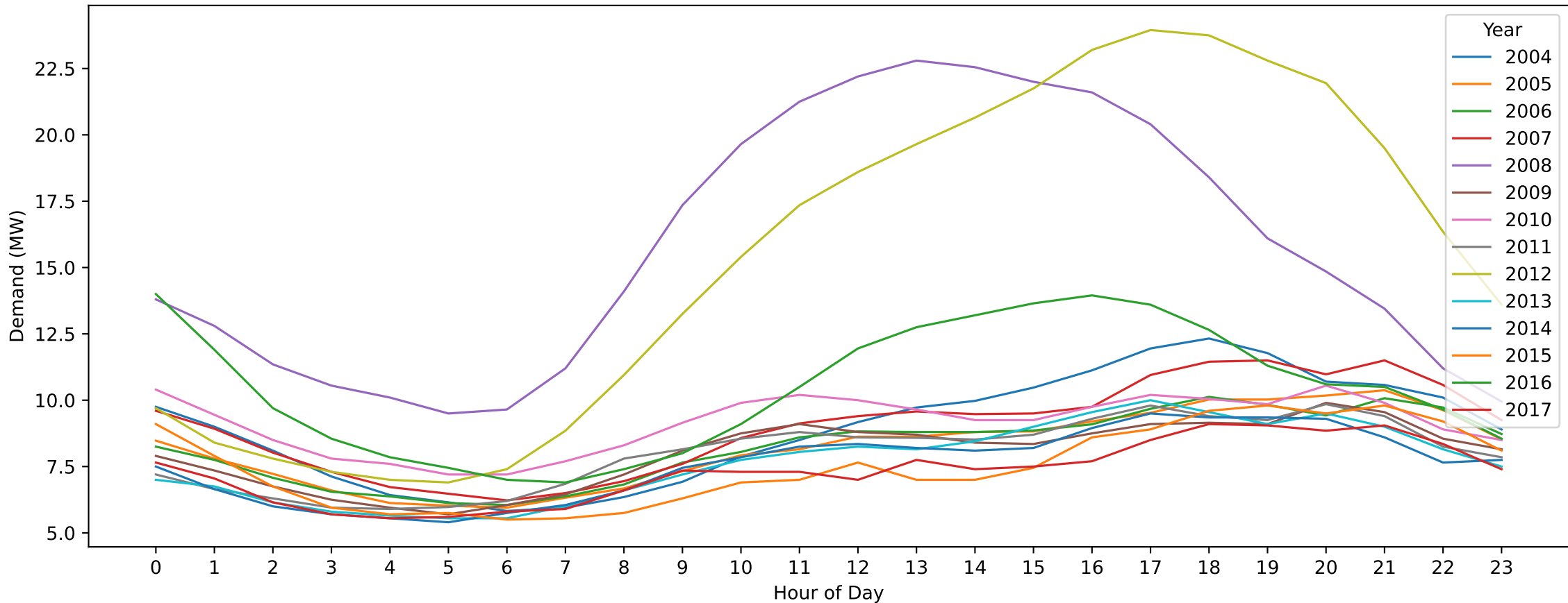
BU — New Year's Day (Hourly Demand Across Years)
