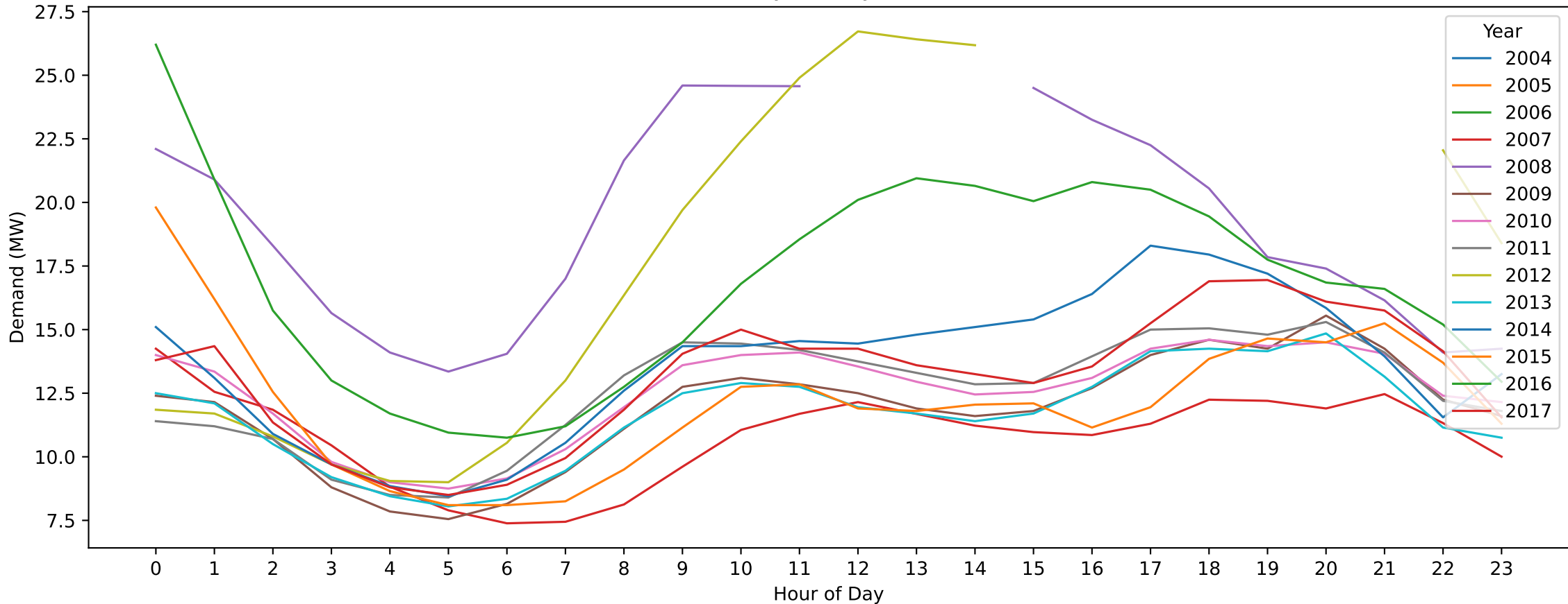
DMA — New Year's Day (Hourly Demand Across Years)
