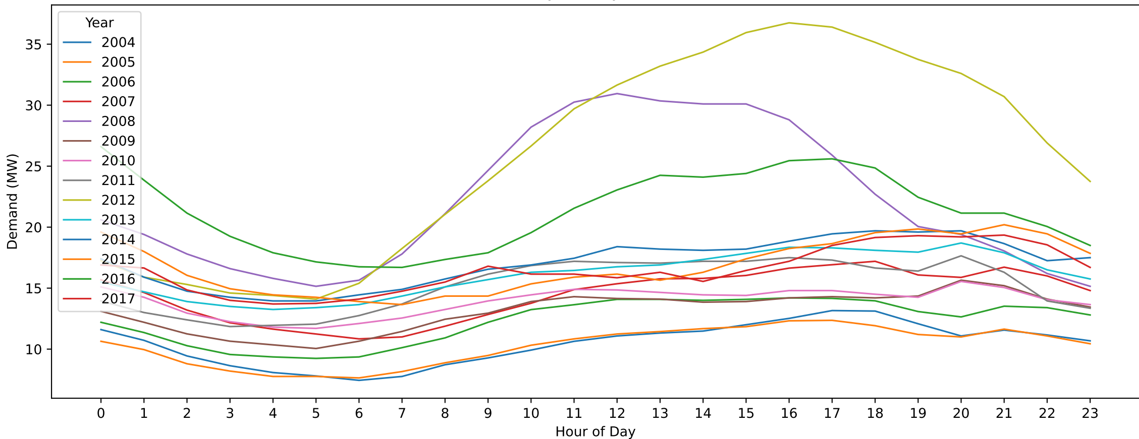
LD — New Year's Day (Hourly Demand Across Years)
