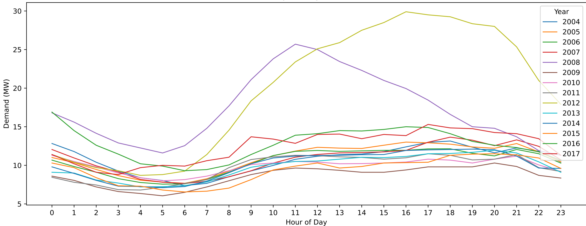
MR — New Year's Day (Hourly Demand Across Years)
