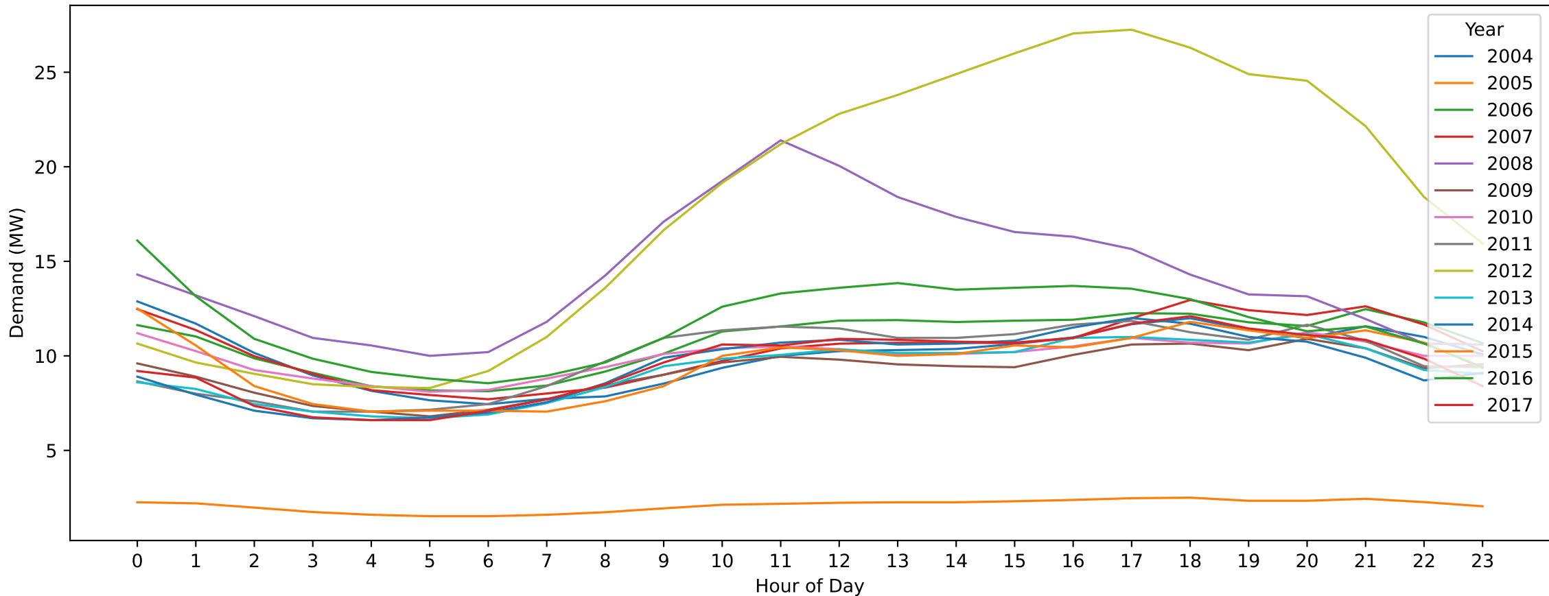
M — New Year's Day (Hourly Demand Across Years)
