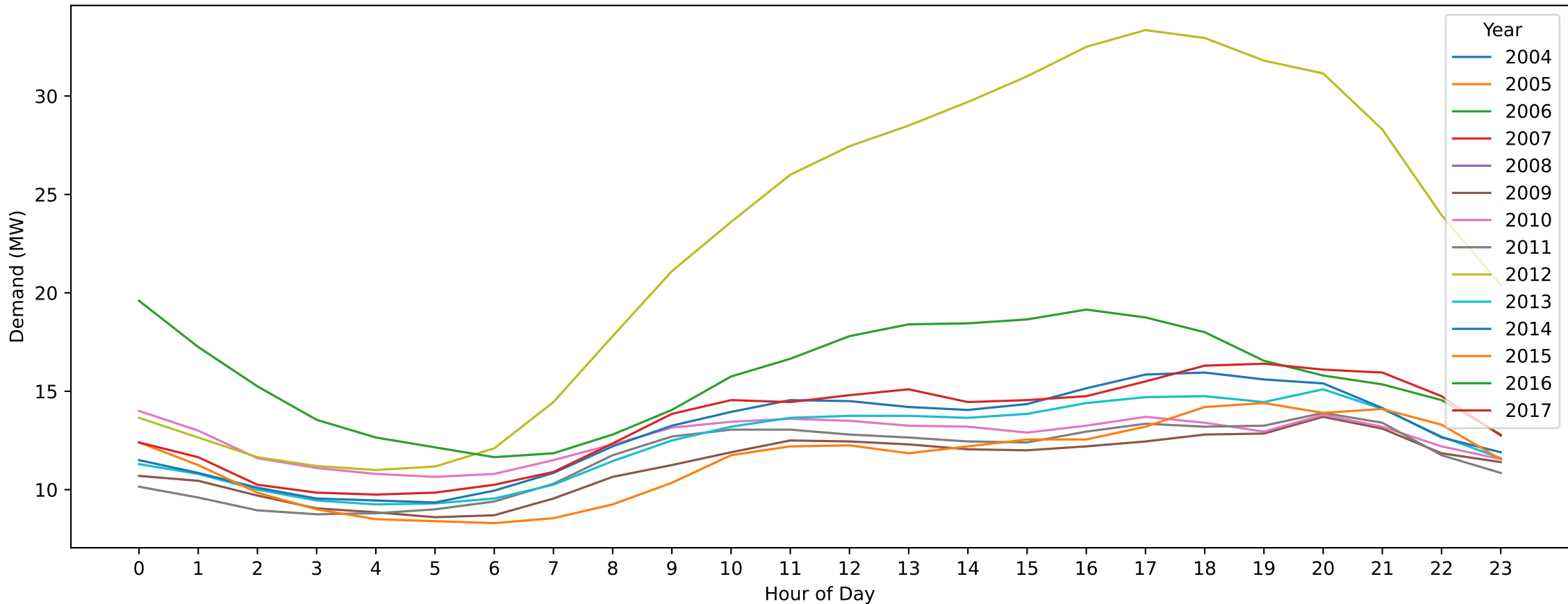
CFD — New Year's Day (Hourly Demand Across Years)
