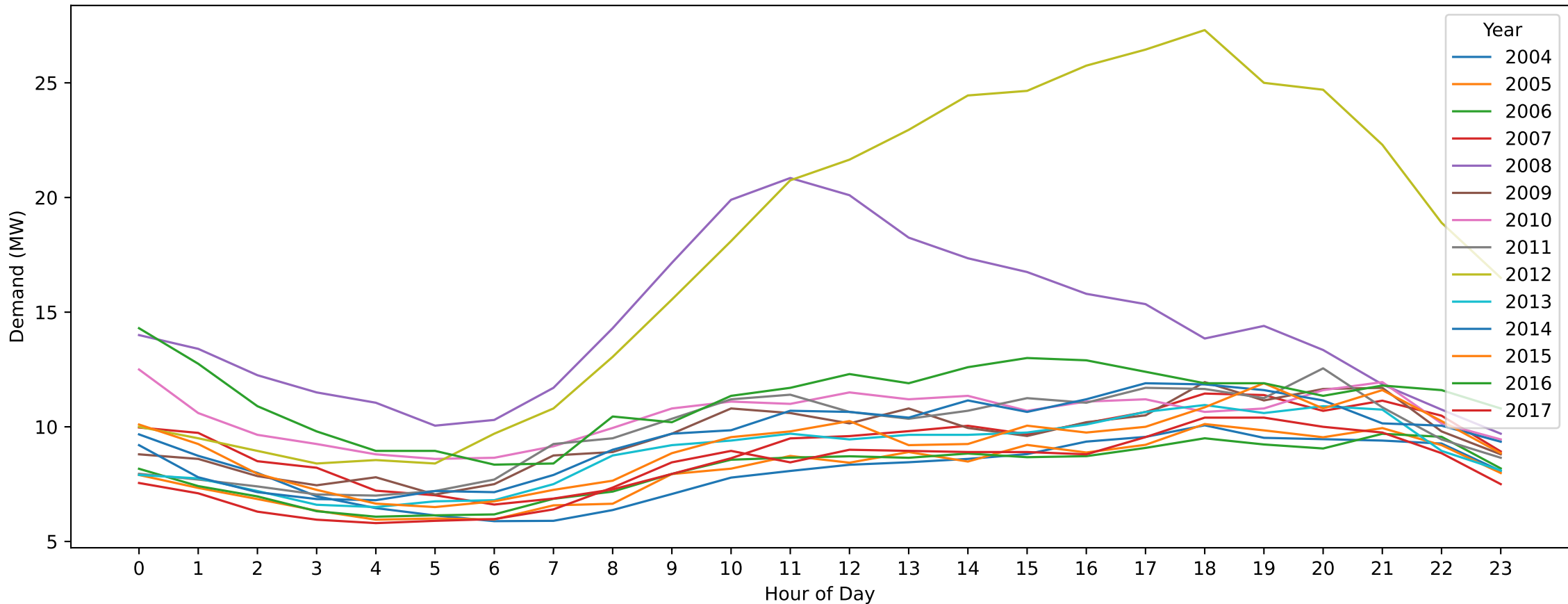
SR — New Year's Day (Hourly Demand Across Years)
