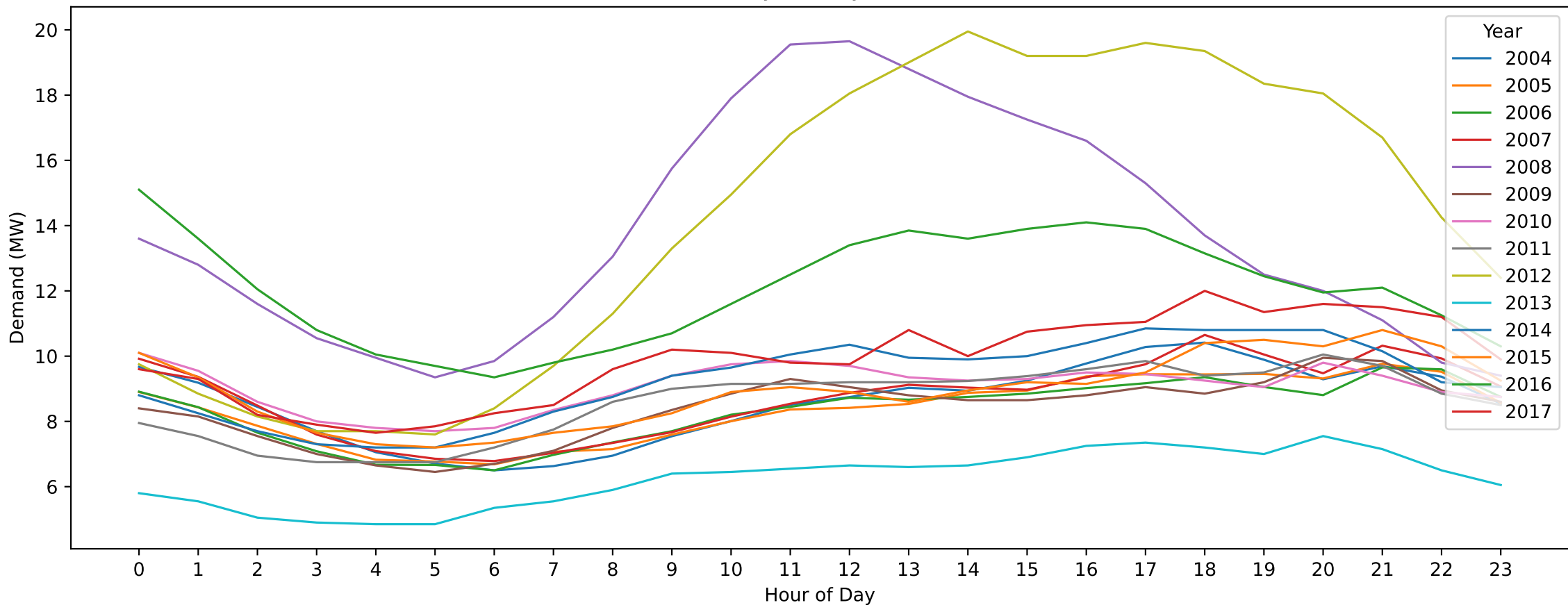
CDA — New Year's Day (Hourly Demand Across Years)
