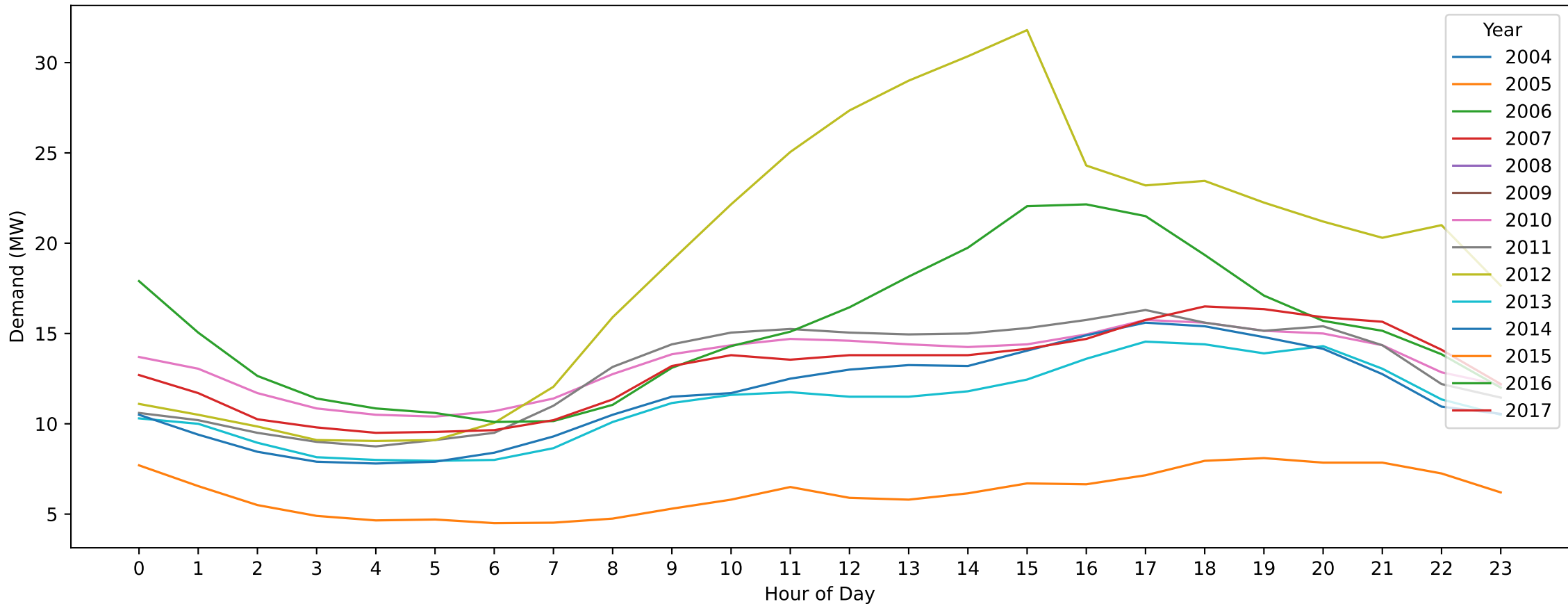
LWN — New Year's Day (Hourly Demand Across Years)
