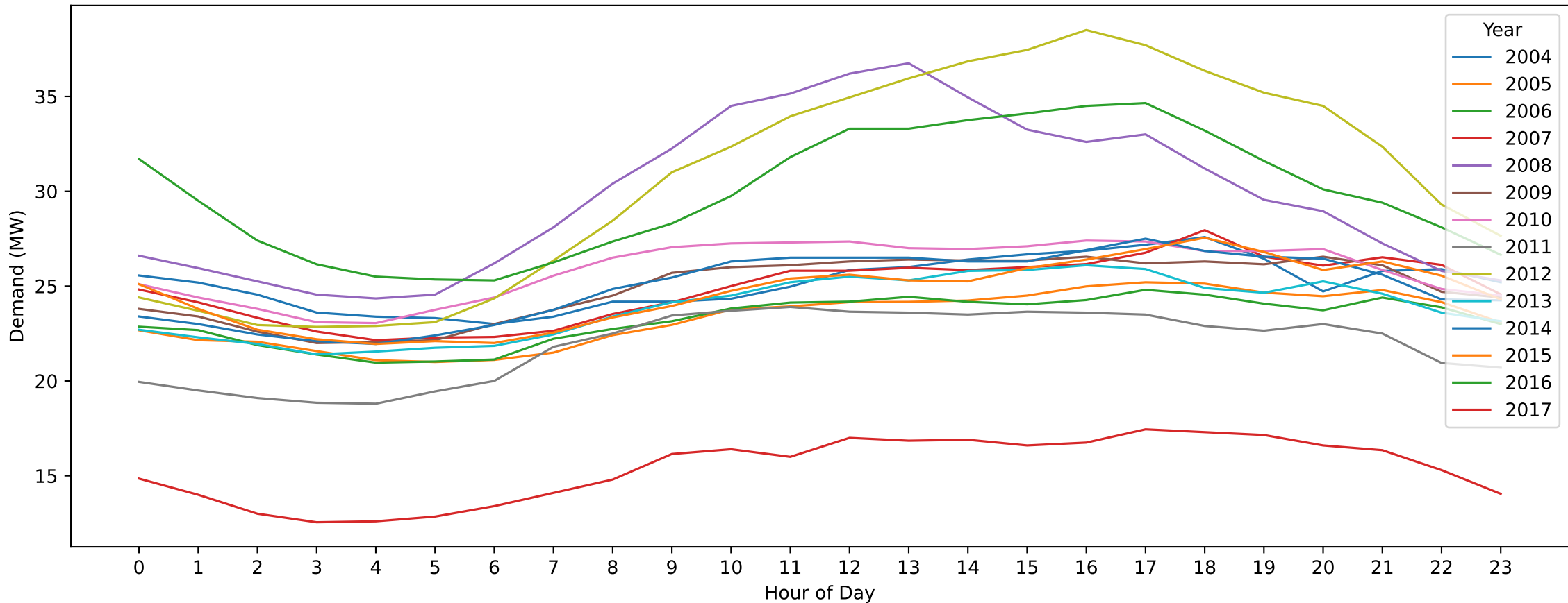
BH — New Year's Day (Hourly Demand Across Years)
