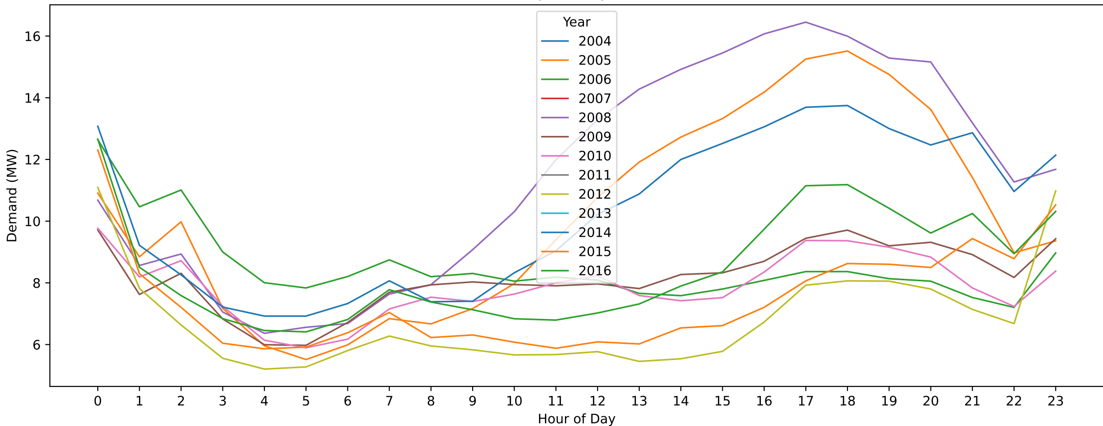
Charlton — Labour Day (Hourly Demand Across Years)
