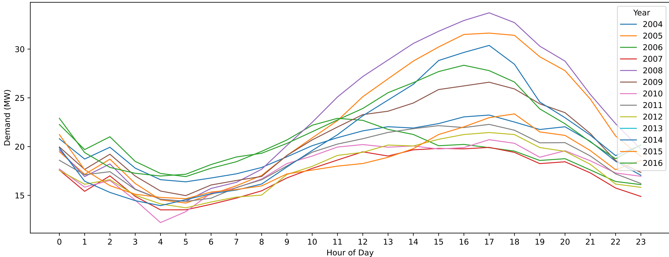
Shepparton — Labour Day (Hourly Demand Across Years)
