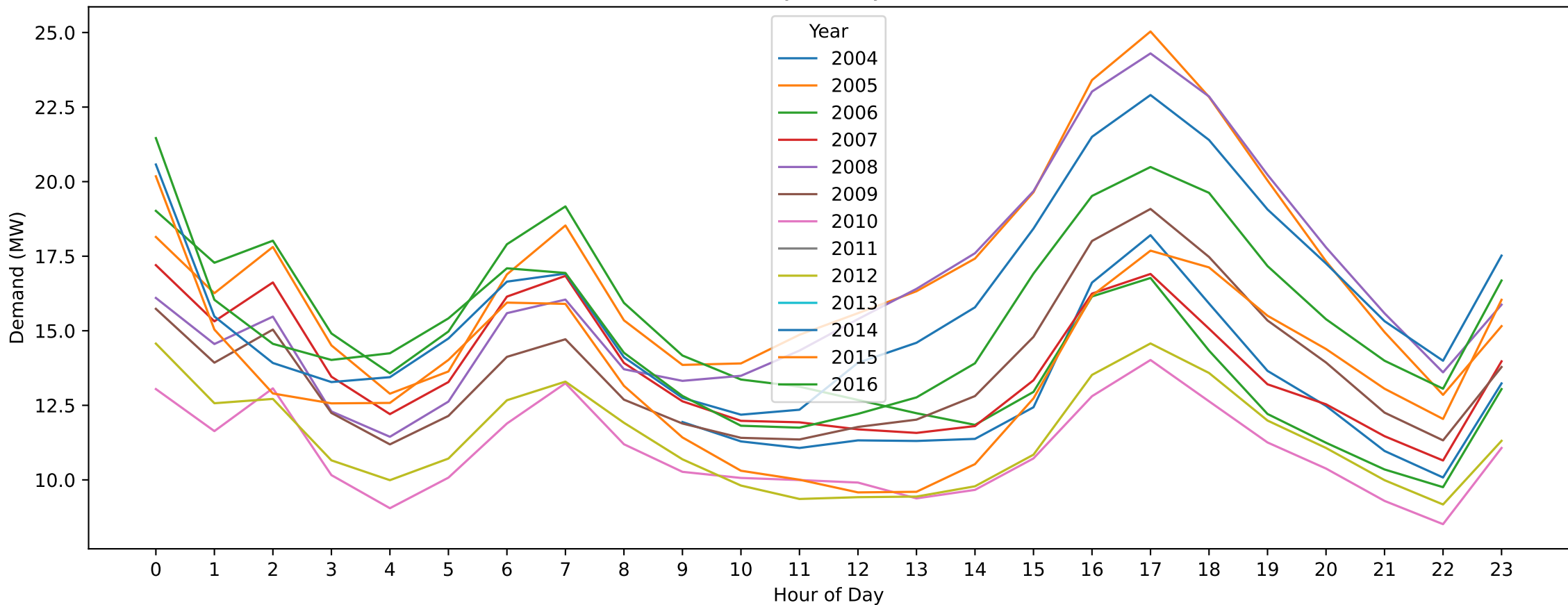
Numurkah — Labour Day (Hourly Demand Across Years)
