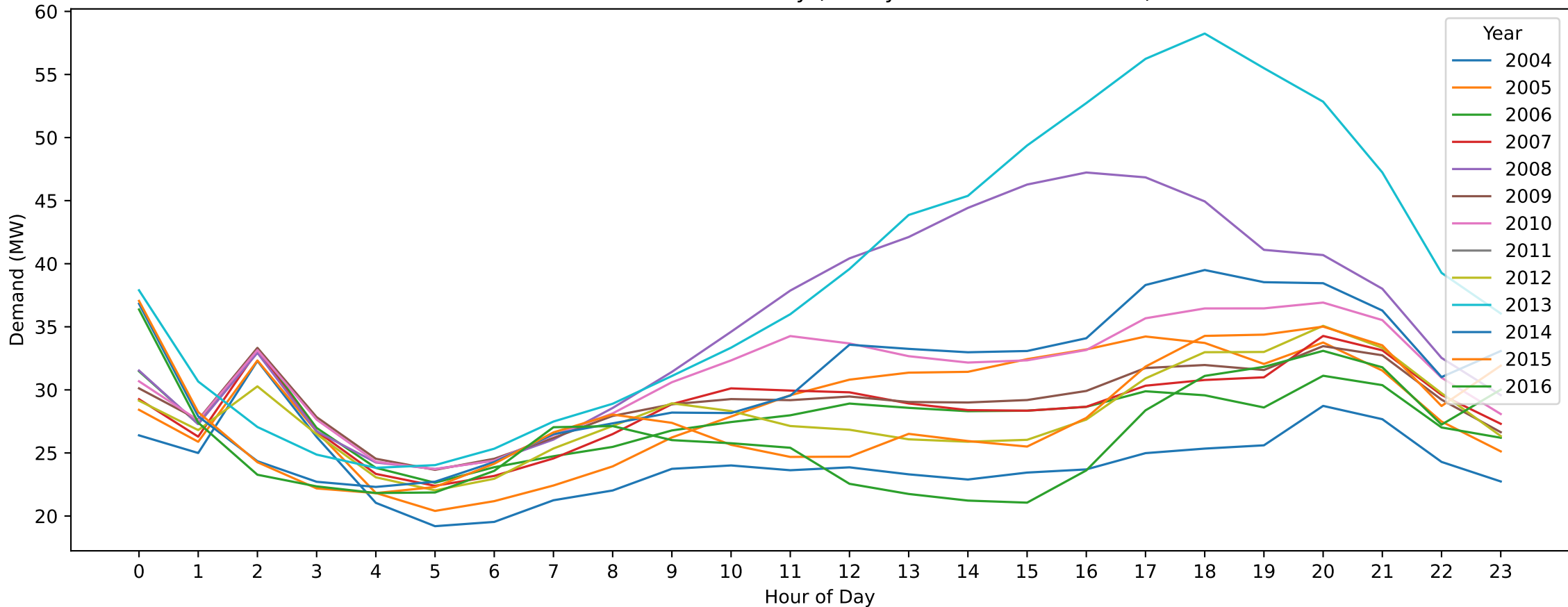
Ballarat South — Labour Day (Hourly Demand Across Years)
