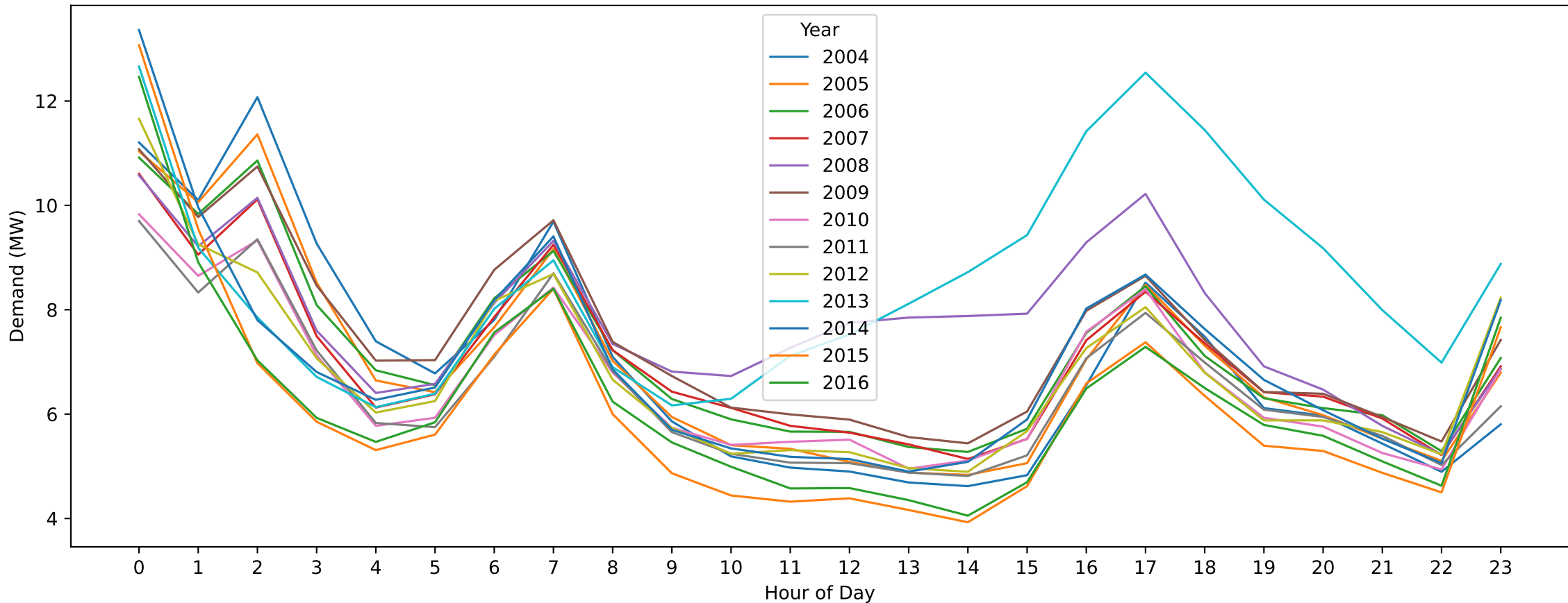
Camperdown — Labour Day (Hourly Demand Across Years)
