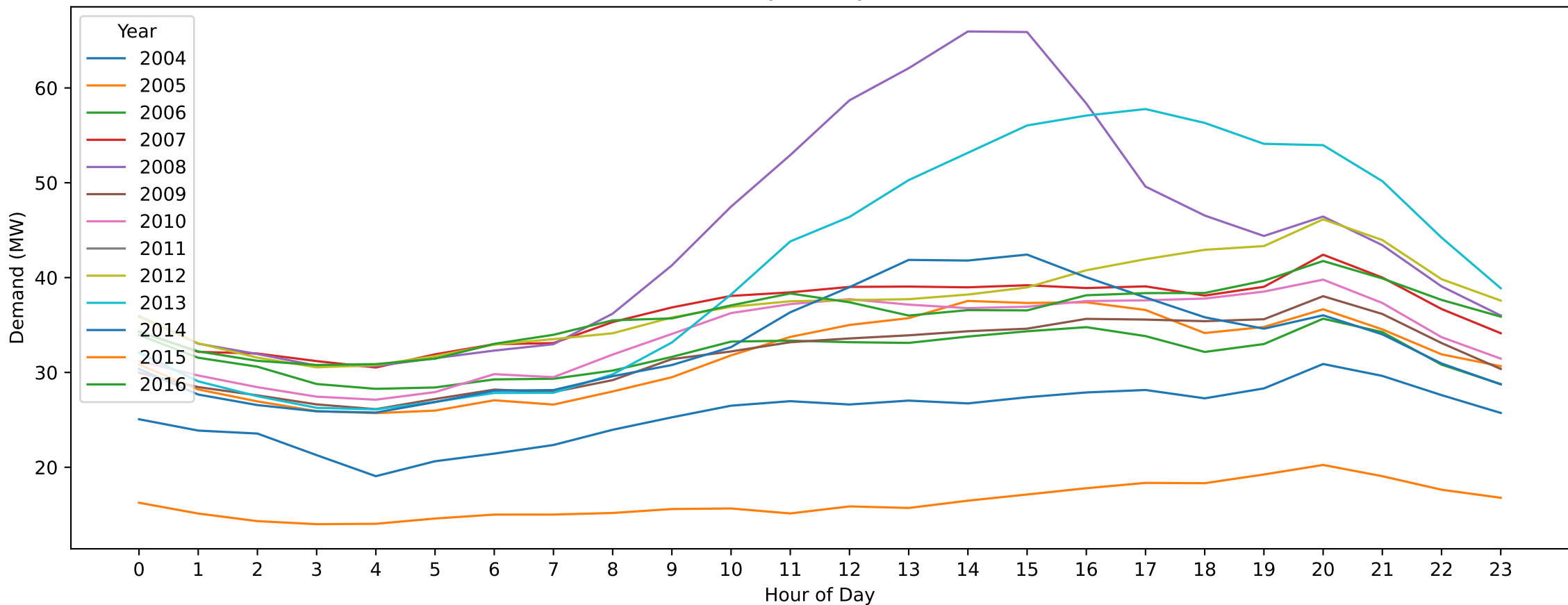
Sunshine — Labour Day (Hourly Demand Across Years)
