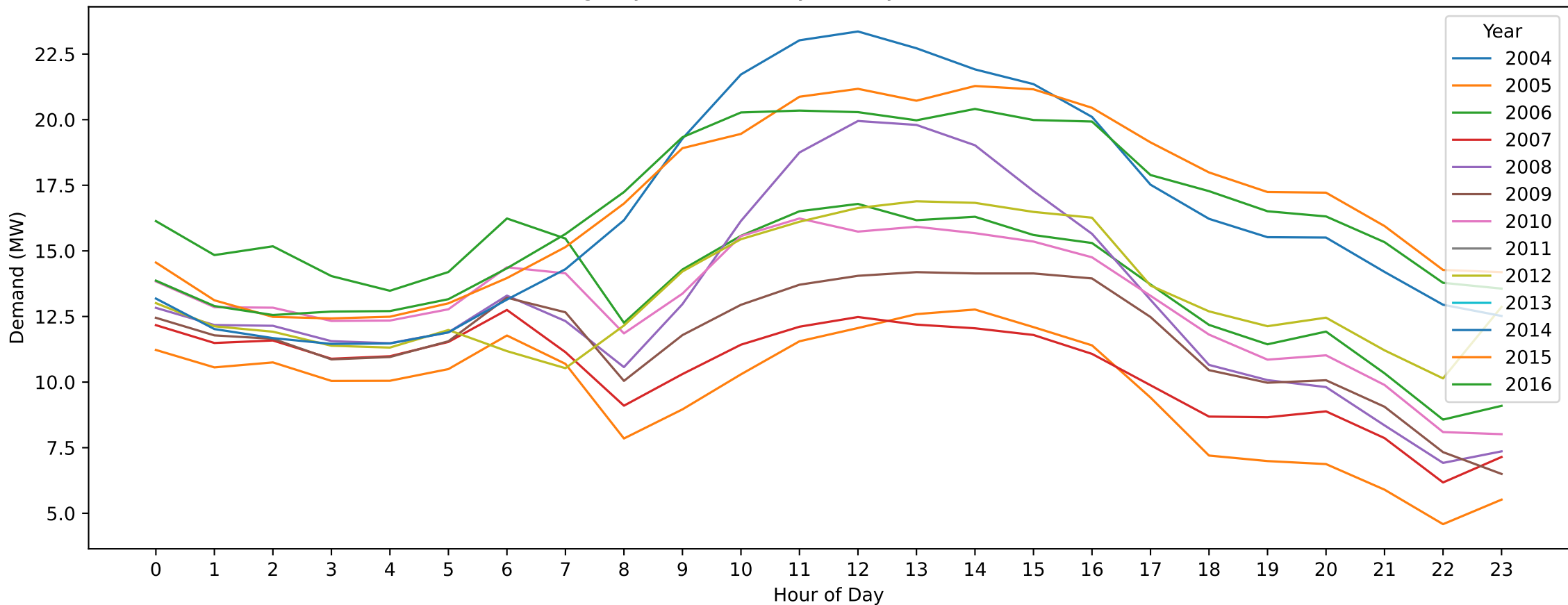
Geelong City — Labour Day (Hourly Demand Across Years)
