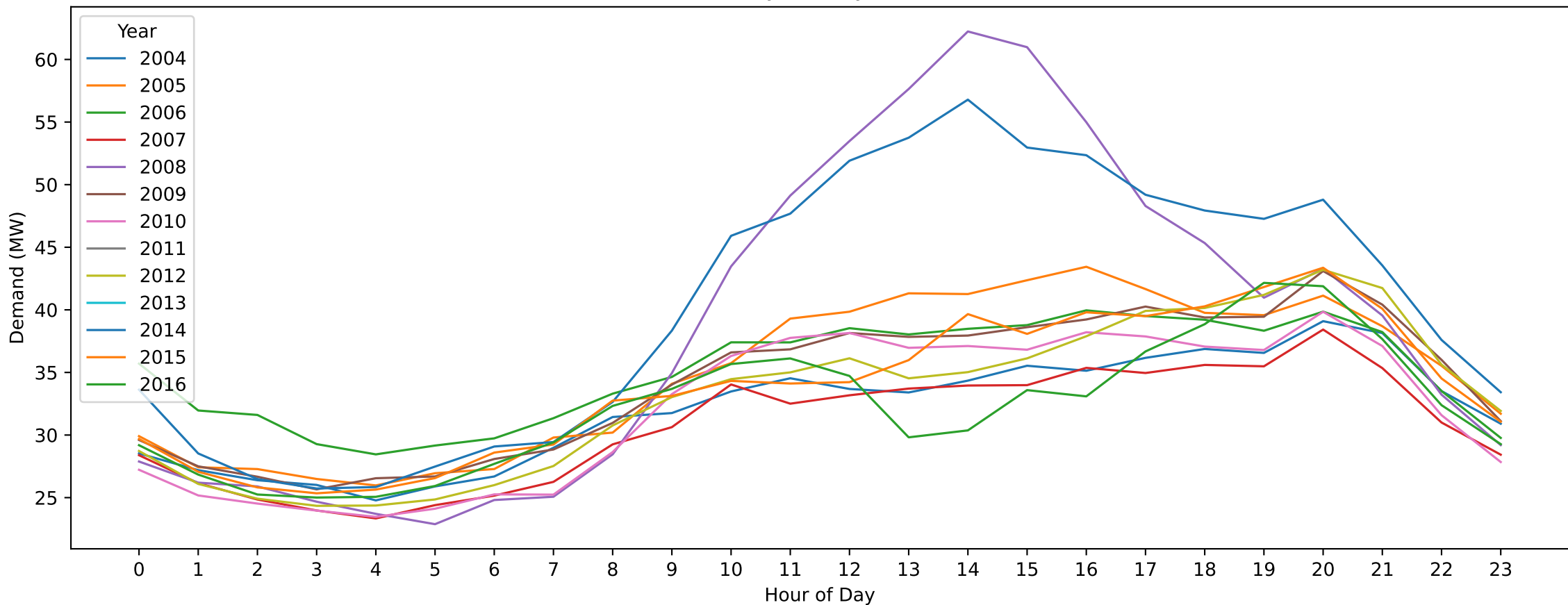
Laverton — Labour Day (Hourly Demand Across Years)
