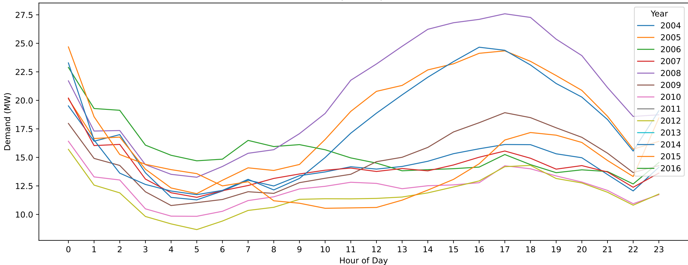
Swan Hill — Labour Day (Hourly Demand Across Years)
