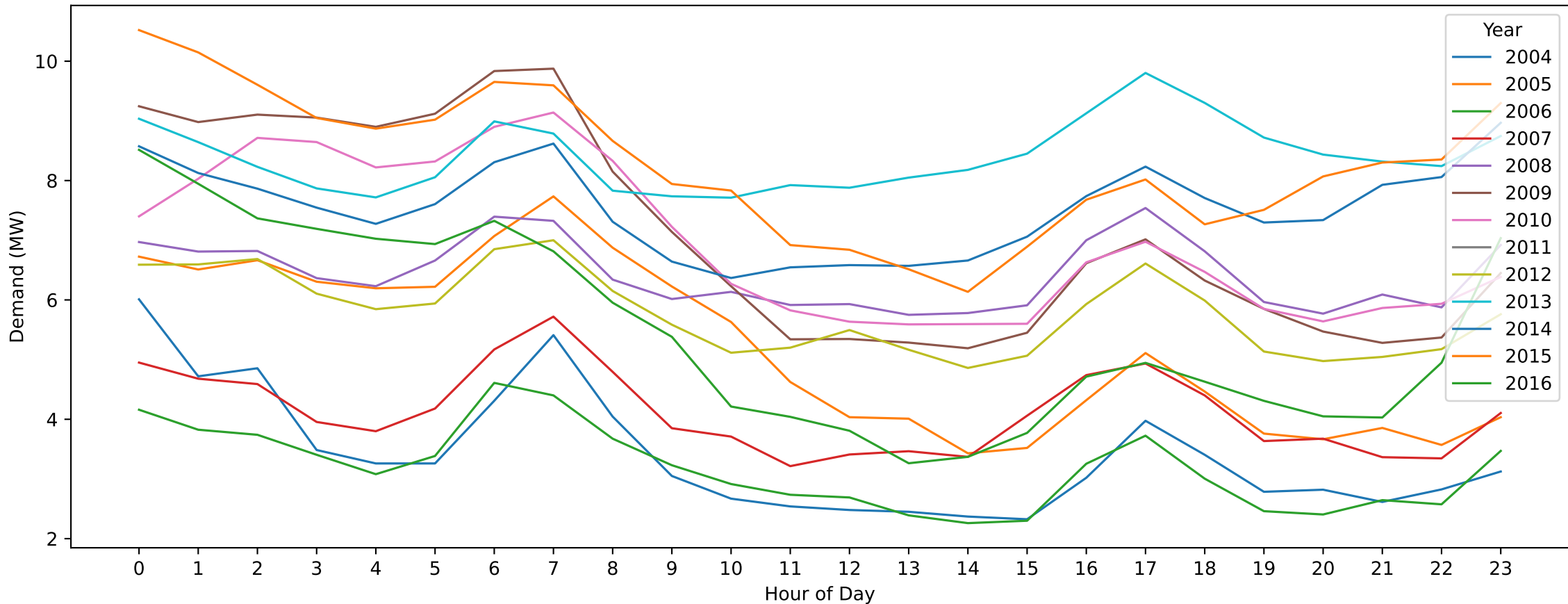
Cobden — Labour Day (Hourly Demand Across Years)
