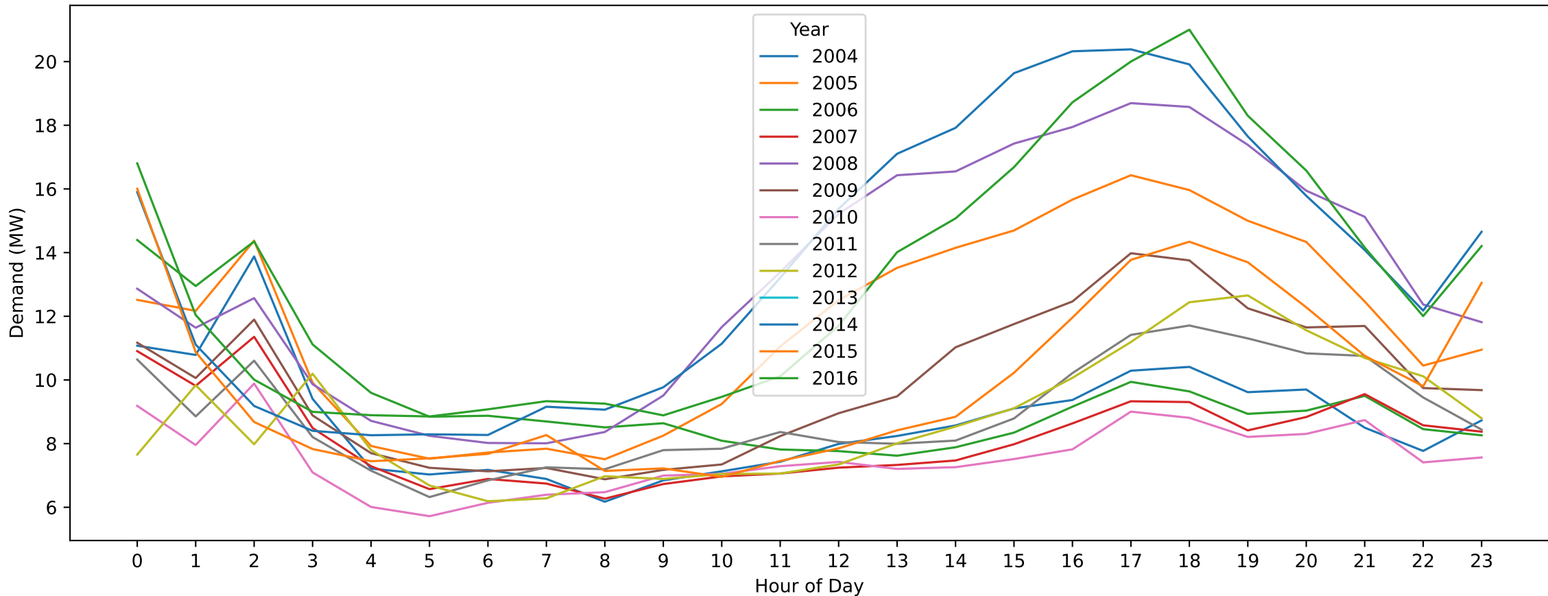
Merbein — Labour Day (Hourly Demand Across Years)
