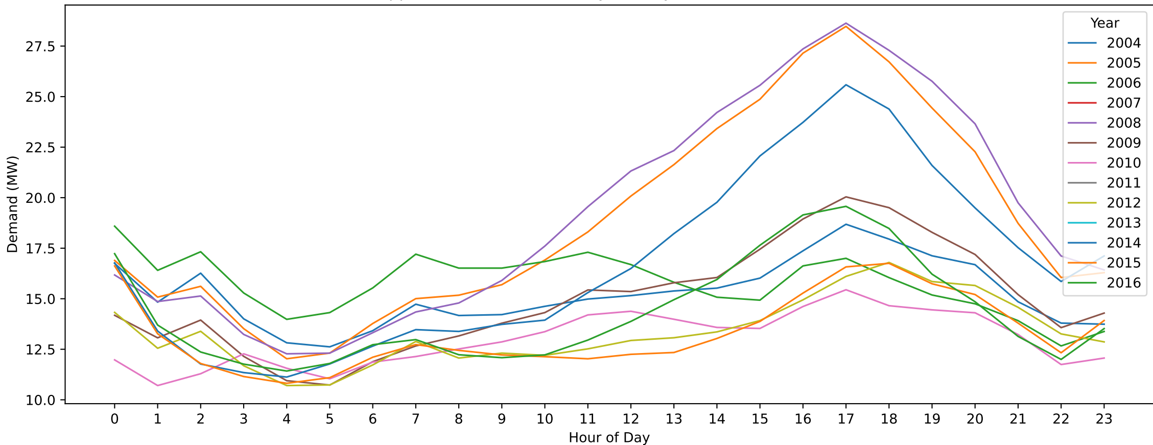
Shepparton Nth — Labour Day (Hourly Demand Across Years)
