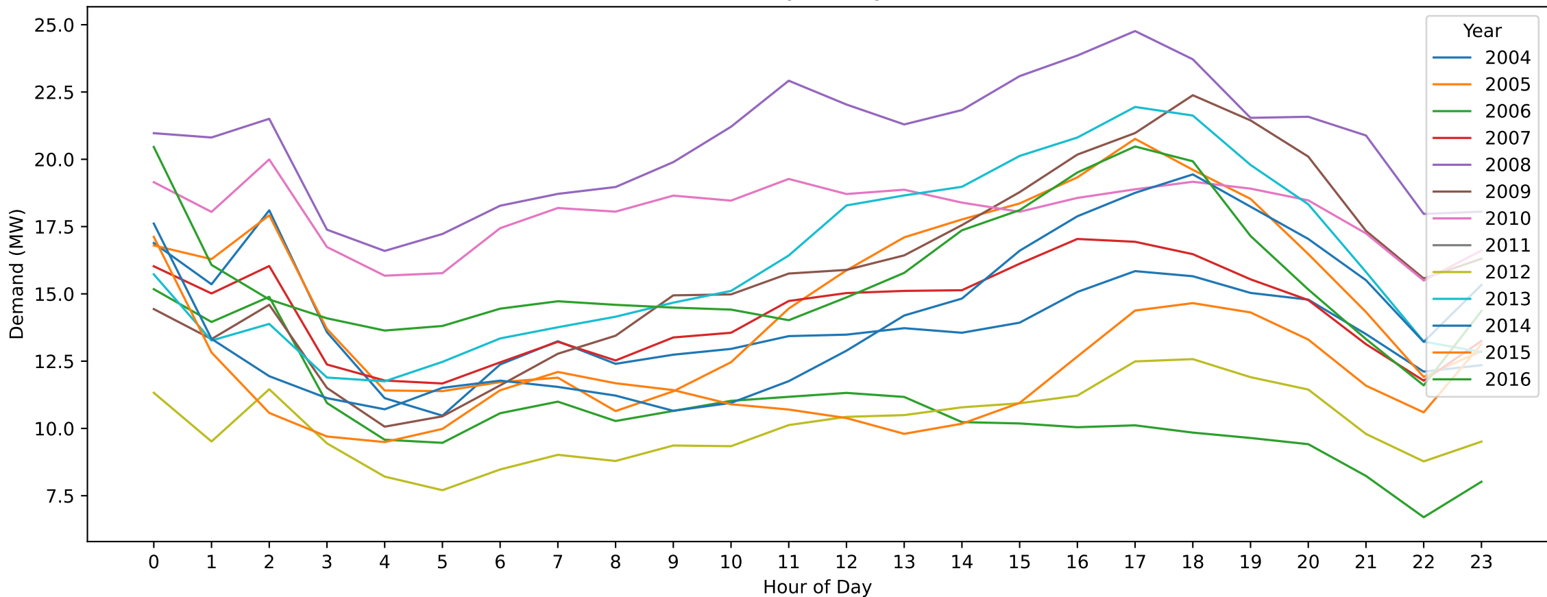
Cobram East — Labour Day (Hourly Demand Across Years)
