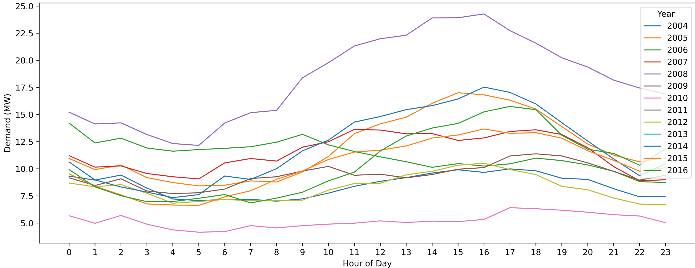
Robinvale — Labour Day (Hourly Demand Across Years)
