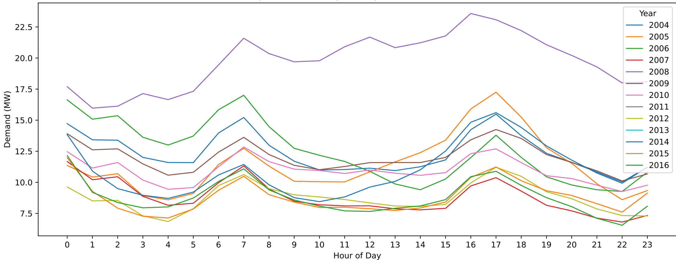
Stanhope — Labour Day (Hourly Demand Across Years)
