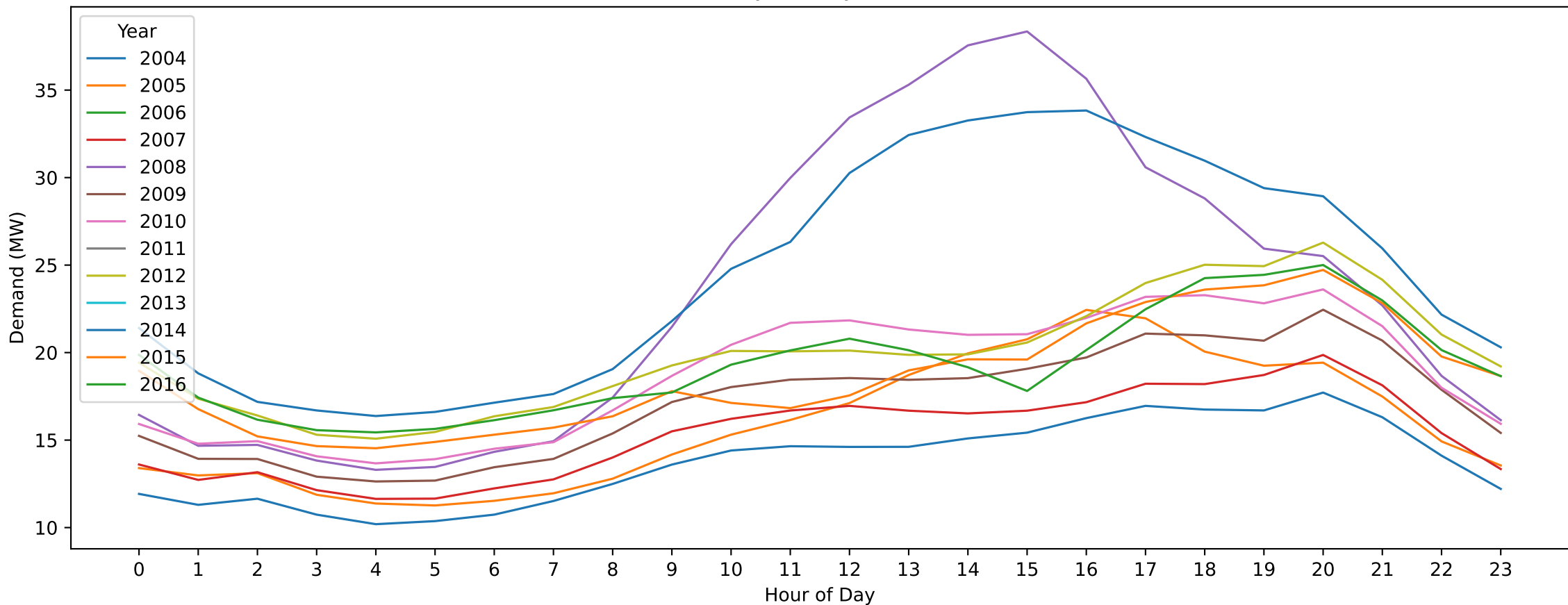
Melton — Labour Day (Hourly Demand Across Years)
