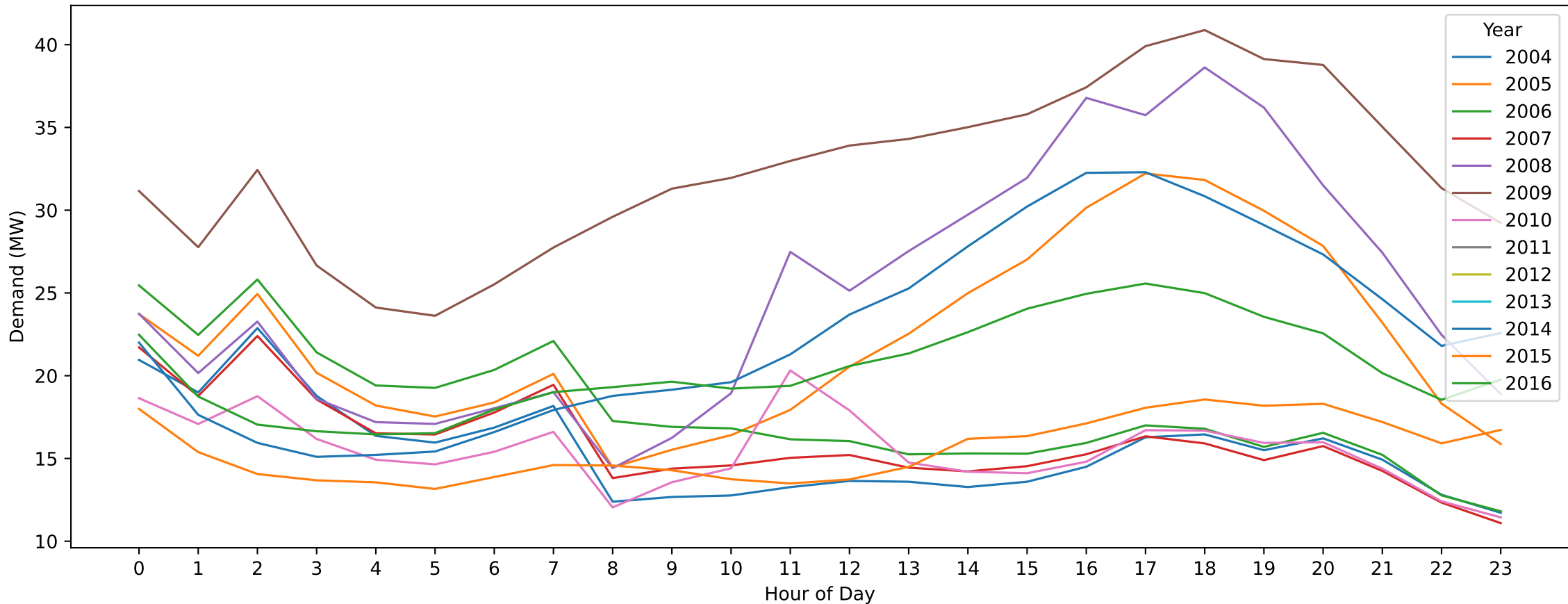
Eaglehawk — Labour Day (Hourly Demand Across Years)
