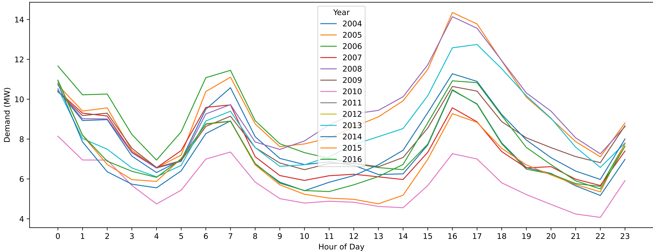
Cohuna — Labour Day (Hourly Demand Across Years)
