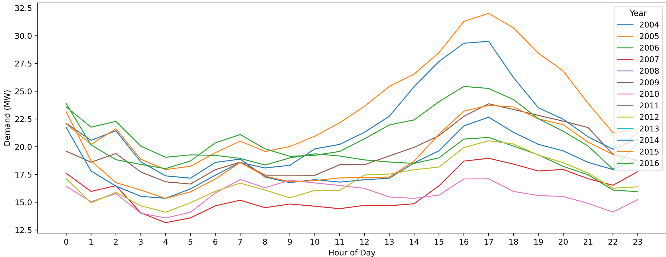
Mooroopna — Labour Day (Hourly Demand Across Years)
