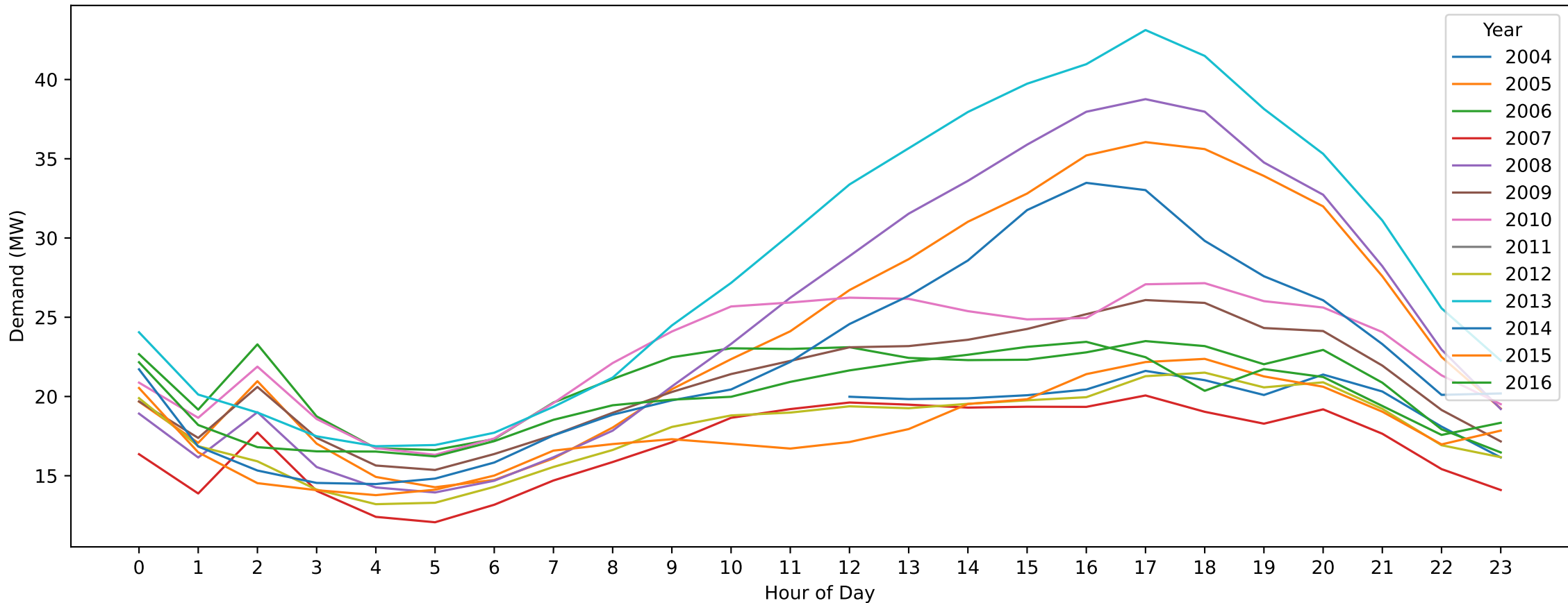
Bendigo — Labour Day (Hourly Demand Across Years)
