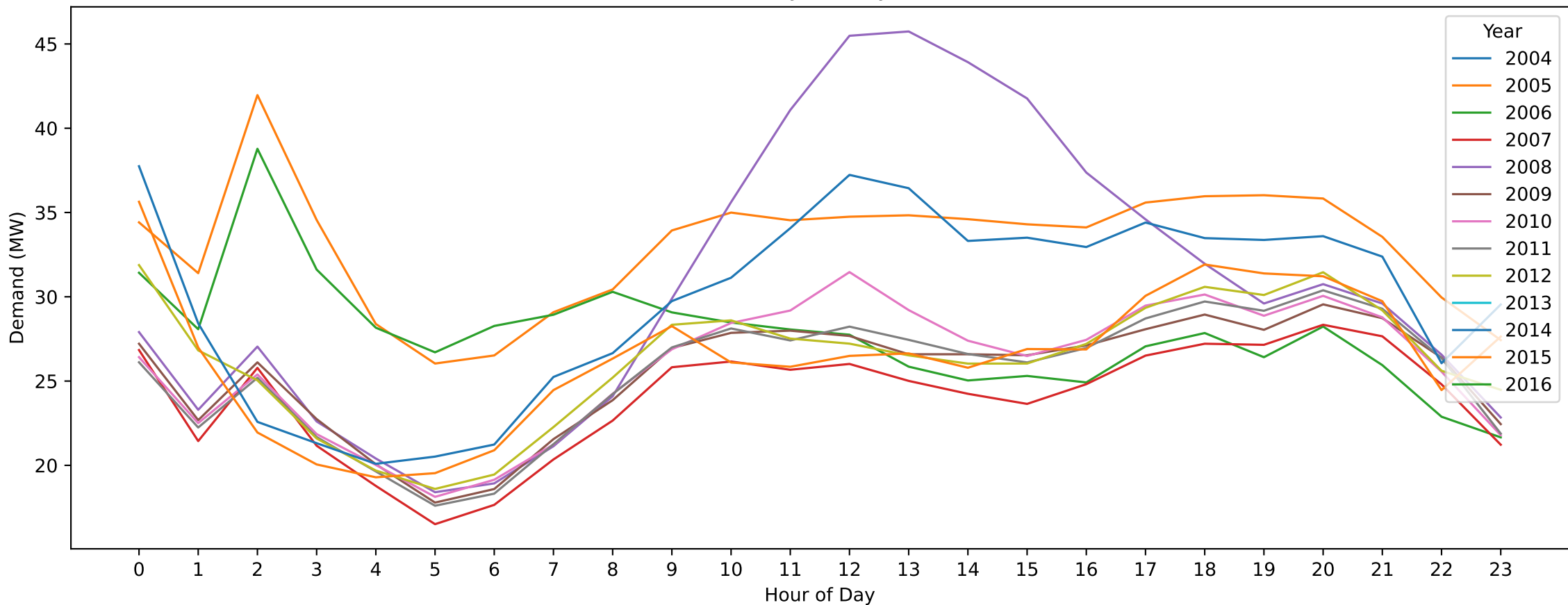
Waurn Ponds — Labour Day (Hourly Demand Across Years)
