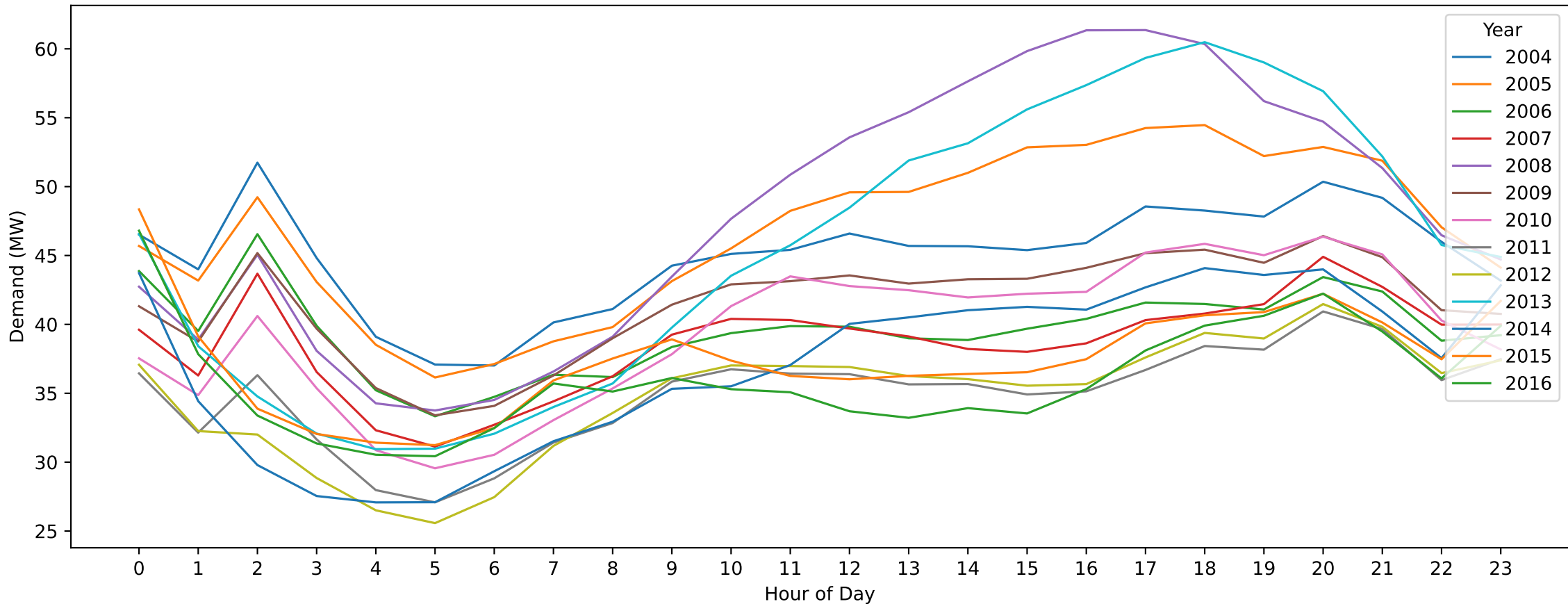
Ballarat North — Labour Day (Hourly Demand Across Years)
