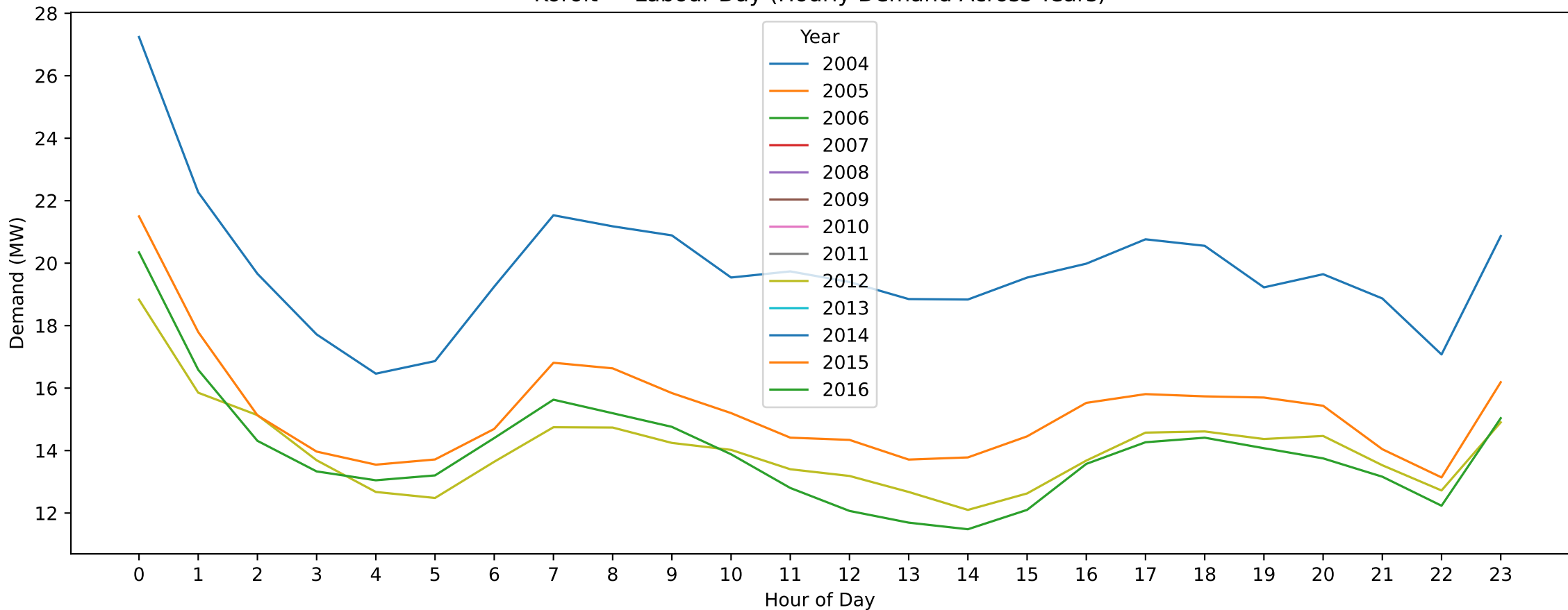
Koroit — Labour Day (Hourly Demand Across Years)
