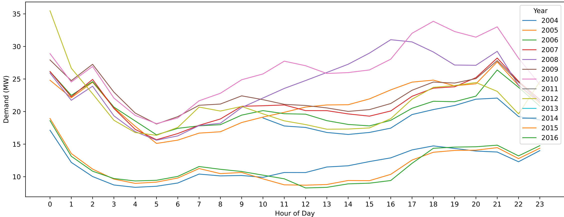
Woodend — Labour Day (Hourly Demand Across Years)
