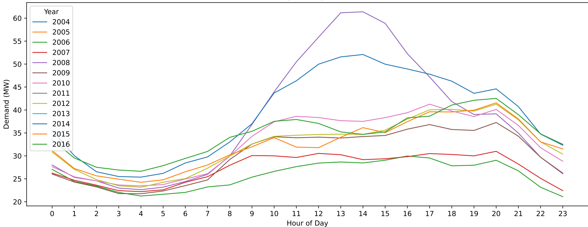
Werribee — Labour Day (Hourly Demand Across Years)
