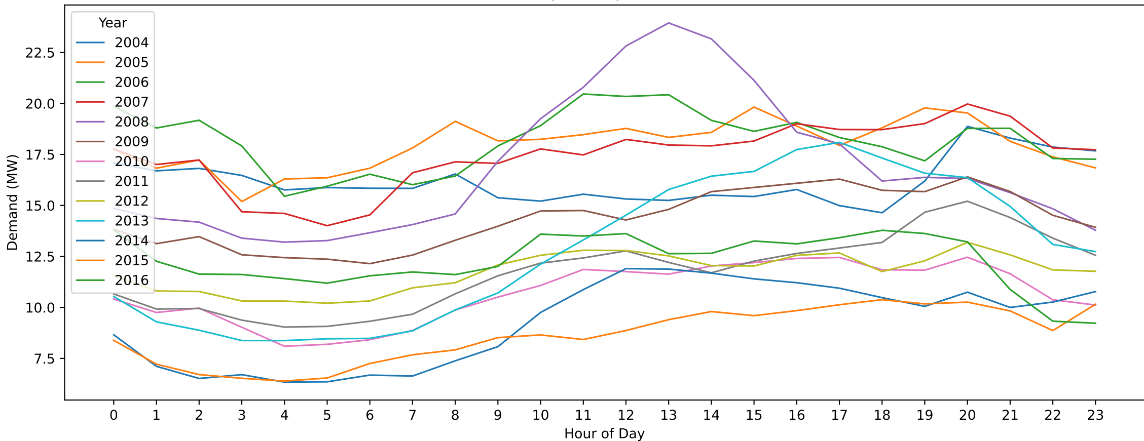
Corio — Labour Day (Hourly Demand Across Years)
