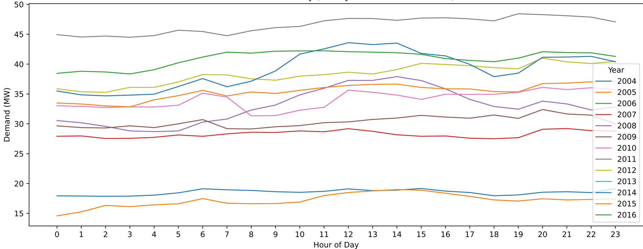
LVN22 — Labour Day (Hourly Demand Across Years)
