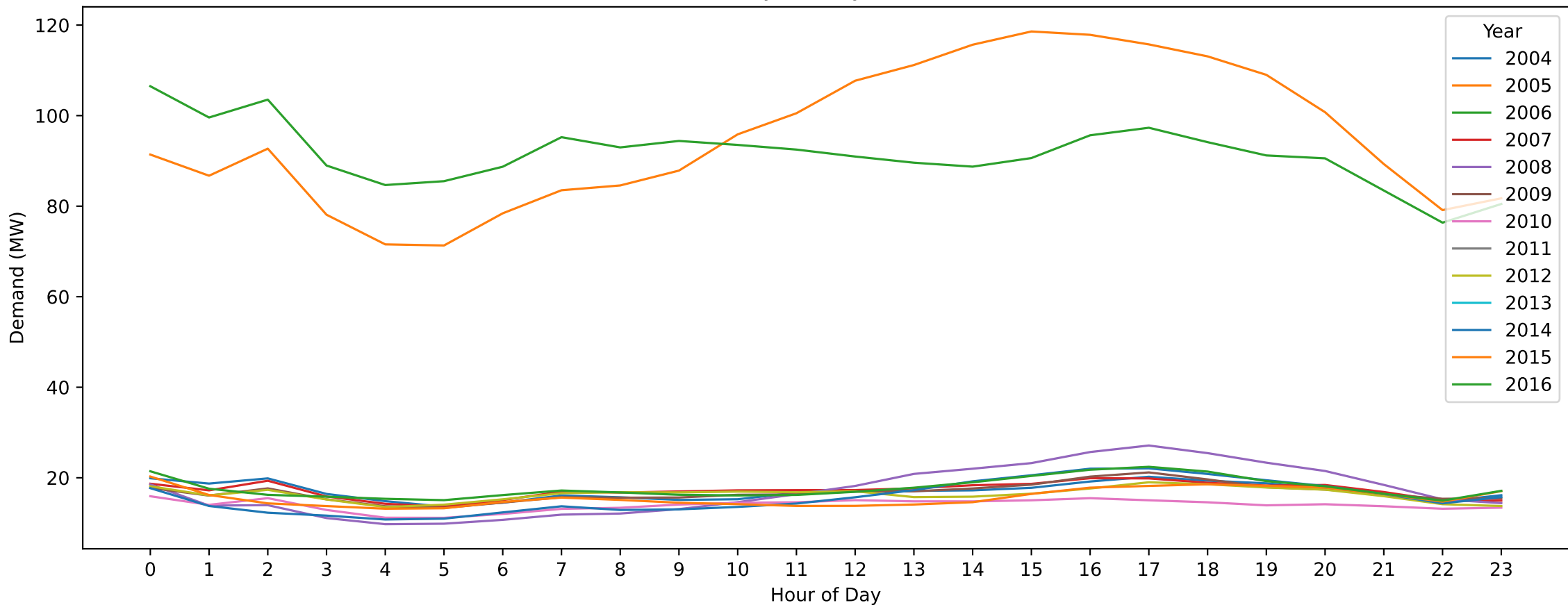
Echuca — Labour Day (Hourly Demand Across Years)
