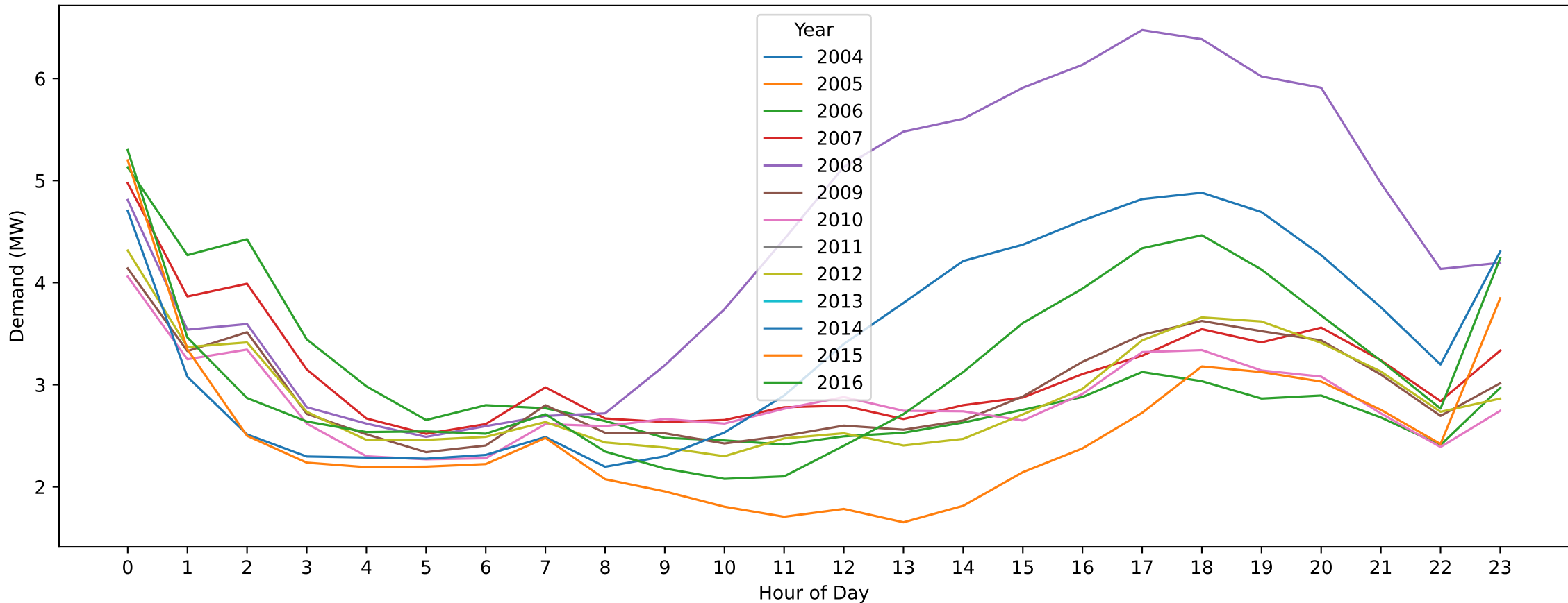
Ouyen — Labour Day (Hourly Demand Across Years)
