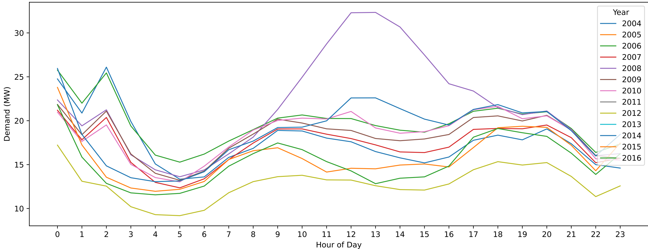
Drysdale — Labour Day (Hourly Demand Across Years)
