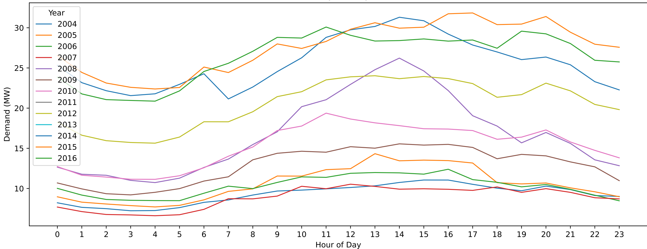
Sunshine East — Labour Day (Hourly Demand Across Years)
