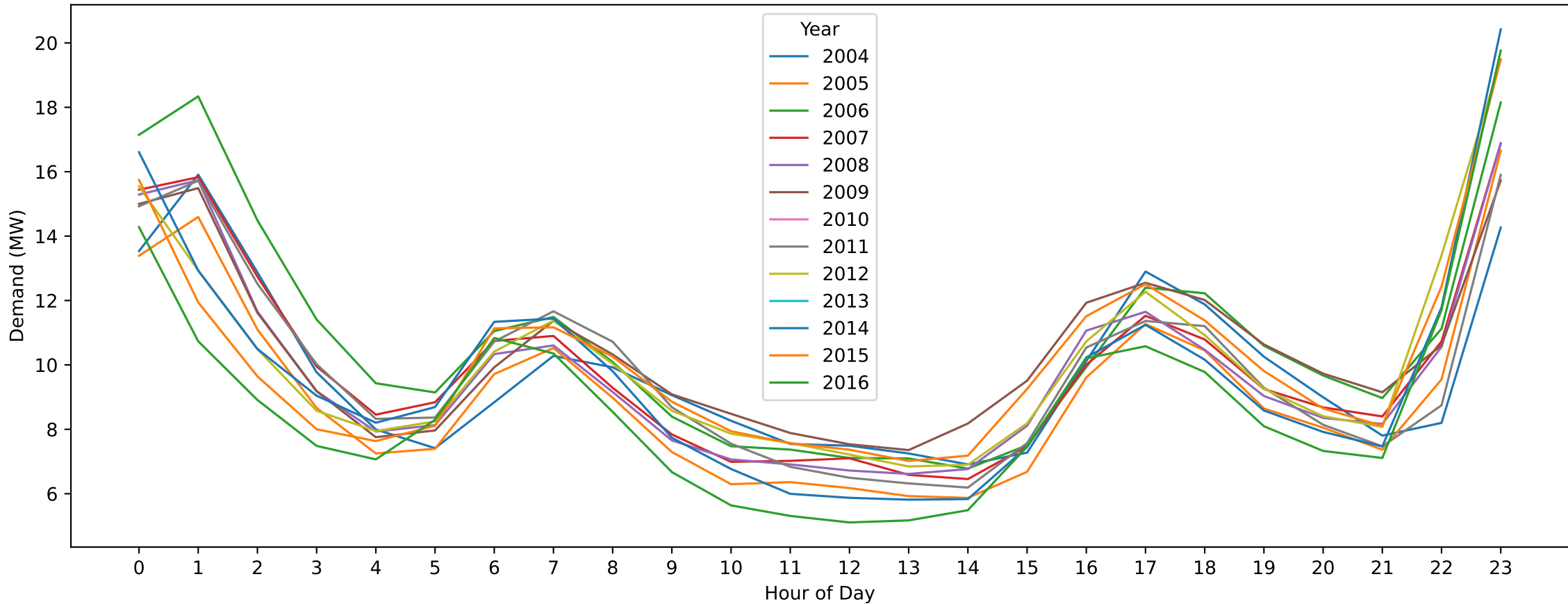
Terang — ANZAC Day (Hourly Demand Across Years)
