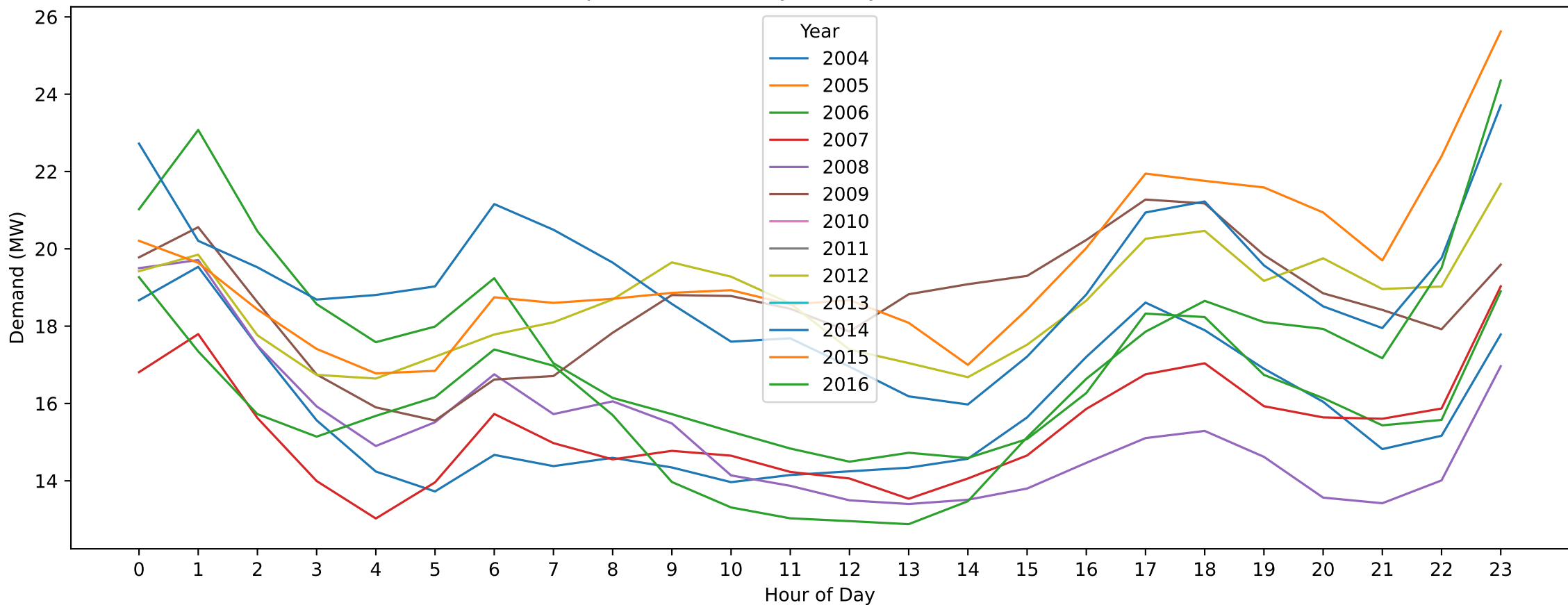
Mooroopna — ANZAC Day (Hourly Demand Across Years)
