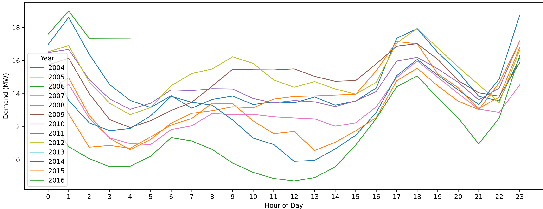
Shepparton Nth — ANZAC Day (Hourly Demand Across Years)
