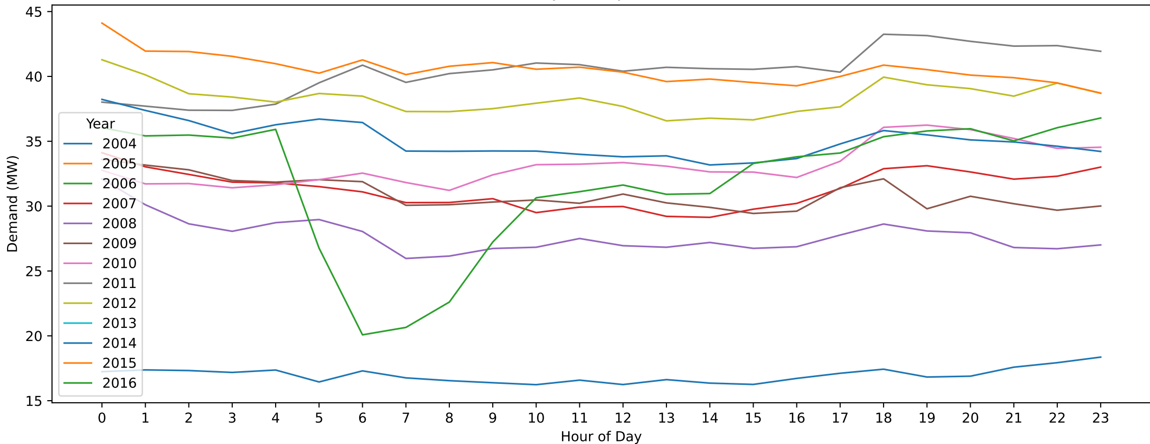
LVN22 — ANZAC Day (Hourly Demand Across Years)
