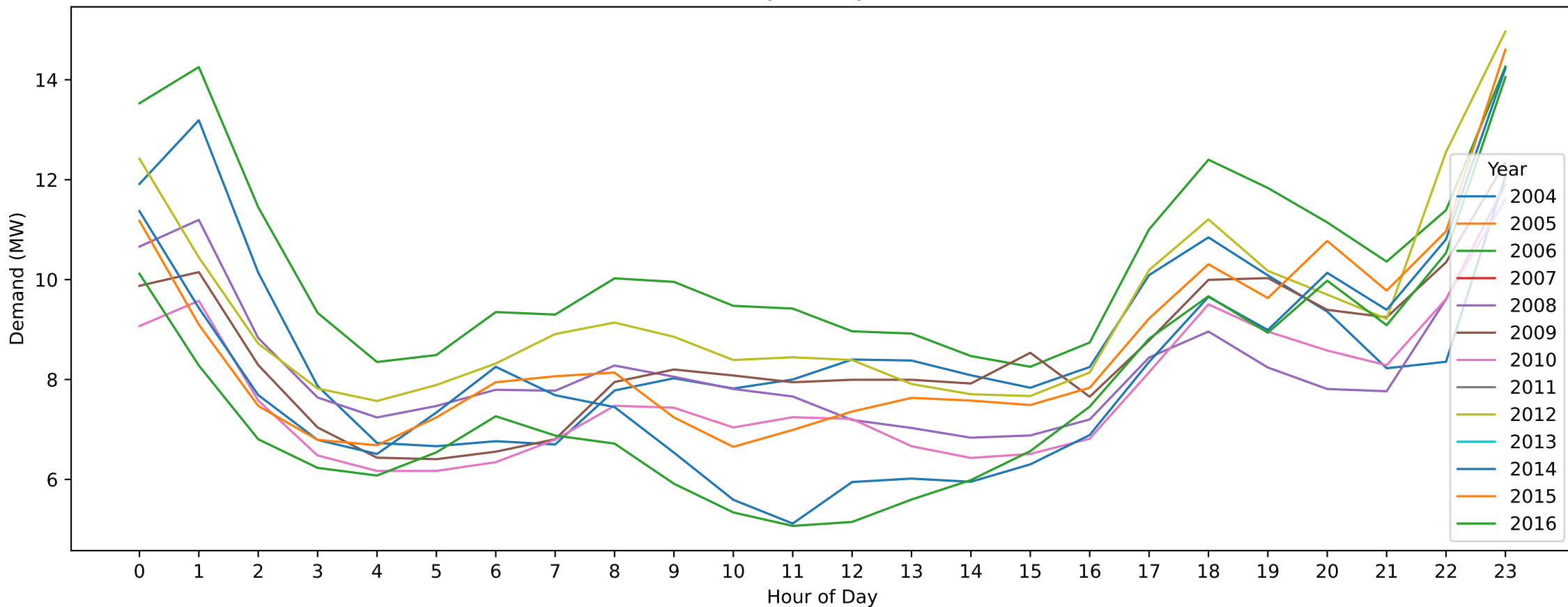
Charlton — ANZAC Day (Hourly Demand Across Years)
