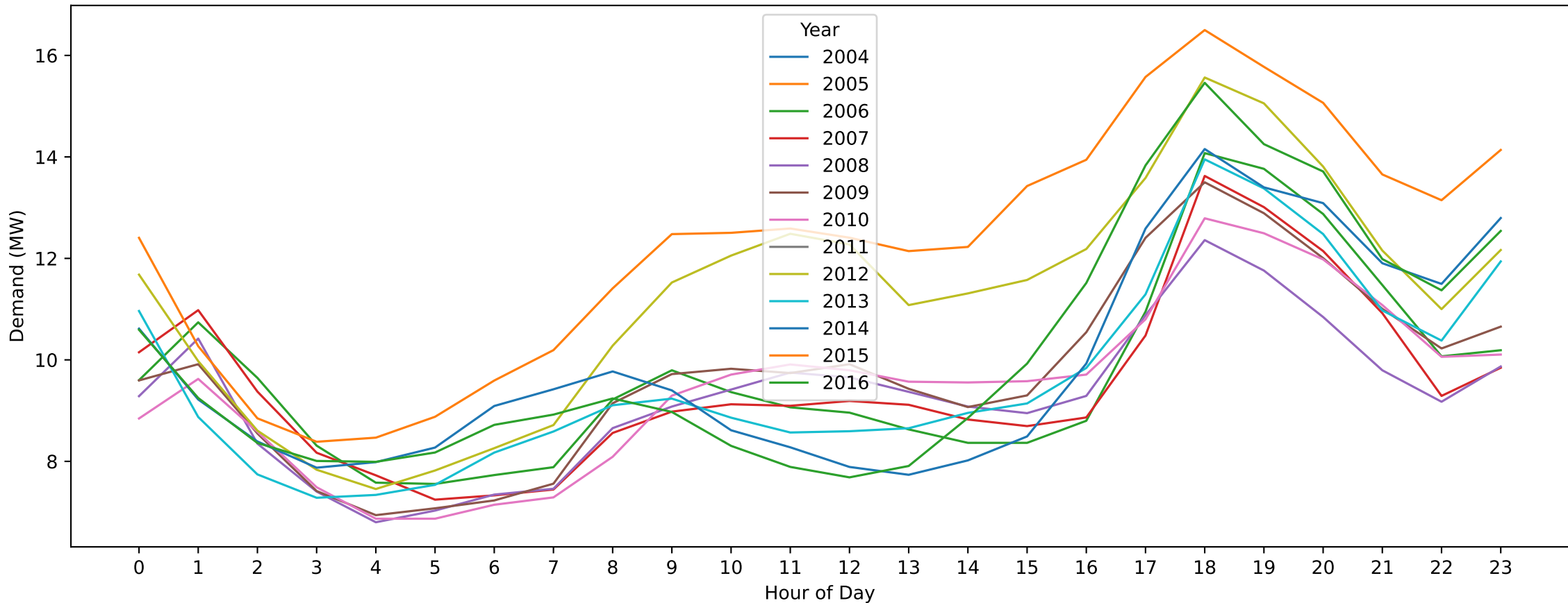
Bacchus Marsh — ANZAC Day (Hourly Demand Across Years)
