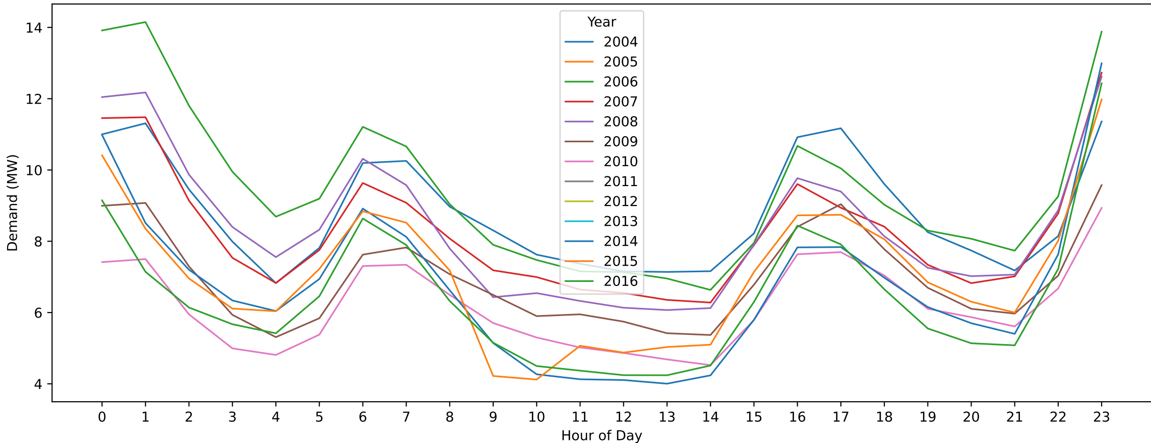
Cohuna — ANZAC Day (Hourly Demand Across Years)
