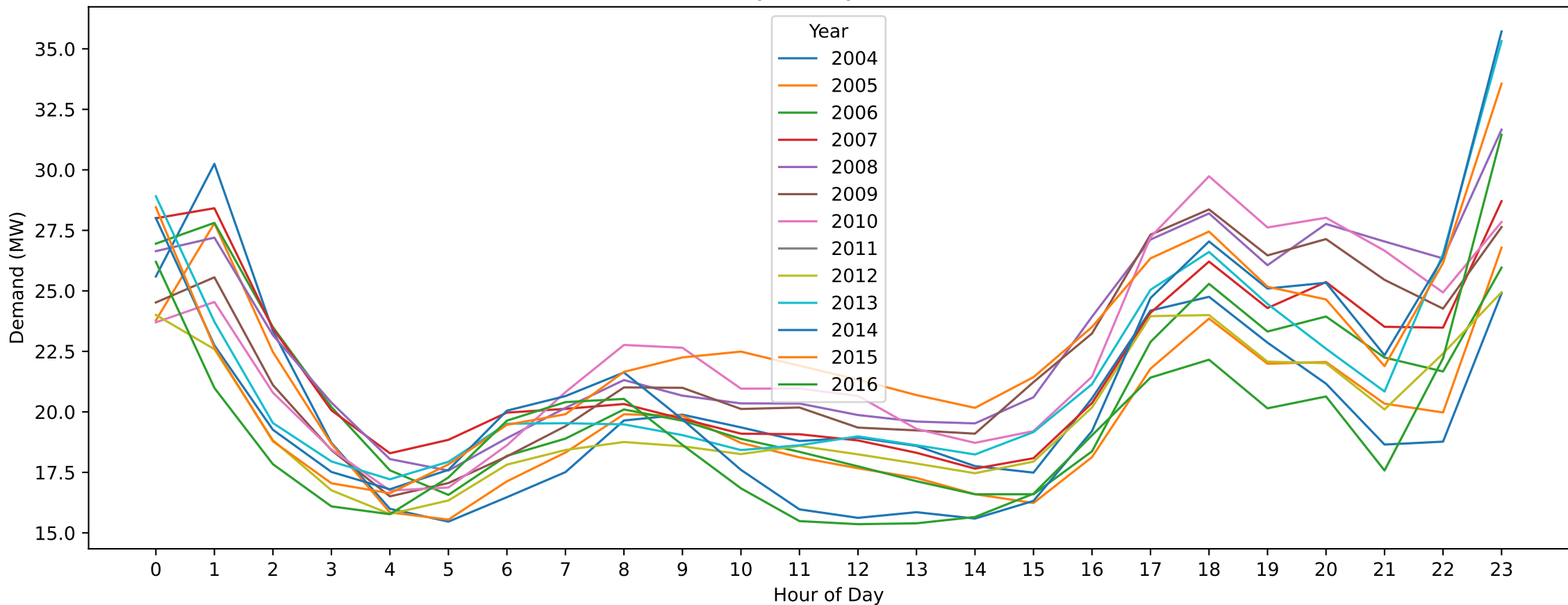
Colac — ANZAC Day (Hourly Demand Across Years)
