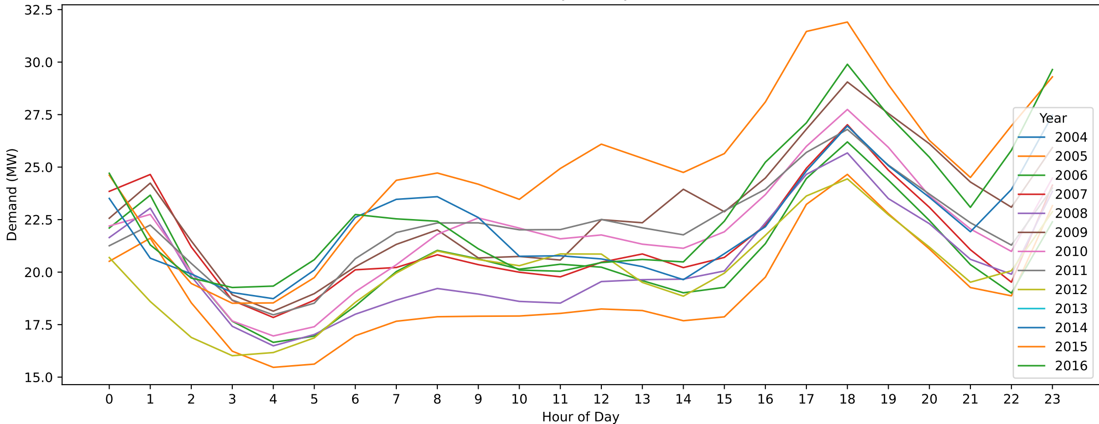
Warrnambool — ANZAC Day (Hourly Demand Across Years)
