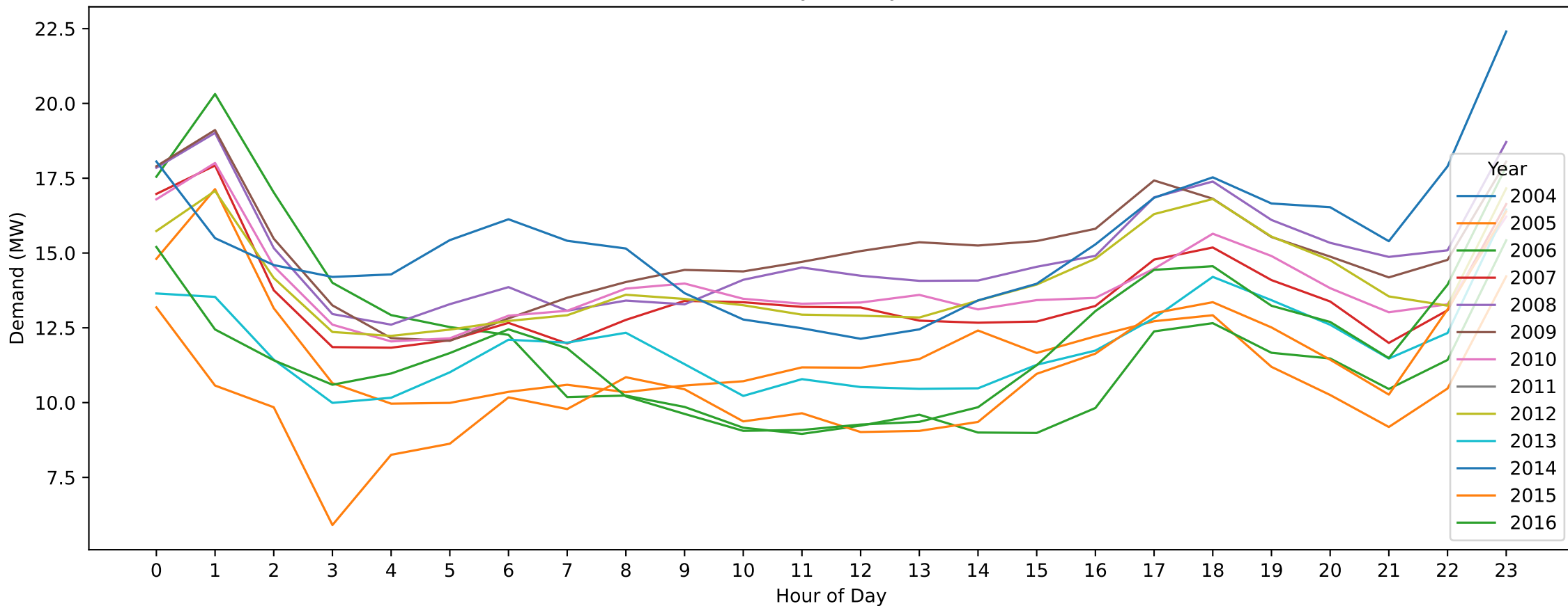
Cobram East — ANZAC Day (Hourly Demand Across Years)
