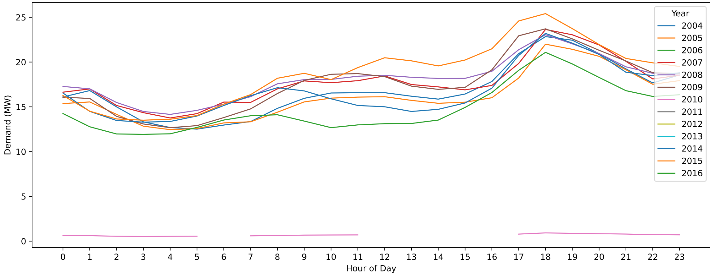
Geelong East — ANZAC Day (Hourly Demand Across Years)
