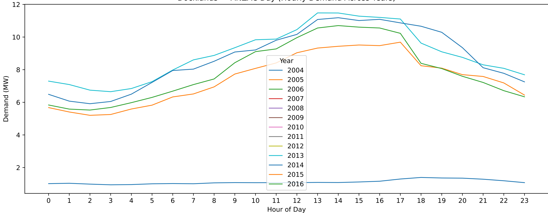
Docklands — ANZAC Day (Hourly Demand Across Years)
