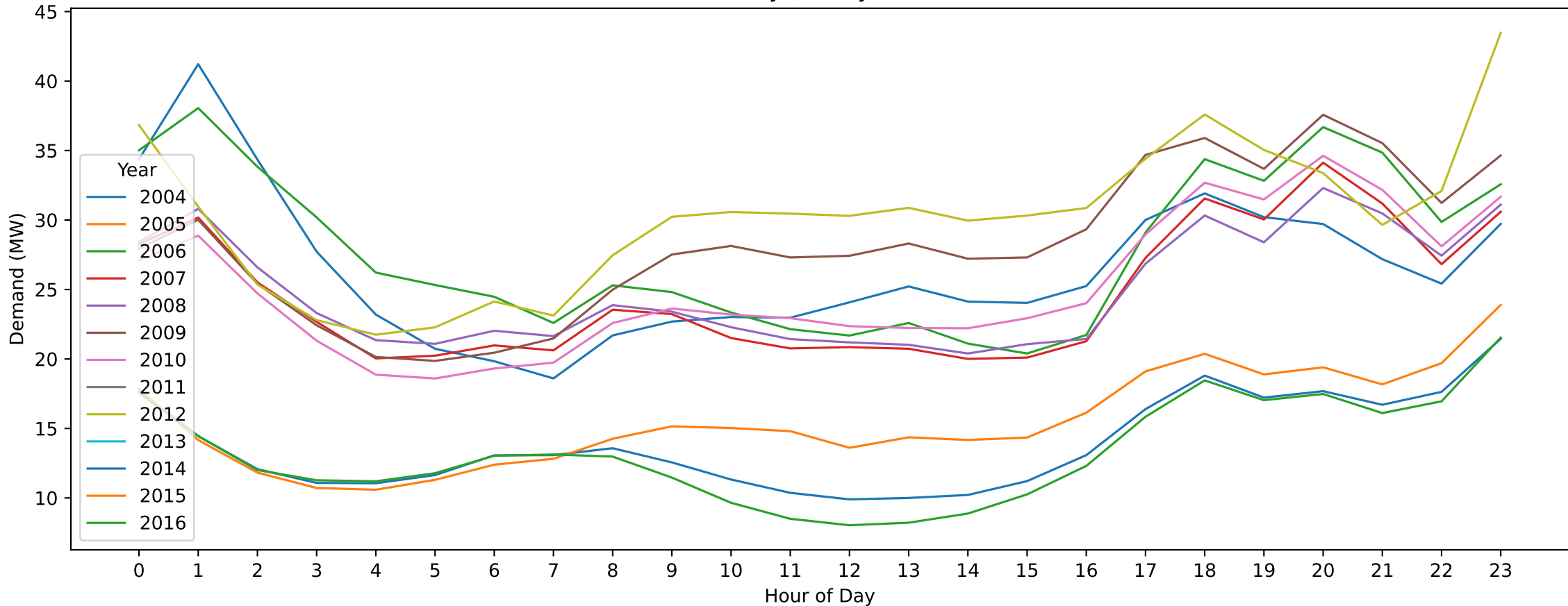
Woodend — ANZAC Day (Hourly Demand Across Years)
