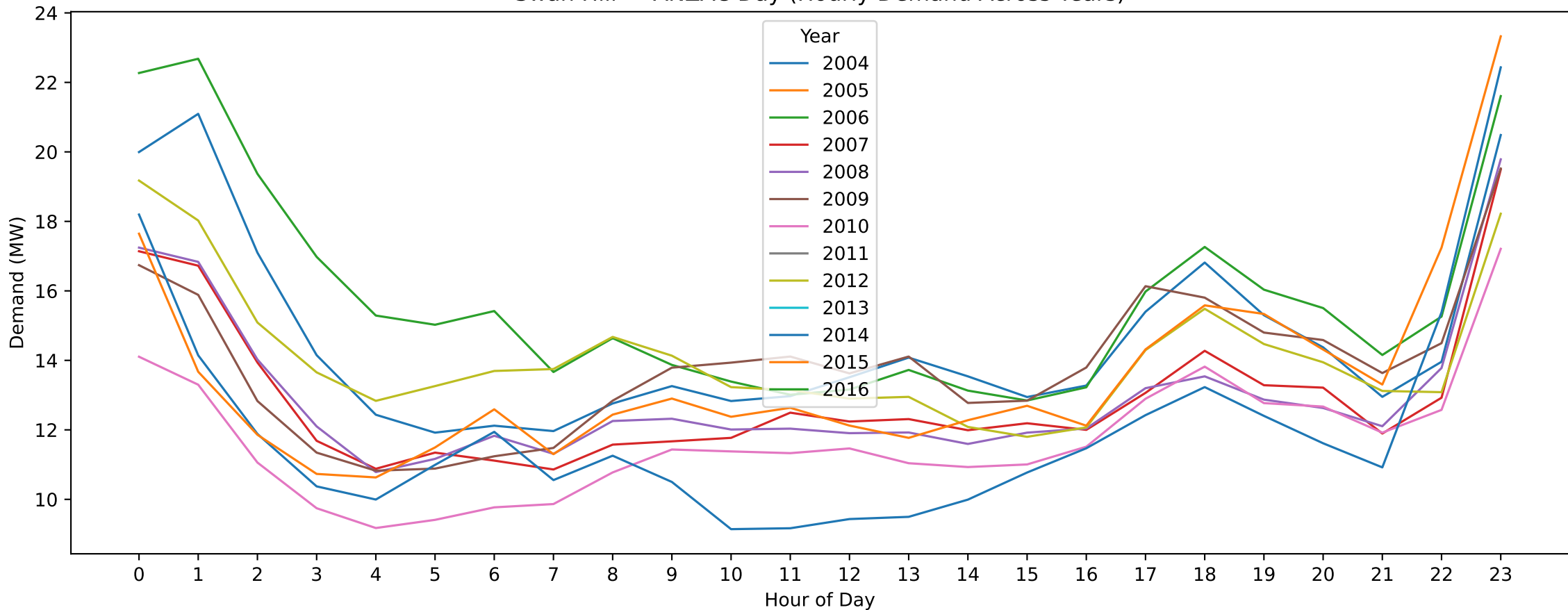
Swan Hill — ANZAC Day (Hourly Demand Across Years)
