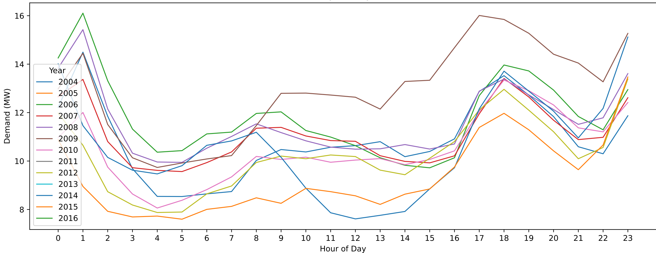
Castlemaine — ANZAC Day (Hourly Demand Across Years)
