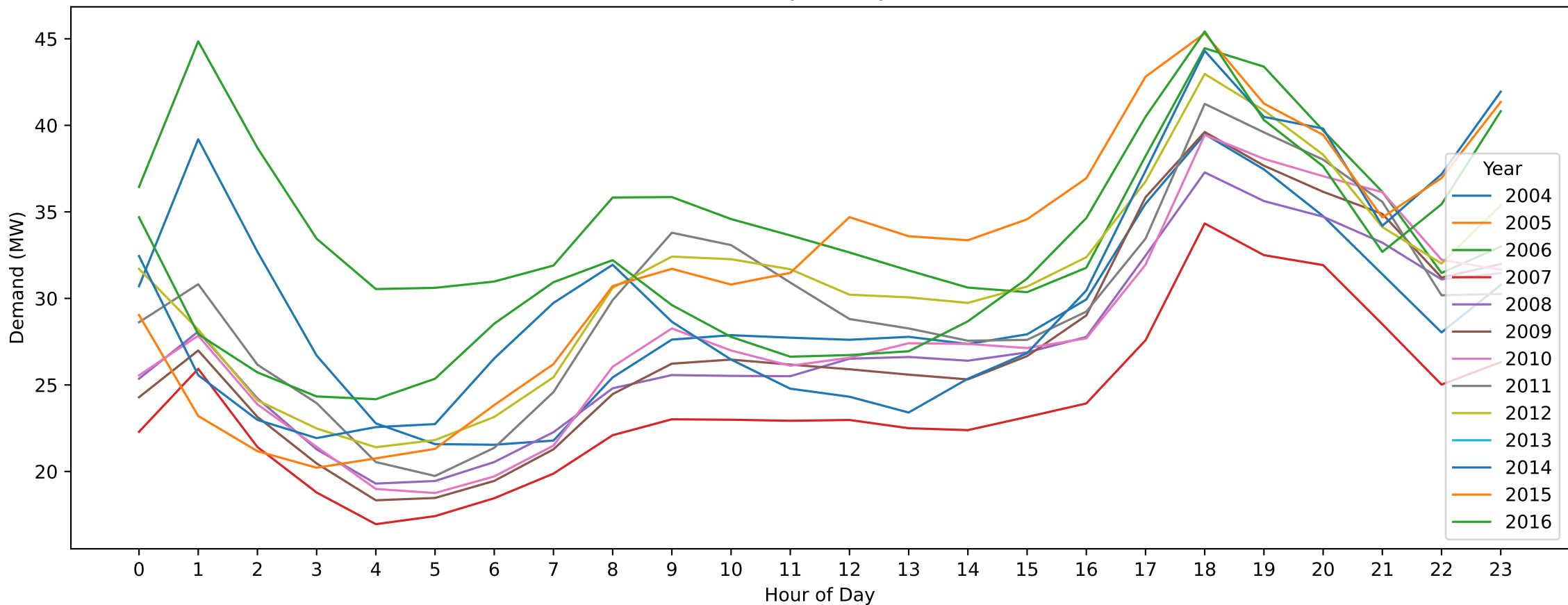
Waurn Ponds — ANZAC Day (Hourly Demand Across Years)
