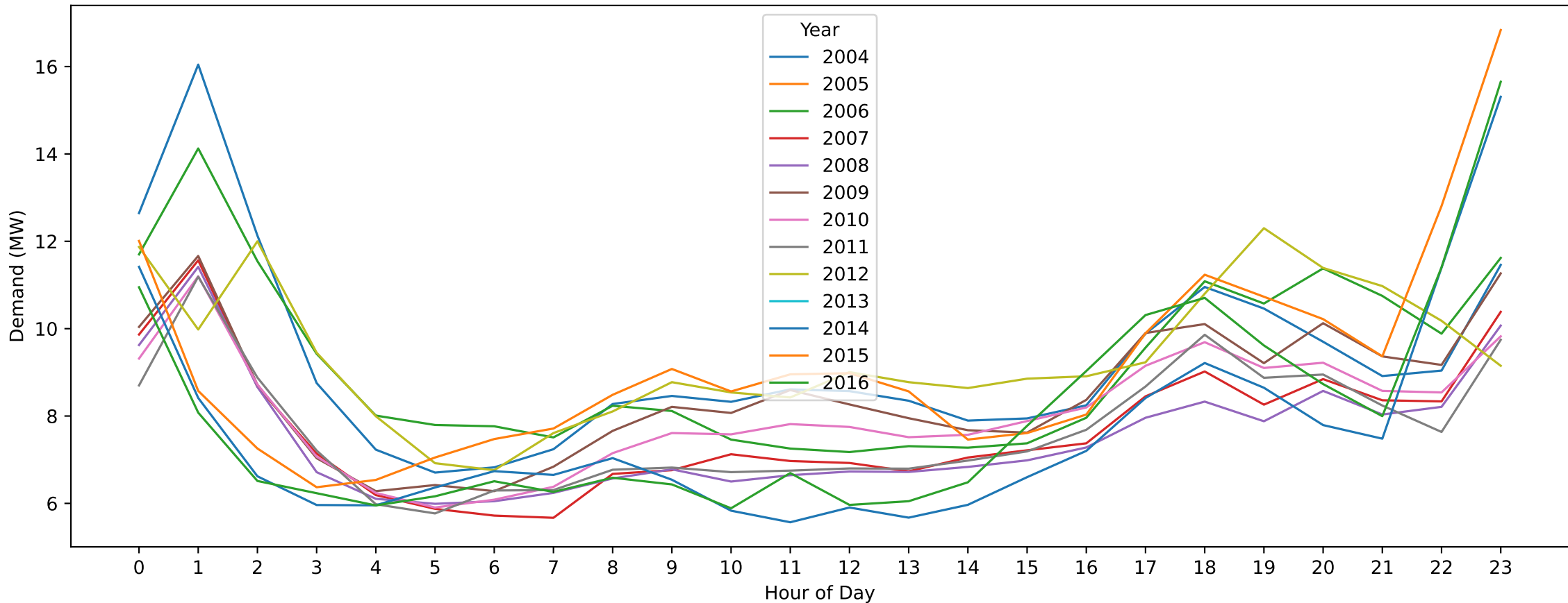
Merbein — ANZAC Day (Hourly Demand Across Years)
