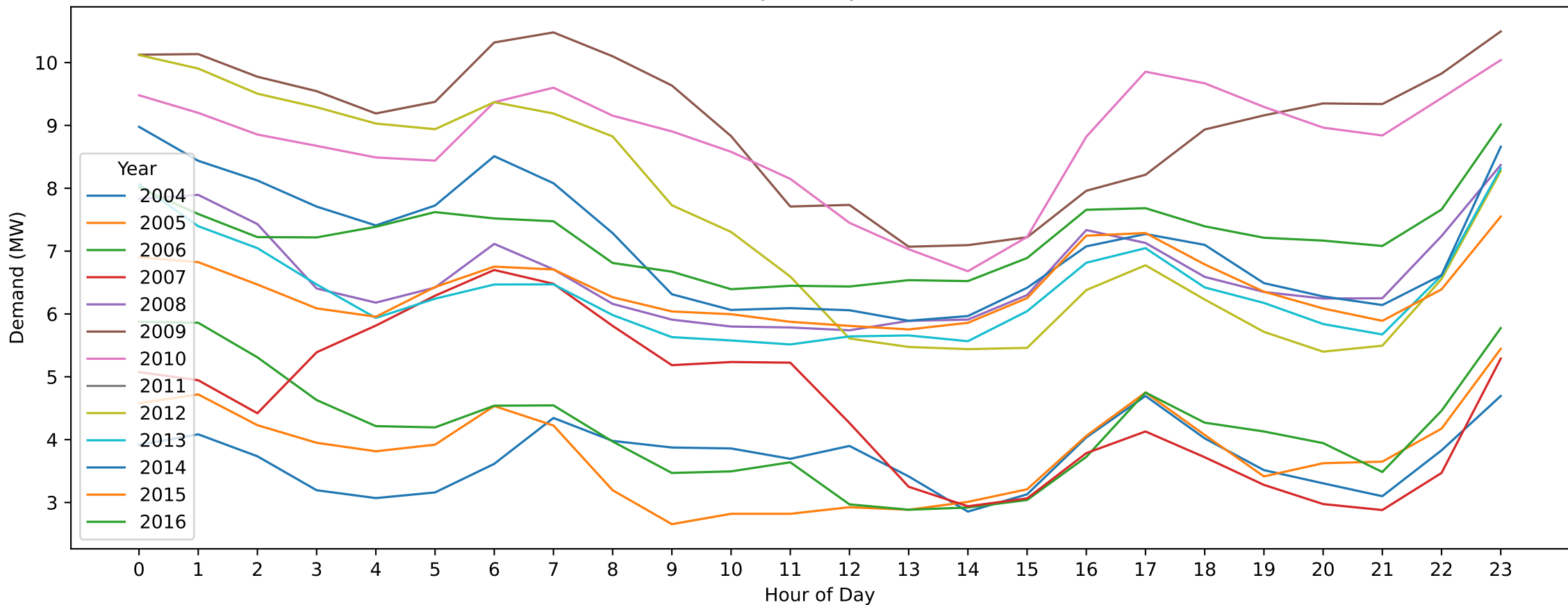
Cobden — ANZAC Day (Hourly Demand Across Years)
