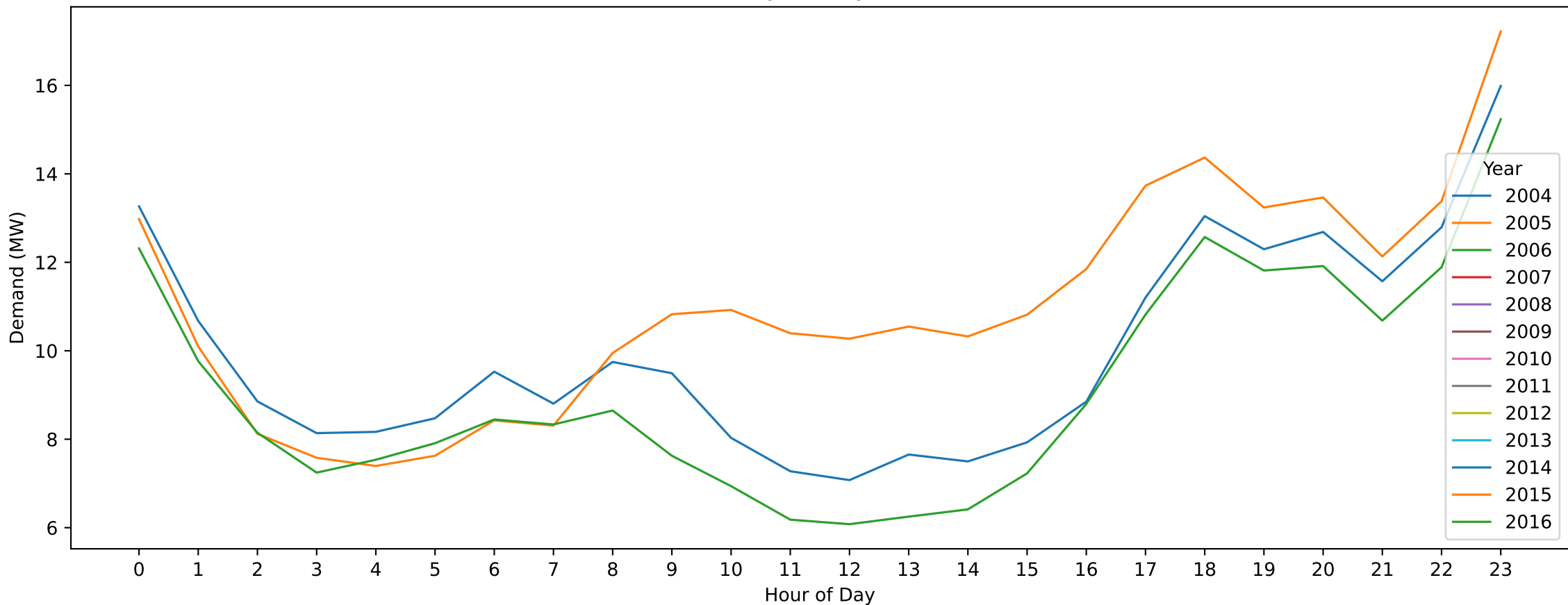
Gisborne — ANZAC Day (Hourly Demand Across Years)
