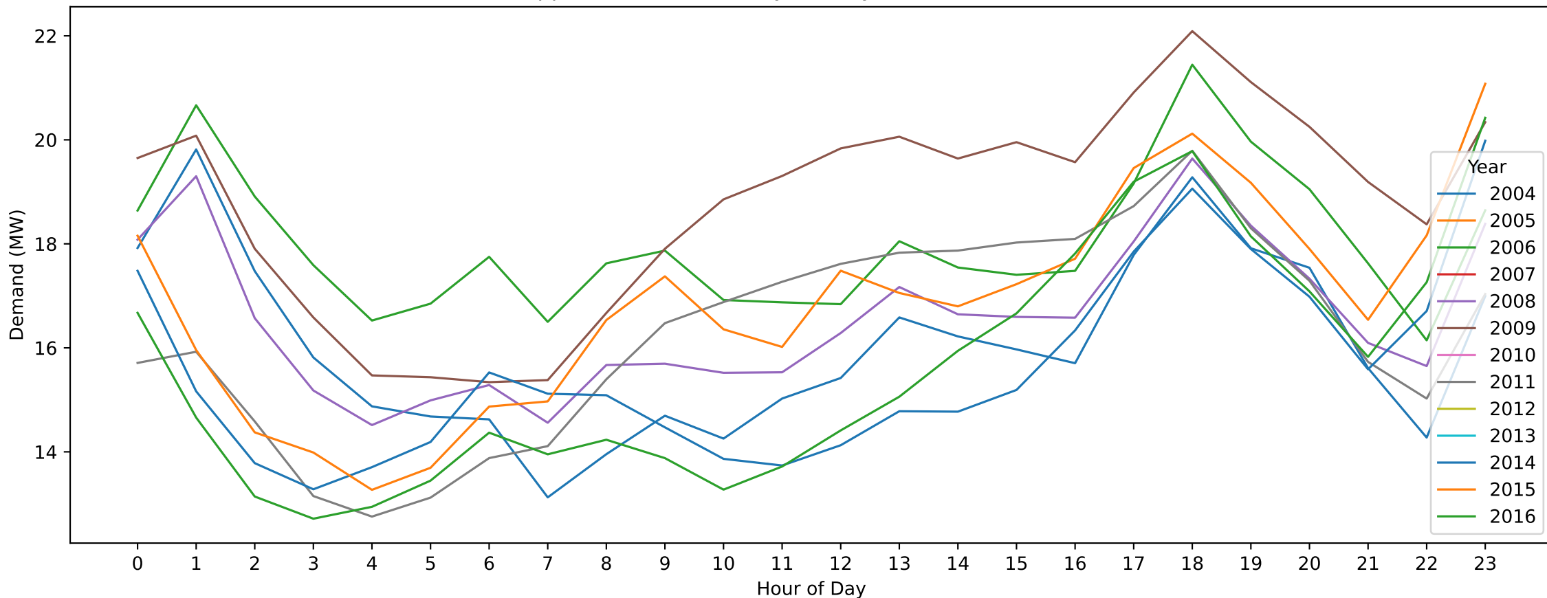
Shepparton — ANZAC Day (Hourly Demand Across Years)
