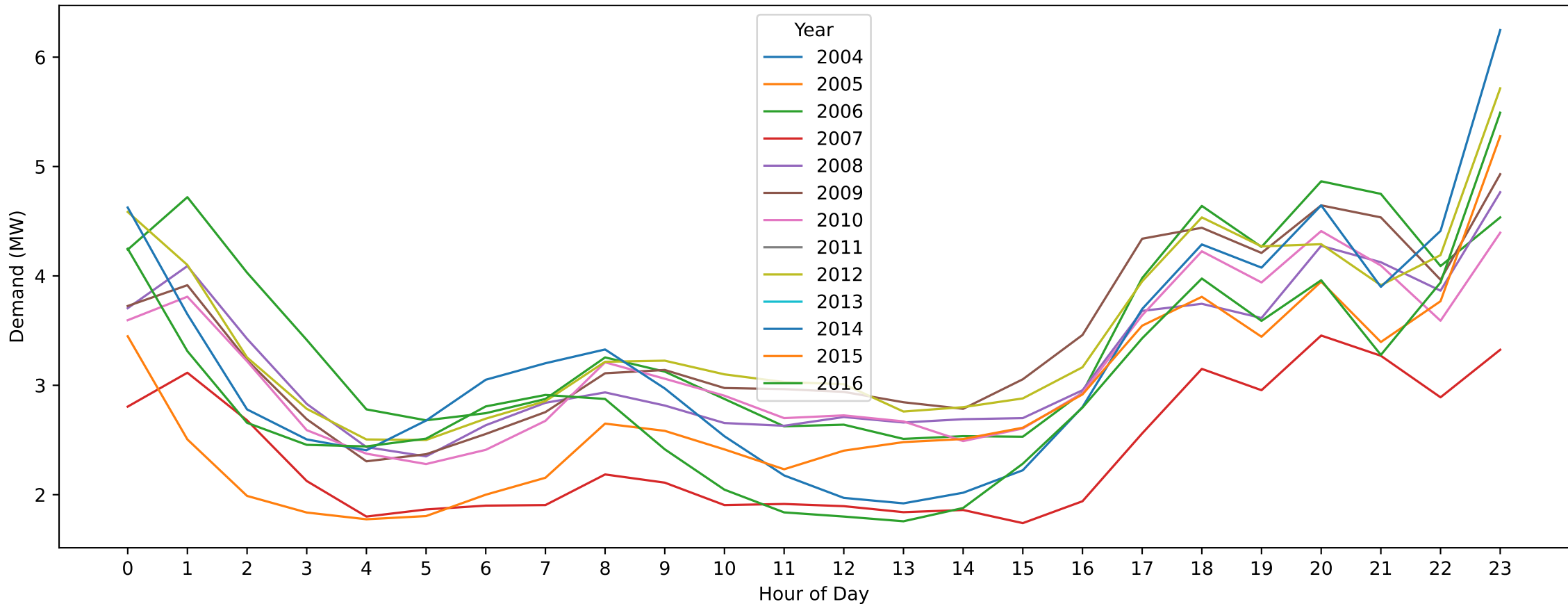
Winchelsea — ANZAC Day (Hourly Demand Across Years)
