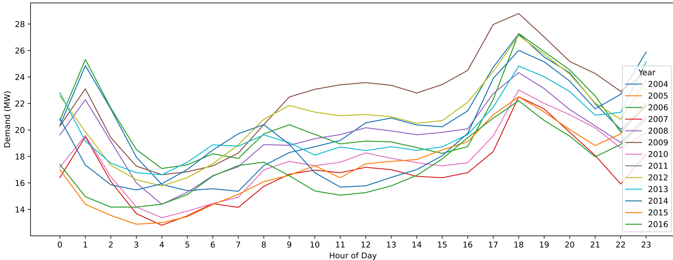
Bendigo — ANZAC Day (Hourly Demand Across Years)
