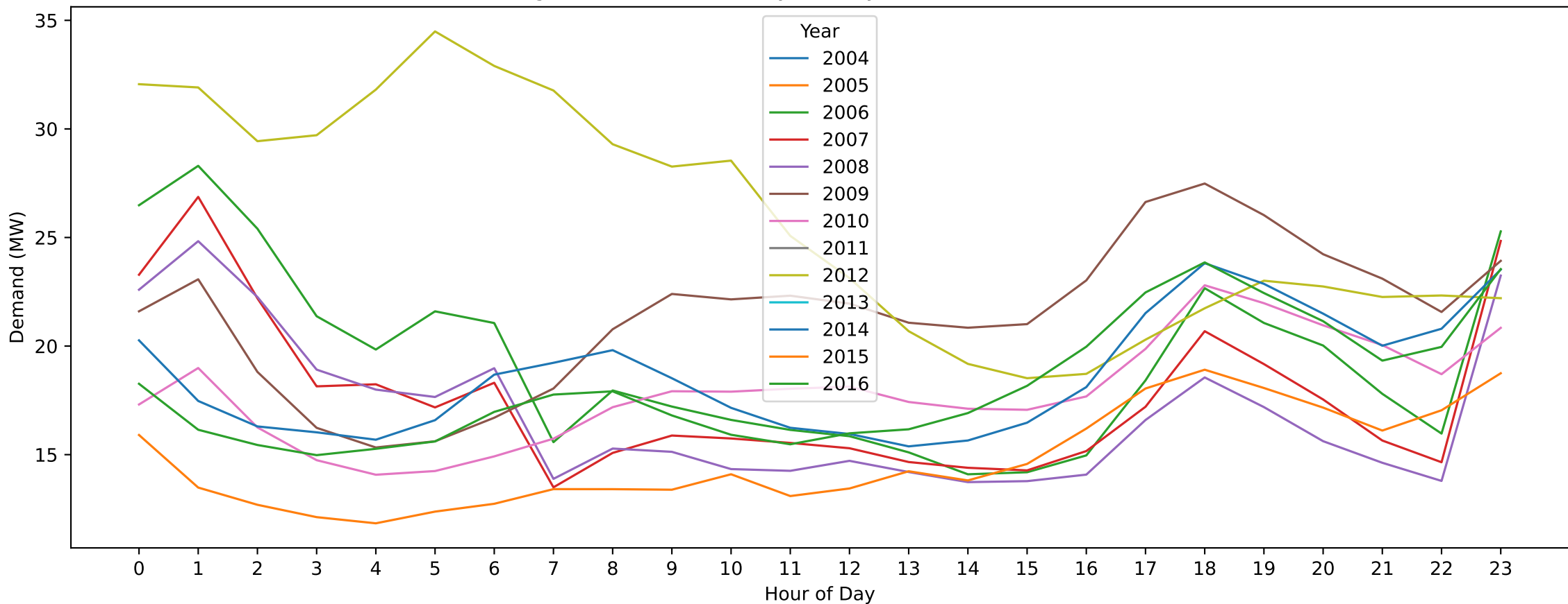
Eaglehawk — ANZAC Day (Hourly Demand Across Years)
