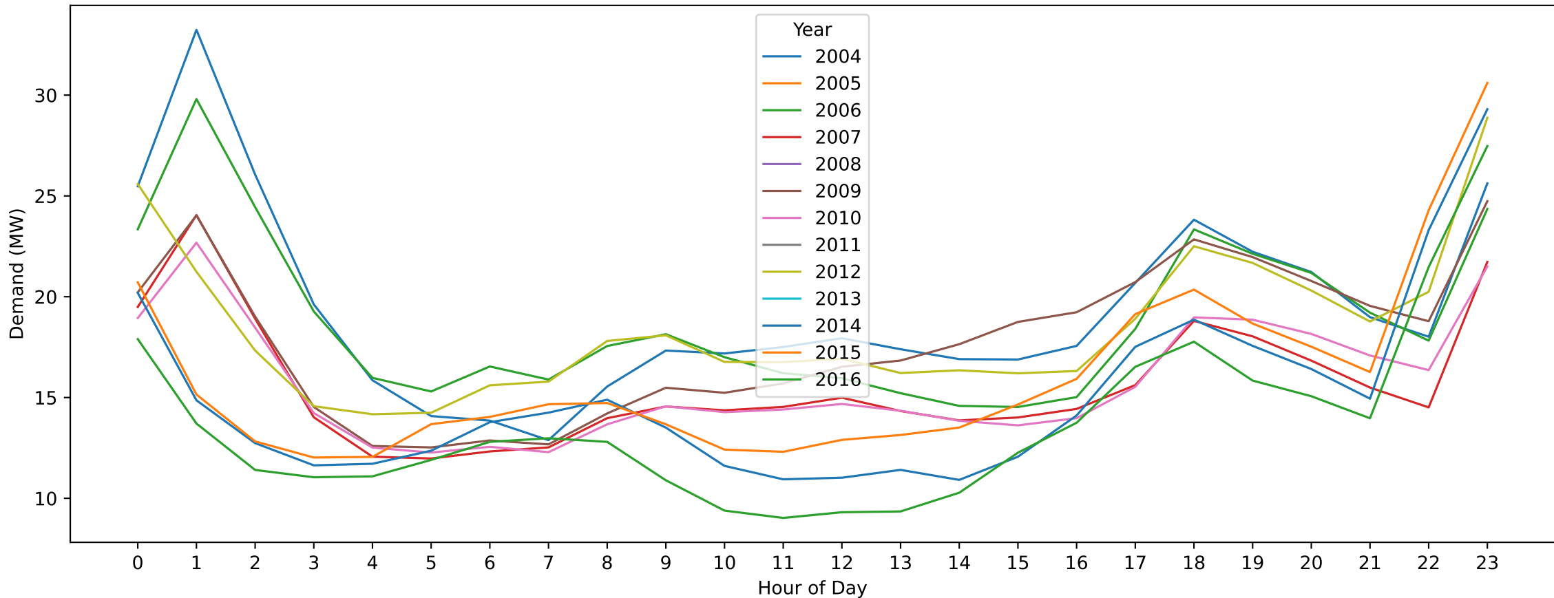
Horsham — ANZAC Day (Hourly Demand Across Years)
