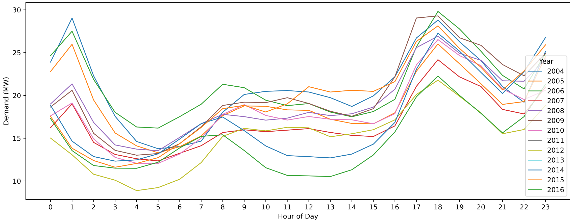
Drysdale — ANZAC Day (Hourly Demand Across Years)
