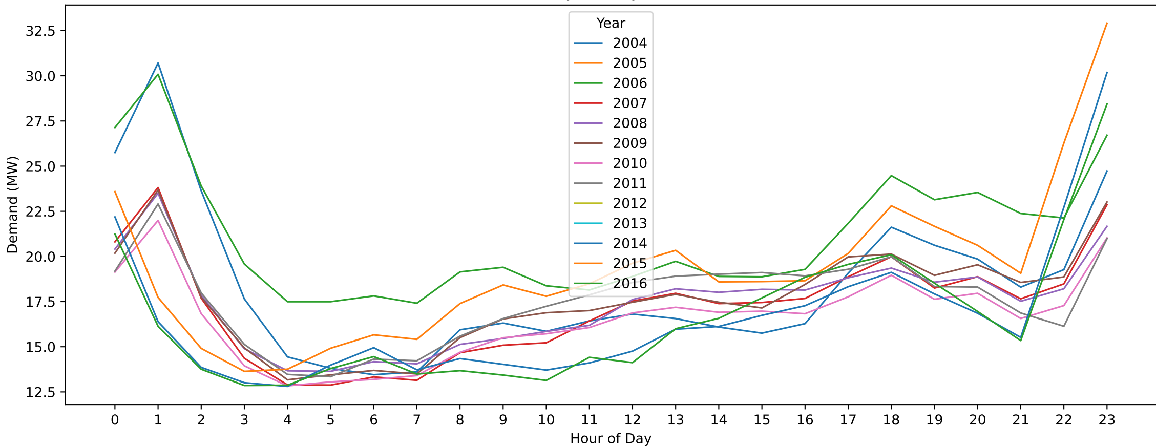
Mildura — ANZAC Day (Hourly Demand Across Years)
