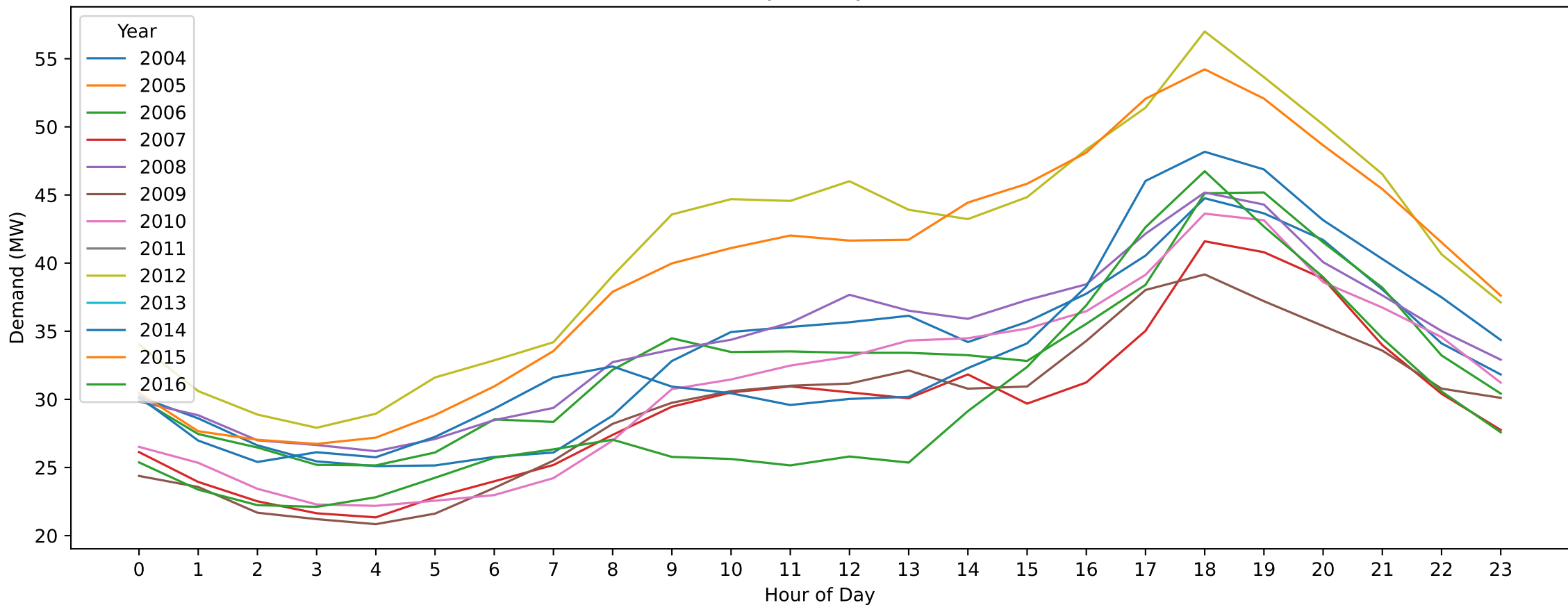
Laverton — ANZAC Day (Hourly Demand Across Years)
