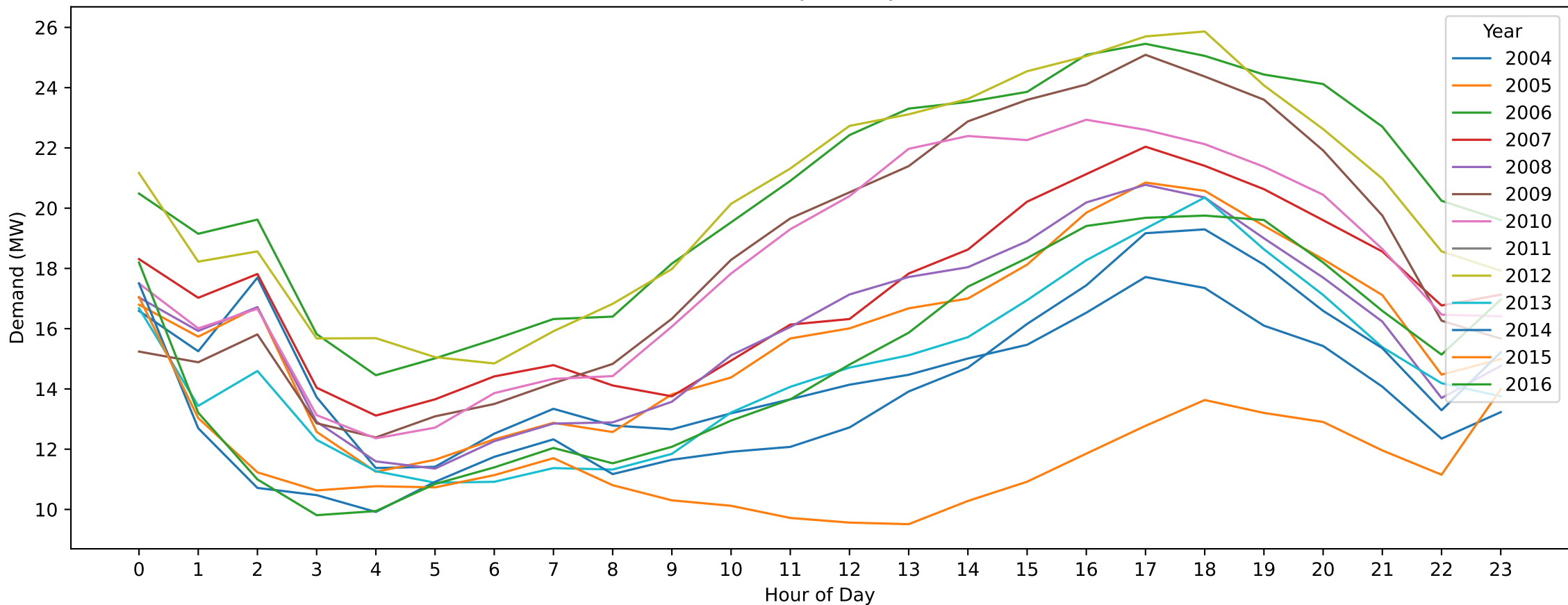
Cobram East — Australia Day (Hourly Demand Across Years)
