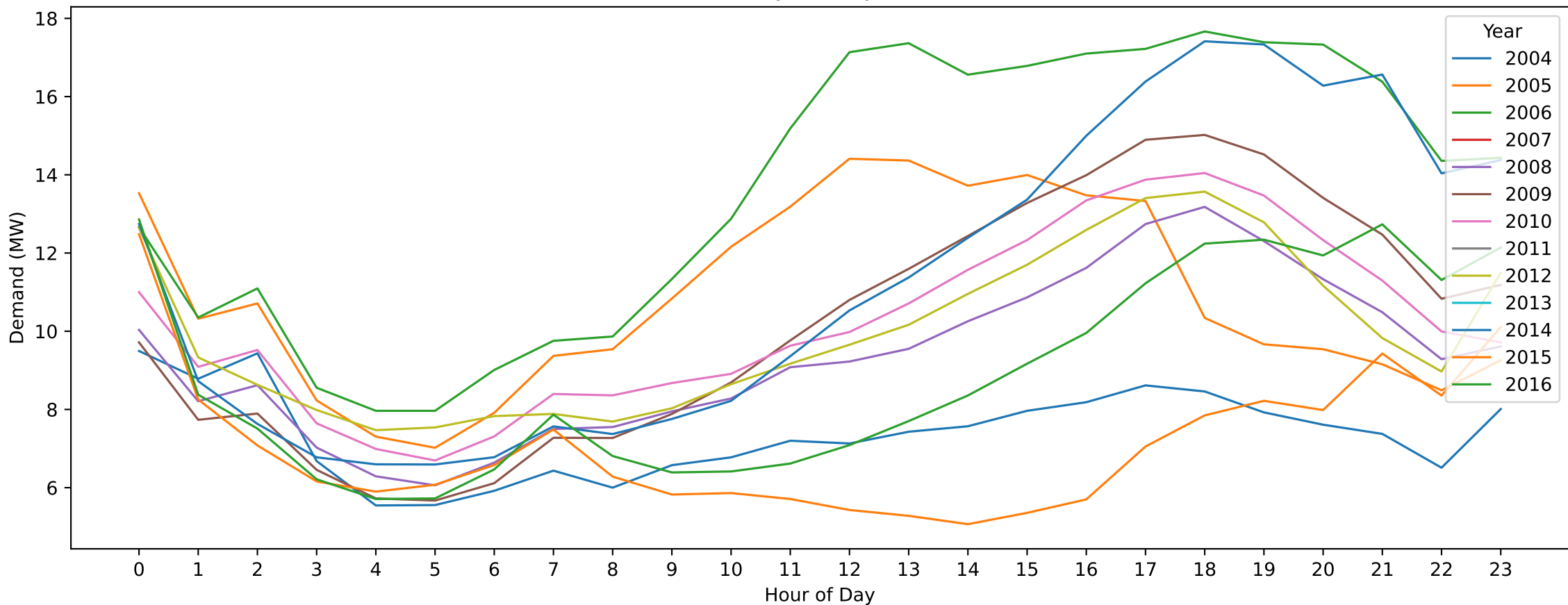
Charlton — Australia Day (Hourly Demand Across Years)
