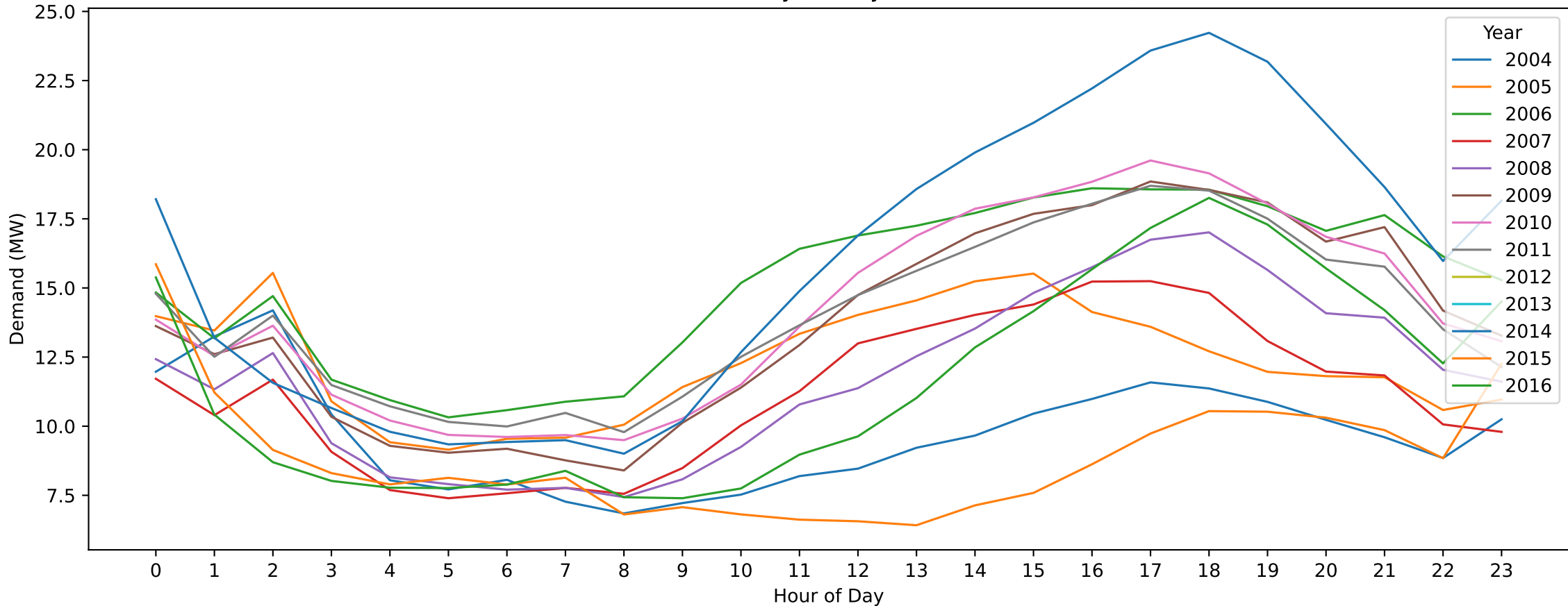
Merbein — Australia Day (Hourly Demand Across Years)
