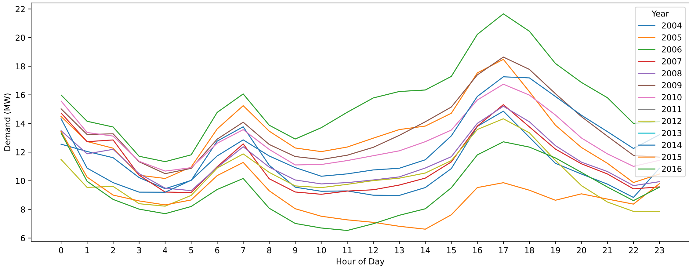
Stanhope — Australia Day (Hourly Demand Across Years)
