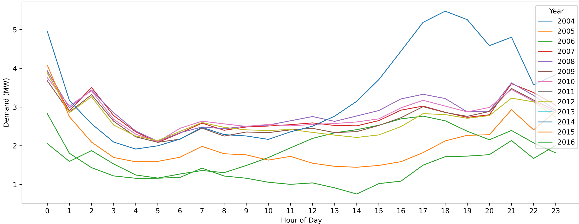
Winchelsea — Australia Day (Hourly Demand Across Years)
