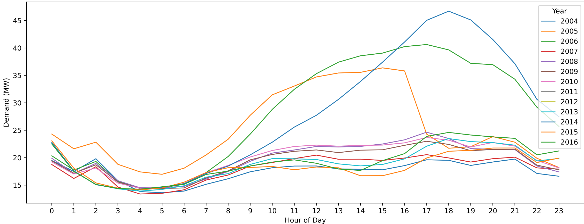
Geelong — Australia Day (Hourly Demand Across Years)
