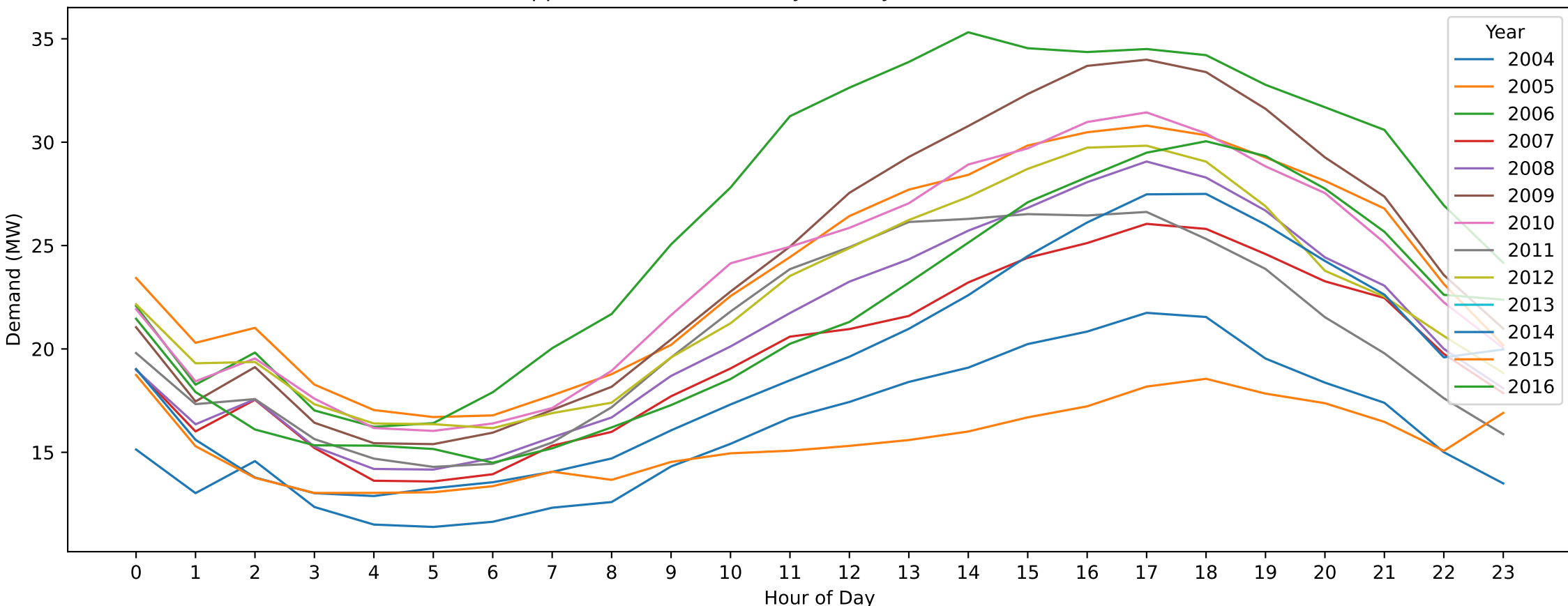
Shepparton — Australia Day (Hourly Demand Across Years)
