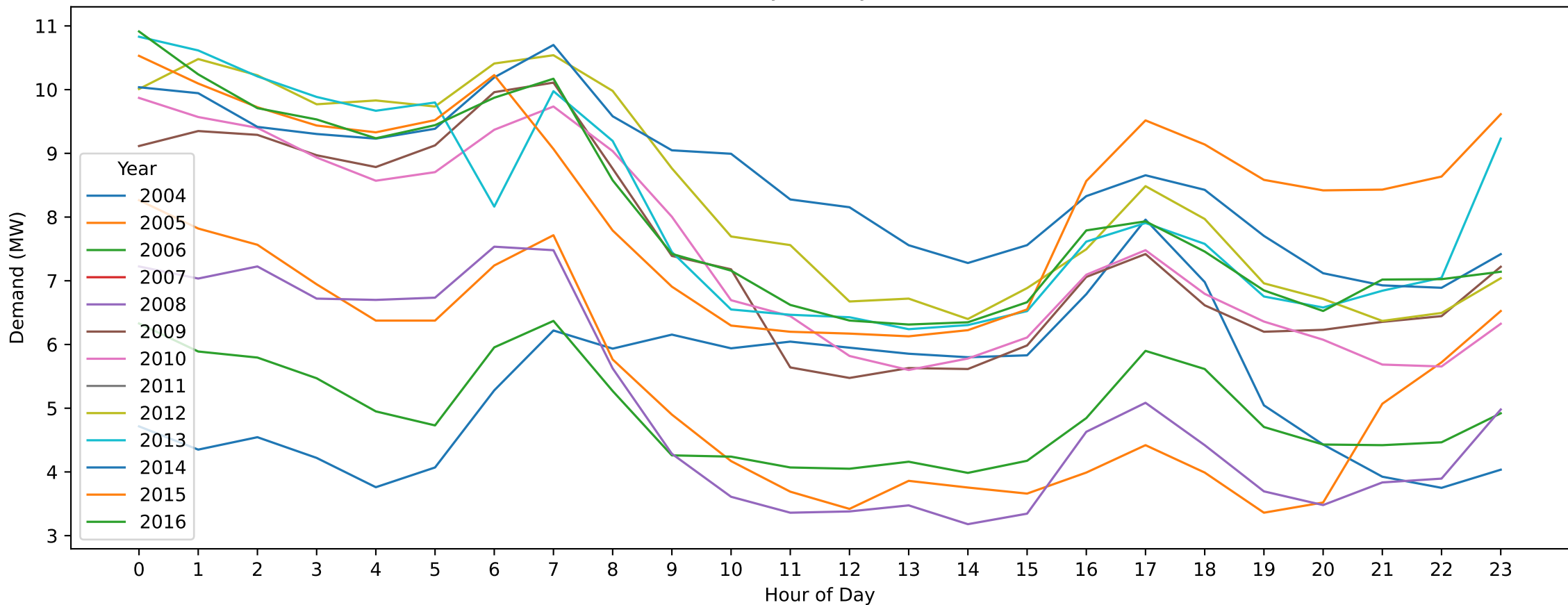
Cobden — Australia Day (Hourly Demand Across Years)
