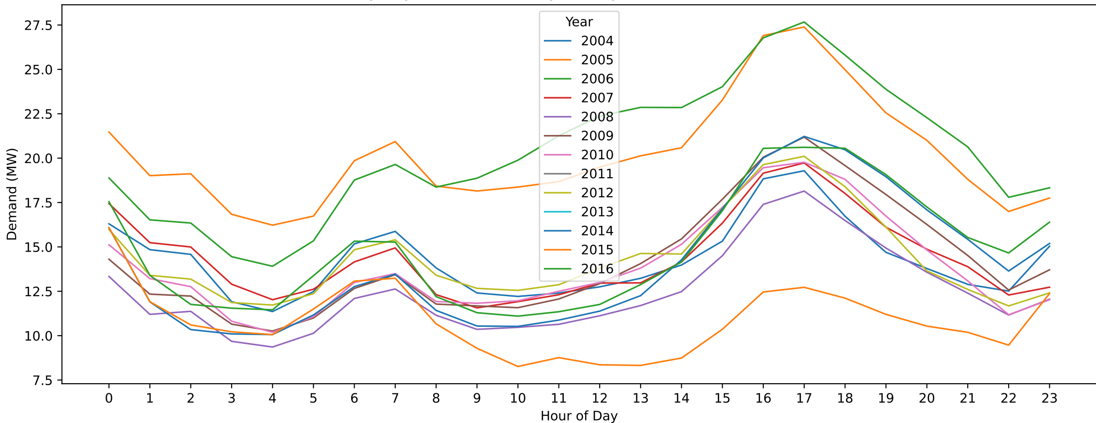
Kyabrym — Australia Day (Hourly Demand Across Years)
