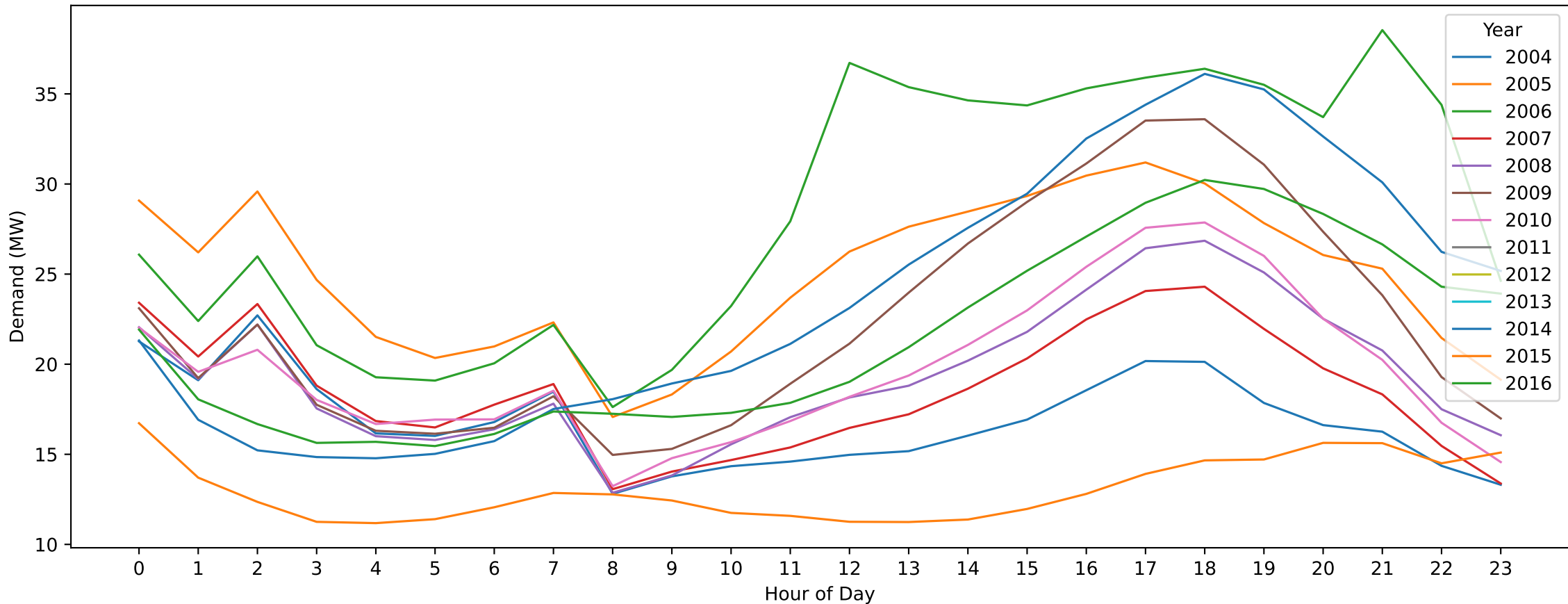
Eaglehawk — Australia Day (Hourly Demand Across Years)
