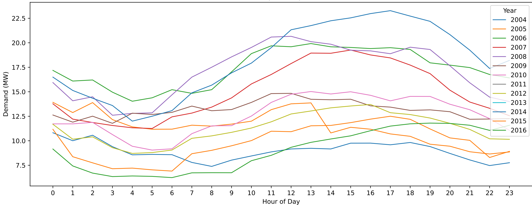
Robinvale — Australia Day (Hourly Demand Across Years)
