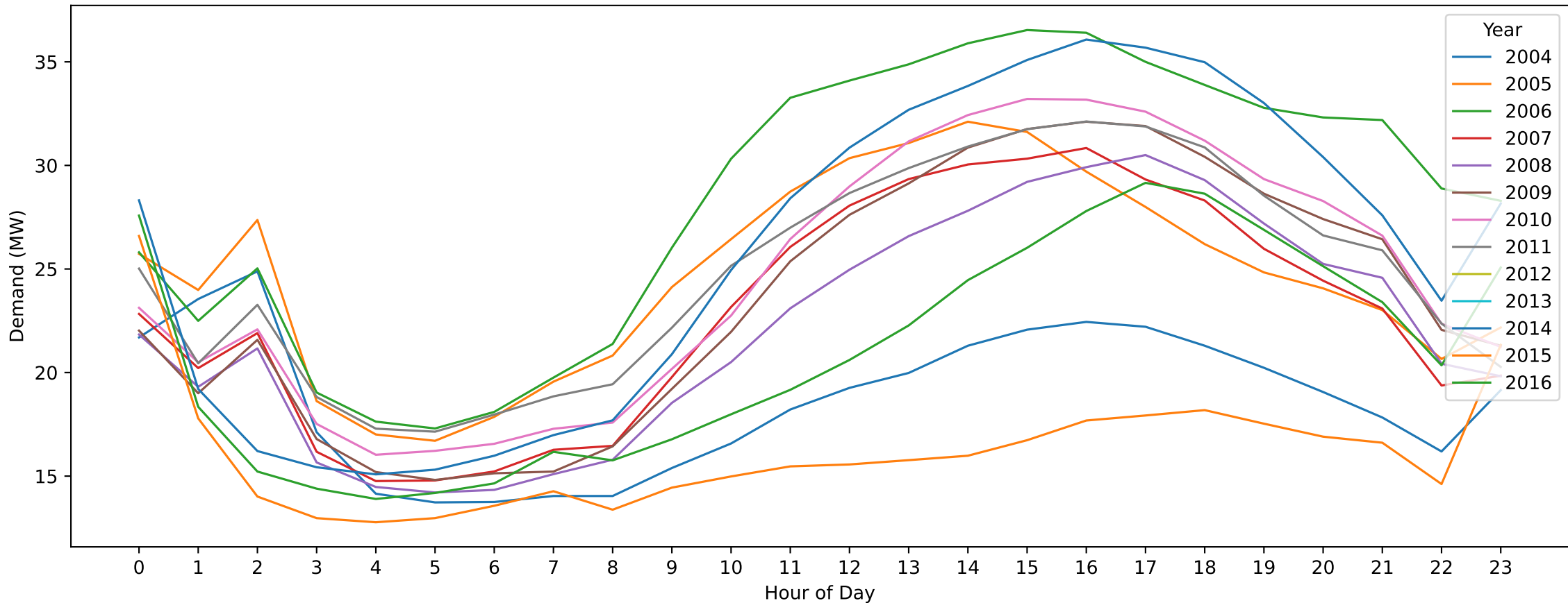
Mildura — Australia Day (Hourly Demand Across Years)
