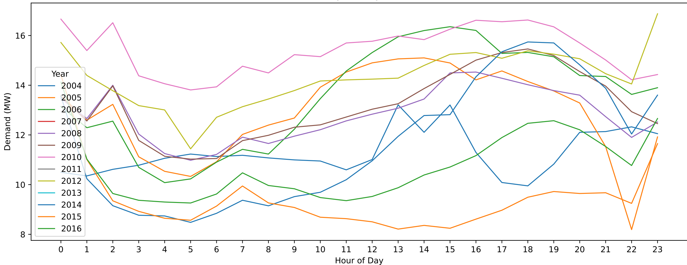
Stawell — Australia Day (Hourly Demand Across Years)
