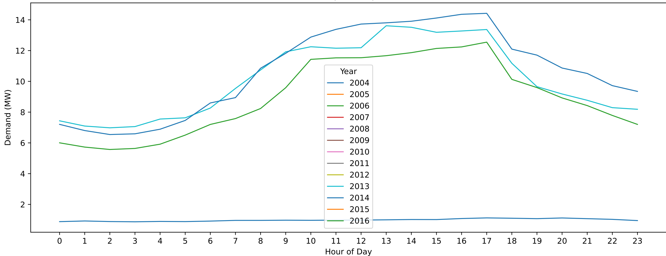
Docklands — Australia Day (Hourly Demand Across Years)
