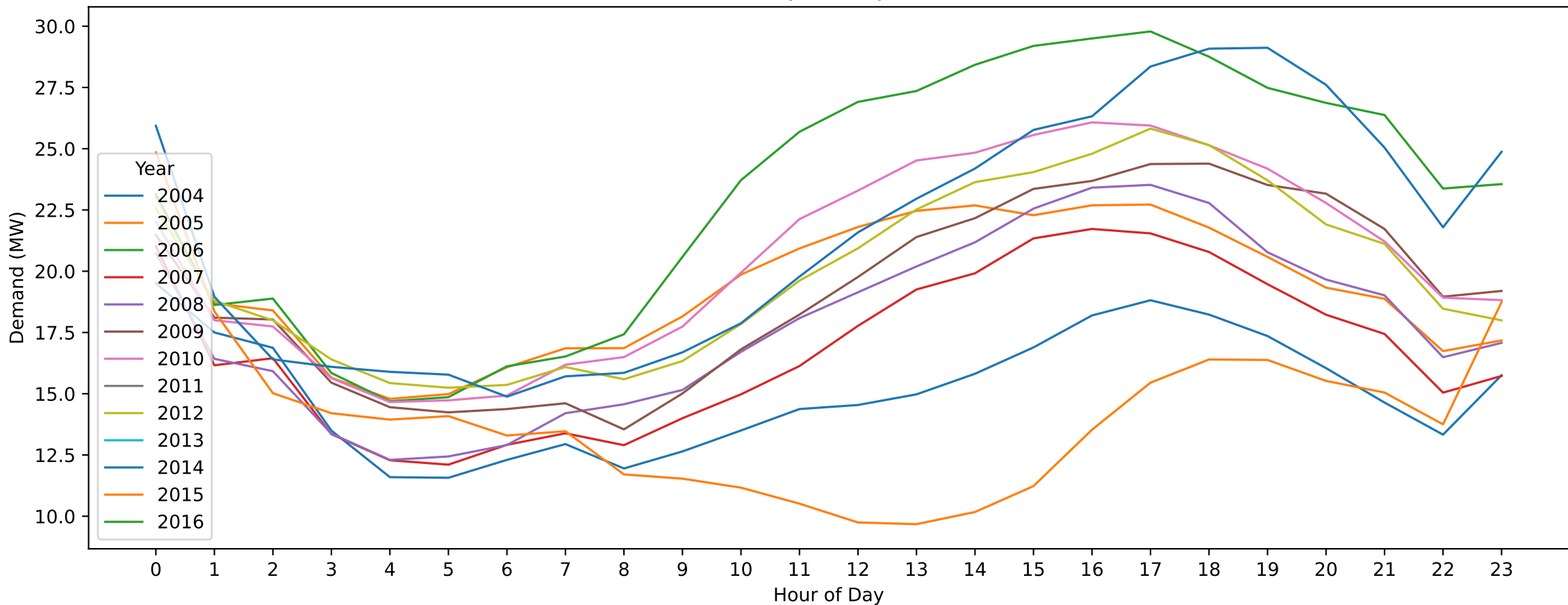
Swan Hill — Australia Day (Hourly Demand Across Years)
