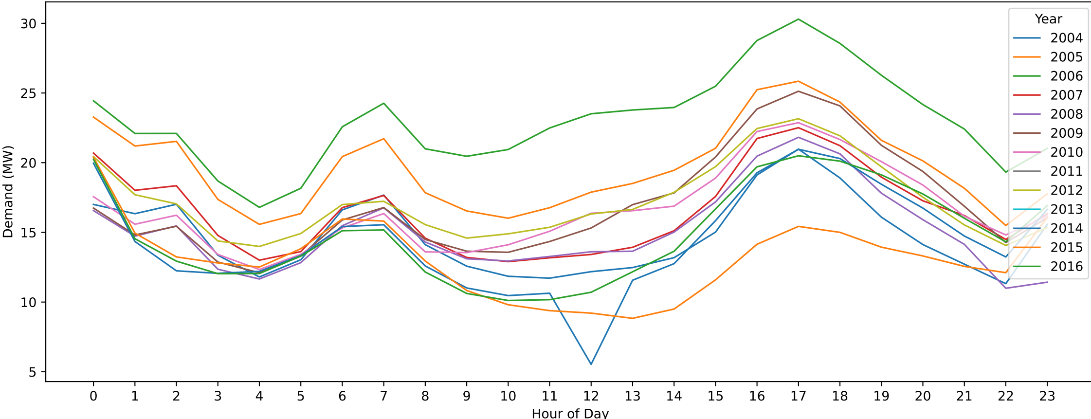
Numurkah — Australia Day (Hourly Demand Across Years)
