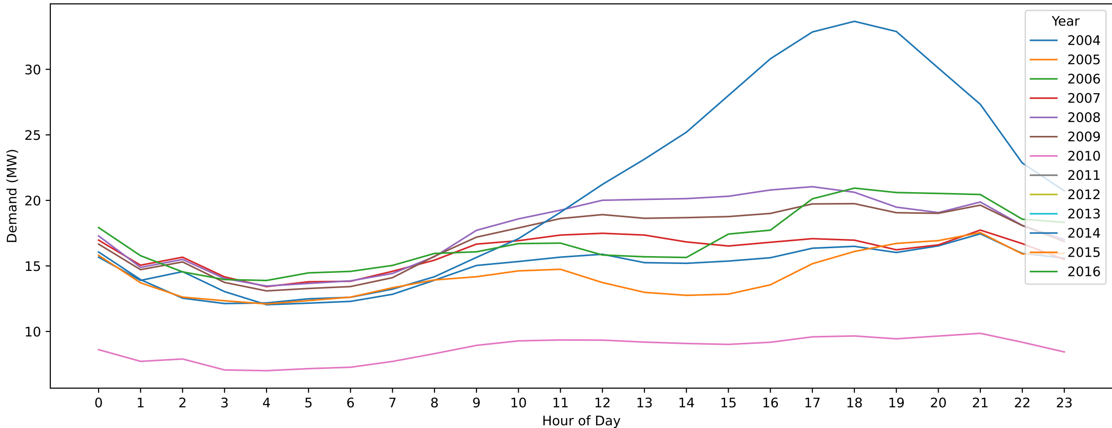
Geelong East — Australia Day (Hourly Demand Across Years)
