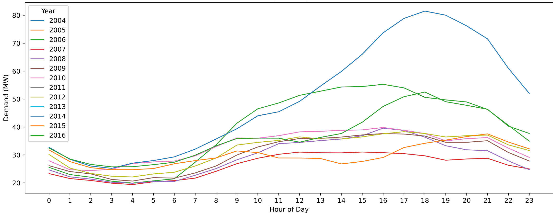
Werribee — Australia Day (Hourly Demand Across Years)
