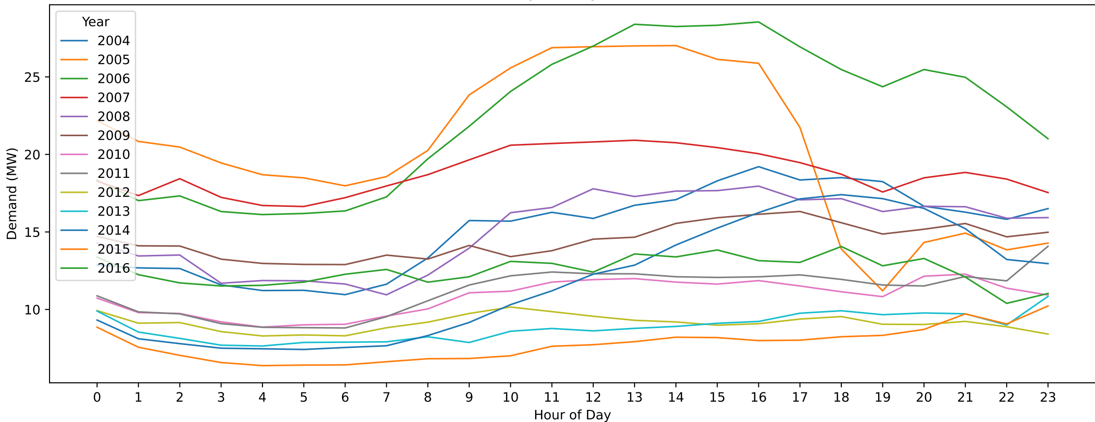
Corio — Australia Day (Hourly Demand Across Years)
