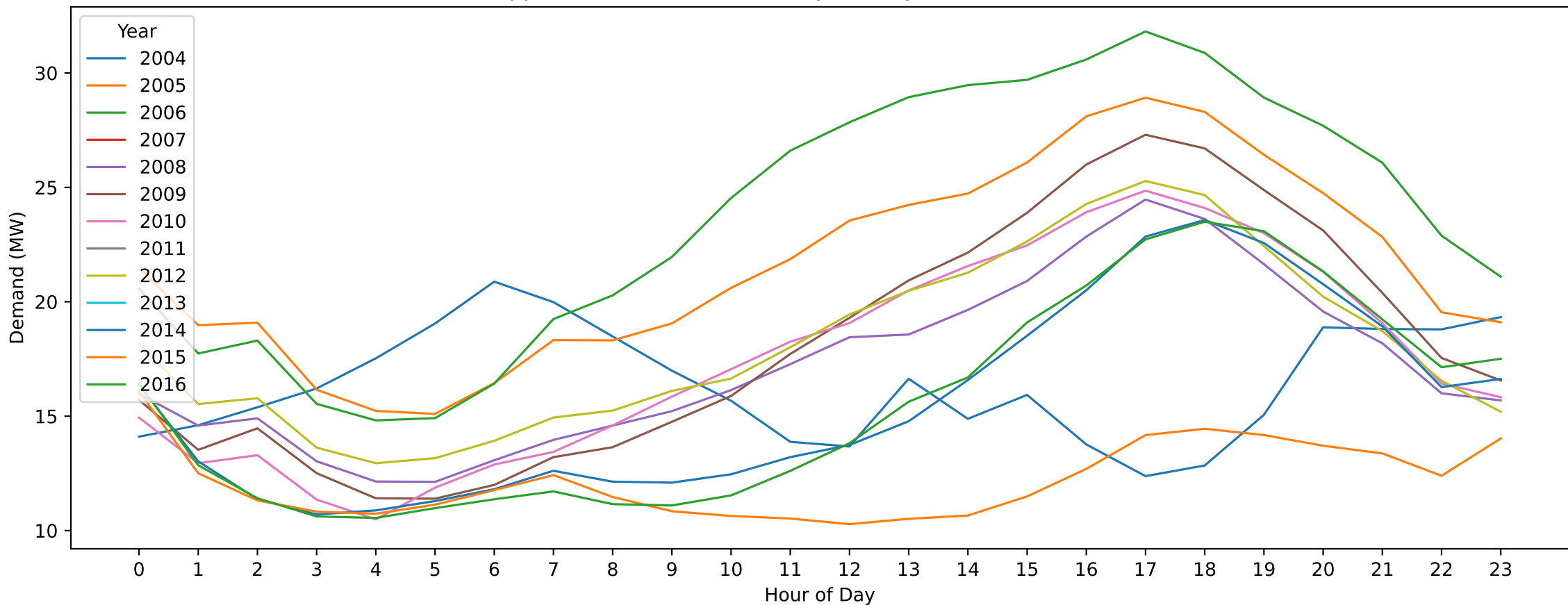
Shepparton Nth — Australia Day (Hourly Demand Across Years)
