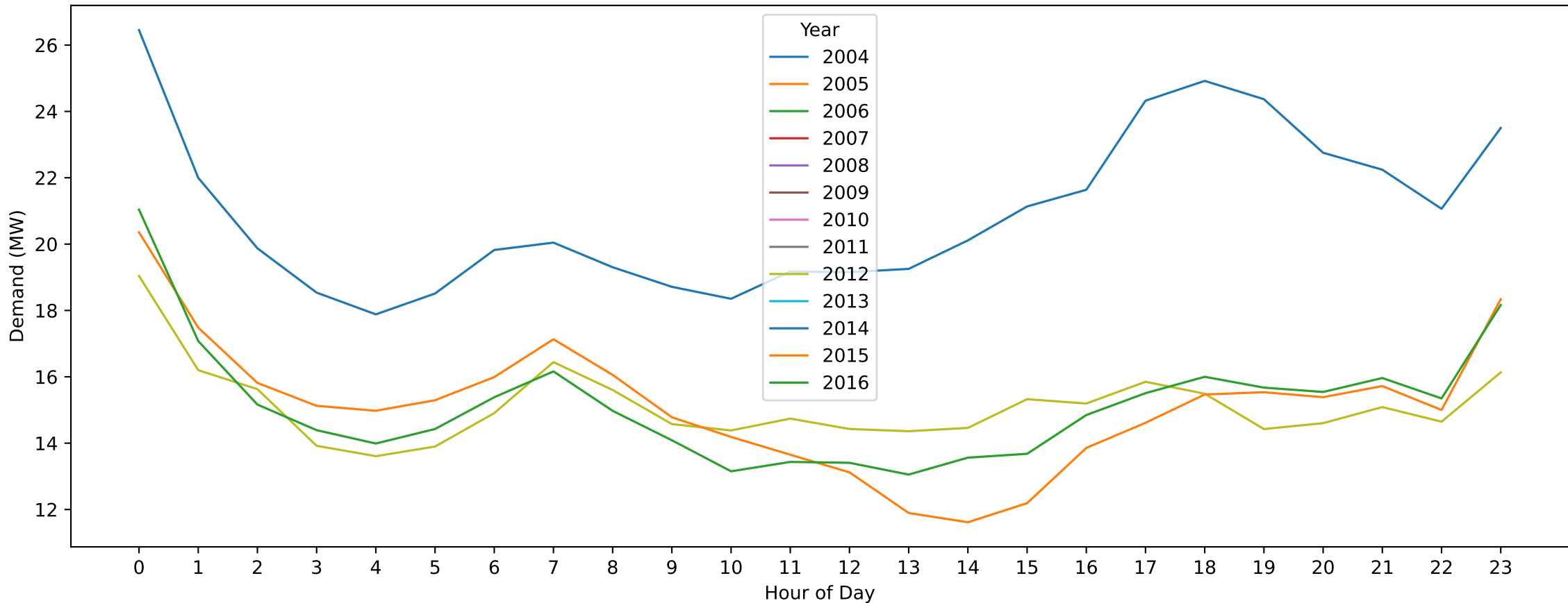
Koroit — Australia Day (Hourly Demand Across Years)
