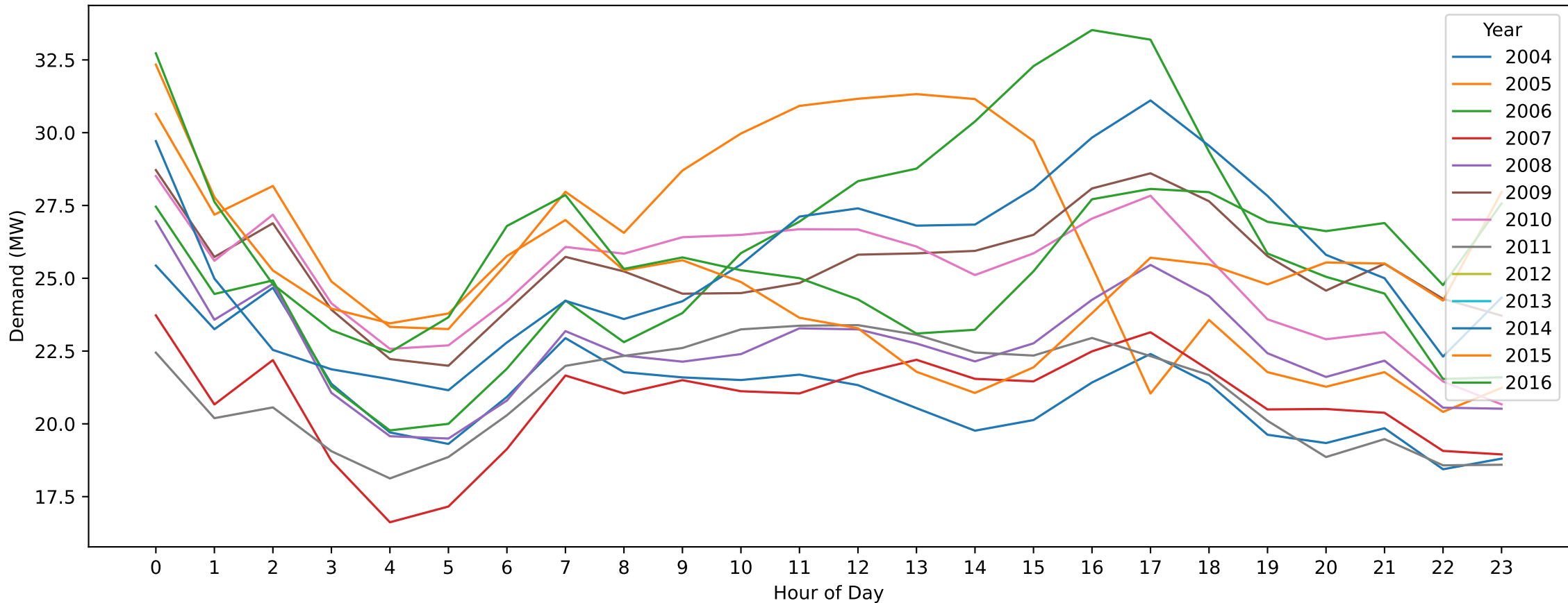
Warrnambool — Australia Day (Hourly Demand Across Years)
