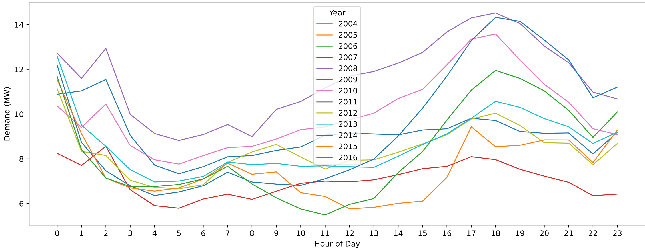
Castlemaine — Australia Day (Hourly Demand Across Years)
