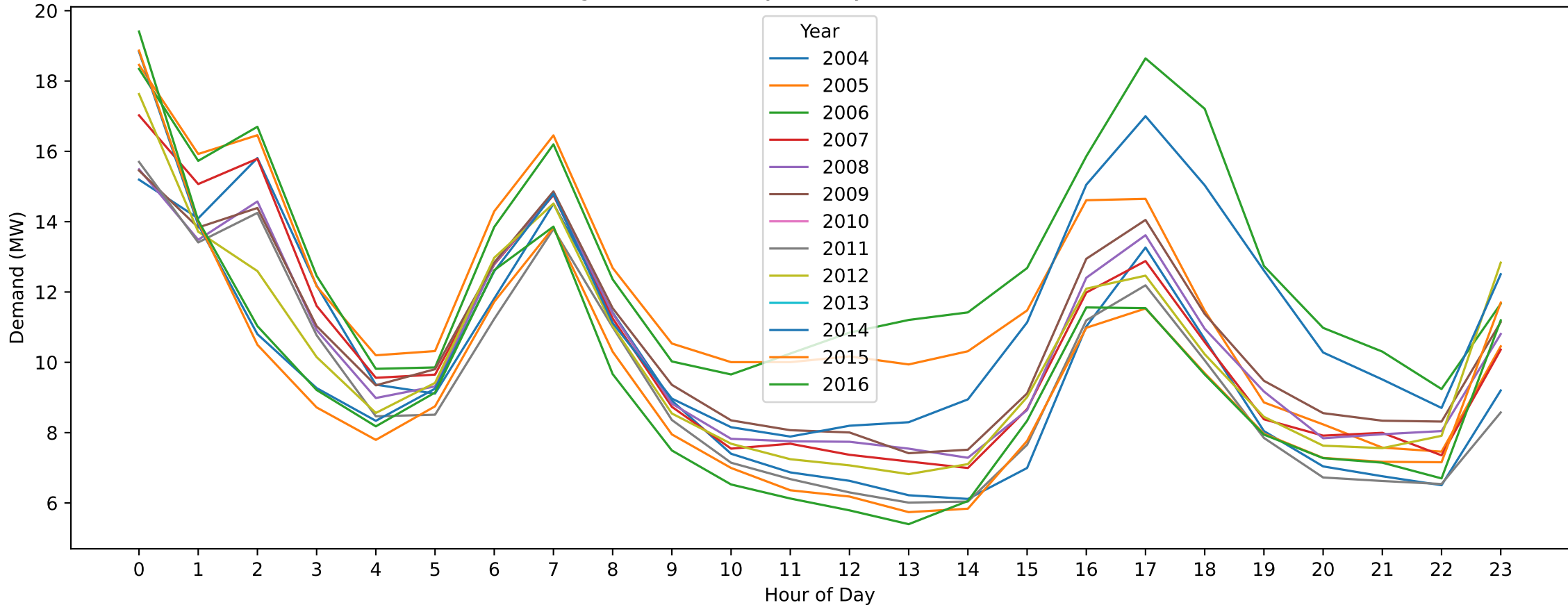
Terang — Australia Day (Hourly Demand Across Years)
