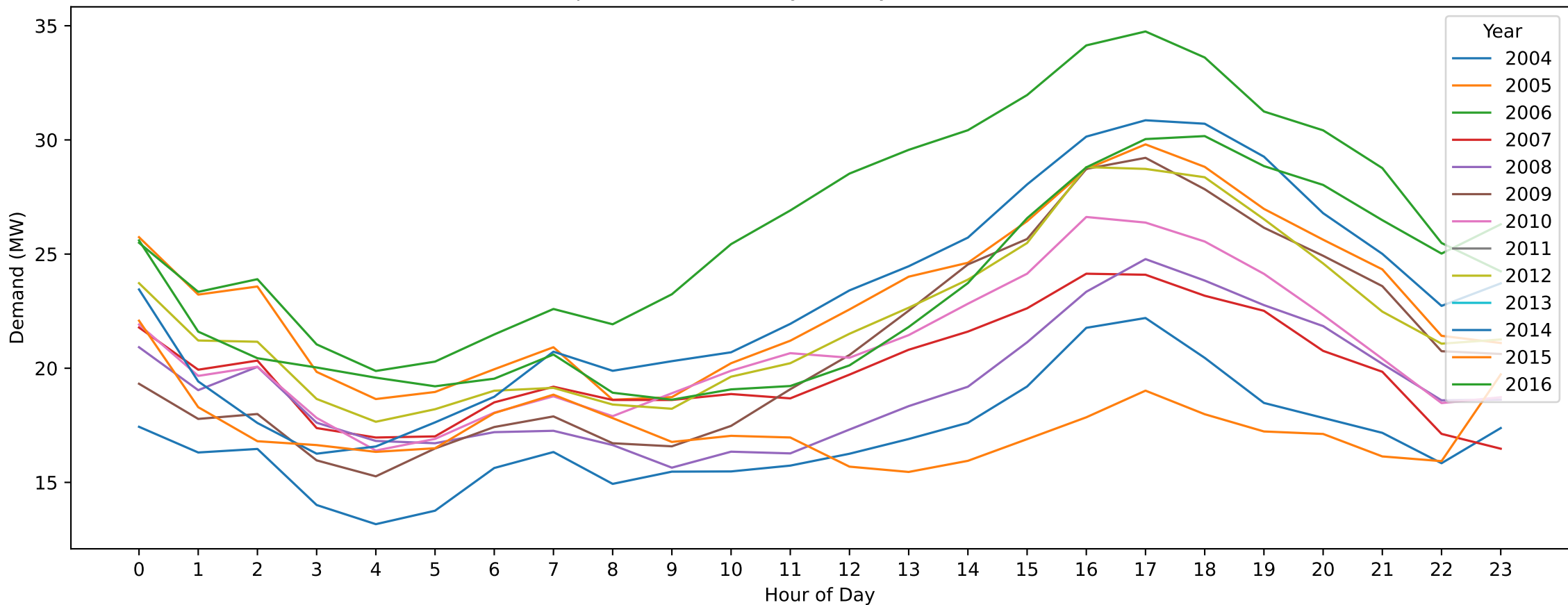
Mooroopna — Australia Day (Hourly Demand Across Years)
