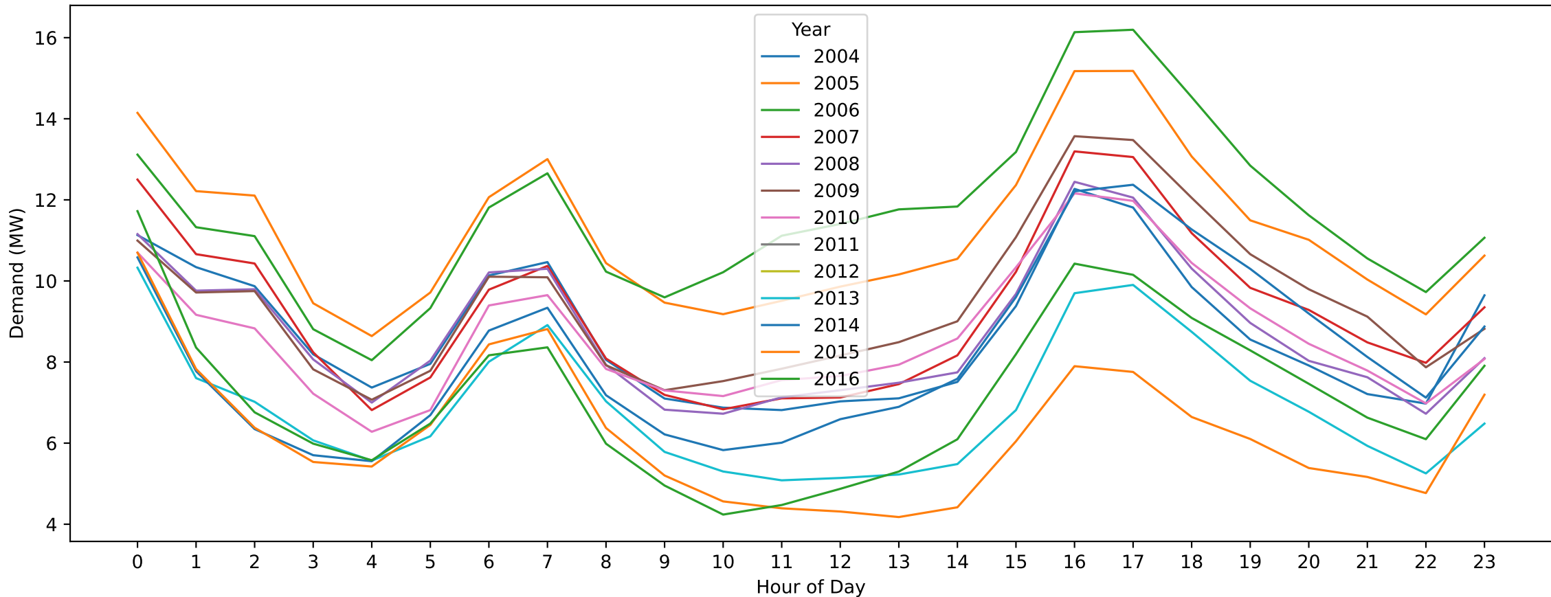
Cohuna — Australia Day (Hourly Demand Across Years)
