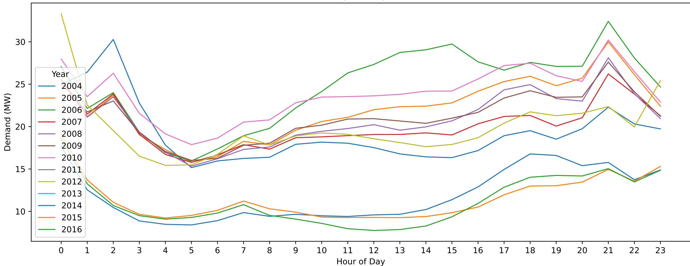
Woodend — Australia Day (Hourly Demand Across Years)
