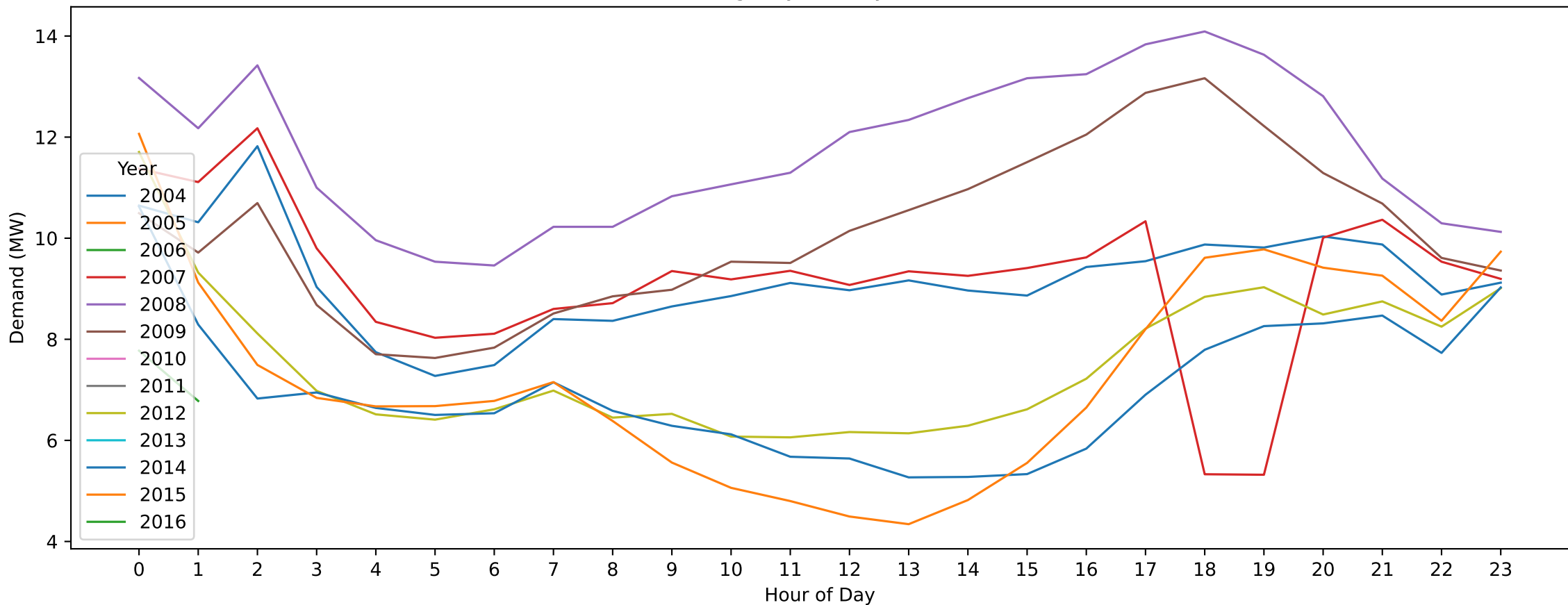
Castlemaine — Boxing Day (Hourly Demand Across Years)
