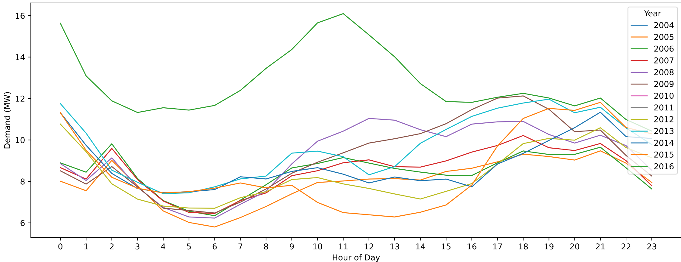
Bacchus Marsh — Boxing Day (Hourly Demand Across Years)
