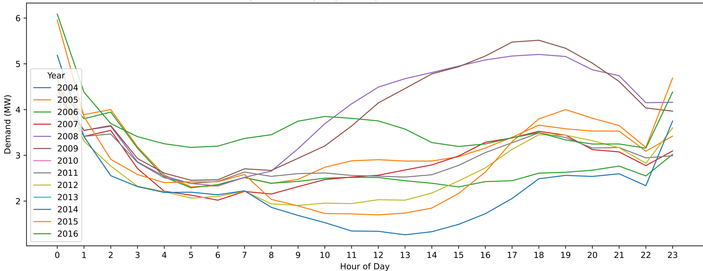
Ouyen — Boxing Day (Hourly Demand Across Years)
