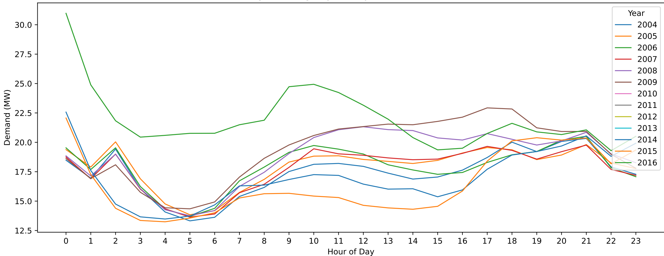
Geelong — Boxing Day (Hourly Demand Across Years)
