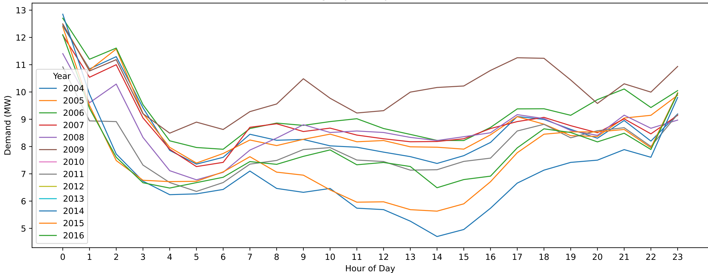
Portland — Boxing Day (Hourly Demand Across Years)
