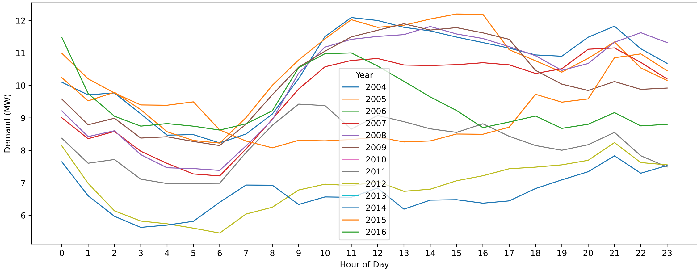
Corio — Boxing Day (Hourly Demand Across Years)
