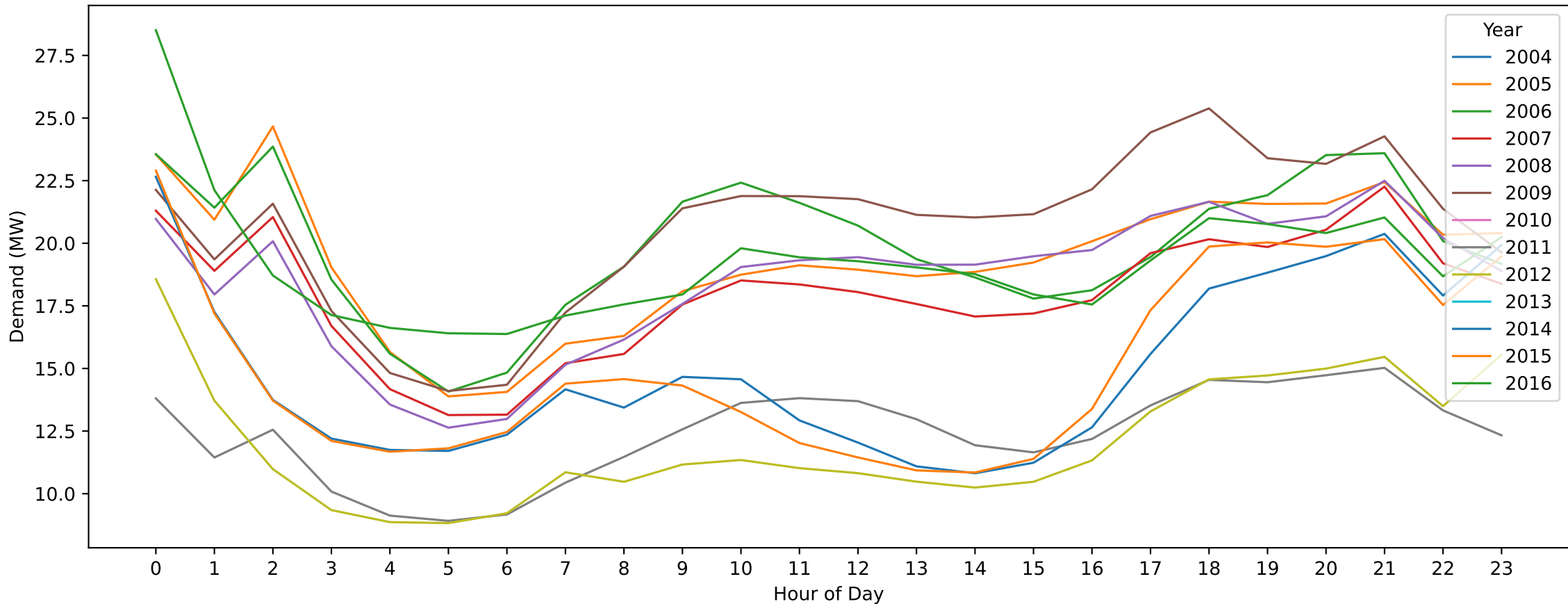
Drysdale — Boxing Day (Hourly Demand Across Years)
