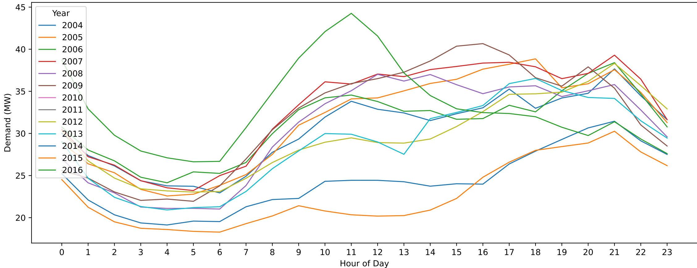
St Albans — Boxing Day (Hourly Demand Across Years)
