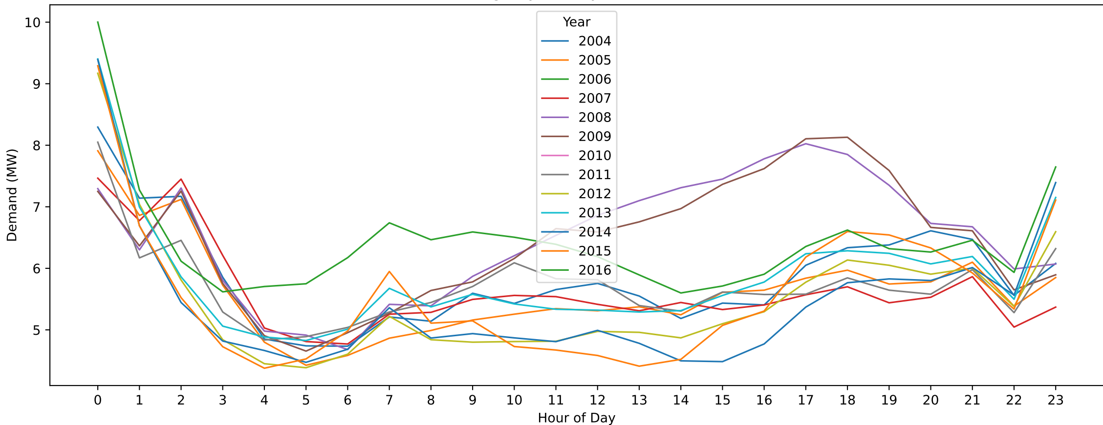
Ararat — Boxing Day (Hourly Demand Across Years)
