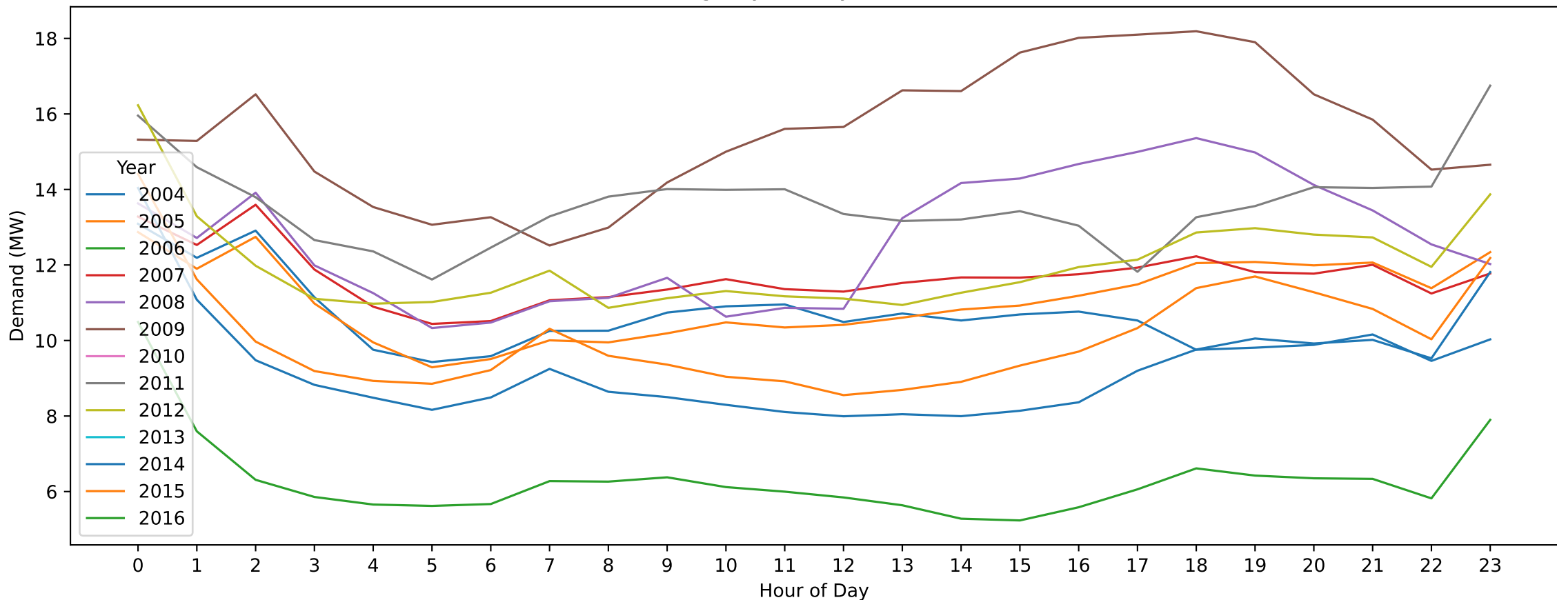
Stawell — Boxing Day (Hourly Demand Across Years)
