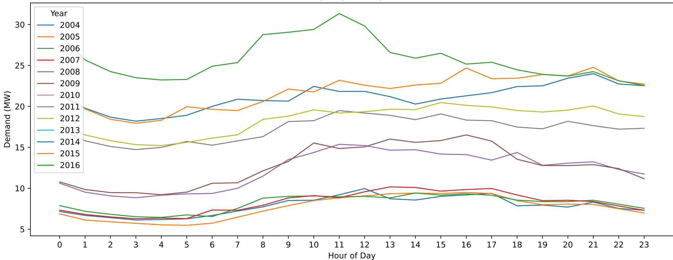
Sunshine East — Boxing Day (Hourly Demand Across Years)
