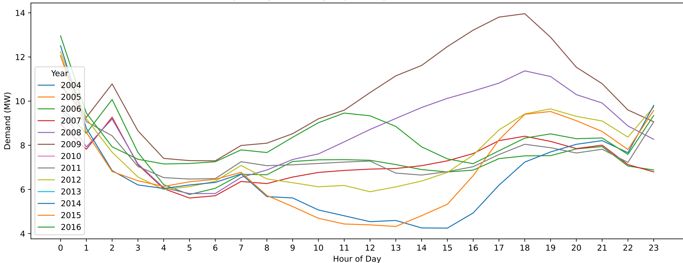
Maryborough — Boxing Day (Hourly Demand Across Years)
