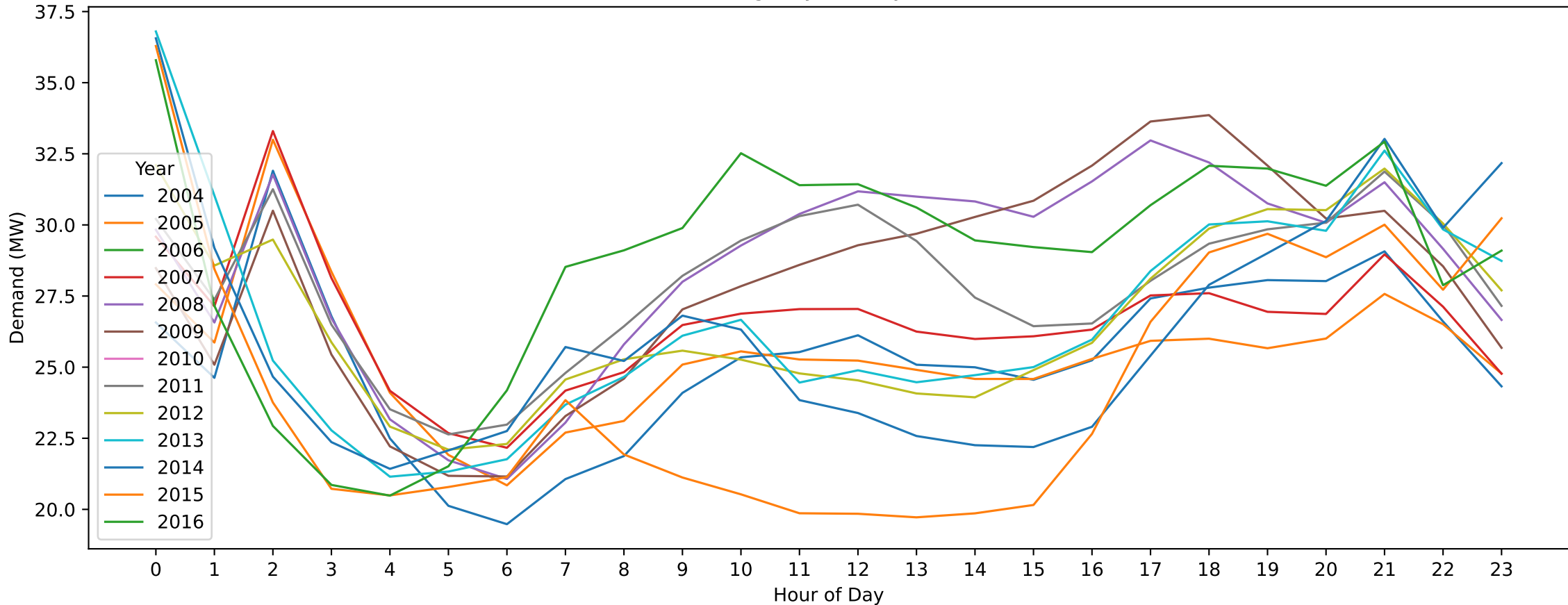
Ballarat South — Boxing Day (Hourly Demand Across Years)
