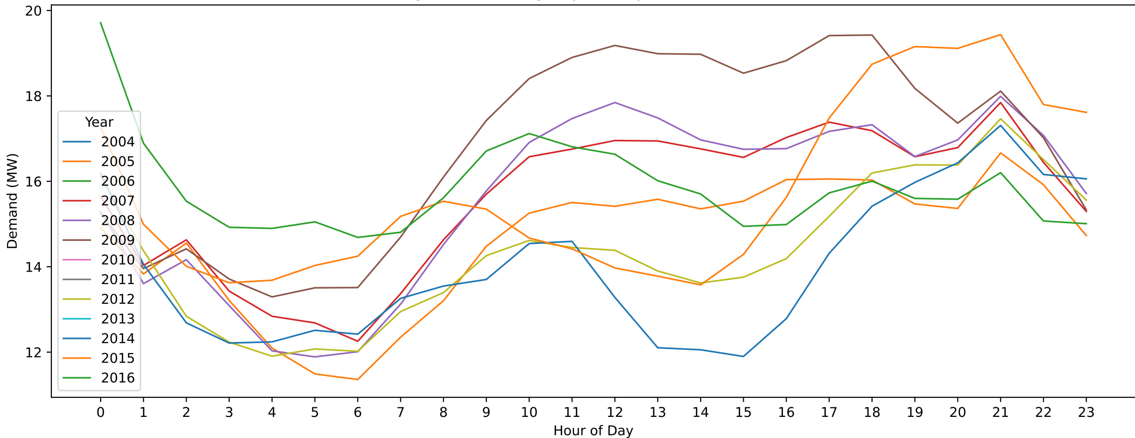
Geelong East — Boxing Day (Hourly Demand Across Years)
