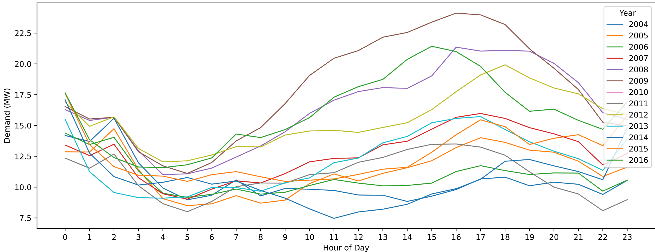
Cobram East — Boxing Day (Hourly Demand Across Years)
