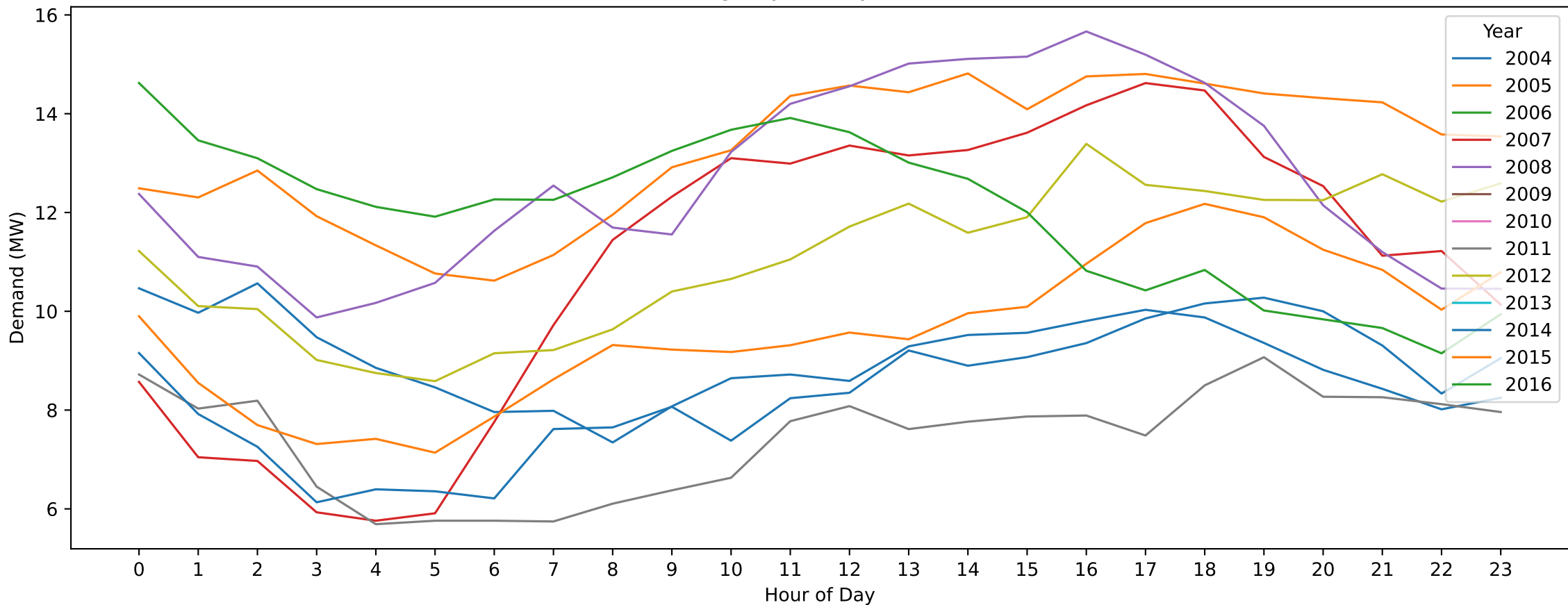
Robinvale — Boxing Day (Hourly Demand Across Years)
