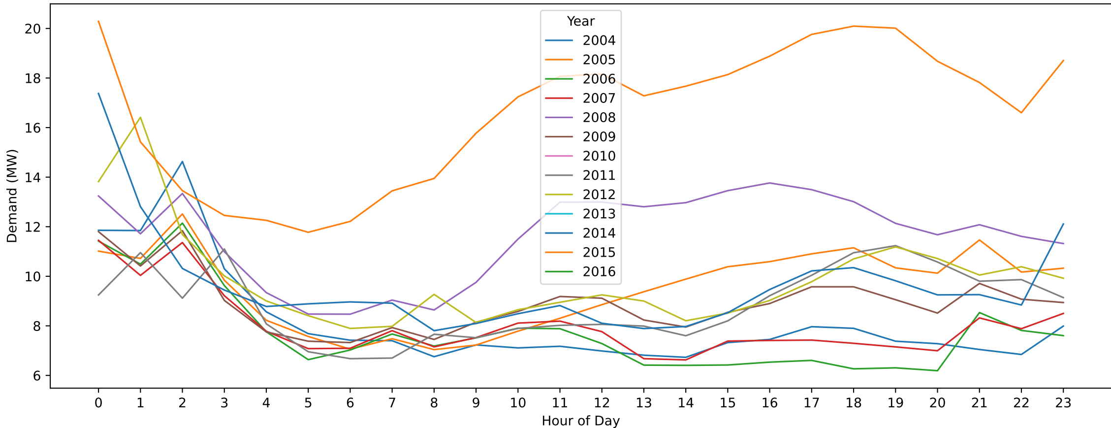
Merbein — Christmas Day (Hourly Demand Across Years)
