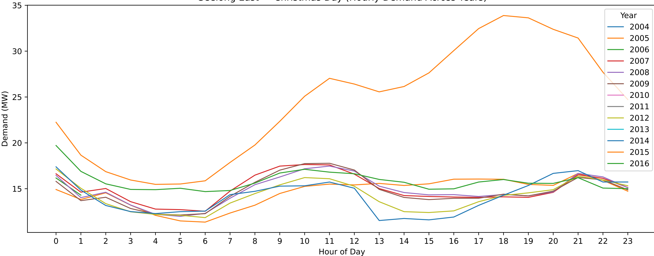
Geelong East — Christmas Day (Hourly Demand Across Years)
