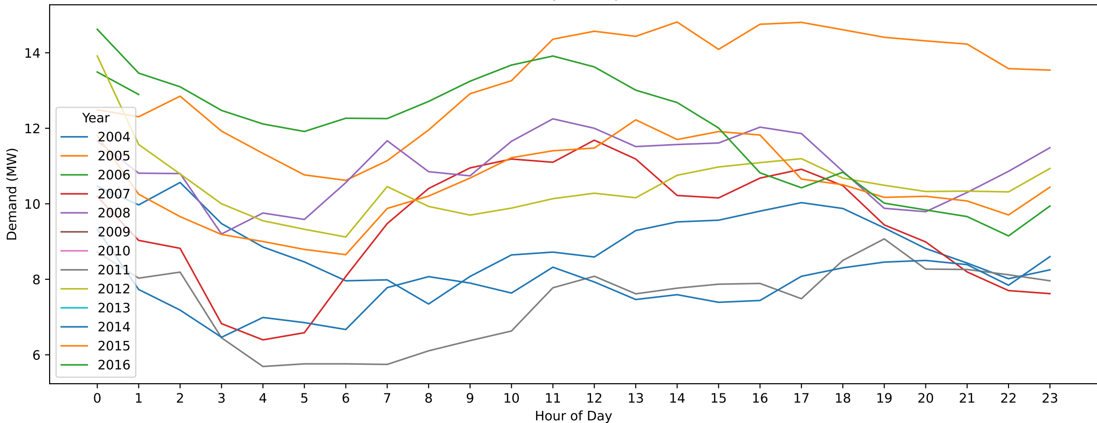
Robinvale — Christmas Day (Hourly Demand Across Years)
