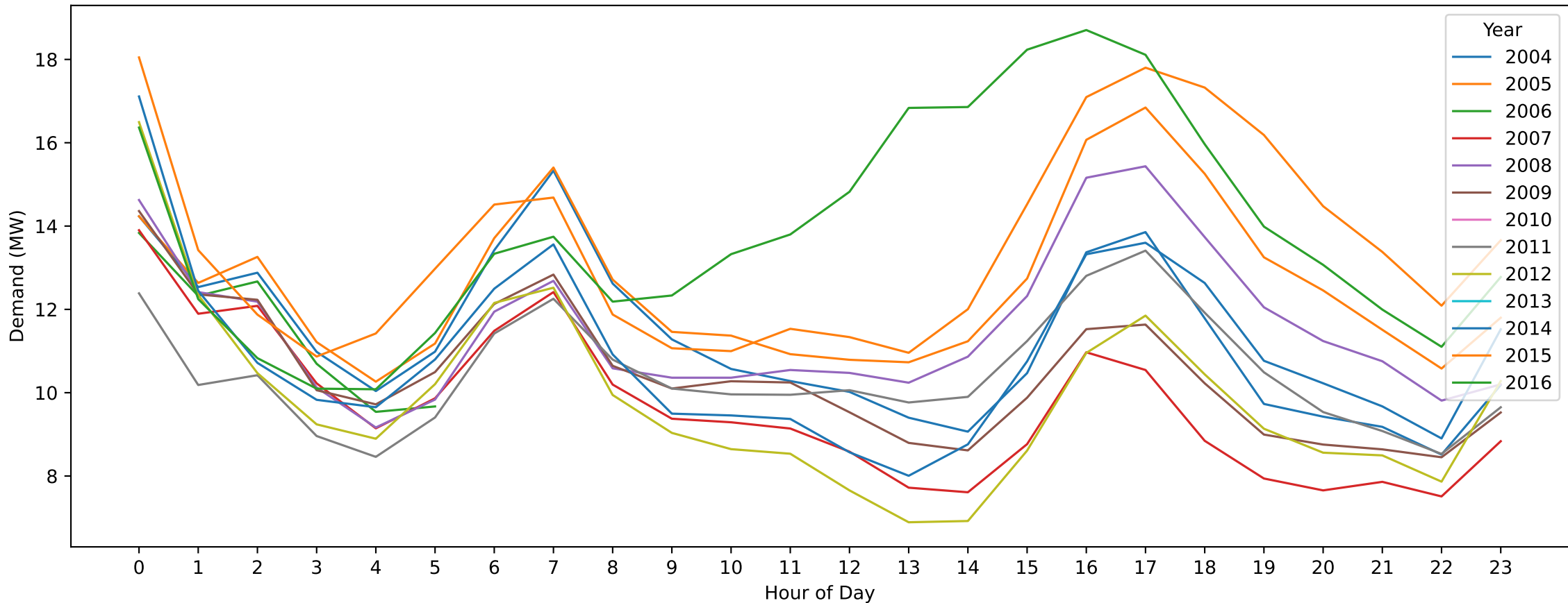
Kyabrym — Christmas Day (Hourly Demand Across Years)
