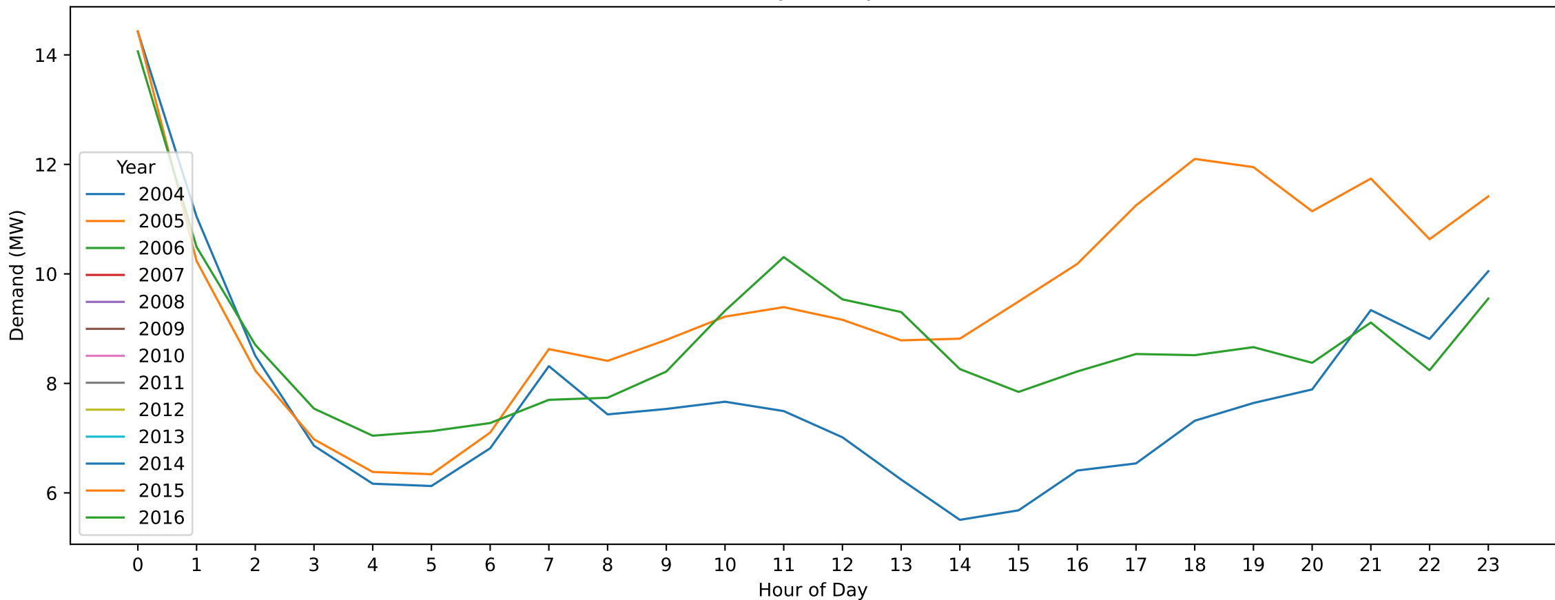
Gisborne — Christmas Day (Hourly Demand Across Years)
