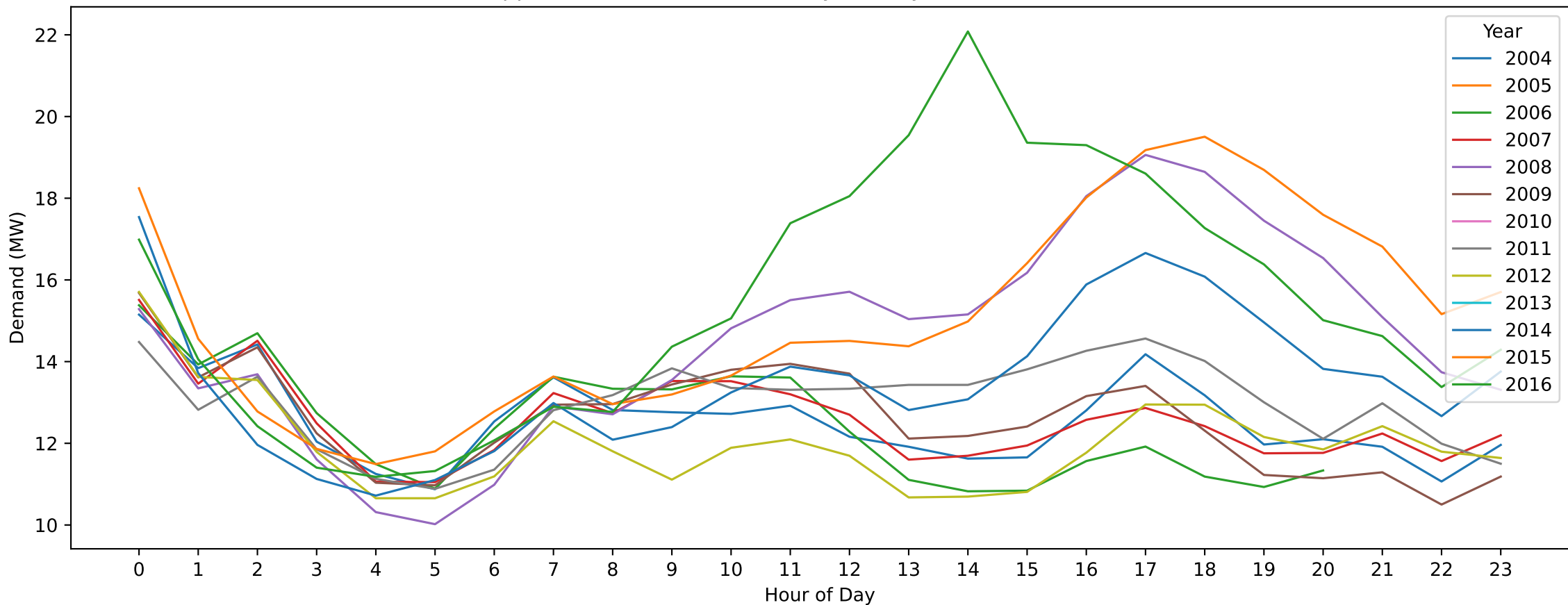
Shepparton Nth — Christmas Day (Hourly Demand Across Years)
