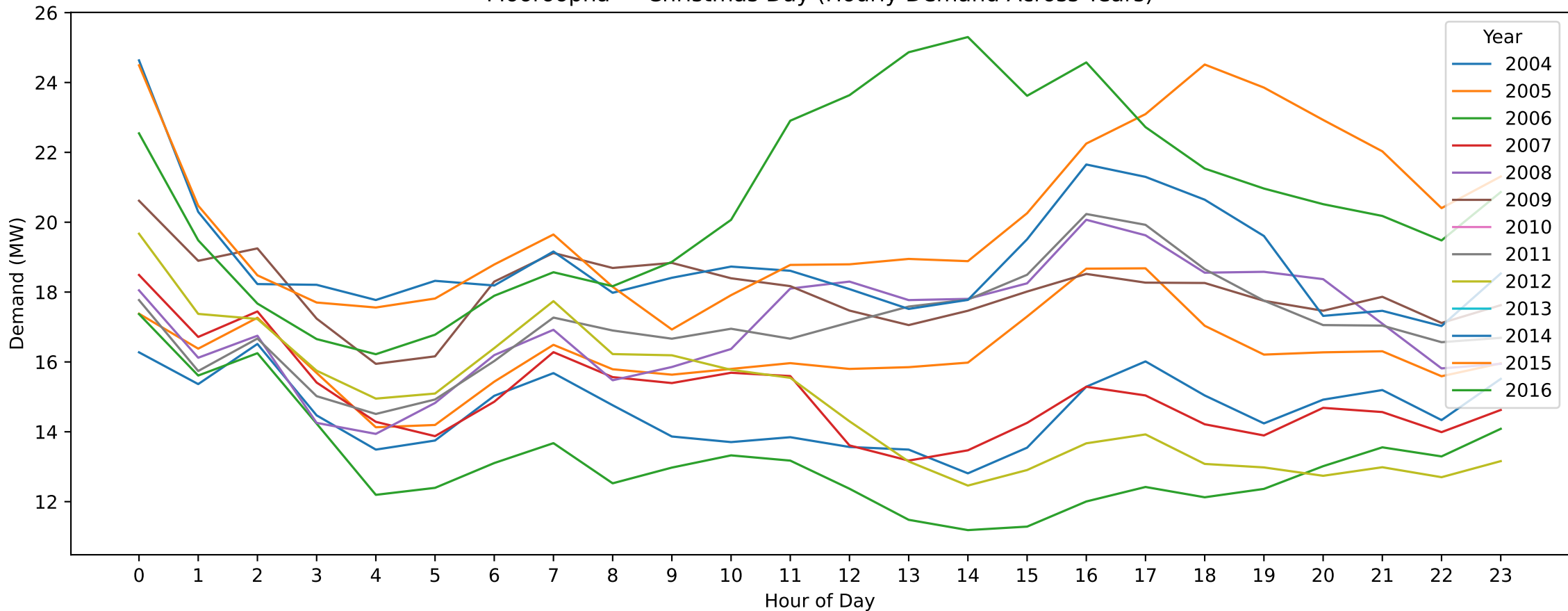
Mooroopna — Christmas Day (Hourly Demand Across Years)
