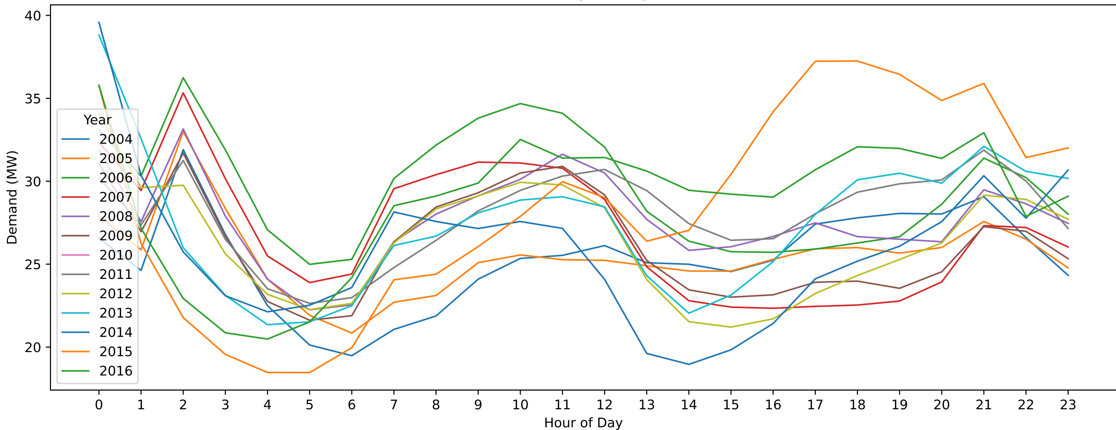
Ballarat South — Christmas Day (Hourly Demand Across Years)
