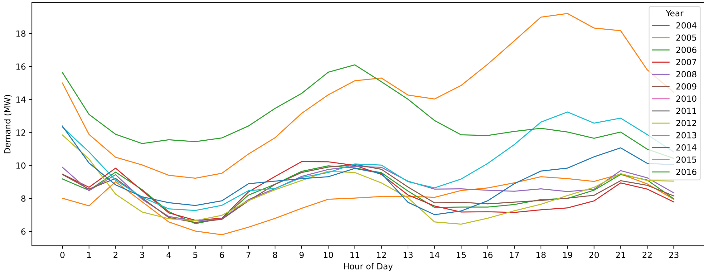
Bacchus Marsh — Christmas Day (Hourly Demand Across Years)
