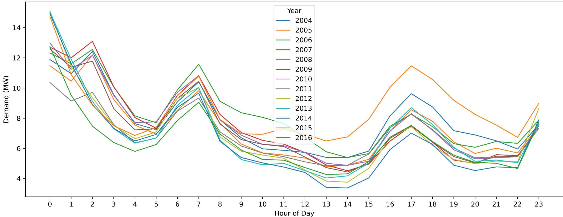
Camperdown — Christmas Day (Hourly Demand Across Years)
