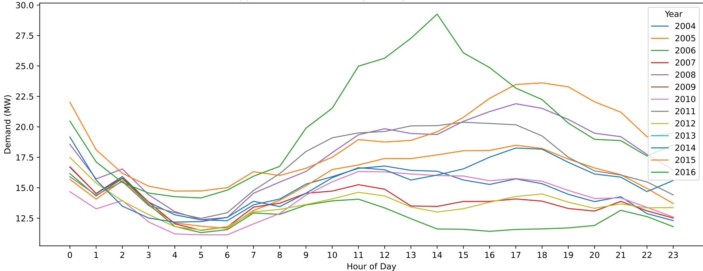
Shepparton — Christmas Day (Hourly Demand Across Years)
