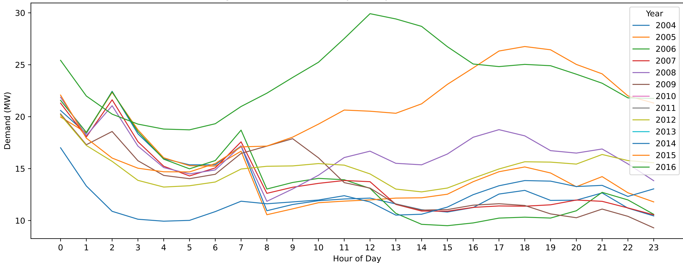
Eaglehawk — Christmas Day (Hourly Demand Across Years)
