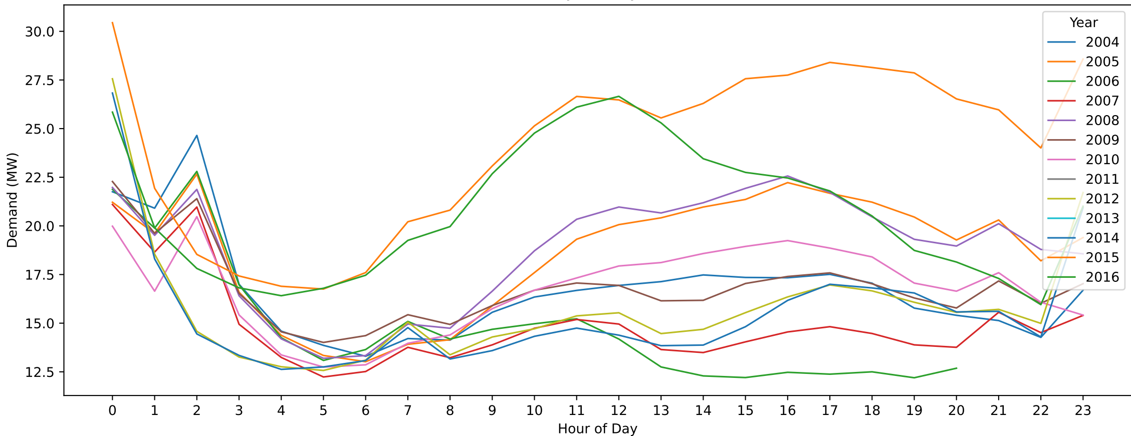
Mildura — Christmas Day (Hourly Demand Across Years)
