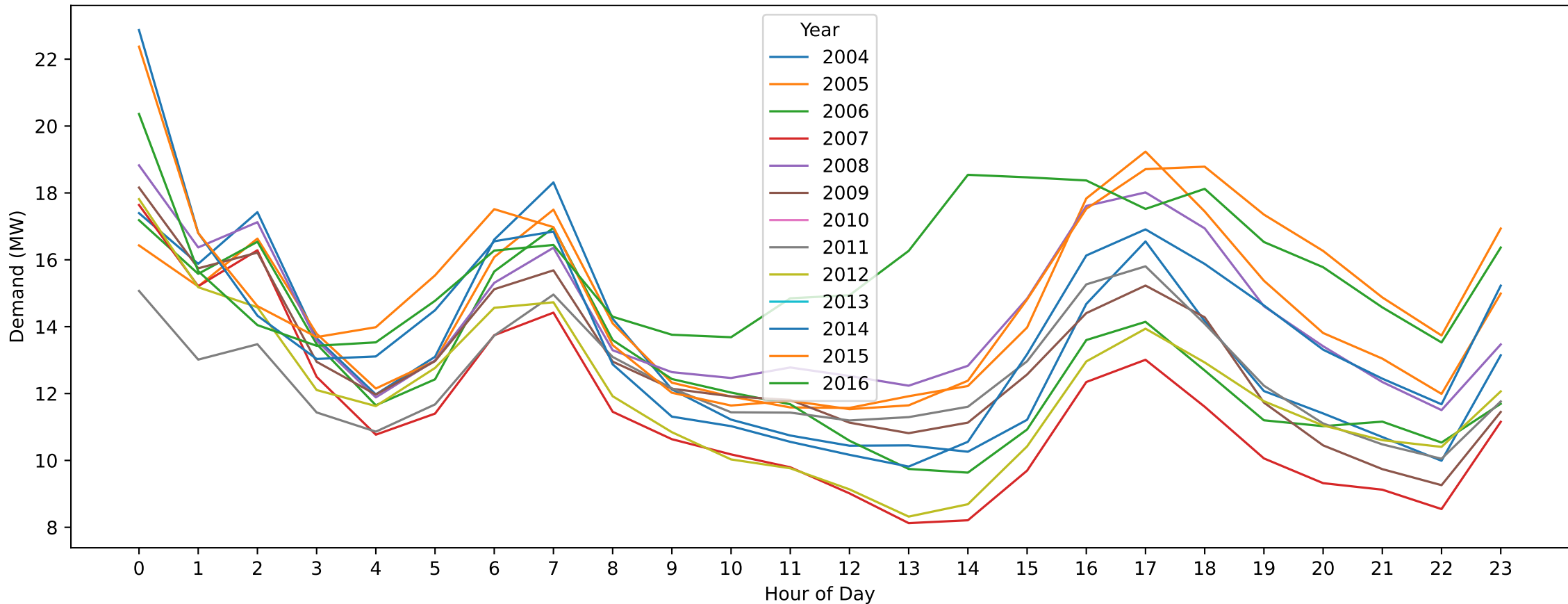
Numurkah — Christmas Day (Hourly Demand Across Years)
