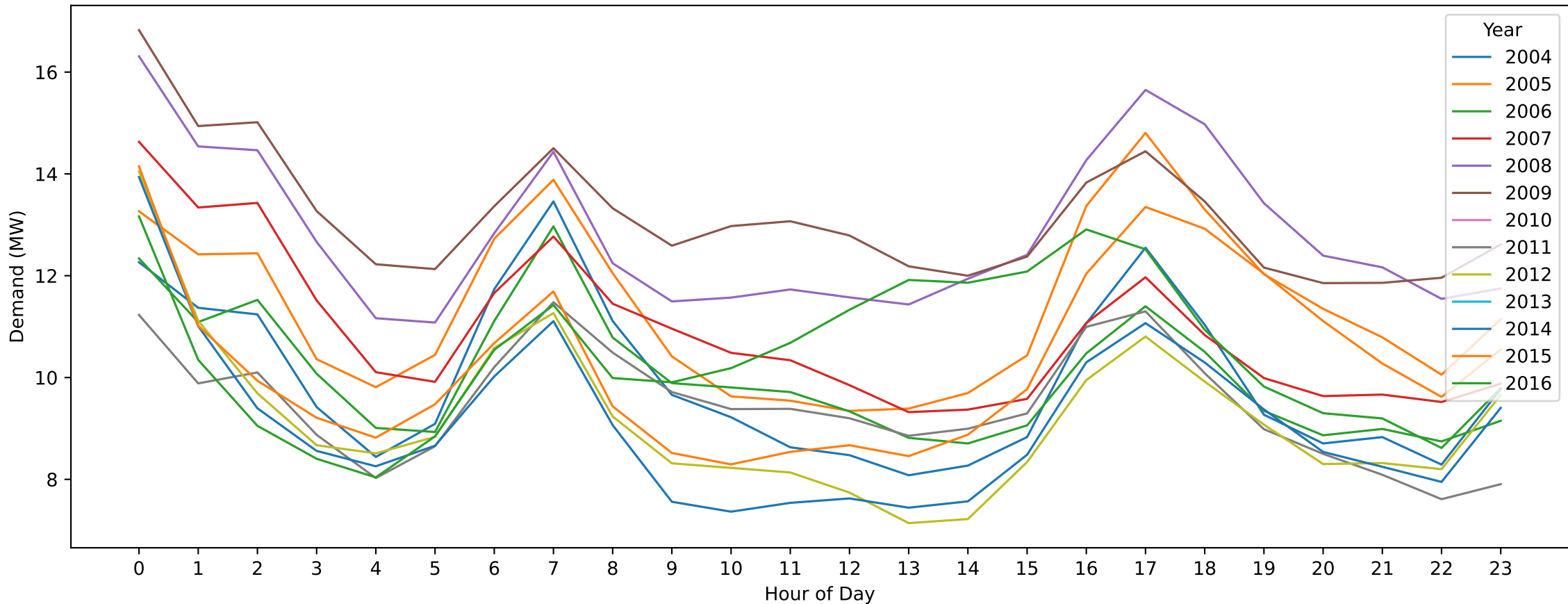
Stanhope — Christmas Day (Hourly Demand Across Years)
