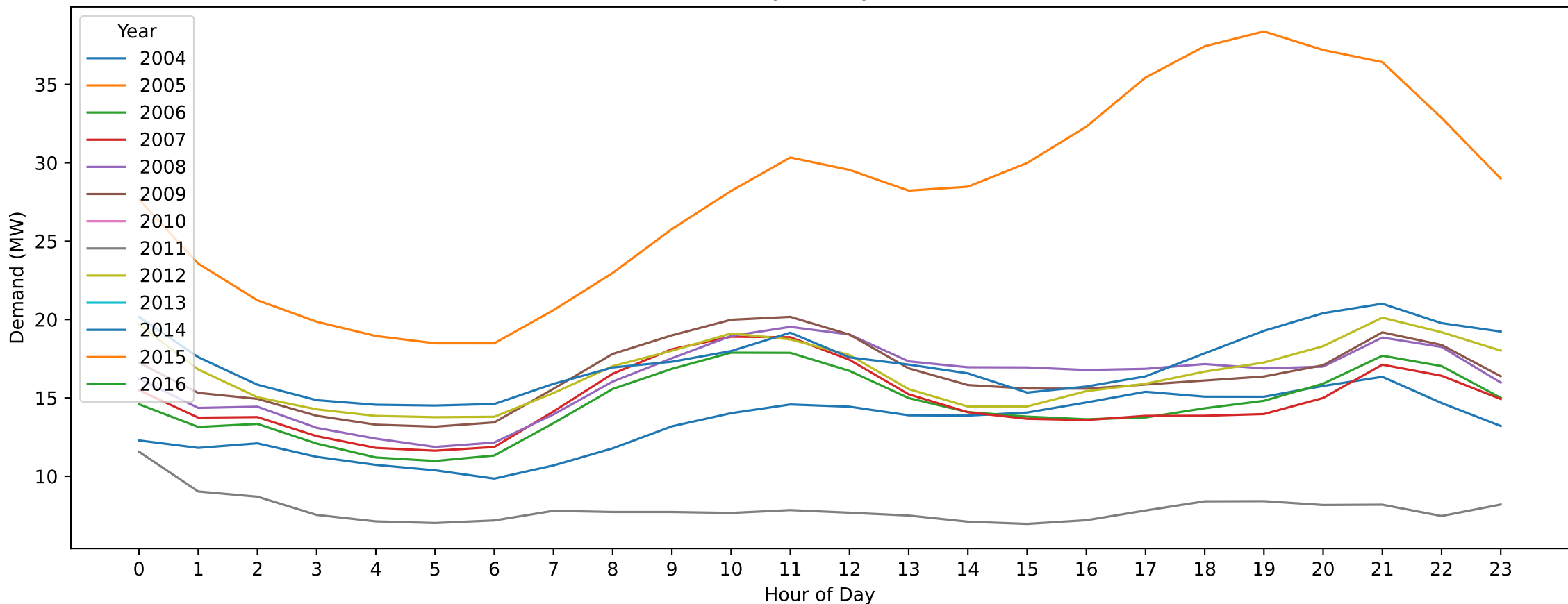
Melton — Christmas Day (Hourly Demand Across Years)
