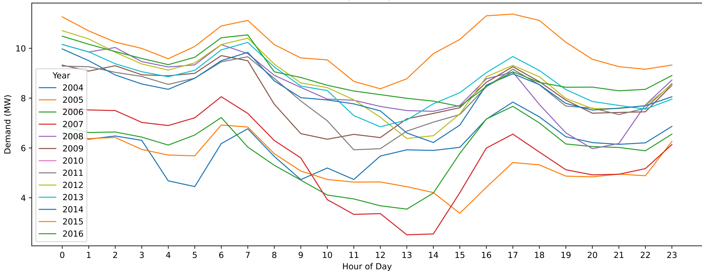
Cobden — Christmas Day (Hourly Demand Across Years)
