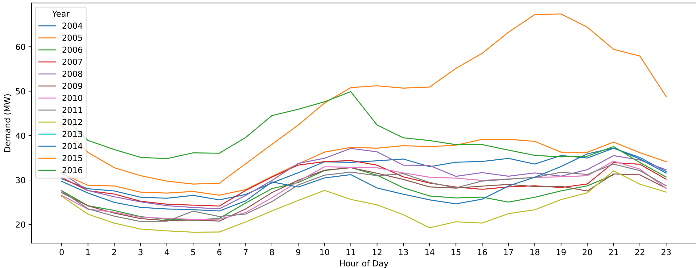
Laverton — Christmas Day (Hourly Demand Across Years)
