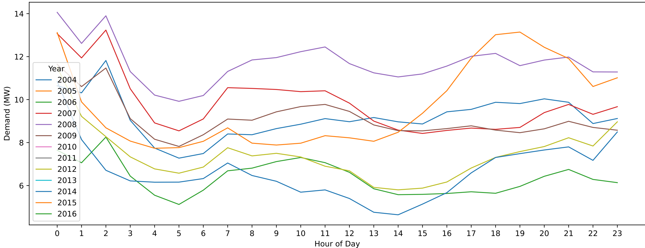
Castlemaine — Christmas Day (Hourly Demand Across Years)
