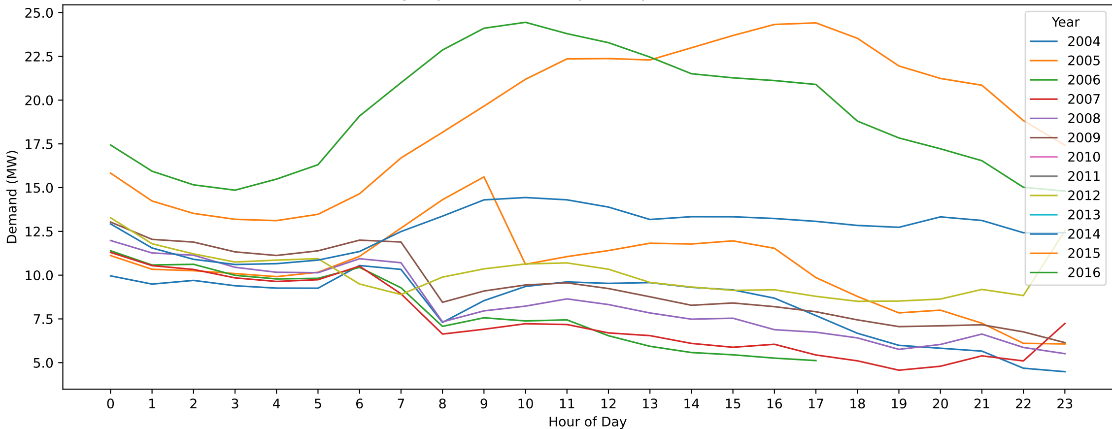
Geelong City — Christmas Day (Hourly Demand Across Years)
