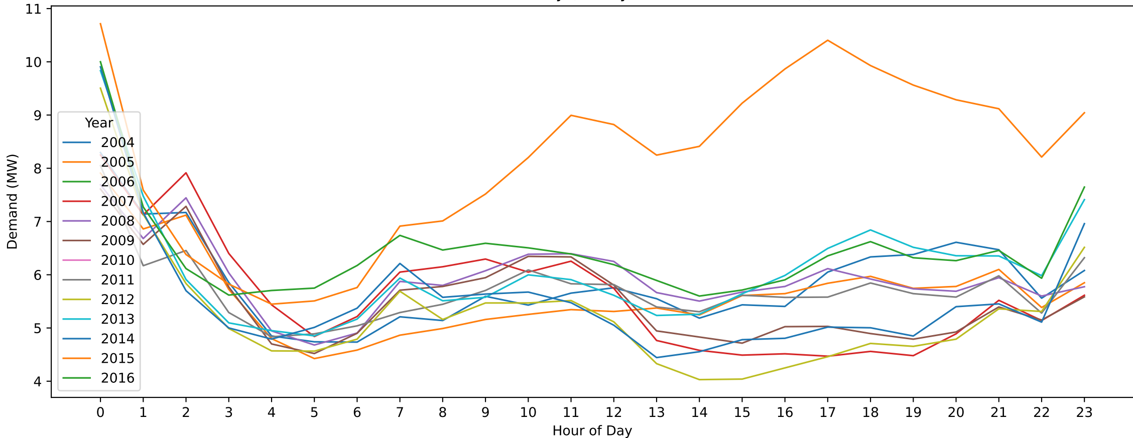
Ararat — Christmas Day (Hourly Demand Across Years)
