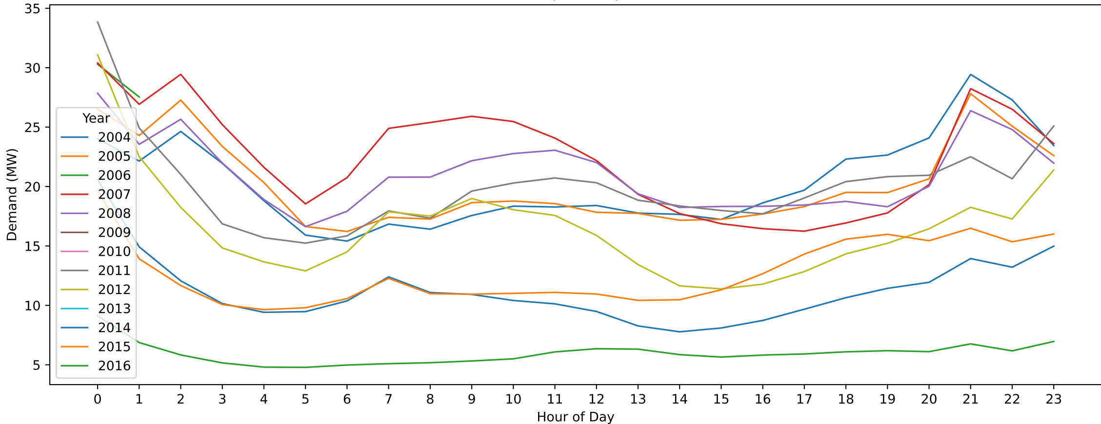
Woodend — Christmas Day (Hourly Demand Across Years)
