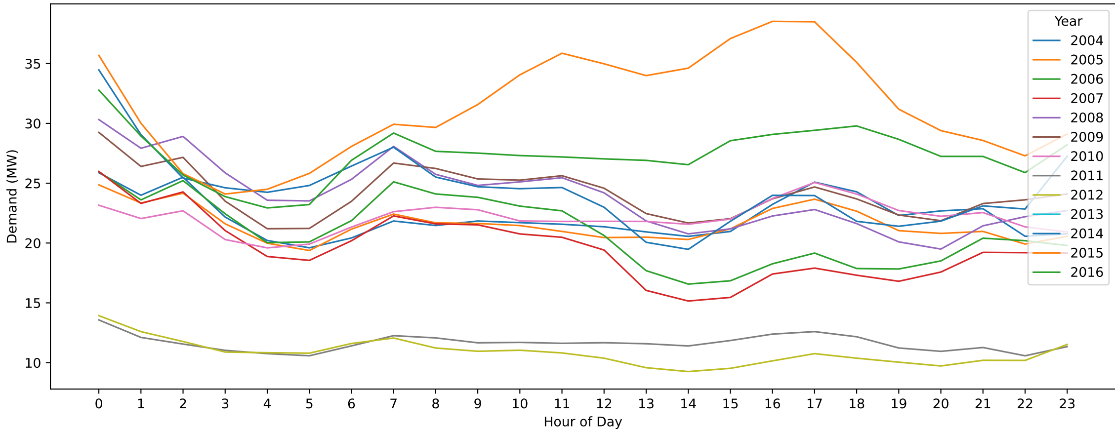
Warrnambool — Christmas Day (Hourly Demand Across Years)
