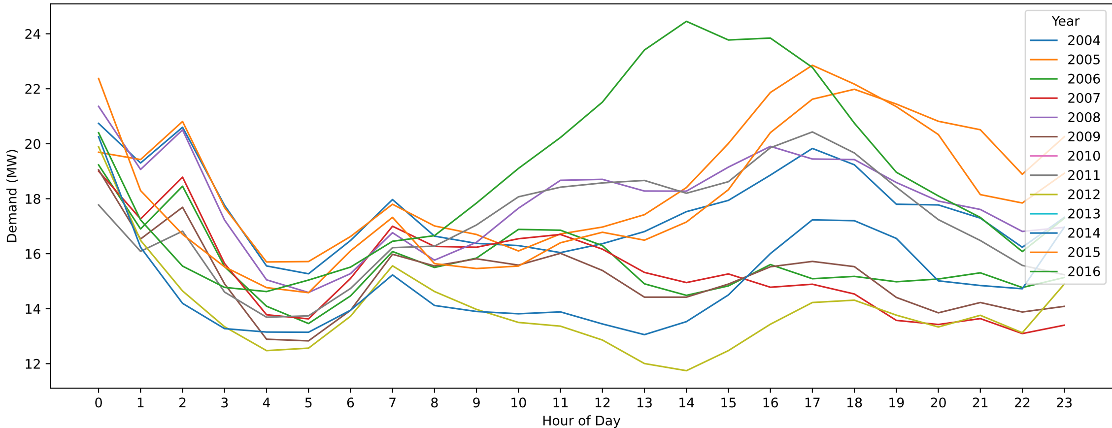
Echuca — Christmas Day (Hourly Demand Across Years)
