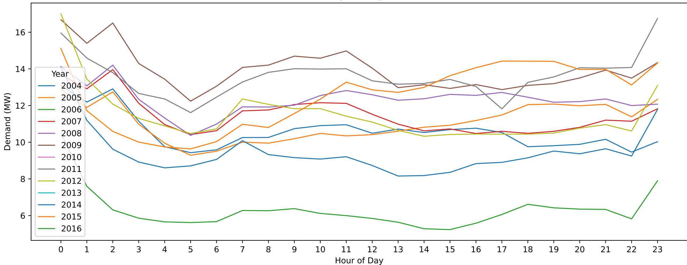
Stawell — Christmas Day (Hourly Demand Across Years)
