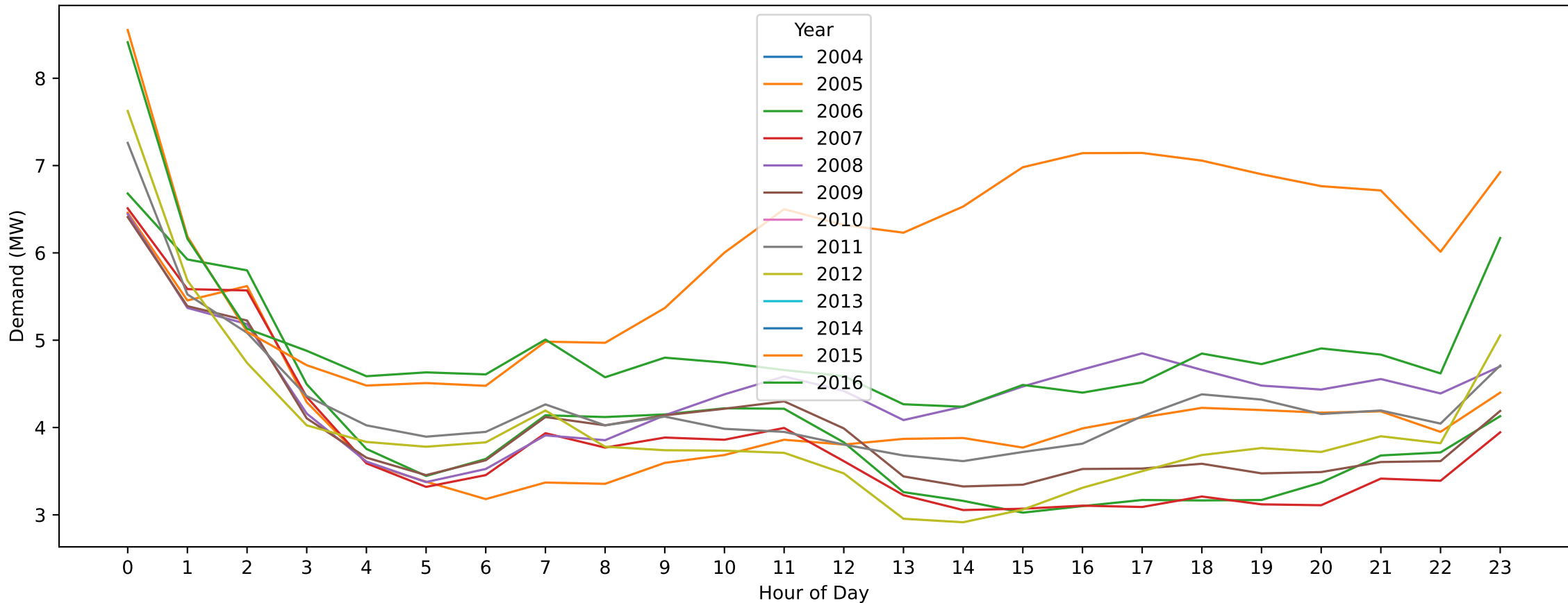
Nhill — Christmas Day (Hourly Demand Across Years)
