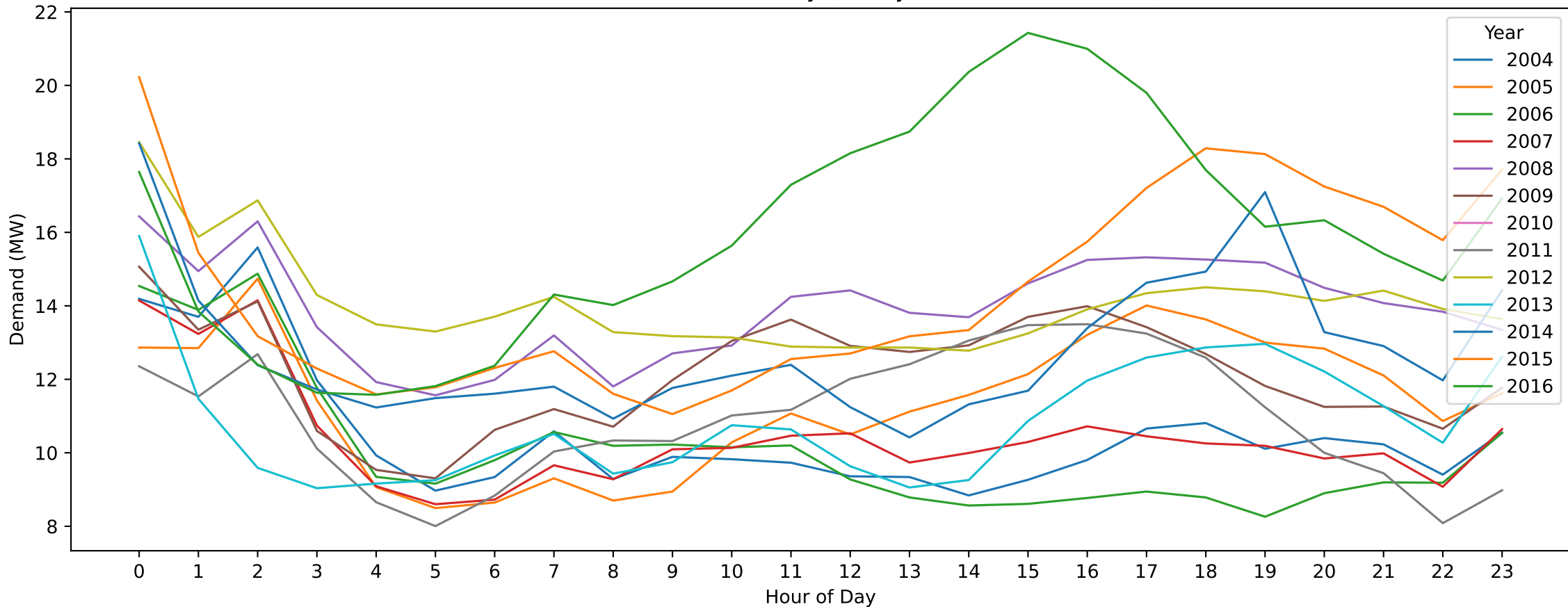
Cobram East — Christmas Day (Hourly Demand Across Years)
