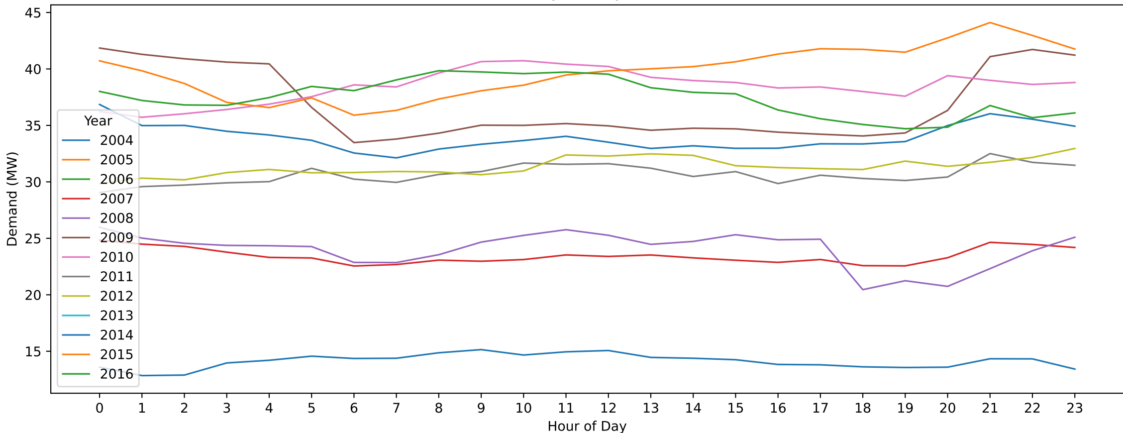
LVN22 — Christmas Day (Hourly Demand Across Years)
