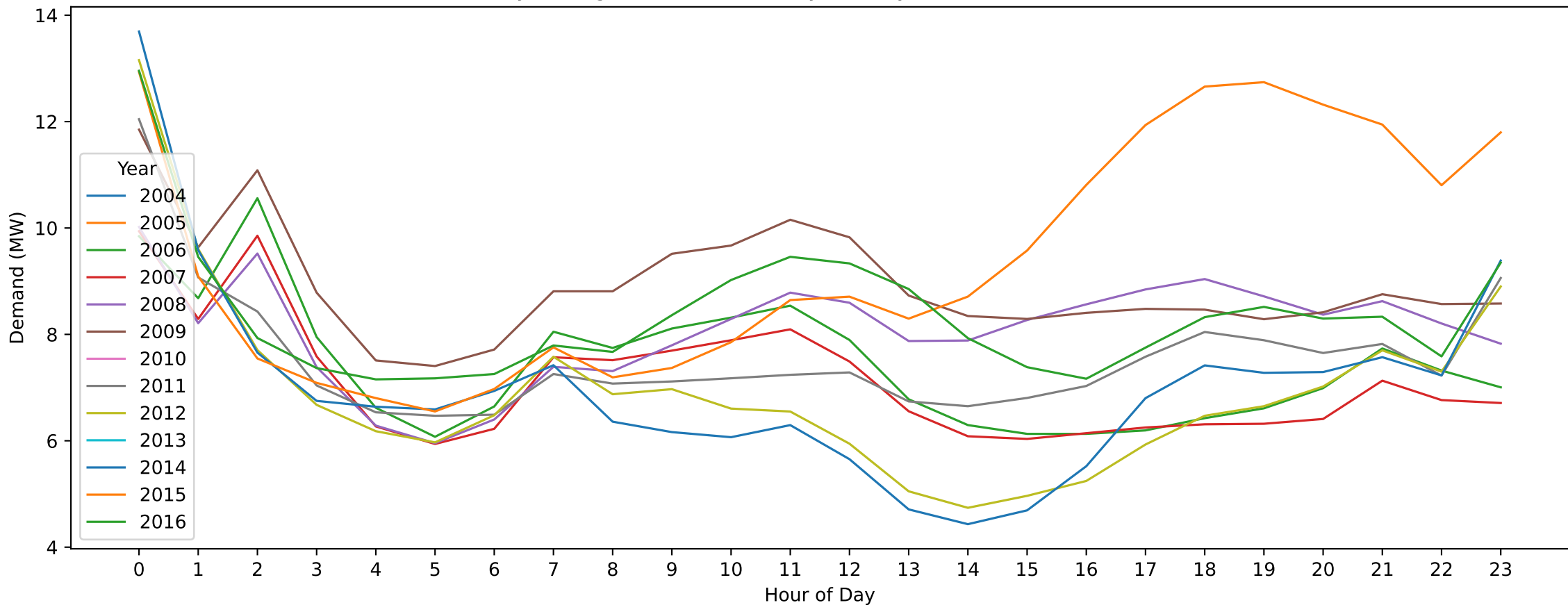
Maryborough — Christmas Day (Hourly Demand Across Years)
