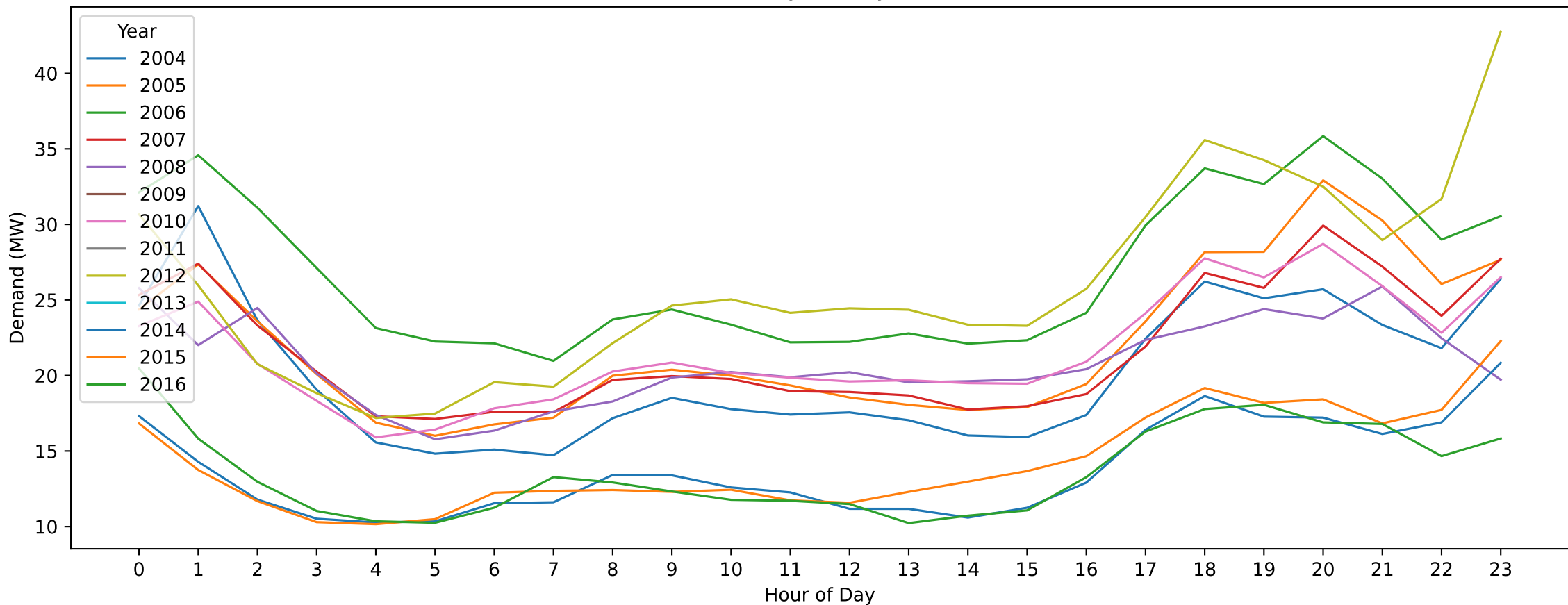
Woodend — Easter Monday (Hourly Demand Across Years)
