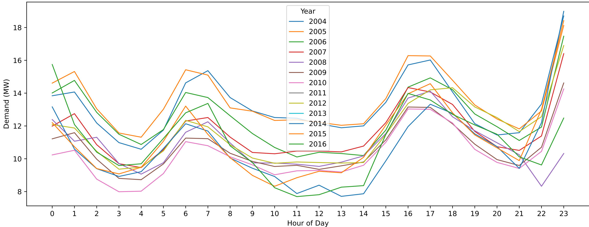
Kyabrym — Easter Monday (Hourly Demand Across Years)
