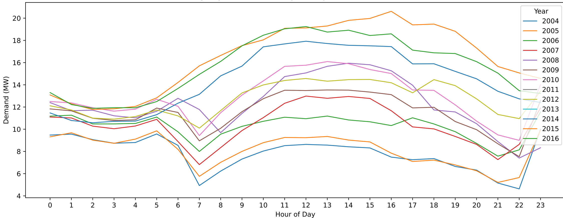
Geelong City — Easter Monday (Hourly Demand Across Years)
