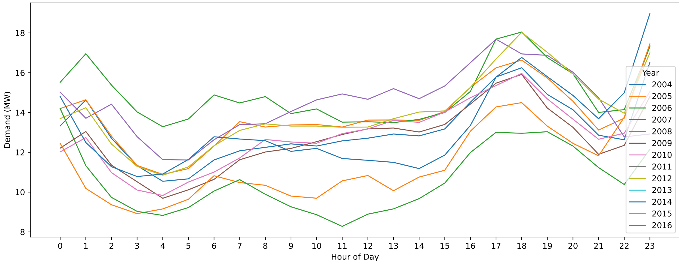
Shepparton Nth — Easter Monday (Hourly Demand Across Years)
