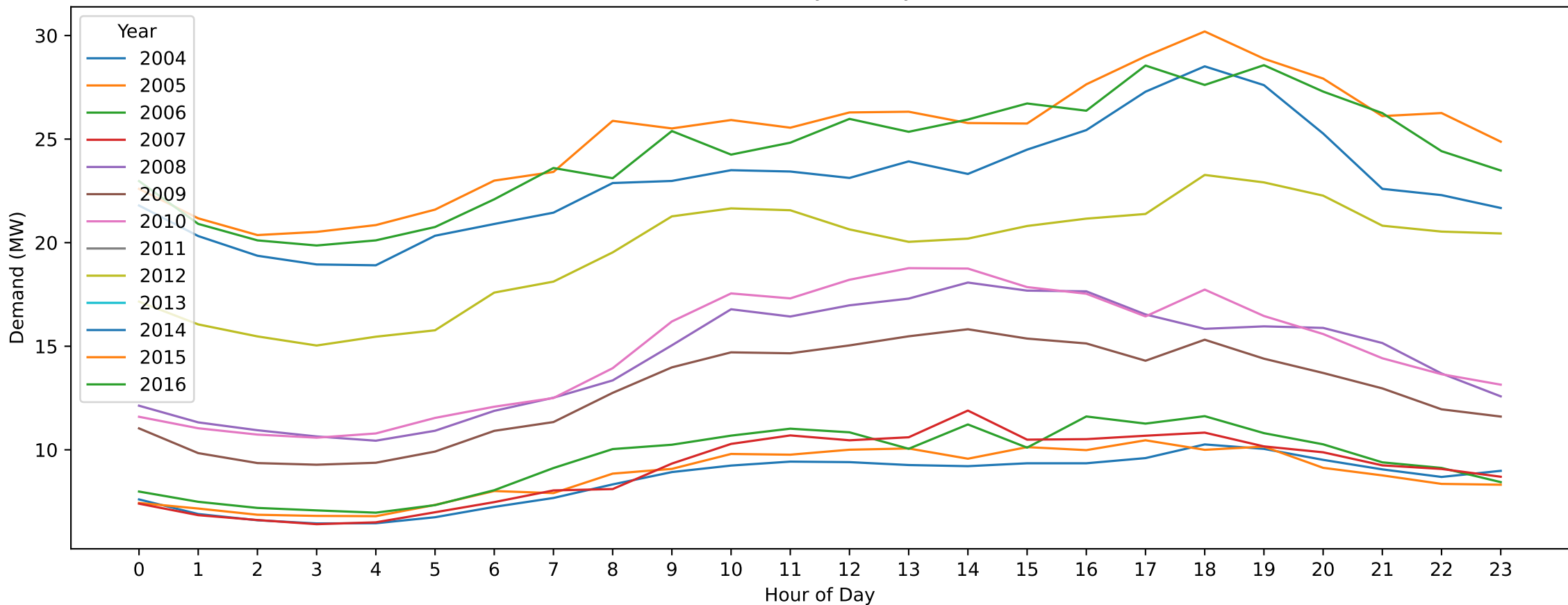
Sunshine East — Easter Monday (Hourly Demand Across Years)
