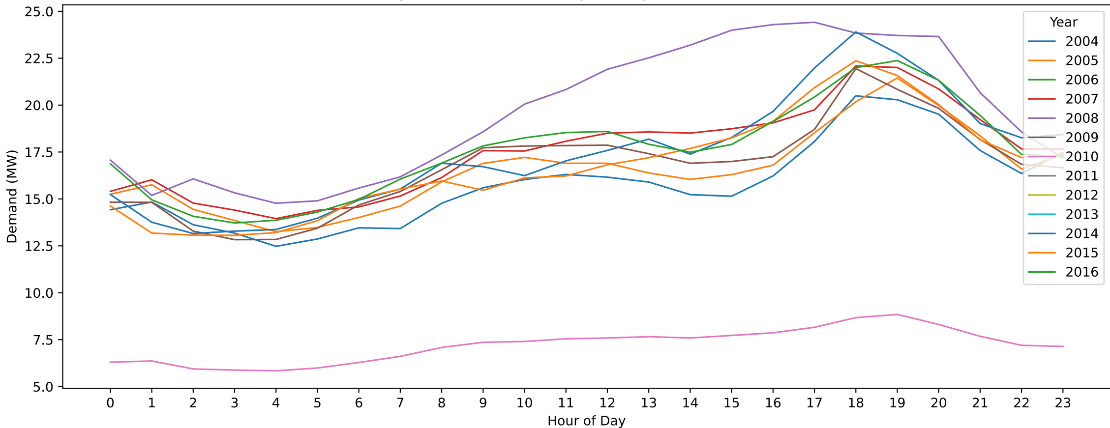
Geelong East — Easter Monday (Hourly Demand Across Years)
