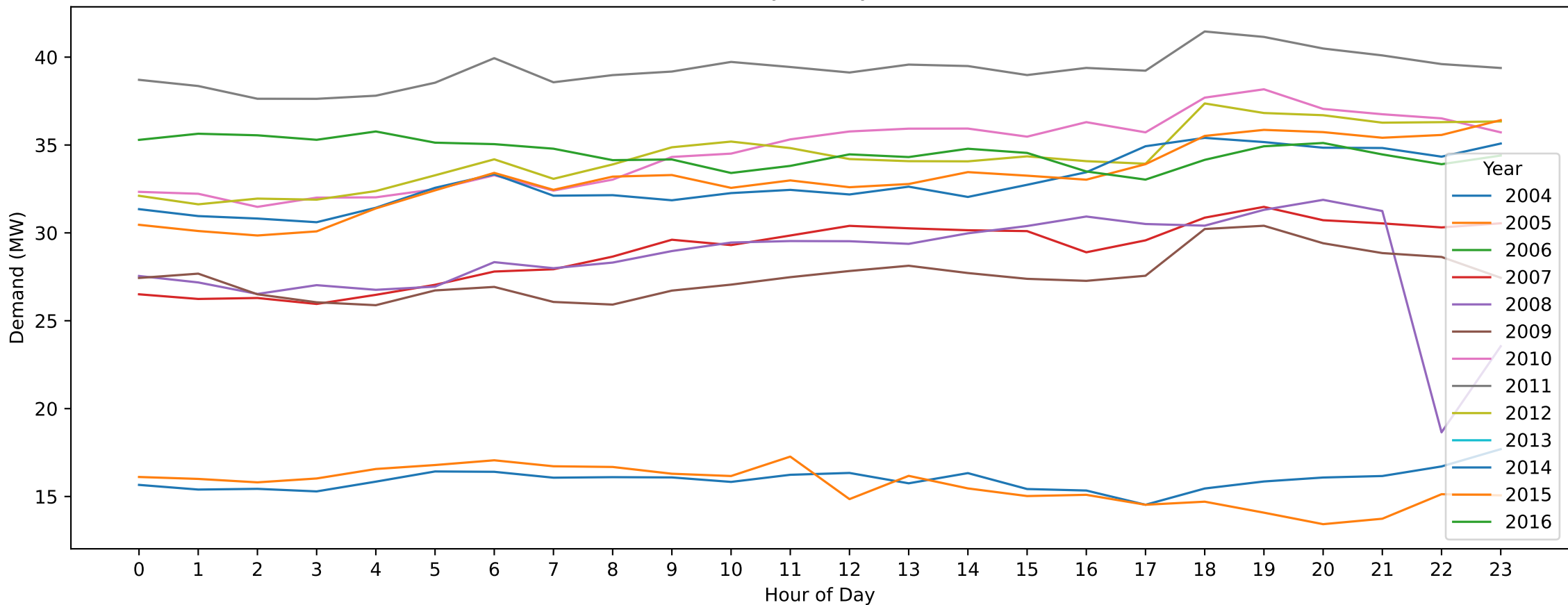
LVN22 — Easter Monday (Hourly Demand Across Years)
