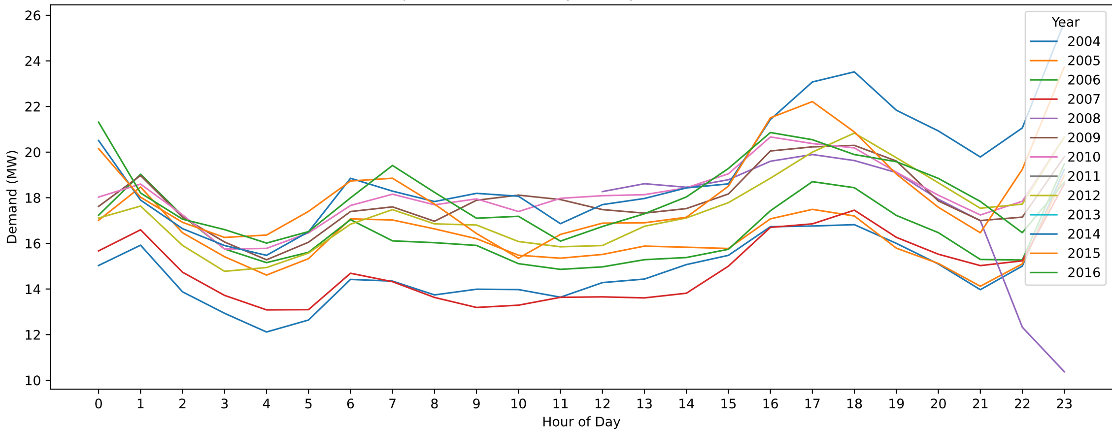
Mooroopna — Easter Monday (Hourly Demand Across Years)
