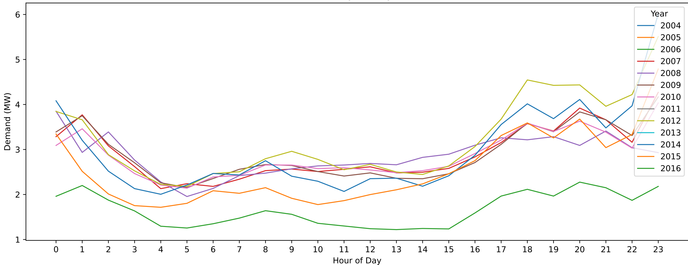
Winchelsea — Easter Monday (Hourly Demand Across Years)
