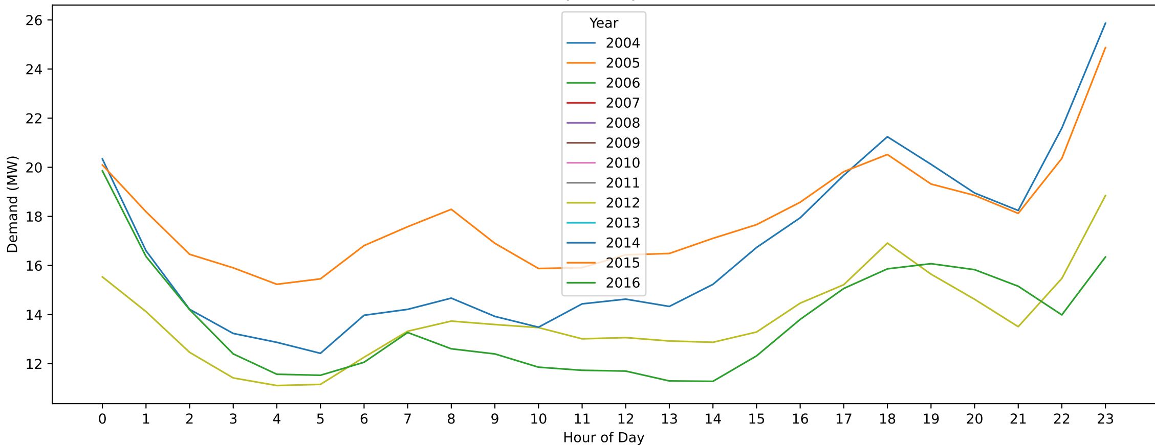
Koroit — Easter Monday (Hourly Demand Across Years)
