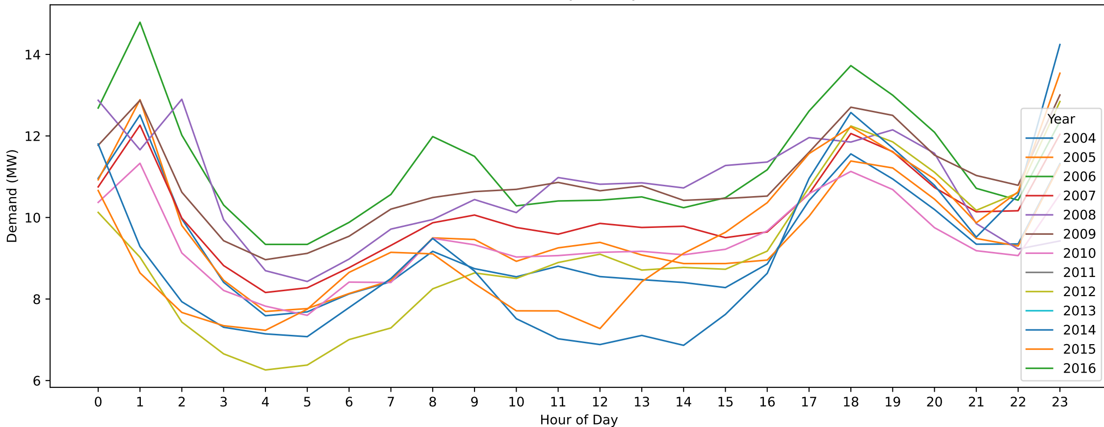
Castlemaine — Easter Monday (Hourly Demand Across Years)
