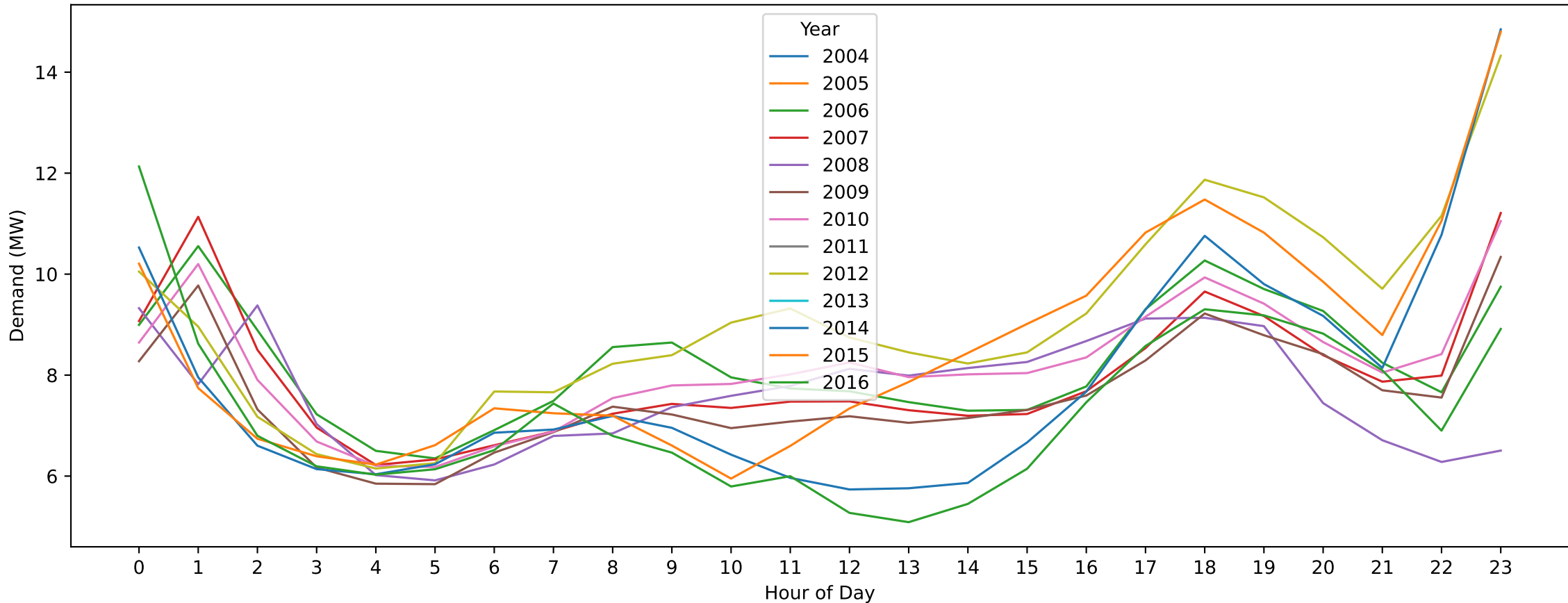
Maryborough — Easter Monday (Hourly Demand Across Years)
