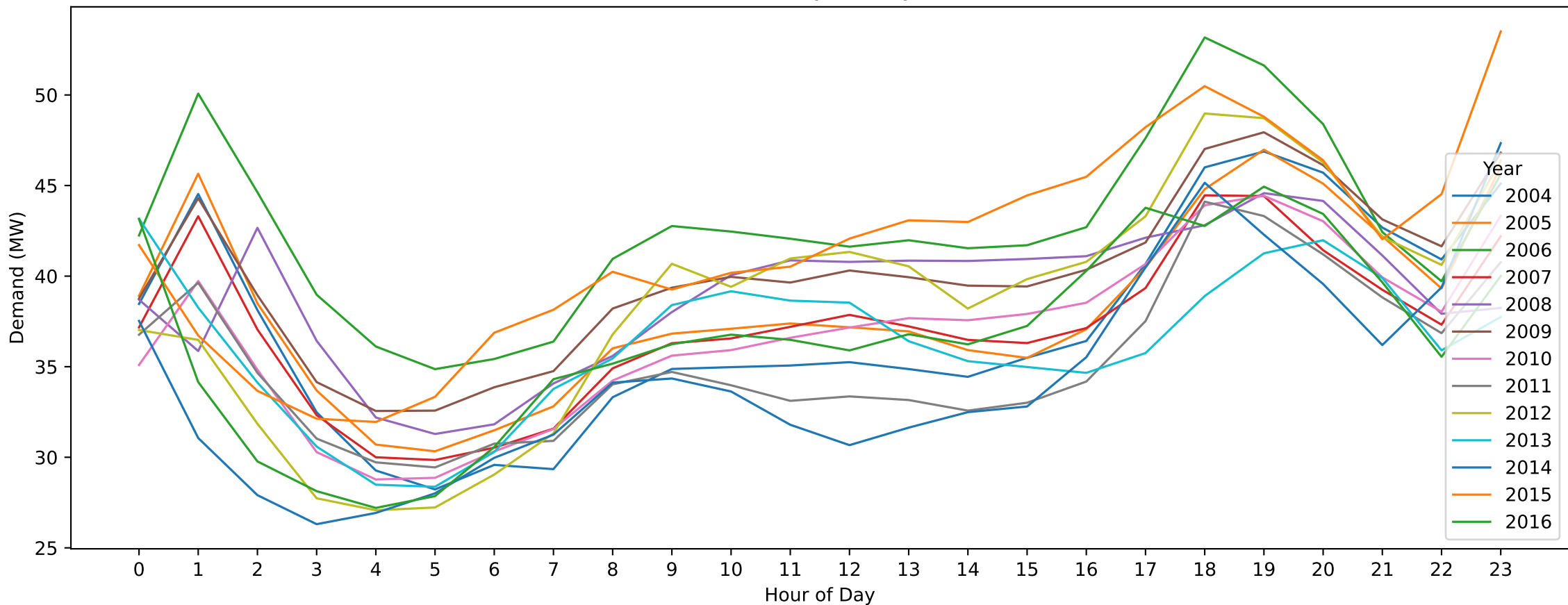
Ballarat North — Easter Monday (Hourly Demand Across Years)
