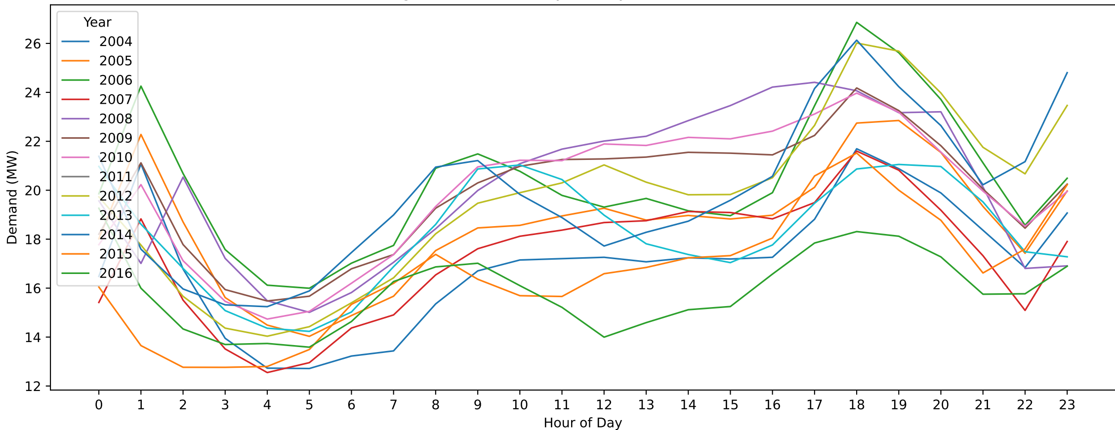
Bendigo — Easter Monday (Hourly Demand Across Years)
