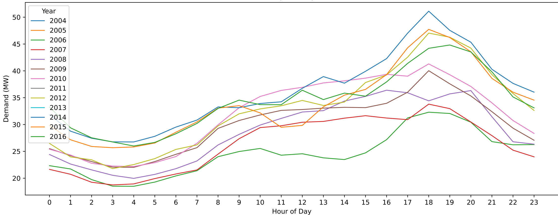
Werribee — Easter Monday (Hourly Demand Across Years)
