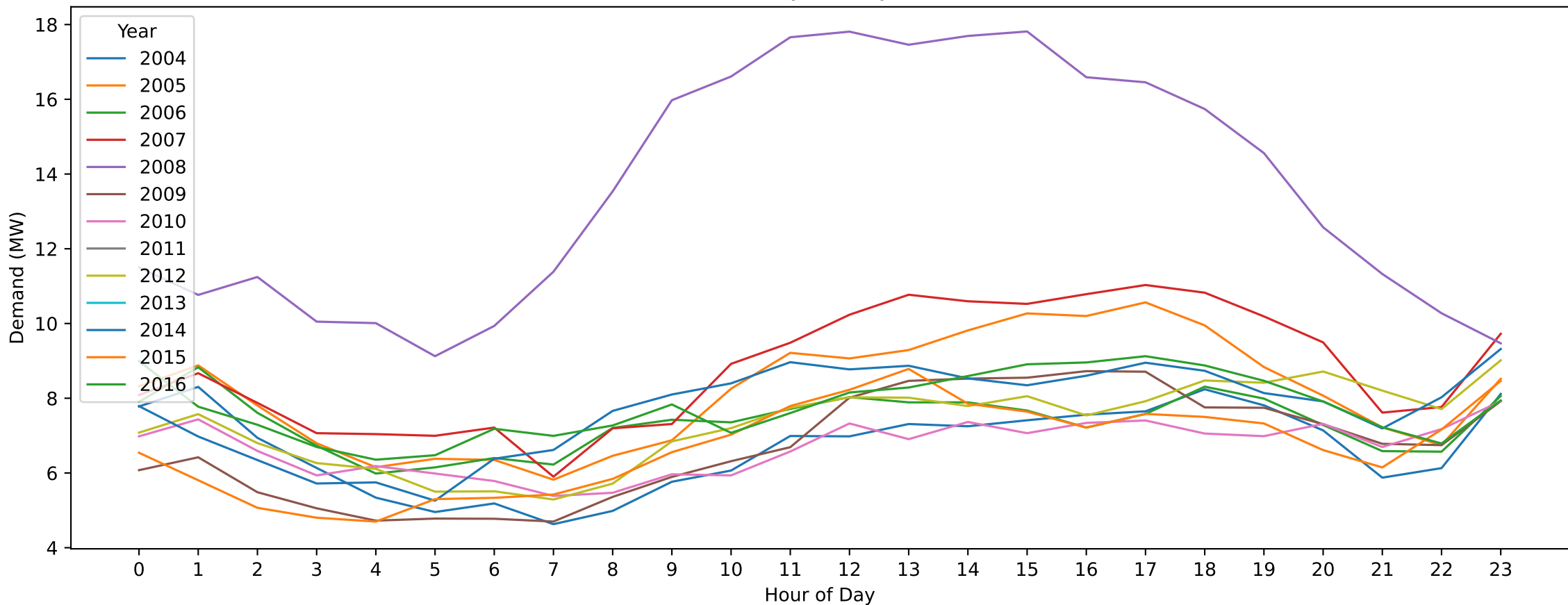
Robinvale — Easter Monday (Hourly Demand Across Years)
