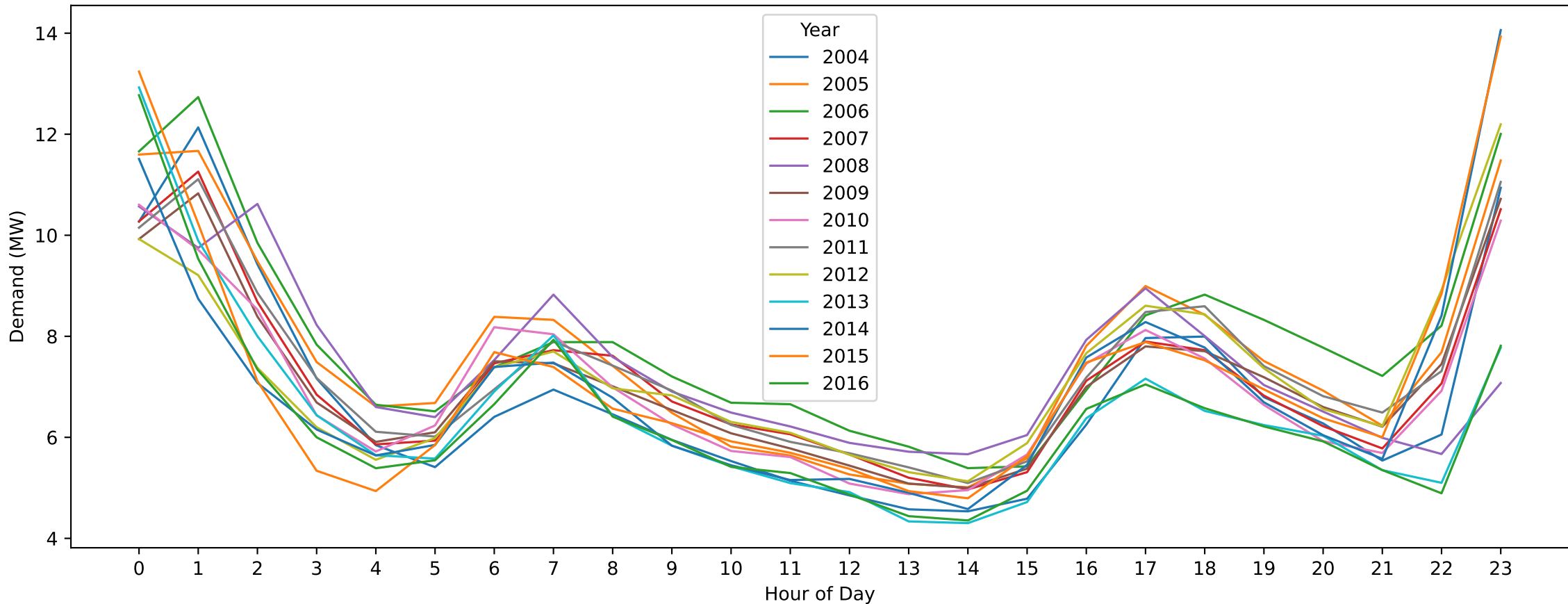
Camperdown — Easter Sunday (Hourly Demand Across Years)
