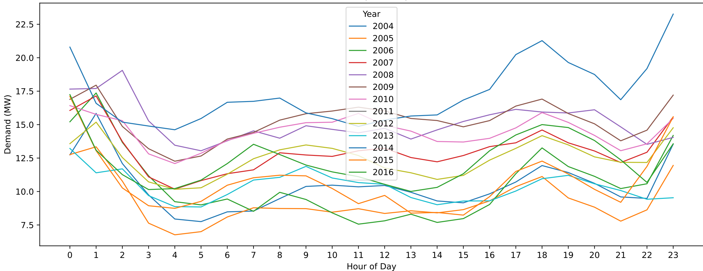
Cobram East — Easter Sunday (Hourly Demand Across Years)
