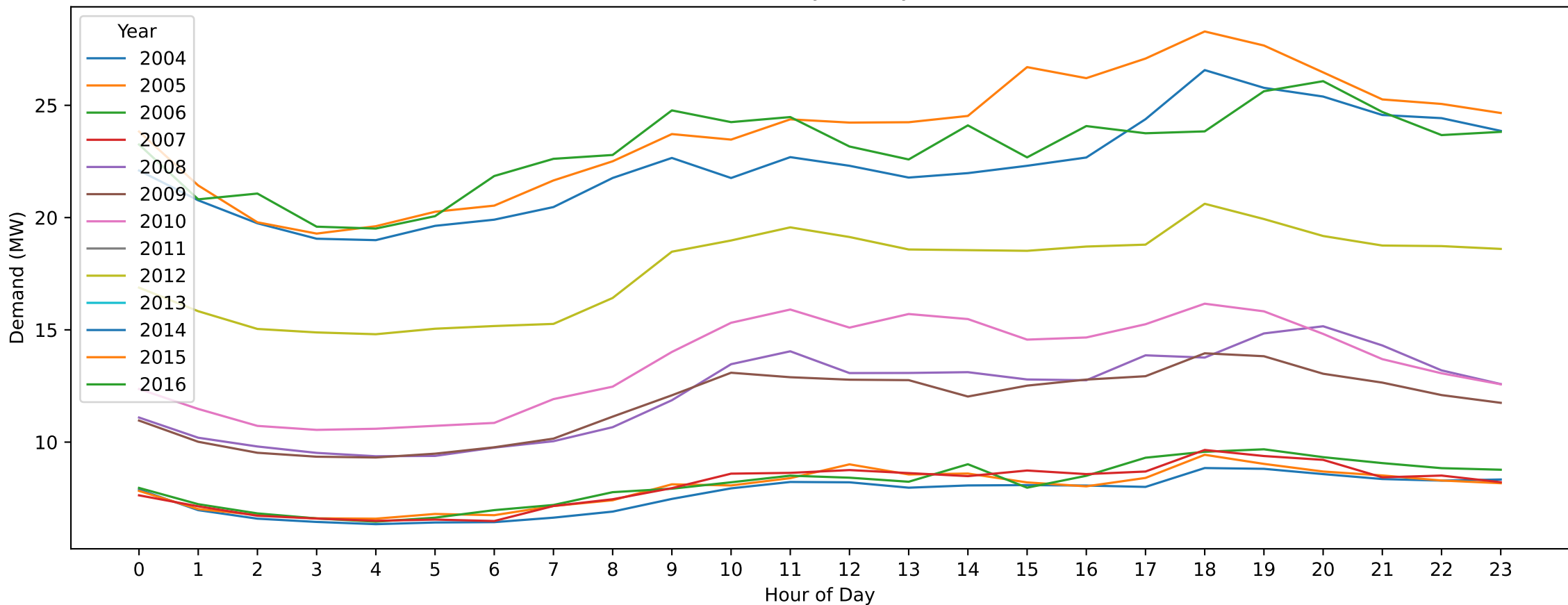
Sunshine East — Easter Sunday (Hourly Demand Across Years)
