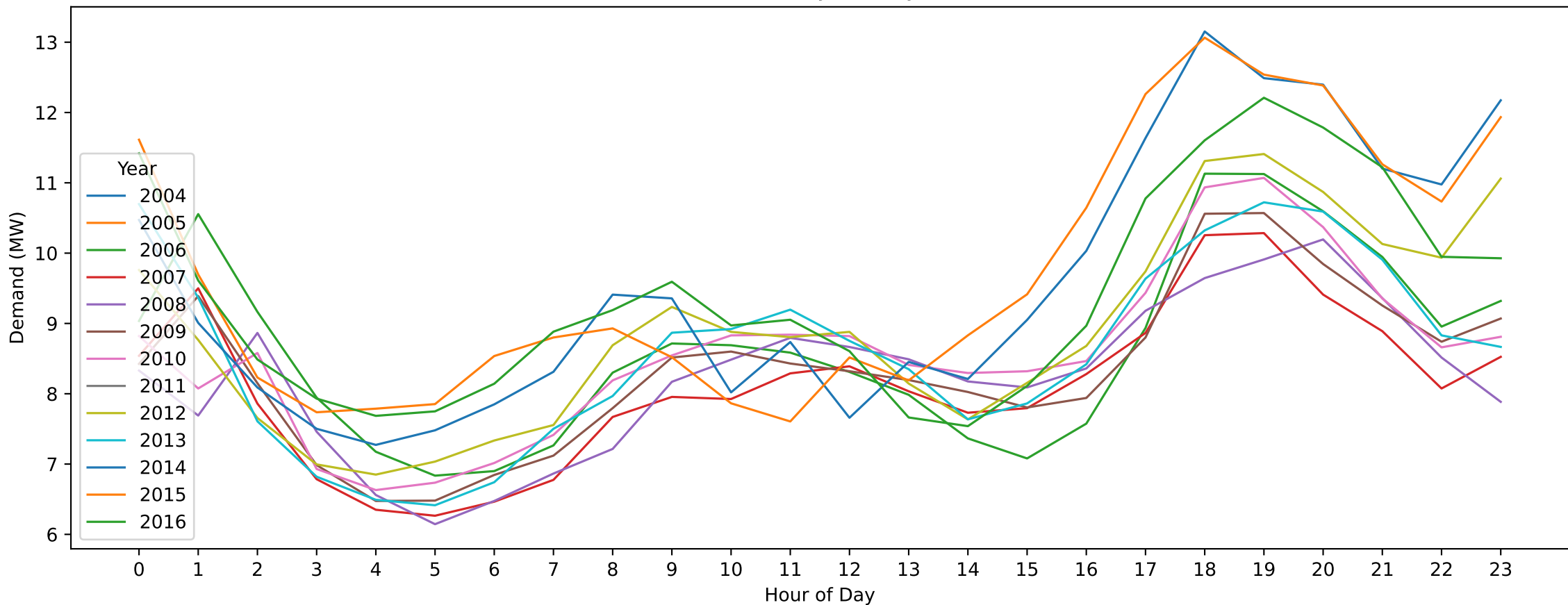
Bacchus Marsh — Easter Sunday (Hourly Demand Across Years)
