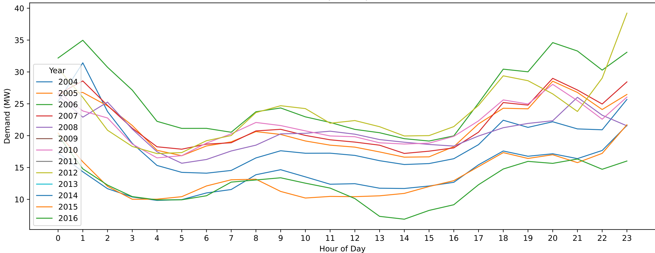
Woodend — Easter Sunday (Hourly Demand Across Years)
