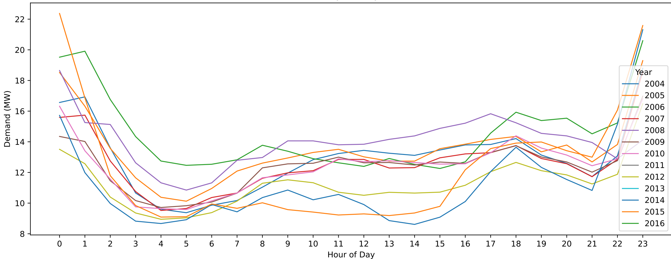
Swan Hill — Easter Sunday (Hourly Demand Across Years)
