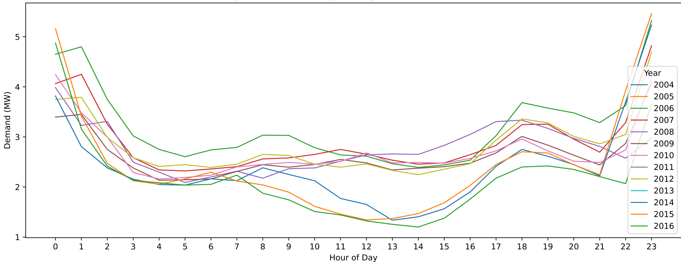
Ouyen — Easter Sunday (Hourly Demand Across Years)
