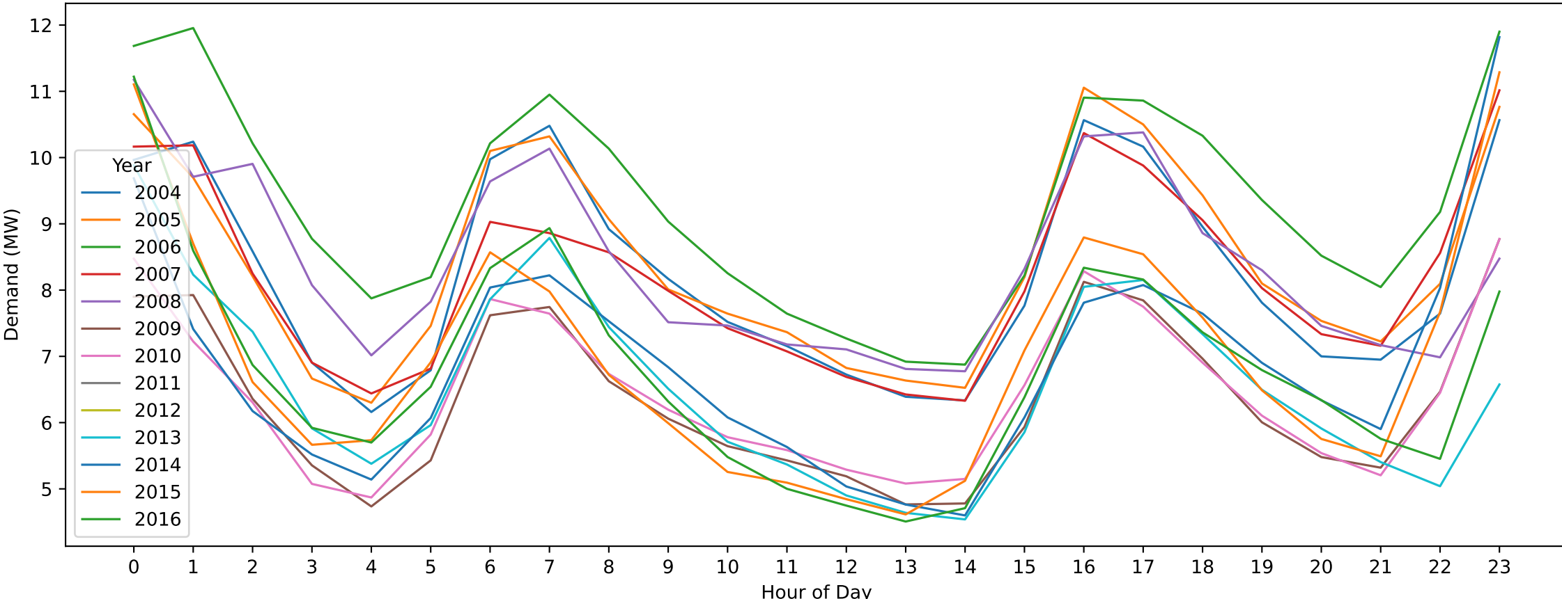
Cohuna — Easter Sunday (Hourly Demand Across Years)
