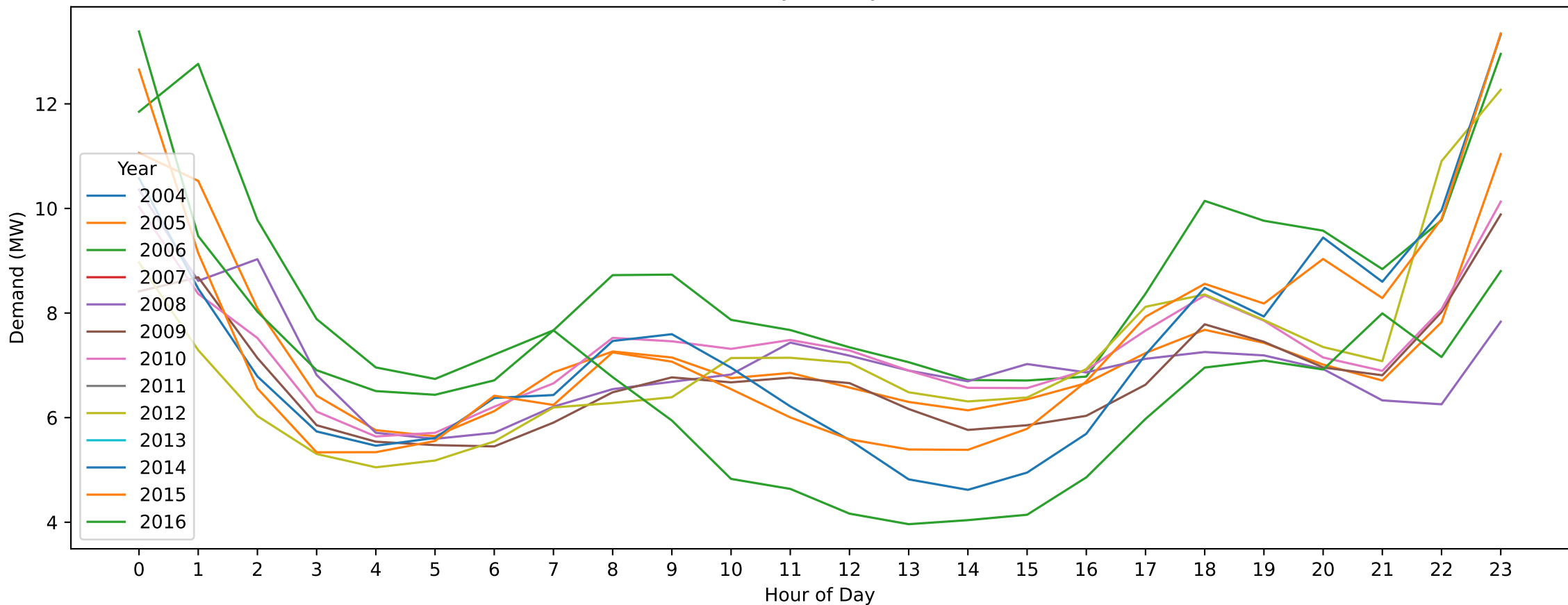
Charlton — Easter Sunday (Hourly Demand Across Years)
