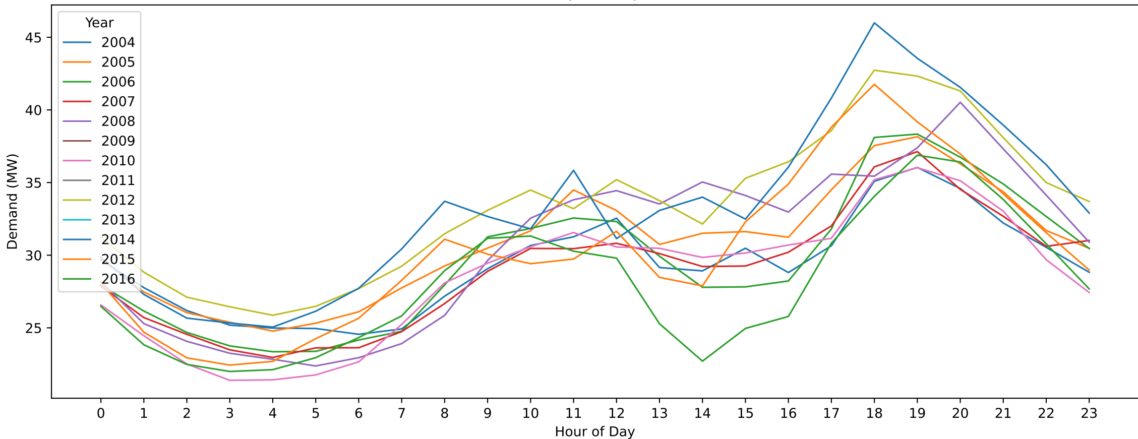
Laverton — Easter Sunday (Hourly Demand Across Years)
