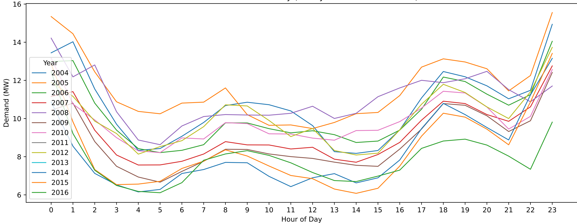
Portland — Easter Sunday (Hourly Demand Across Years)
