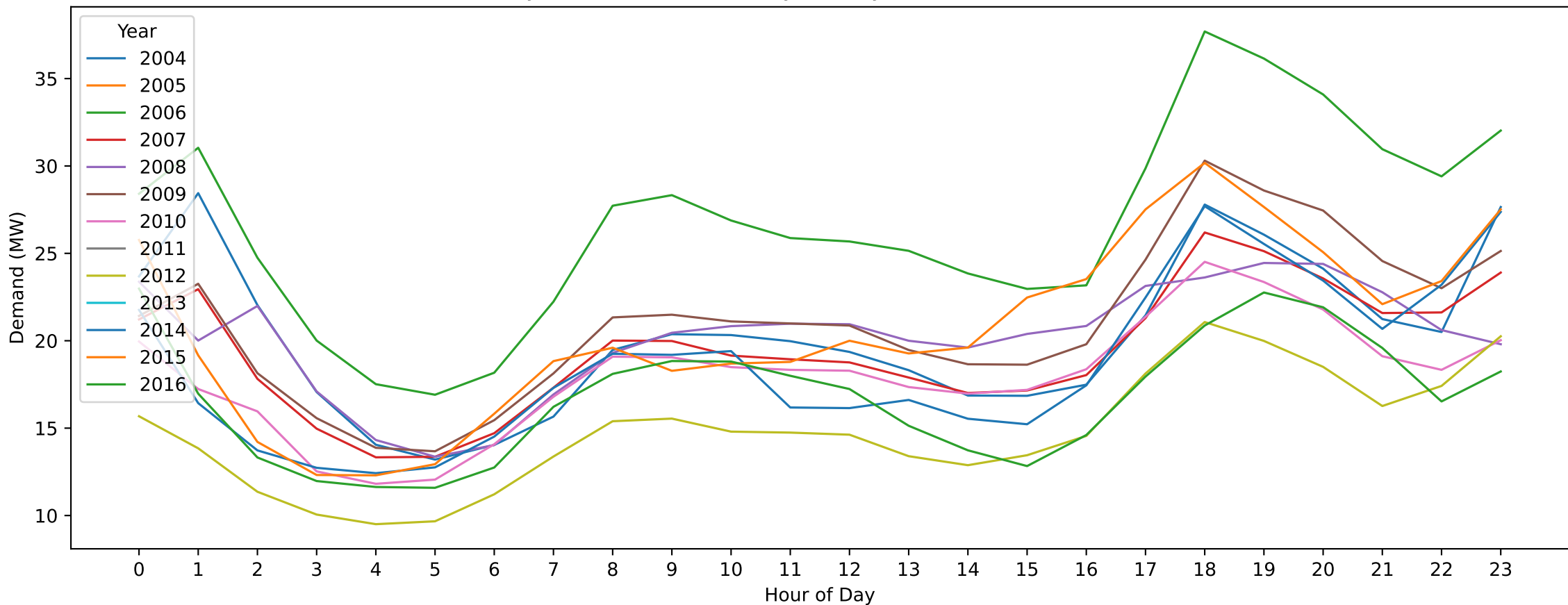
Drysdale — Easter Sunday (Hourly Demand Across Years)
