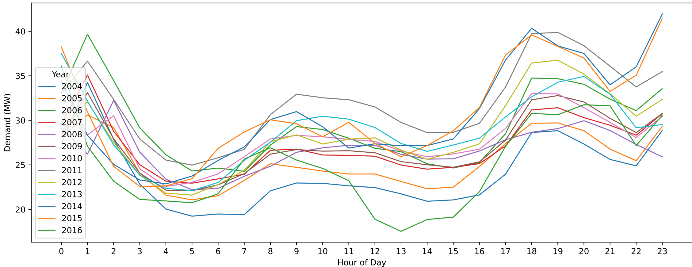
Ballarat South — Easter Sunday (Hourly Demand Across Years)
