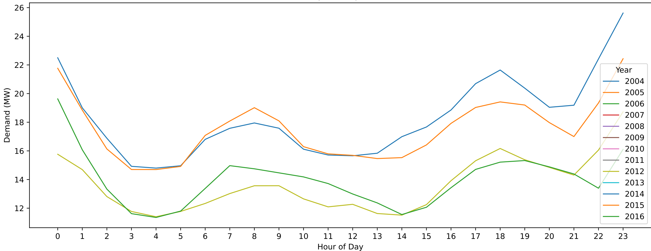
Koroit — Easter Sunday (Hourly Demand Across Years)
