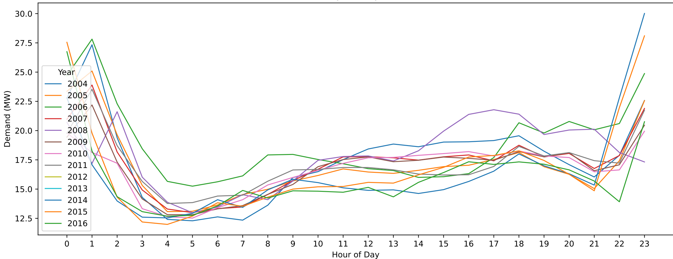
Mildura — Easter Sunday (Hourly Demand Across Years)
