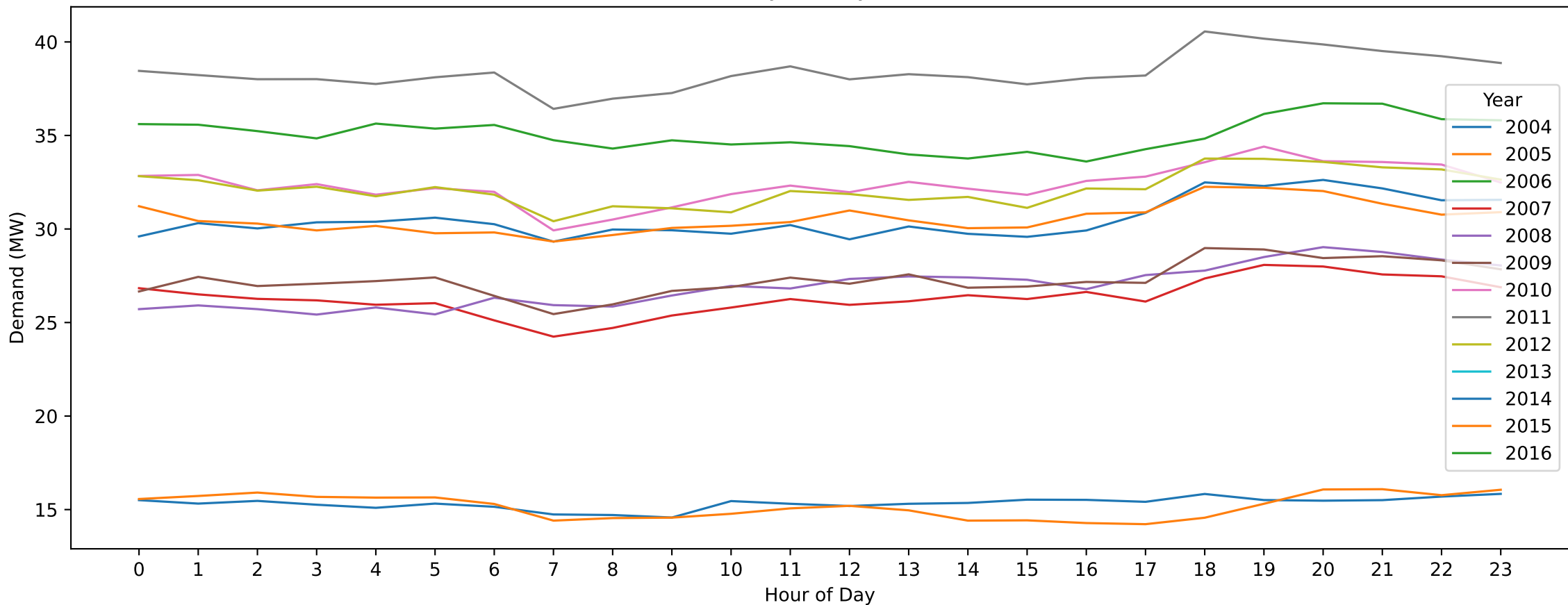
LVN22 — Easter Sunday (Hourly Demand Across Years)
