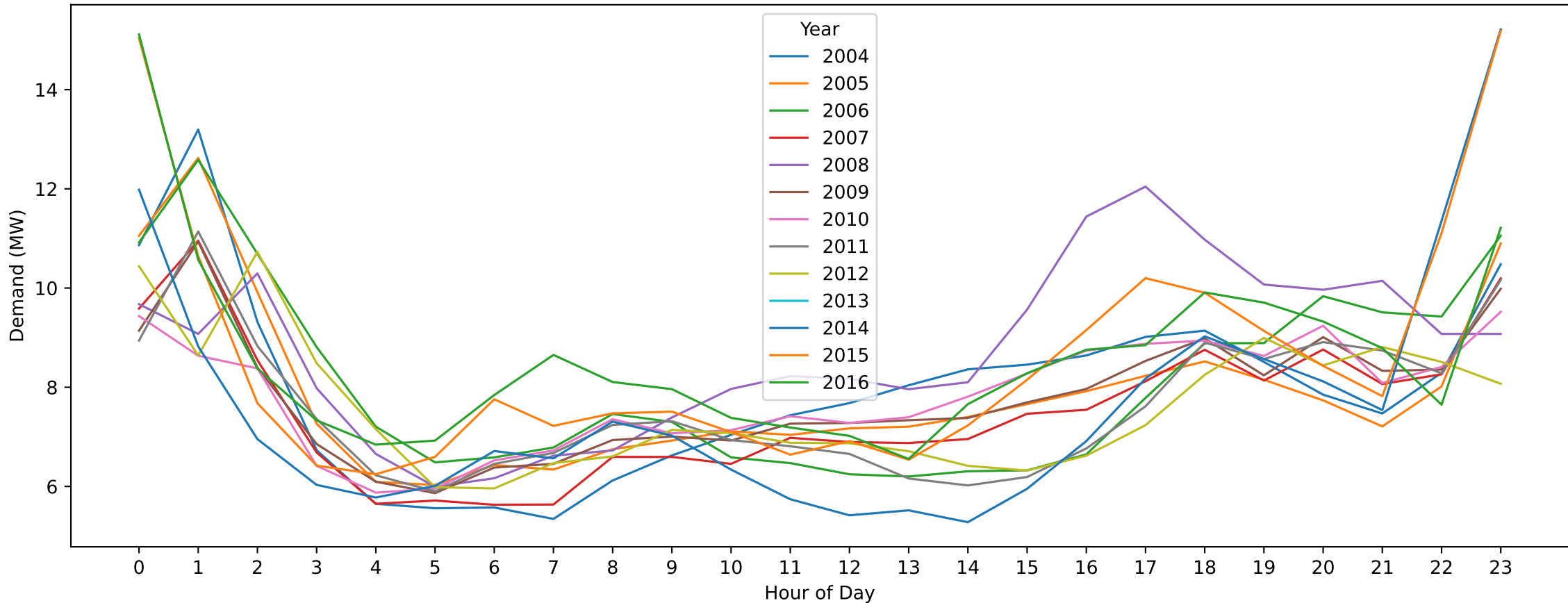
Merbein — Easter Sunday (Hourly Demand Across Years)
