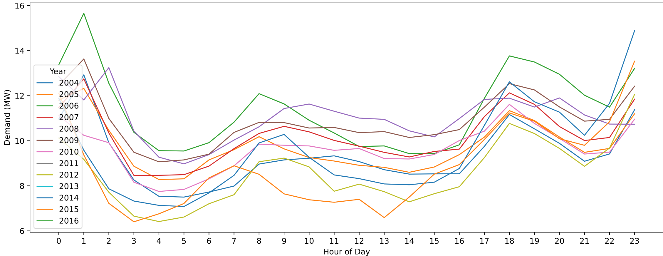
Castlemaine — Easter Sunday (Hourly Demand Across Years)
