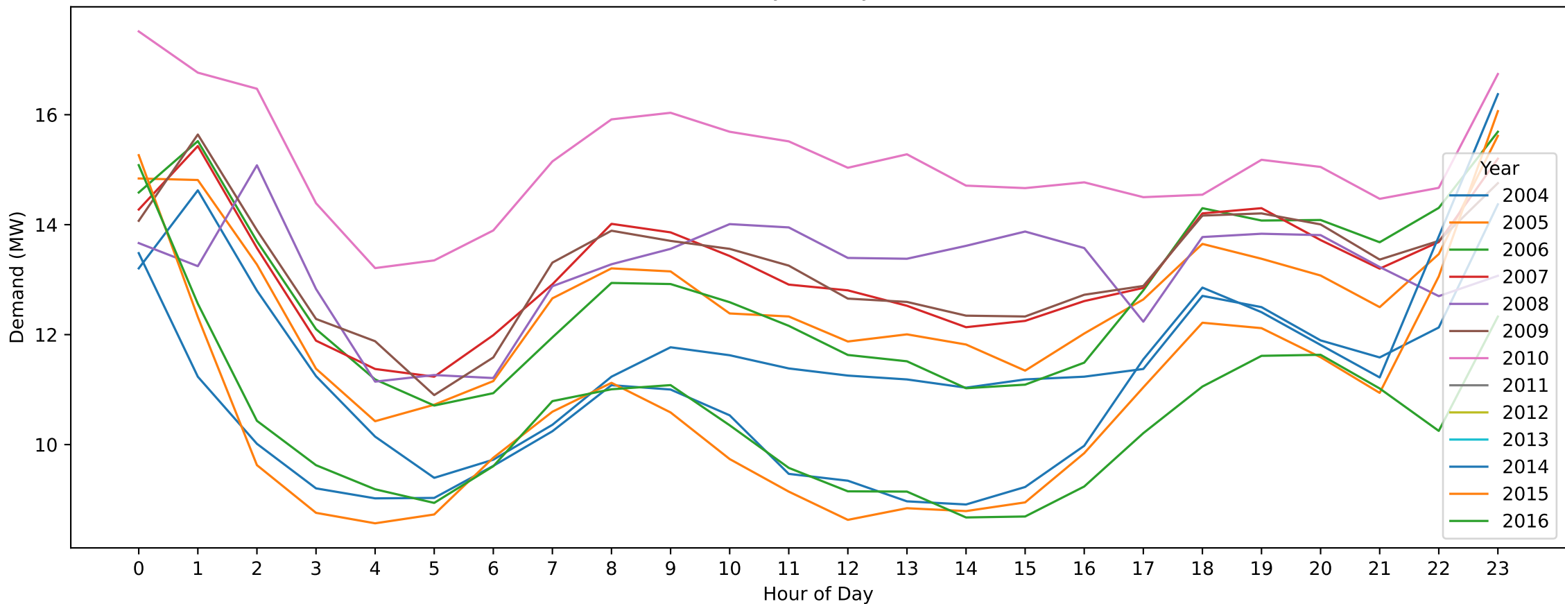
Stawell — Easter Sunday (Hourly Demand Across Years)
