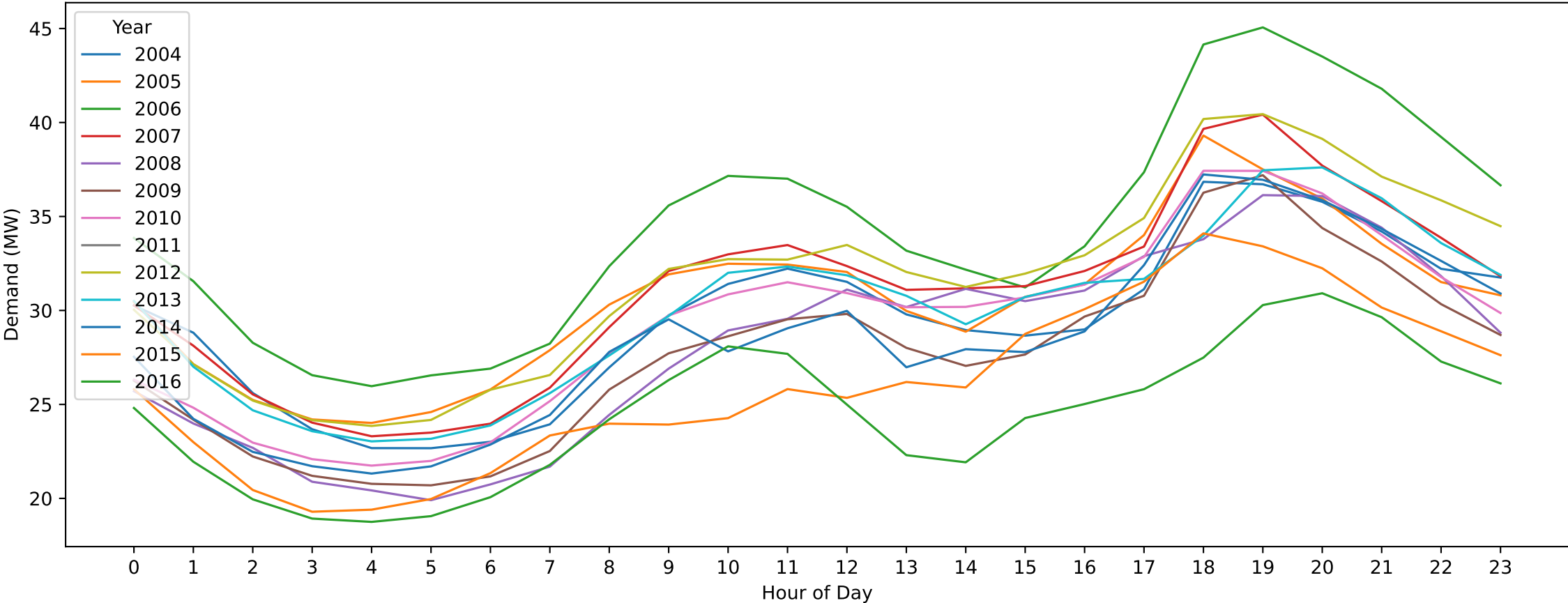
St Albans — Easter Sunday (Hourly Demand Across Years)
