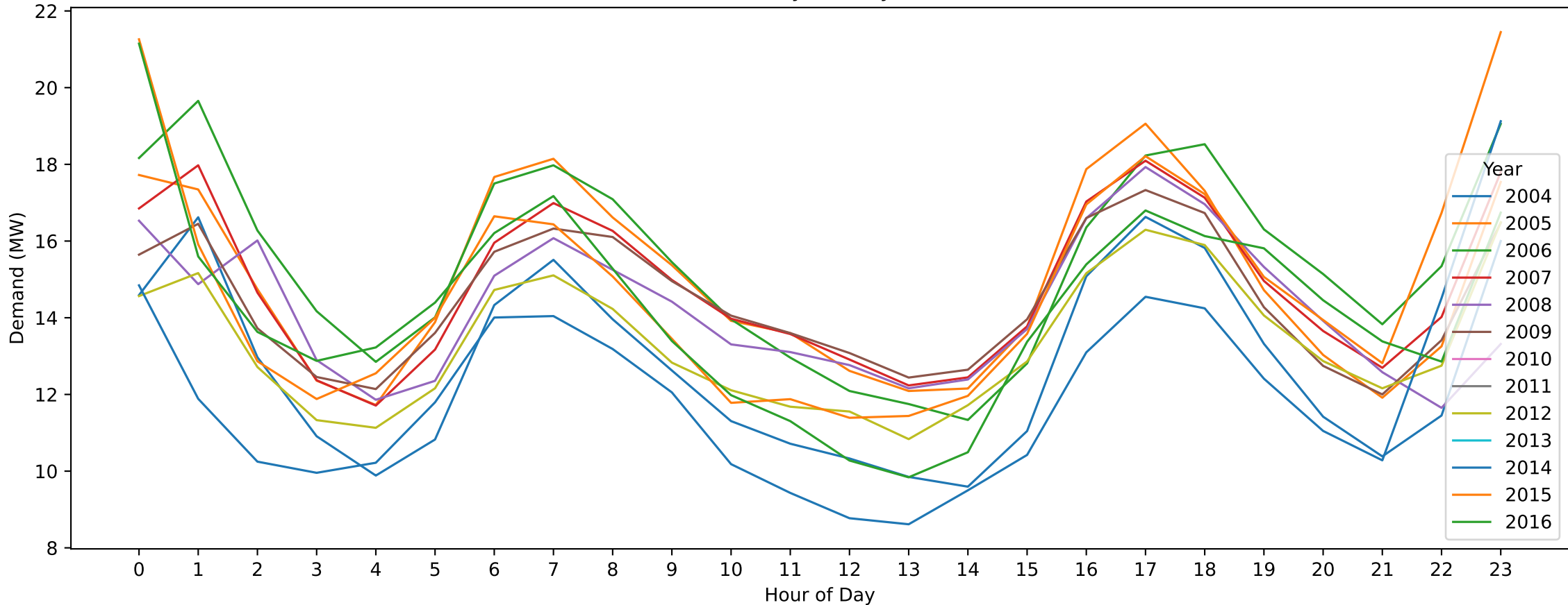
Numurkah — Easter Sunday (Hourly Demand Across Years)
