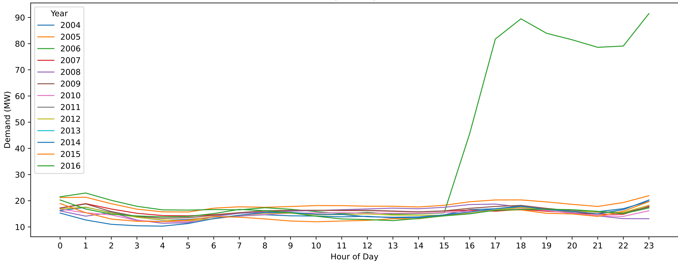
Echuca — Easter Sunday (Hourly Demand Across Years)
