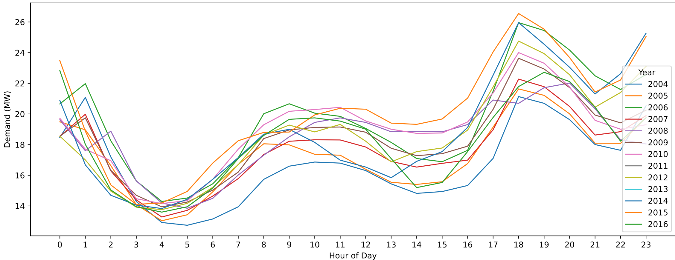
Geelong — Easter Sunday (Hourly Demand Across Years)
