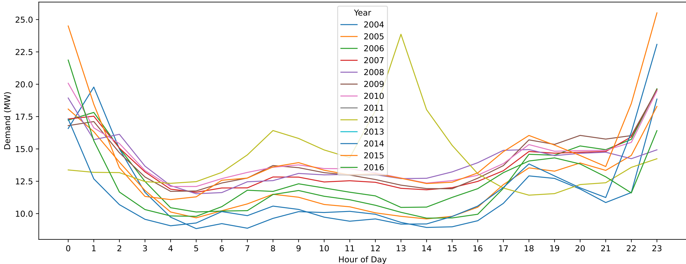
Hamilton — Easter Sunday (Hourly Demand Across Years)
