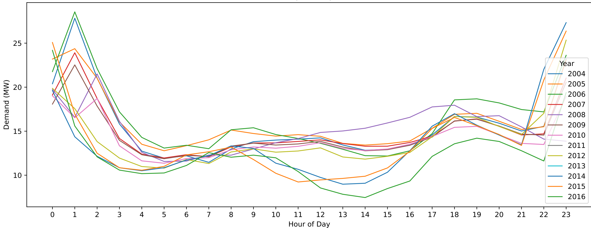
Horsham — Easter Sunday (Hourly Demand Across Years)
