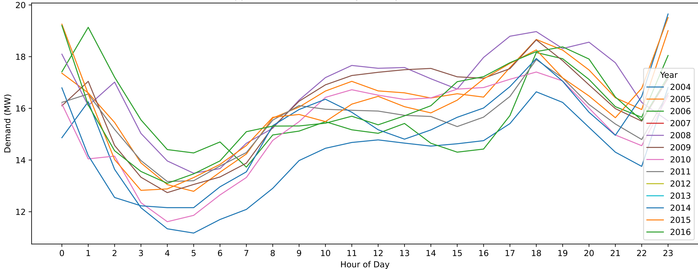
Shepparton — Easter Sunday (Hourly Demand Across Years)
