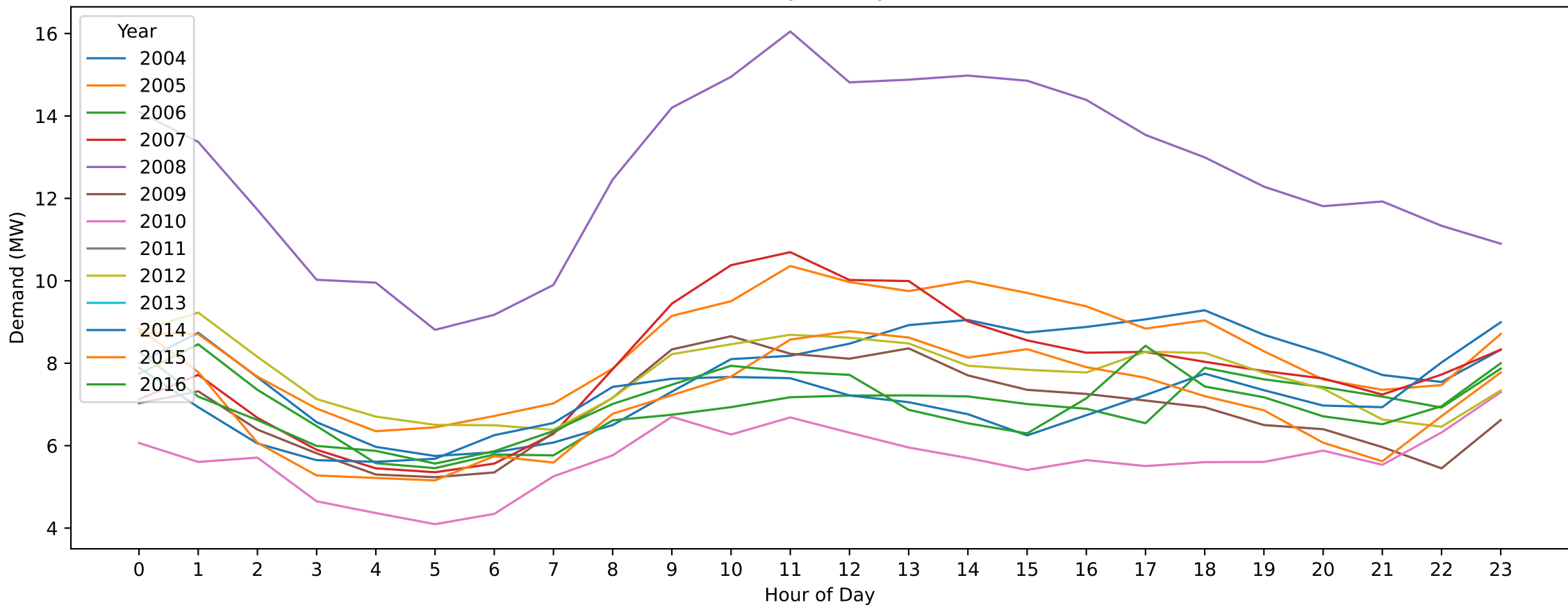
Robinvale — Easter Sunday (Hourly Demand Across Years)
