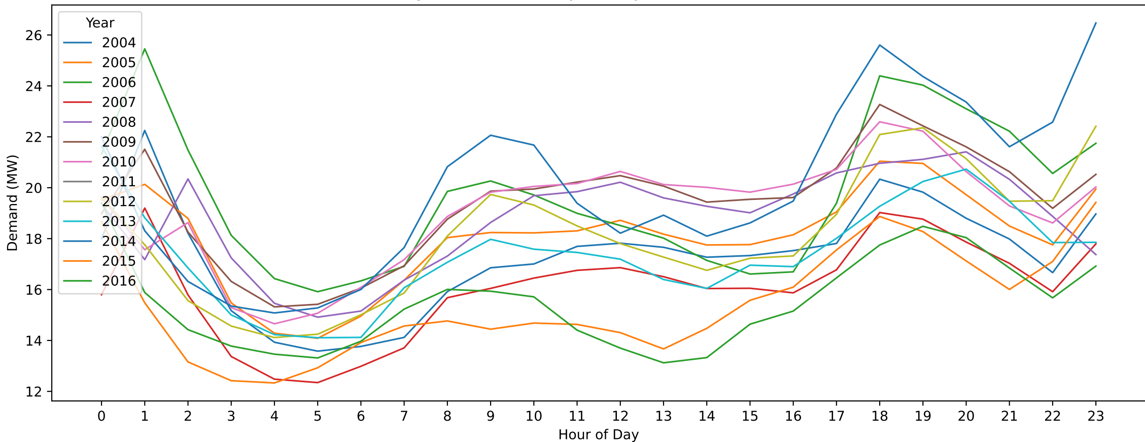
Bendigo — Easter Sunday (Hourly Demand Across Years)
