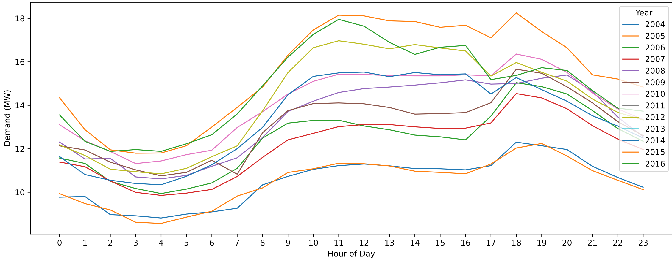
Geelong City — Easter Sunday (Hourly Demand Across Years)
