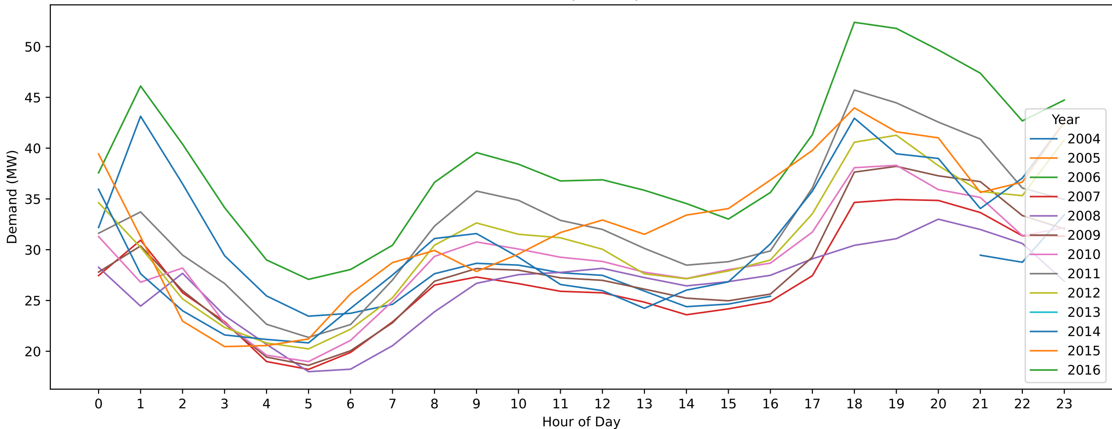
Waurn Ponds — Easter Sunday (Hourly Demand Across Years)
