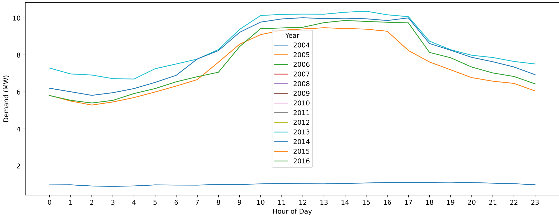
Docklands — Easter Sunday (Hourly Demand Across Years)
