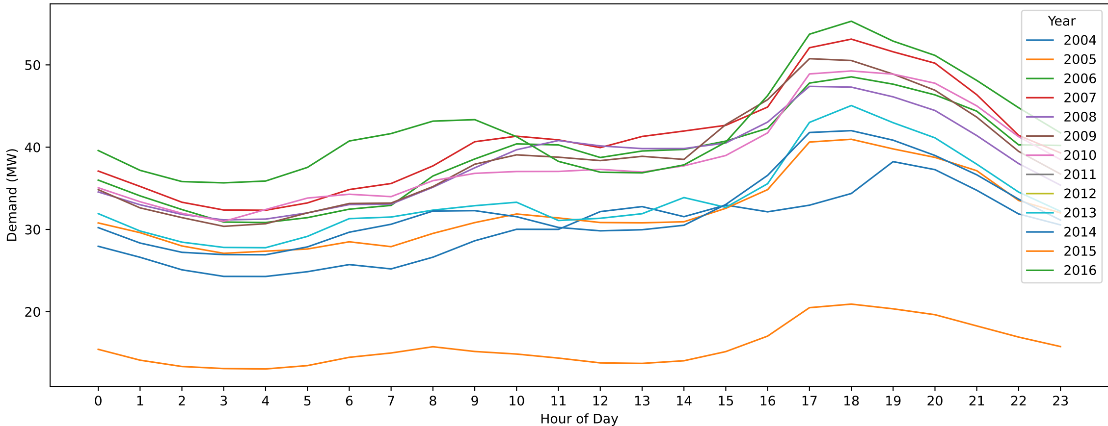
Sunshine — King's Birthday (Hourly Demand Across Years)
