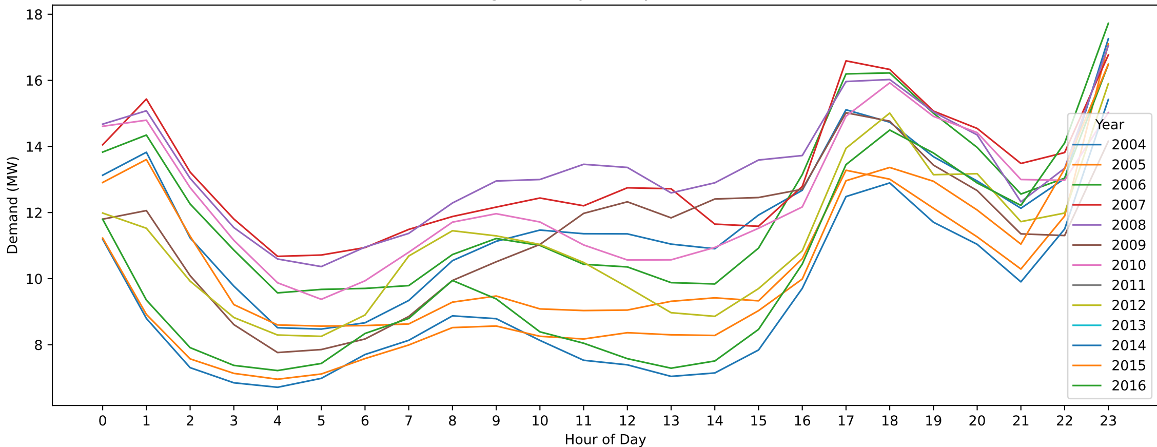
Portland — King's Birthday (Hourly Demand Across Years)
