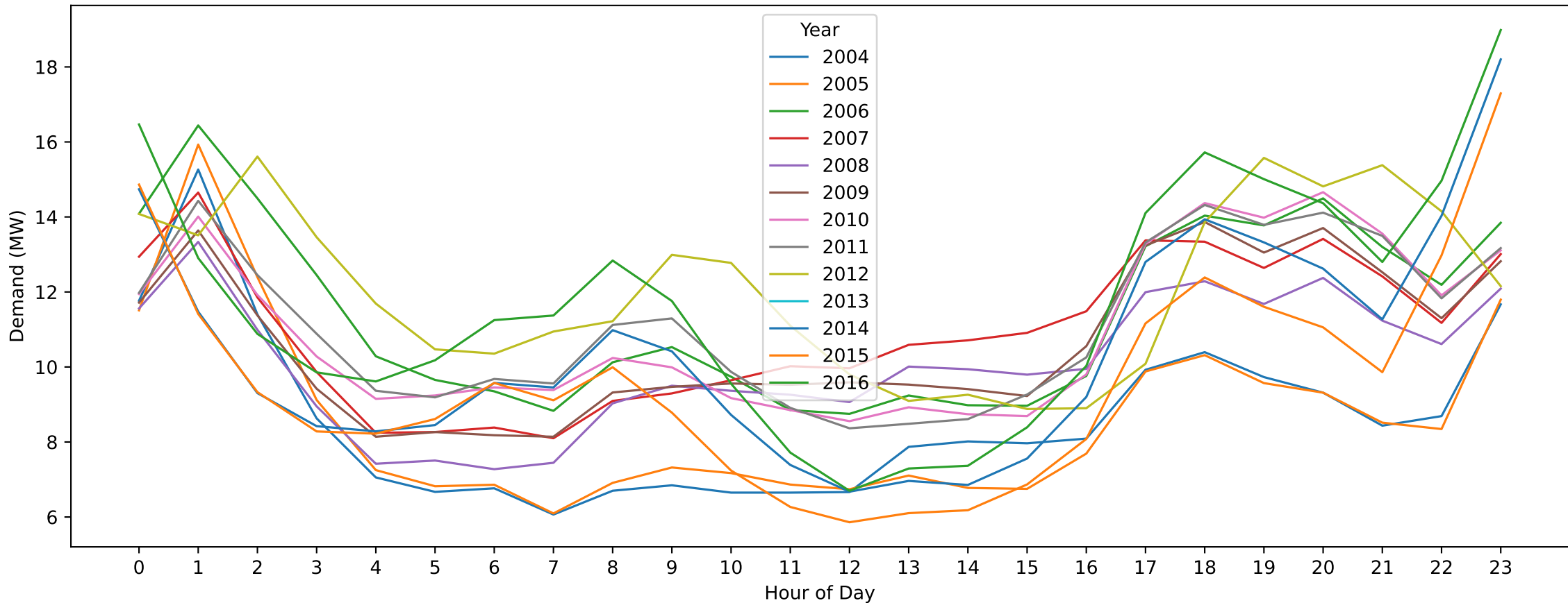
Merbein — King's Birthday (Hourly Demand Across Years)
