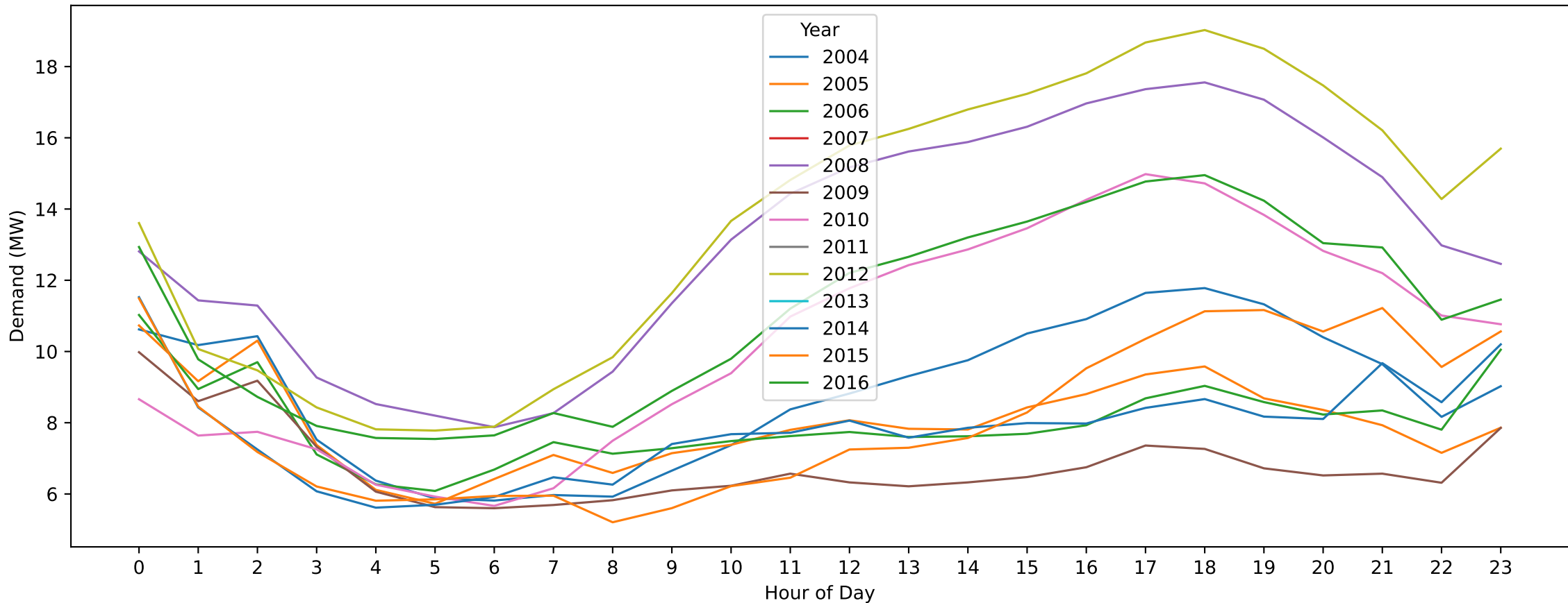
Charlton — New Year's Day (Hourly Demand Across Years)
