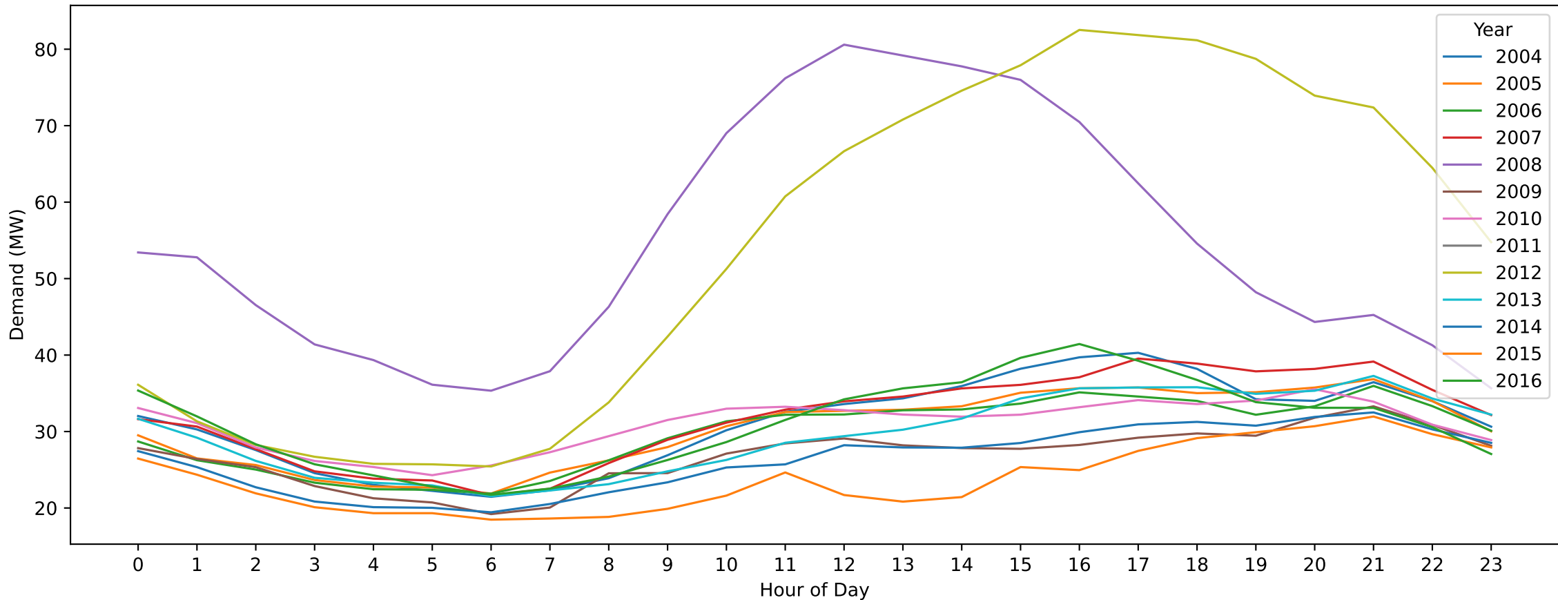
St Albans — New Year's Day (Hourly Demand Across Years)
