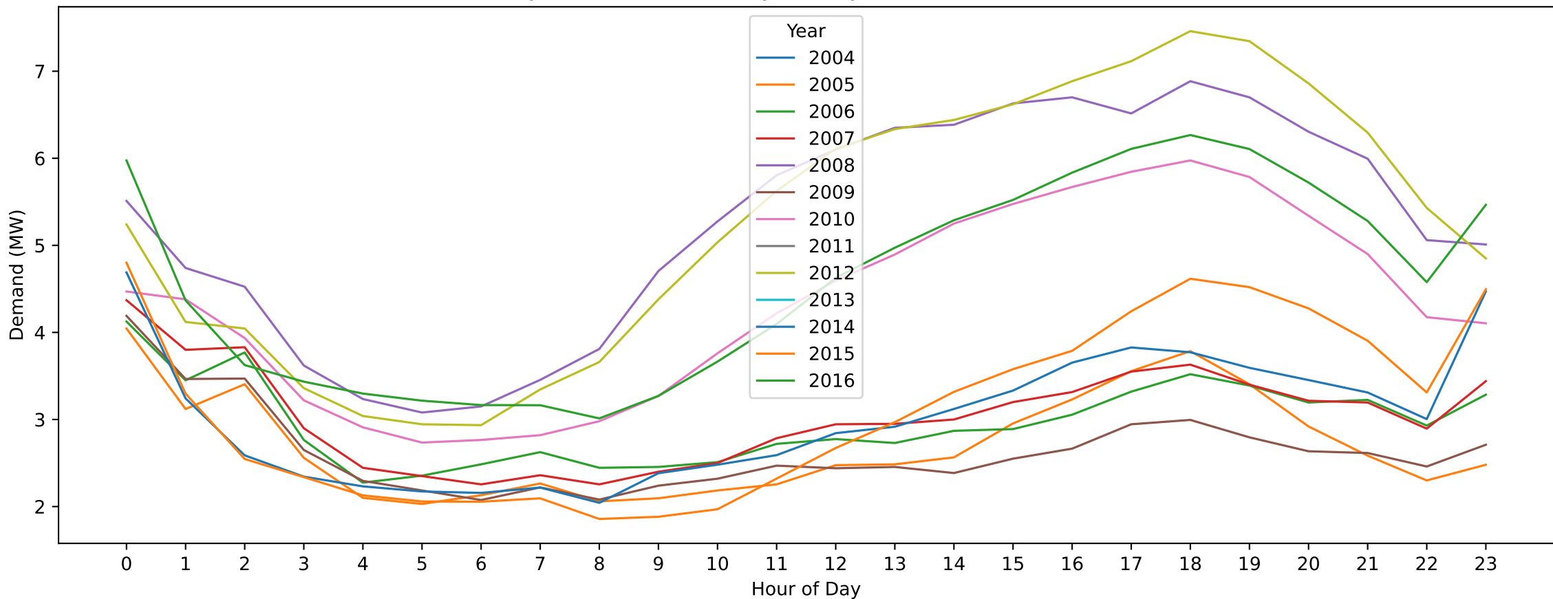
Ouyen — New Year's Day (Hourly Demand Across Years)
