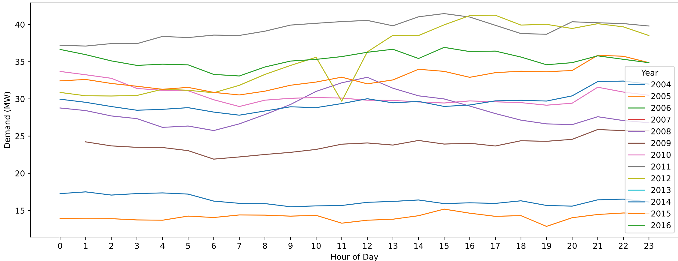
LVN22 — New Year's Day (Hourly Demand Across Years)
