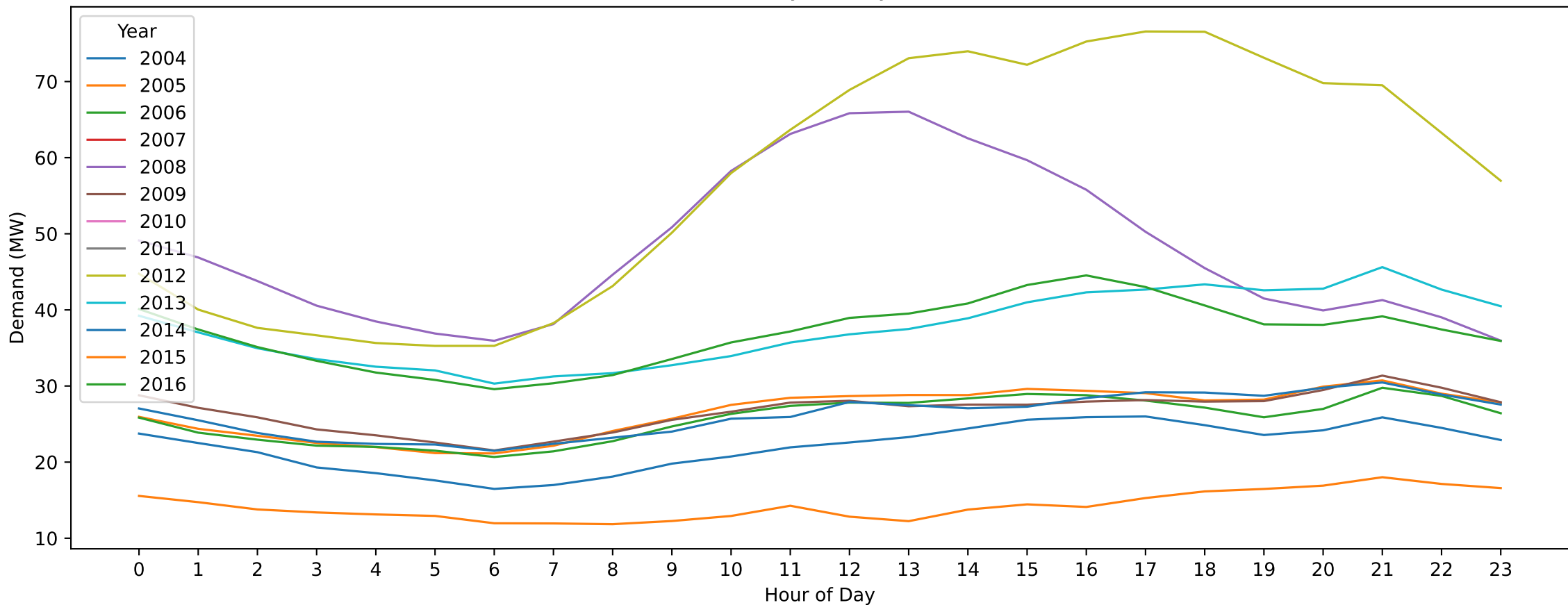
Sunshine — New Year's Day (Hourly Demand Across Years)
