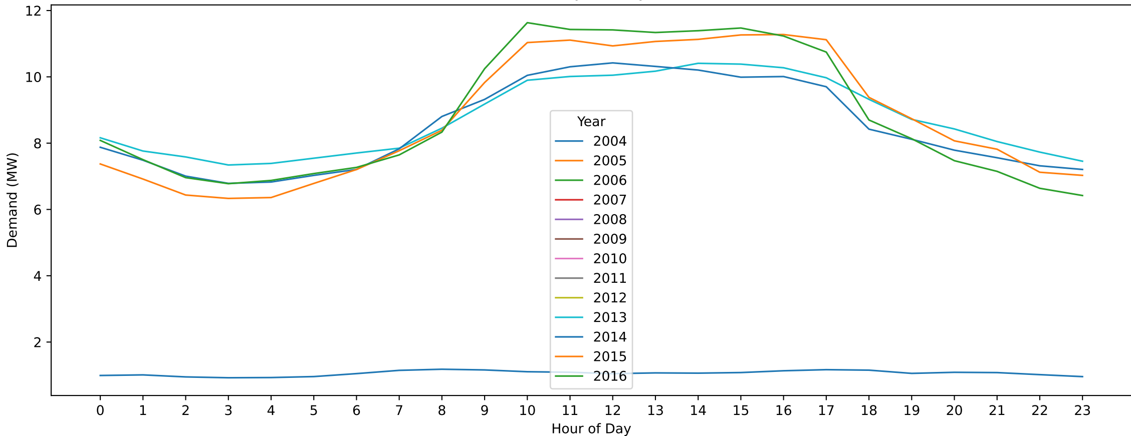
Docklands — New Year's Day (Hourly Demand Across Years)
