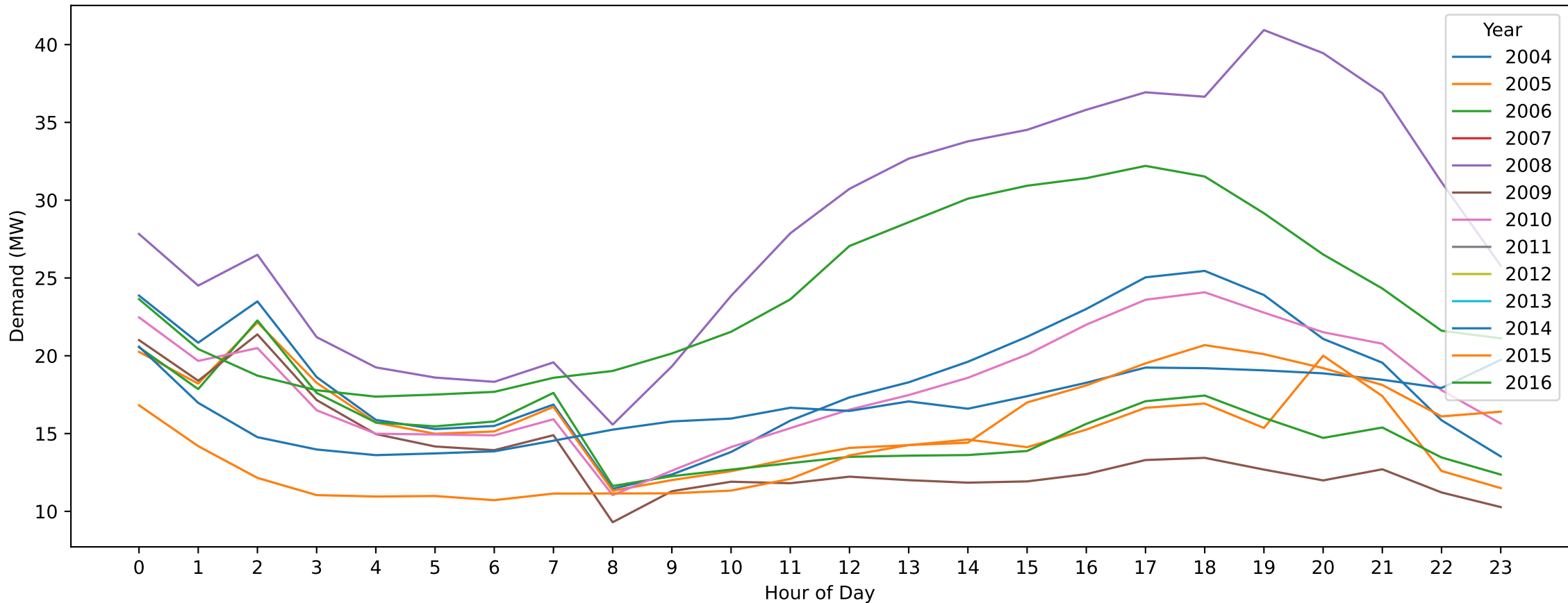
Eaglehawk — New Year's Day (Hourly Demand Across Years)
