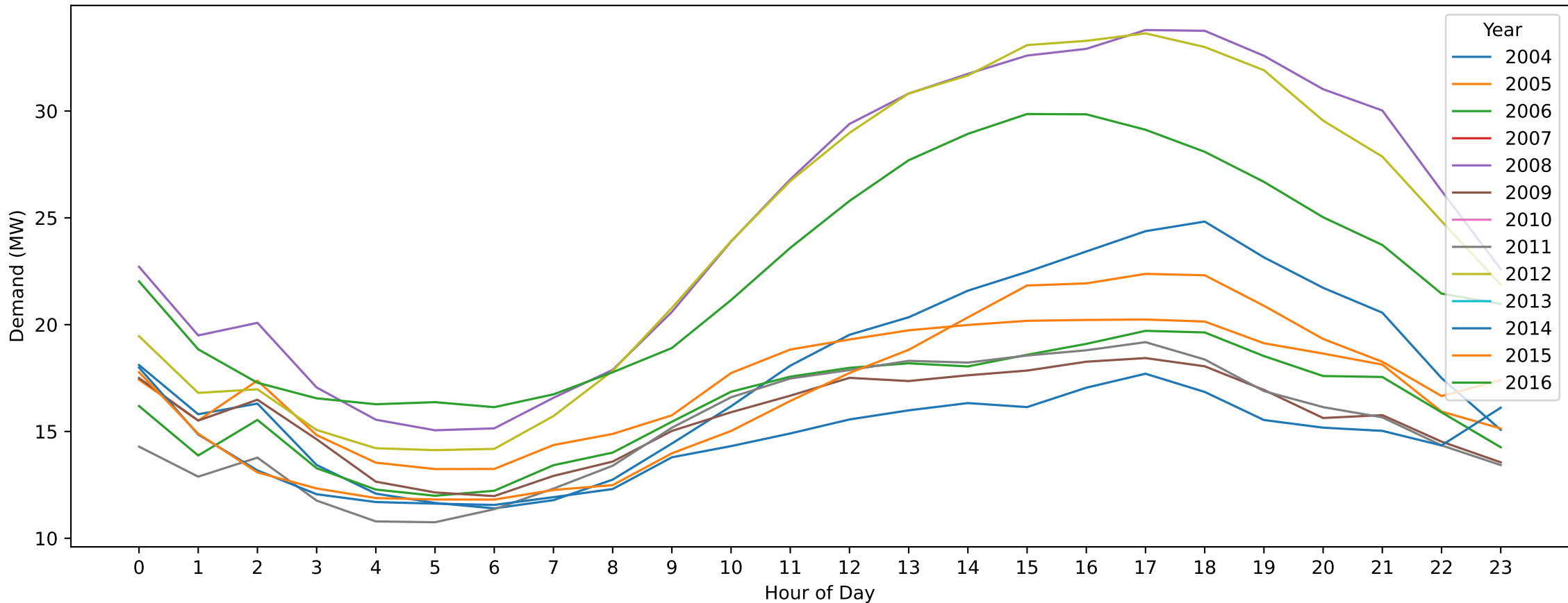
Shepparton — New Year's Day (Hourly Demand Across Years)
