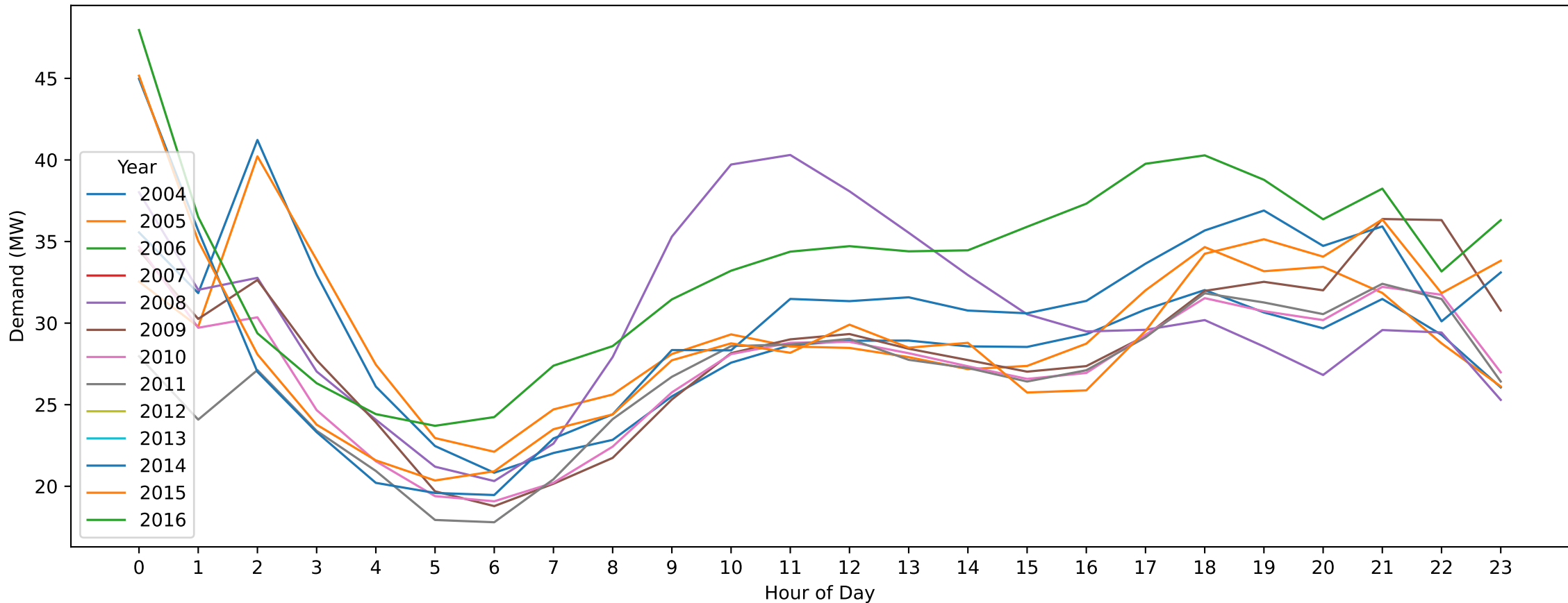
Waurn Ponds — New Year's Day (Hourly Demand Across Years)
