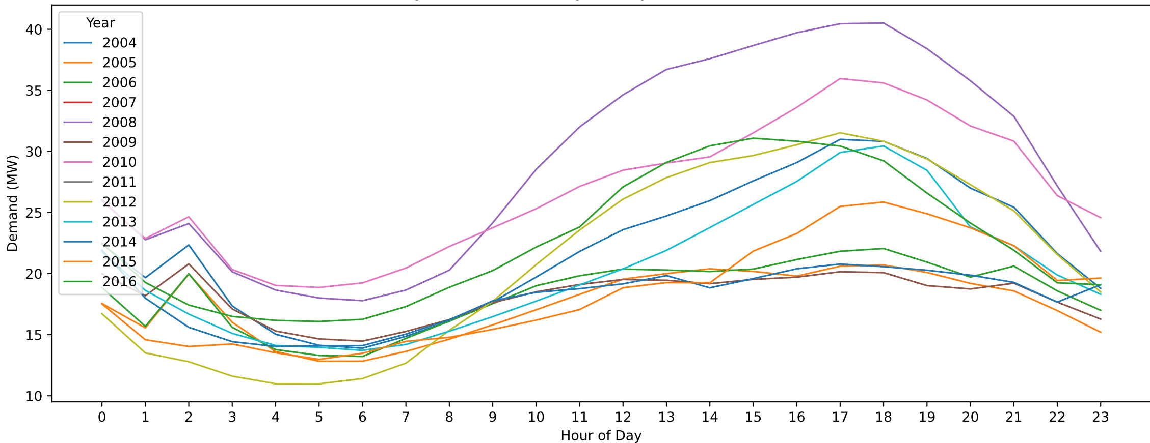
Bendigo — New Year's Day (Hourly Demand Across Years)
