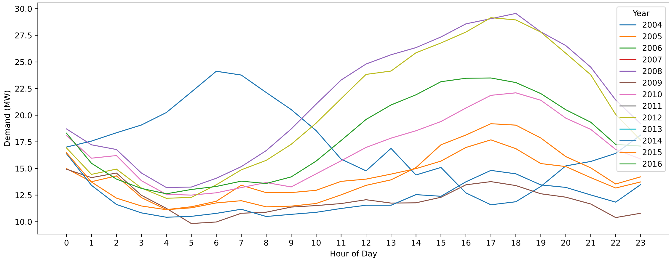
Shepparton Nth — New Year's Day (Hourly Demand Across Years)
