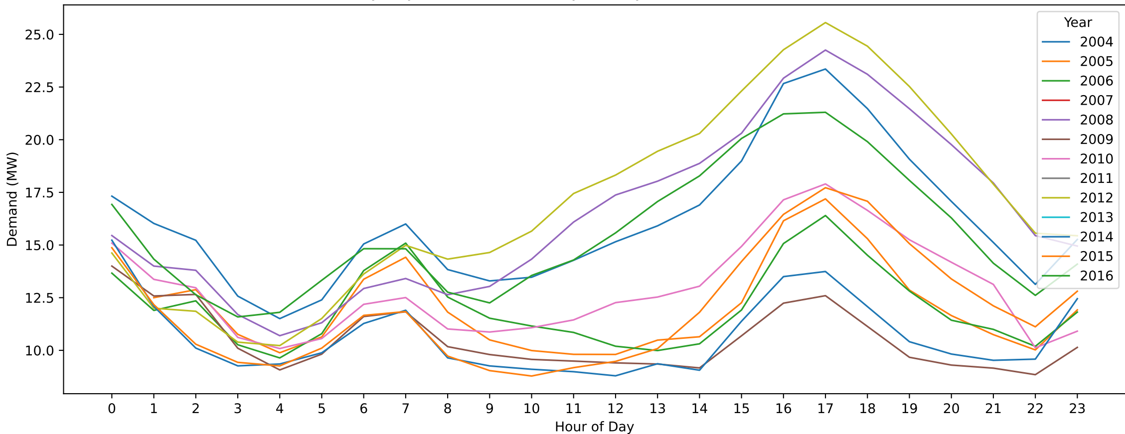
Kyabrym — New Year's Day (Hourly Demand Across Years)
