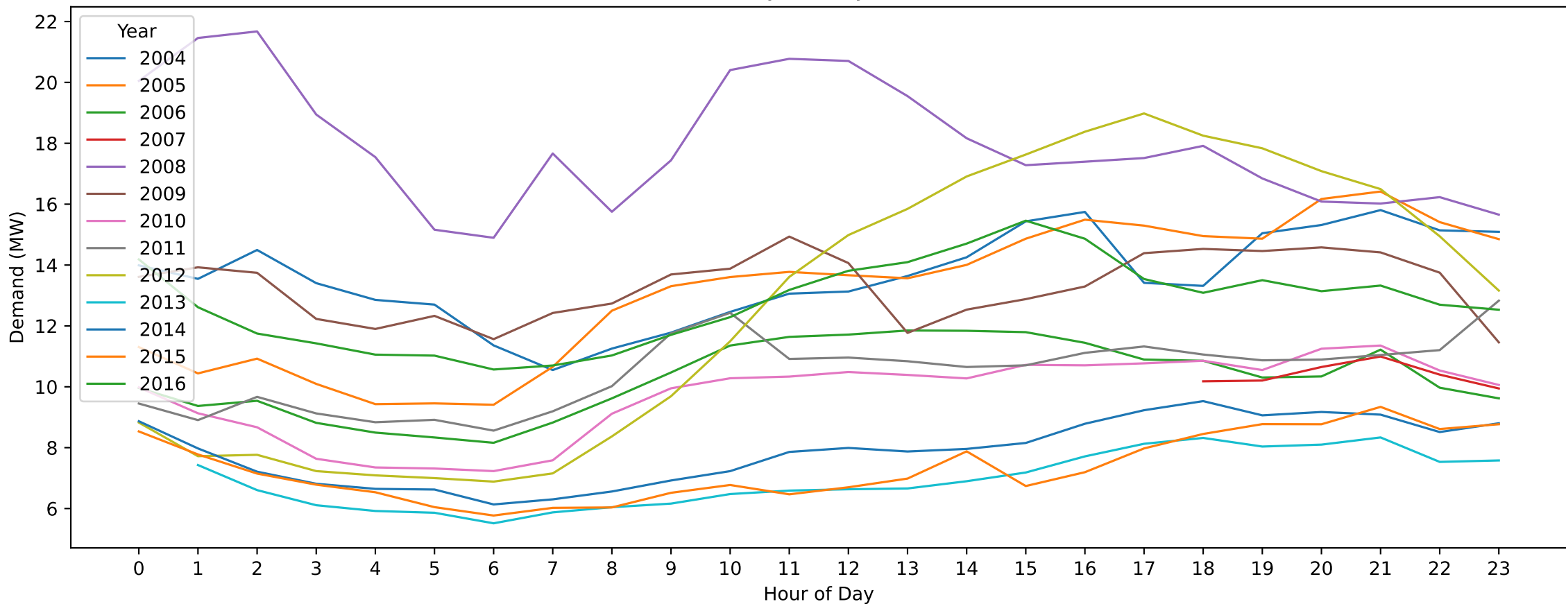
Corio — New Year's Day (Hourly Demand Across Years)
