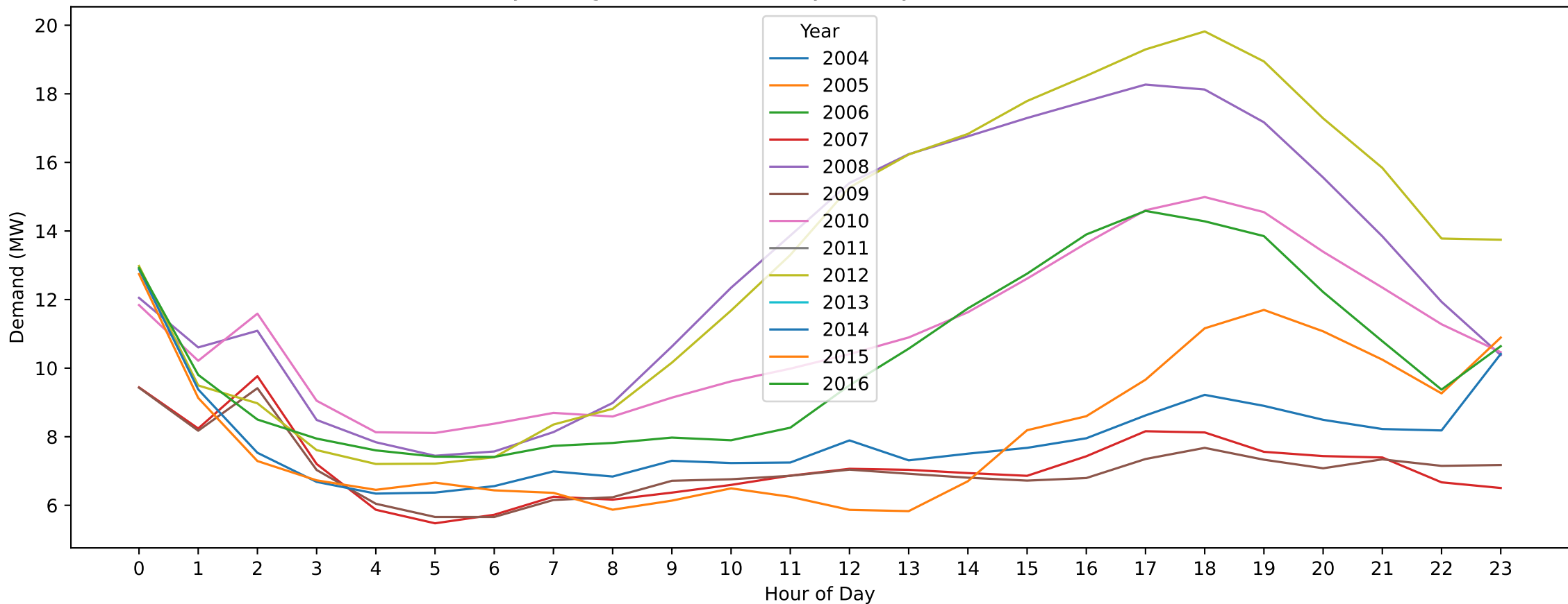
Maryborough — New Year's Day (Hourly Demand Across Years)
