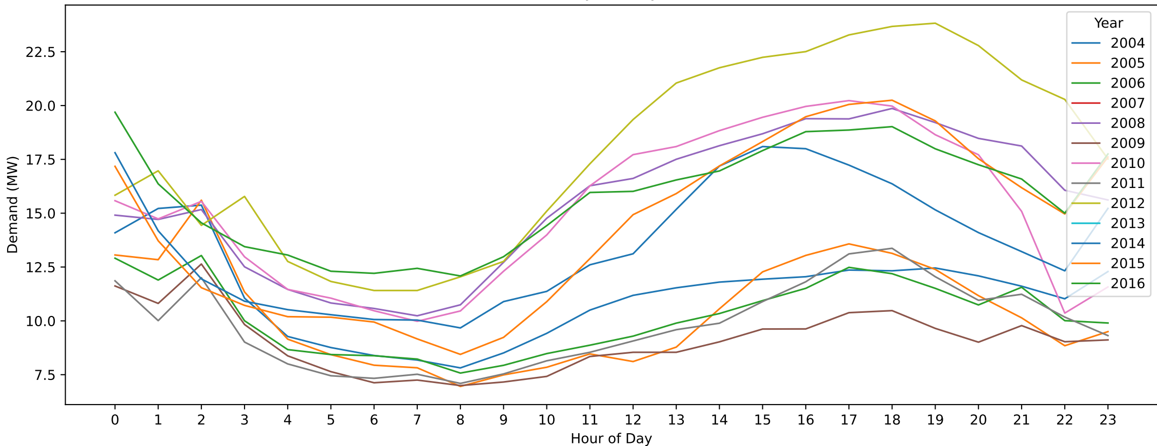
Merbein — New Year's Day (Hourly Demand Across Years)
