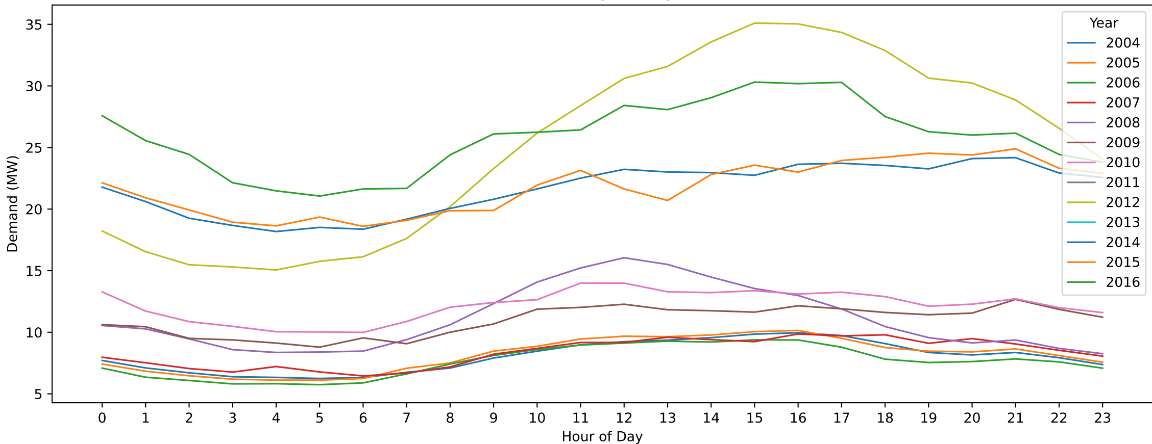
Sunshine East — New Year's Day (Hourly Demand Across Years)
