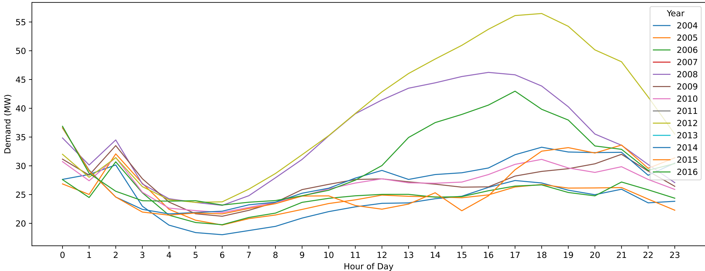
Ballarat South — New Year's Day (Hourly Demand Across Years)
