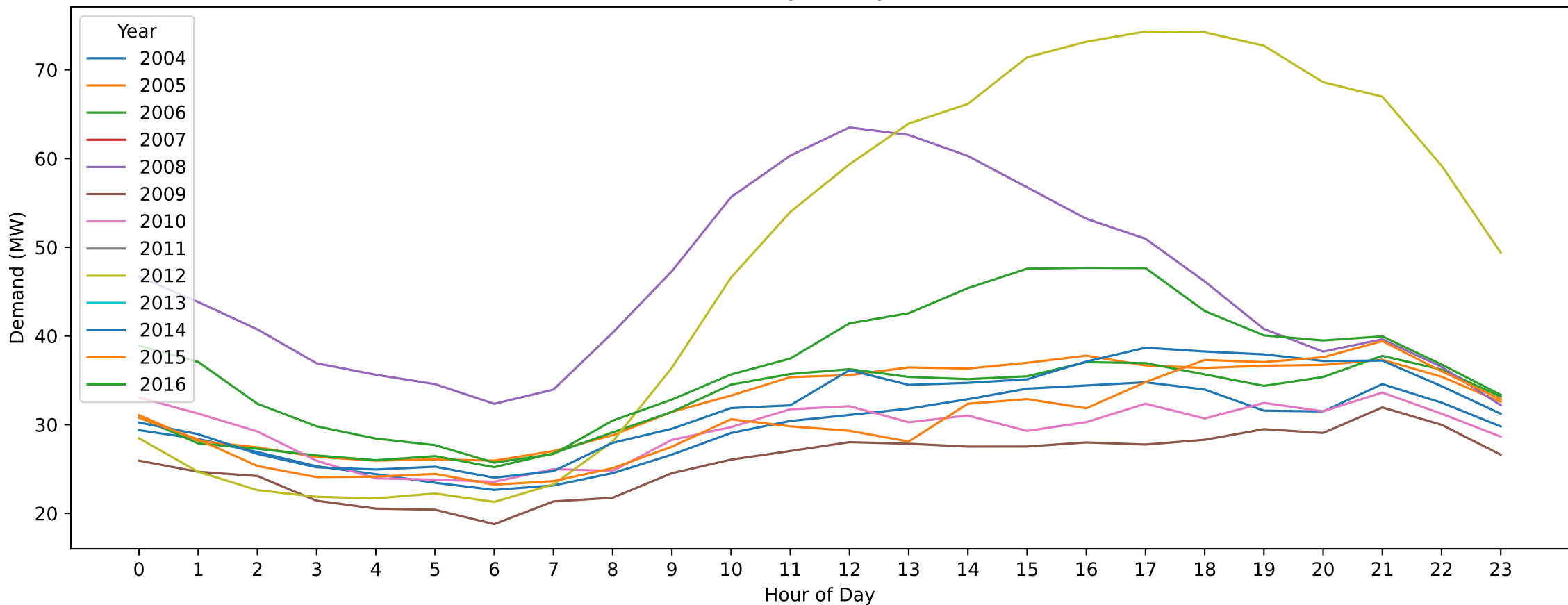
Laverton — New Year's Day (Hourly Demand Across Years)
