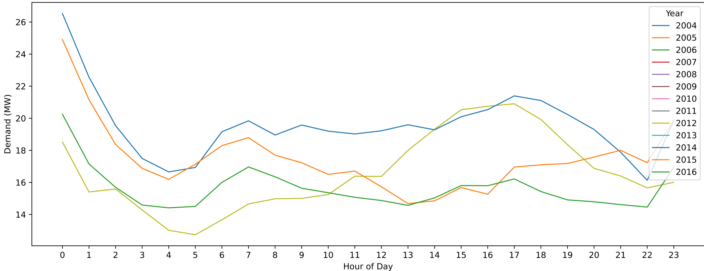
Koroit — New Year's Day (Hourly Demand Across Years)
