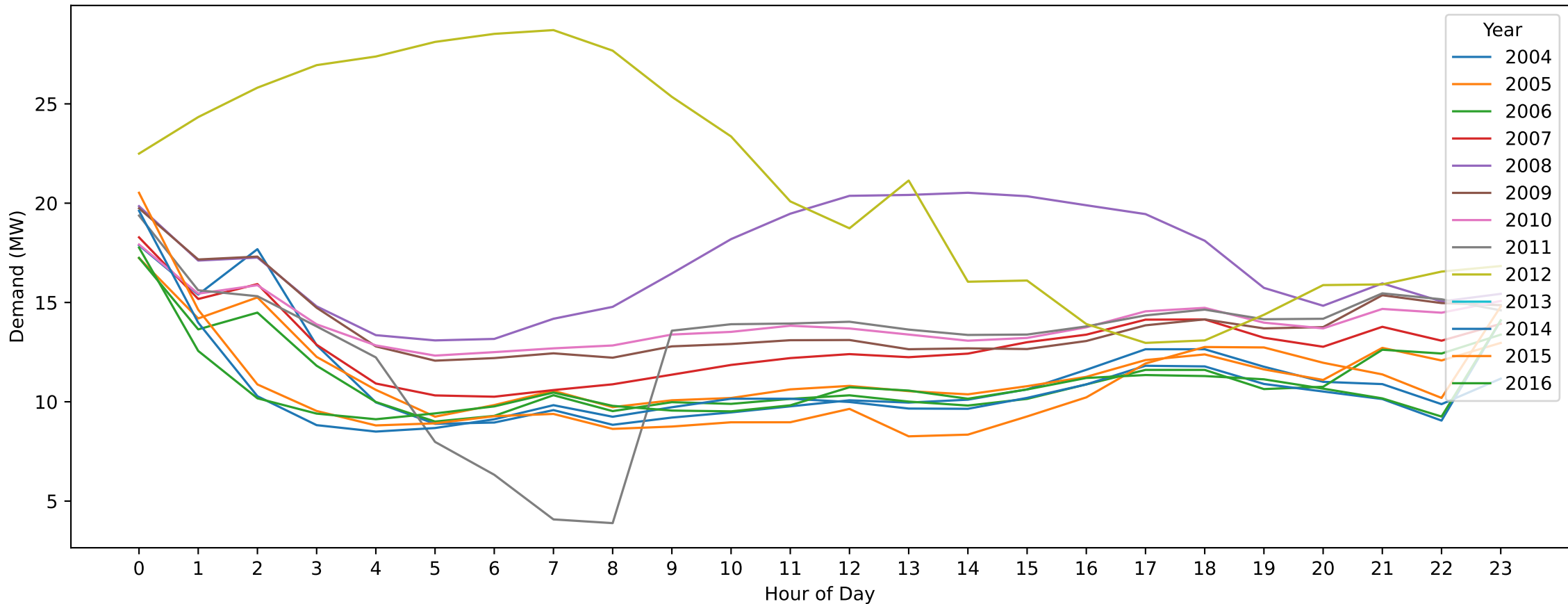
Hamilton — New Year's Day (Hourly Demand Across Years)
