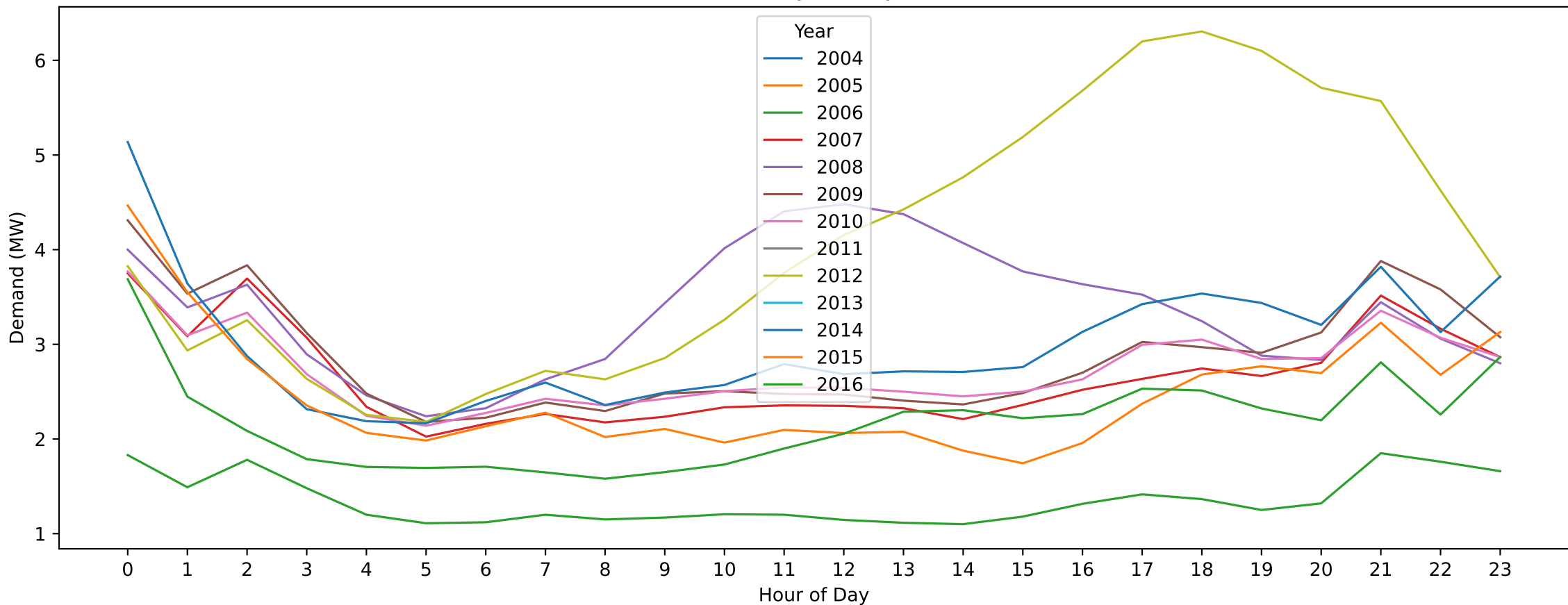
Winchelsea — New Year's Day (Hourly Demand Across Years)
