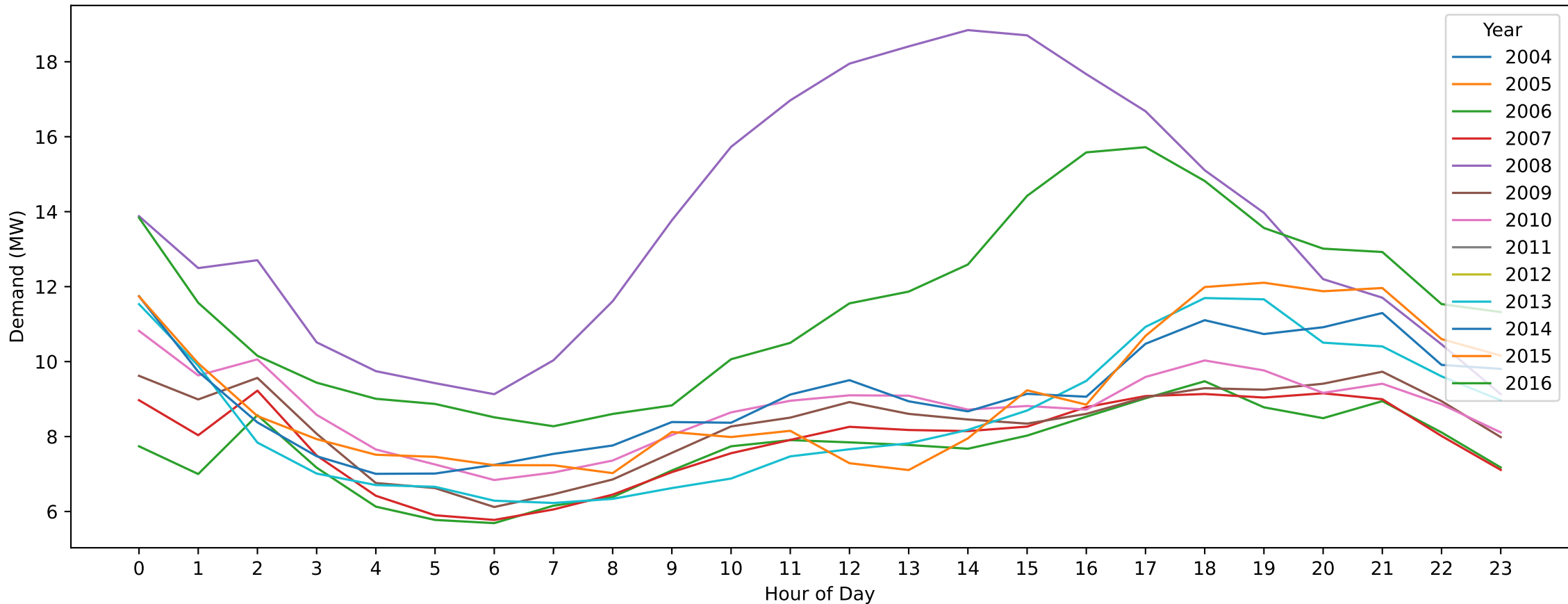
Bacchus Marsh — New Year's Day (Hourly Demand Across Years)
