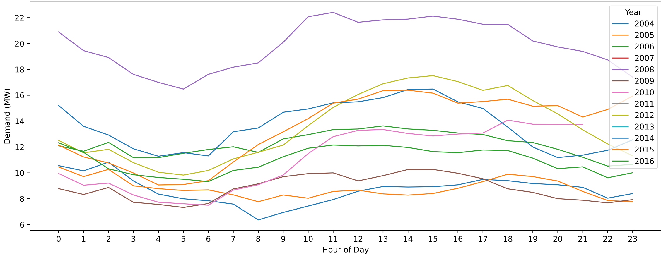
Robinvale — New Year's Day (Hourly Demand Across Years)
