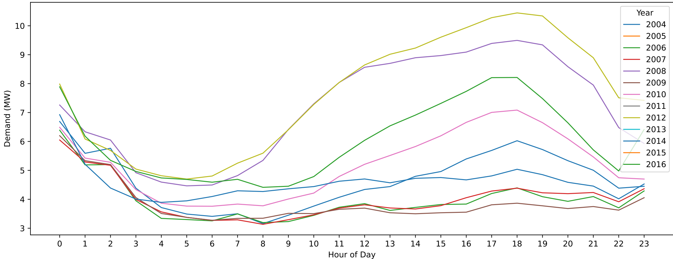
Nhill — New Year's Day (Hourly Demand Across Years)
