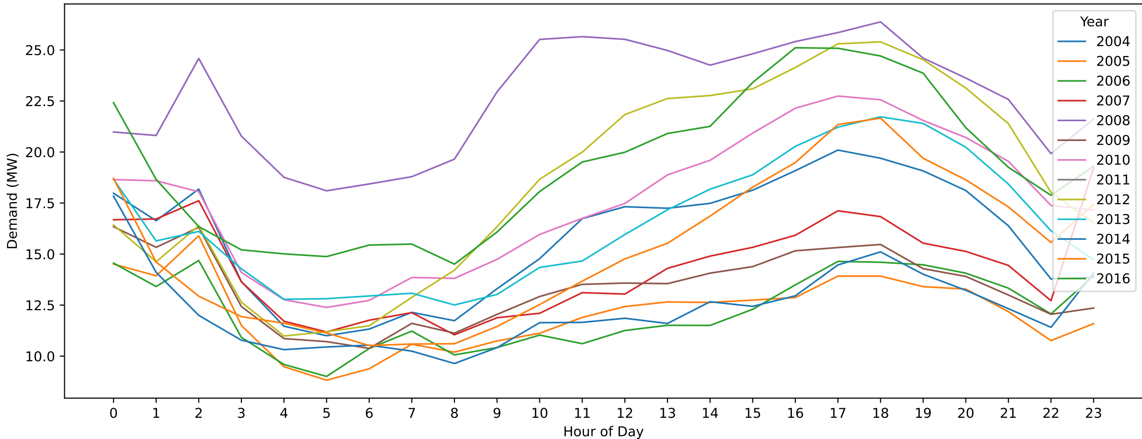
Cobram East — New Year's Day (Hourly Demand Across Years)
