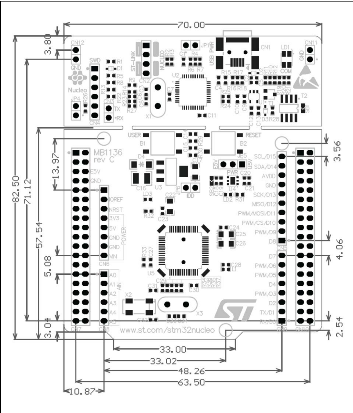
Figure 5. STM32 Nucleo board mechanical dimensions
