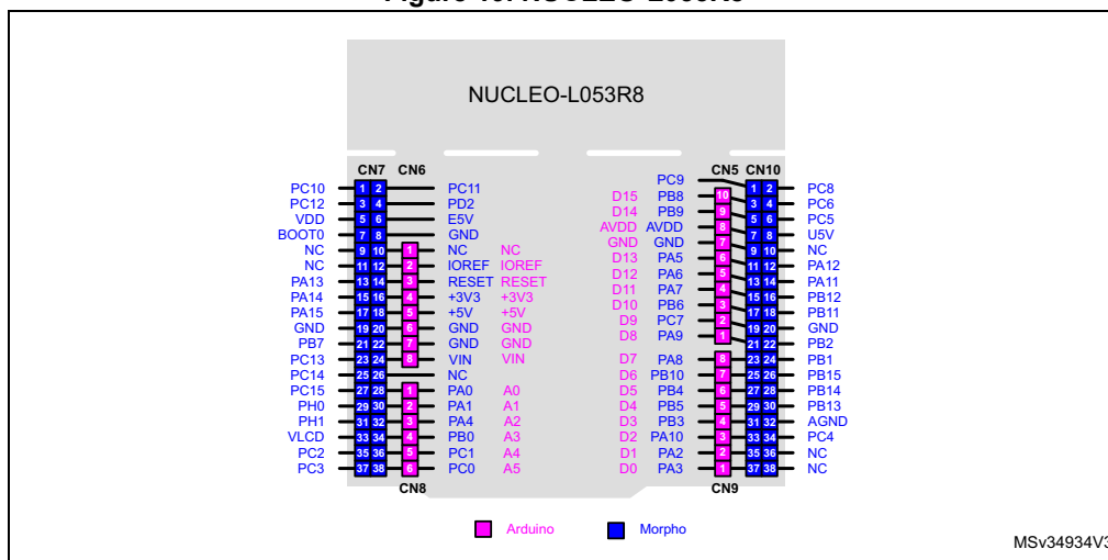
Figure 19. NUCLEO-L053R8
