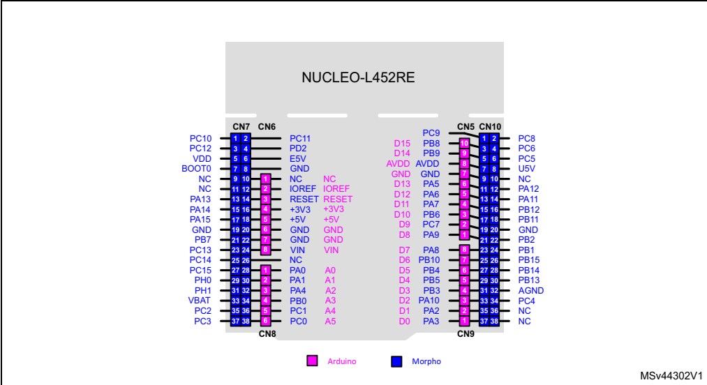
Figure 22. NUCLEO-L452RE
