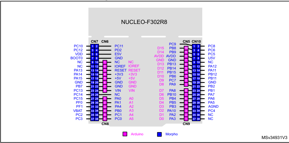
Figure 14. NUCLEO-F302R8
