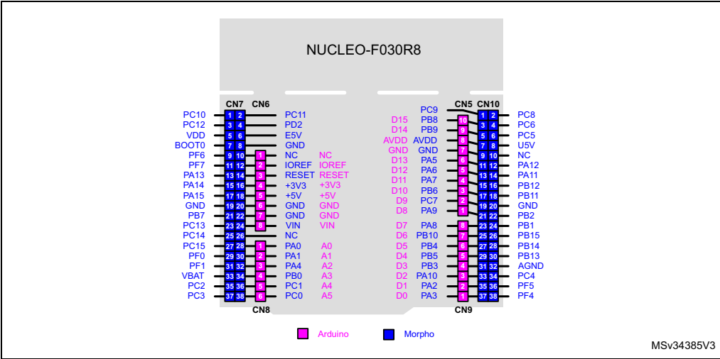
Figure 9. NUCLEO-F030R8
