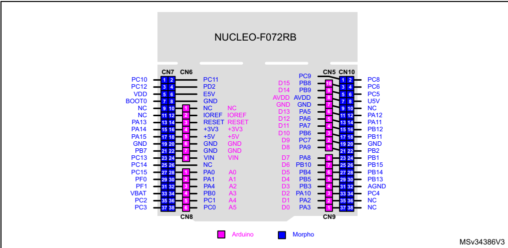
Figure 11. NUCLEO-F072RB
