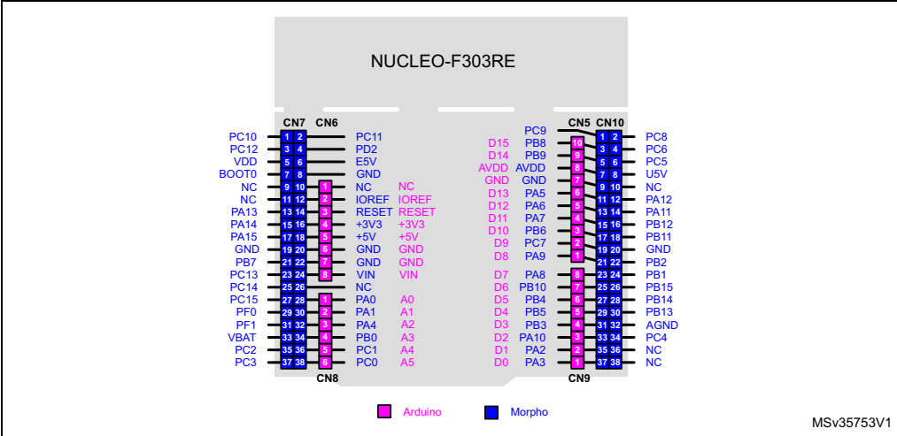
Figure 15. NUCLEO-F303RE
