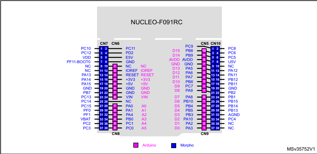
Figure 12. NUCLEO-F091RC
