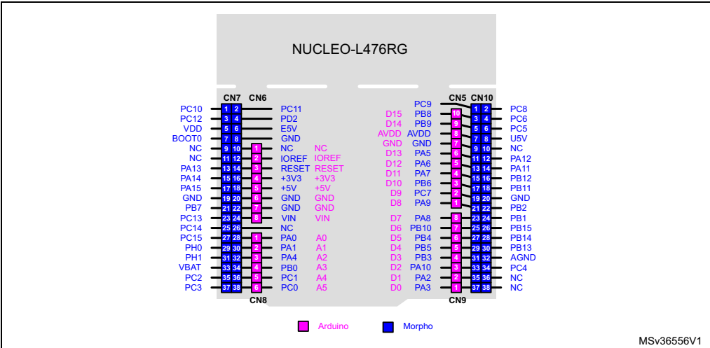
Figure 23. NUCLEO-L476RG
