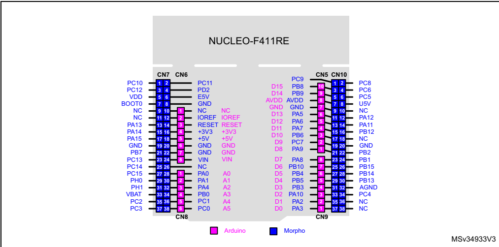
Figure 18. NUCLEO-F411RE
