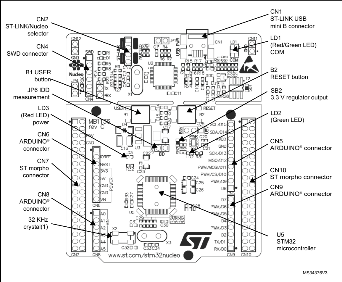
Figure 3. Top layout
