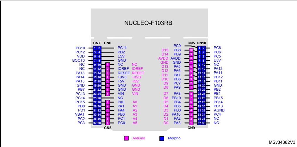
Figure 13. NUCLEO-F103RB
