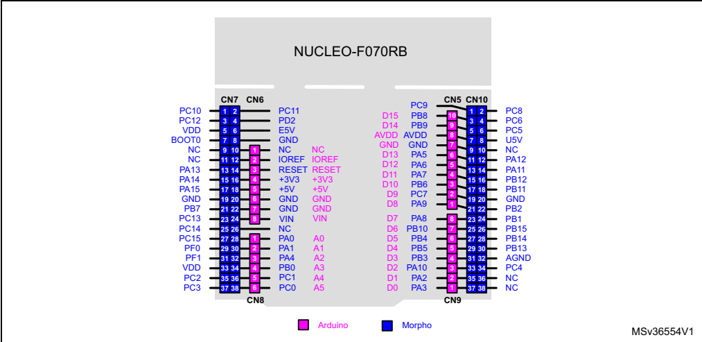
Figure 10. NUCLEO-F070RB
