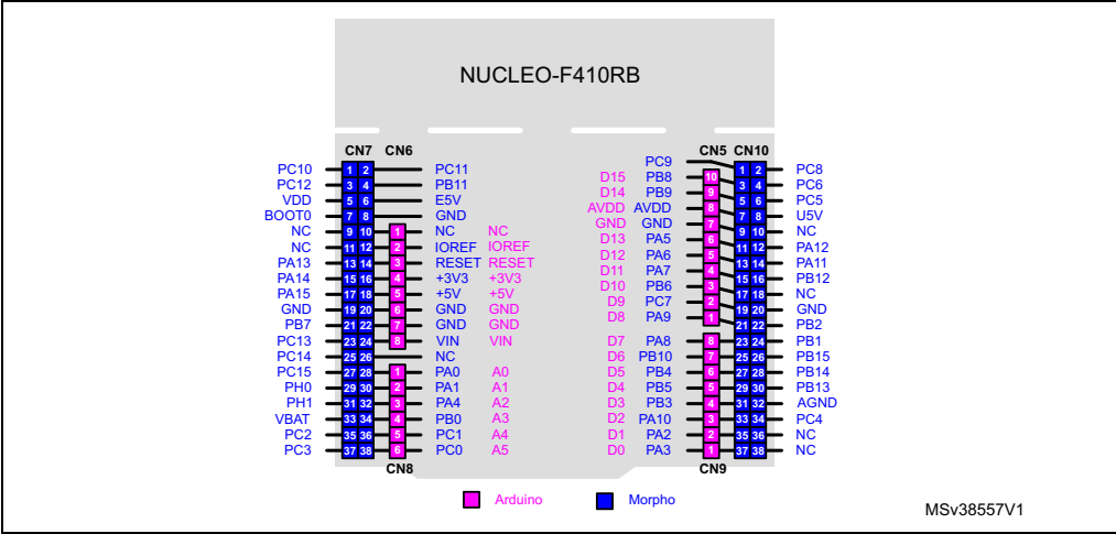
Figure 25. NUCLEO-F410RB
