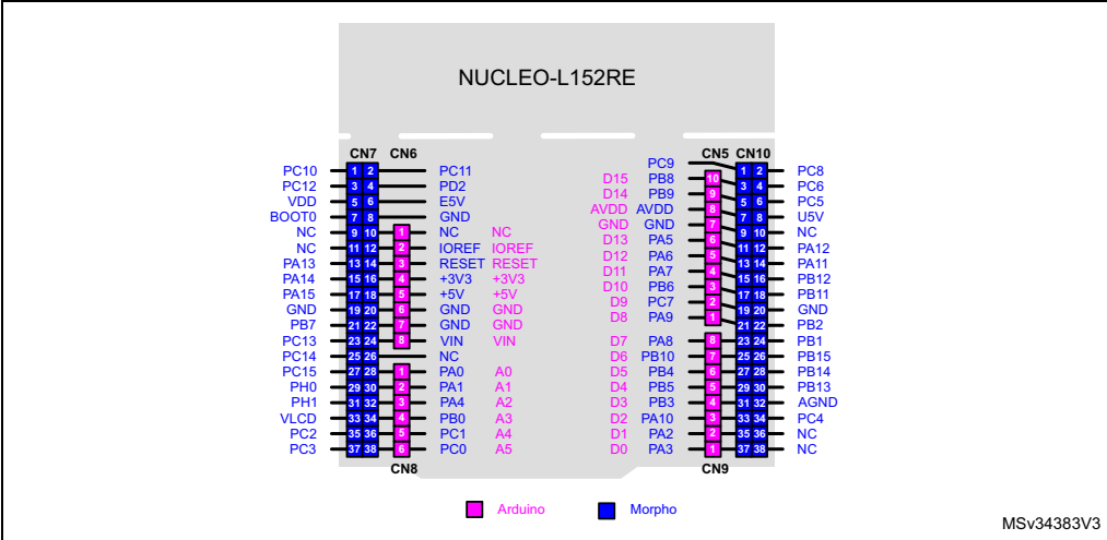
Figure 21. NUCLEO-L152RE
