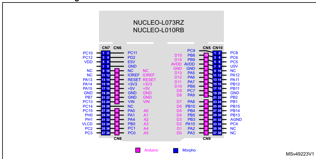
Figure 20. NUCLEO-L073RZ and NUCLEO-L010RB
