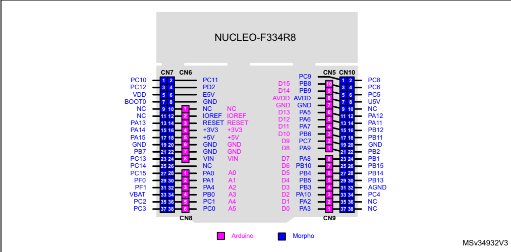
Figure 16. NUCLEO-F334R8
