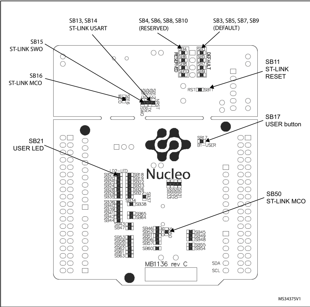
Figure 4. Bottom layout
