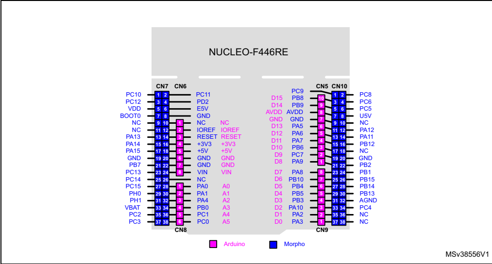
Figure 24. NUCLEO-F446RE
