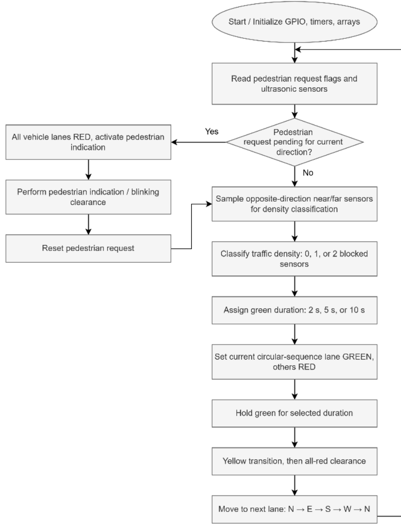
Fig. 2. Flowchart of the adaptive traffic control algorithm.
