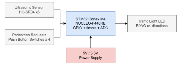
Fig. 1. Embedded system architecture of the proposed adaptive traffic controller.
