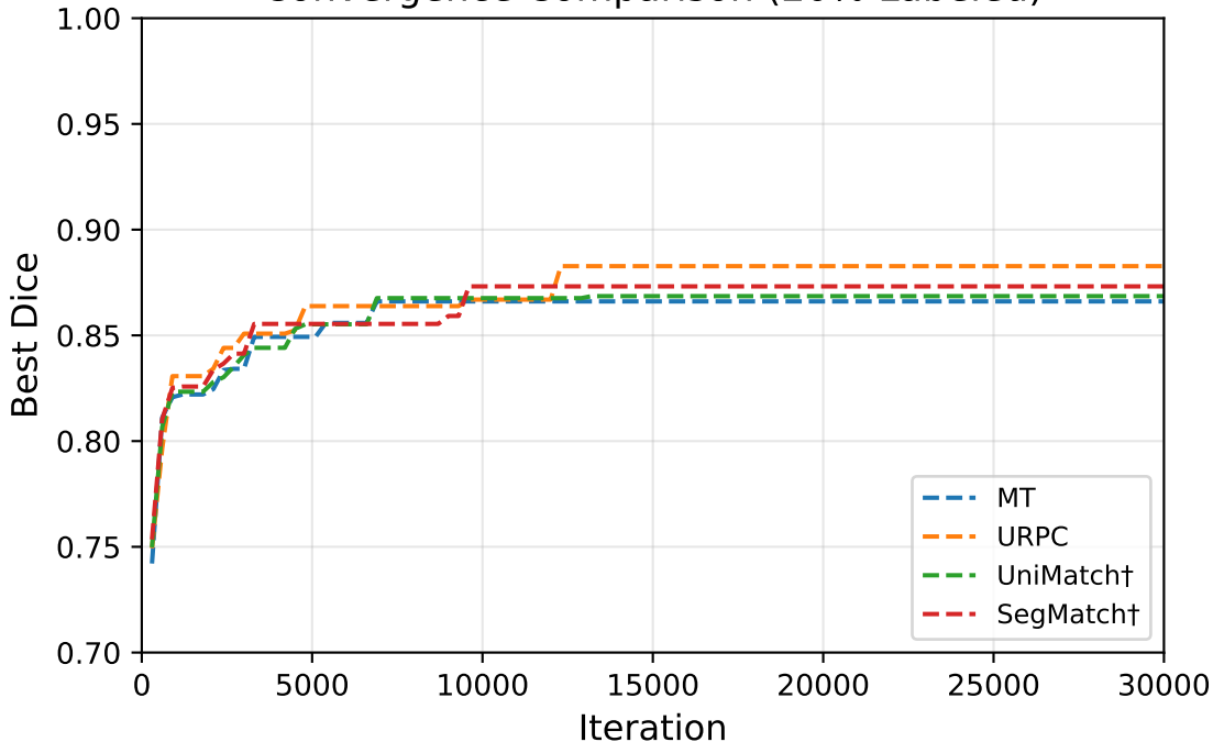
Convergence Comparison (20% Labeled)
