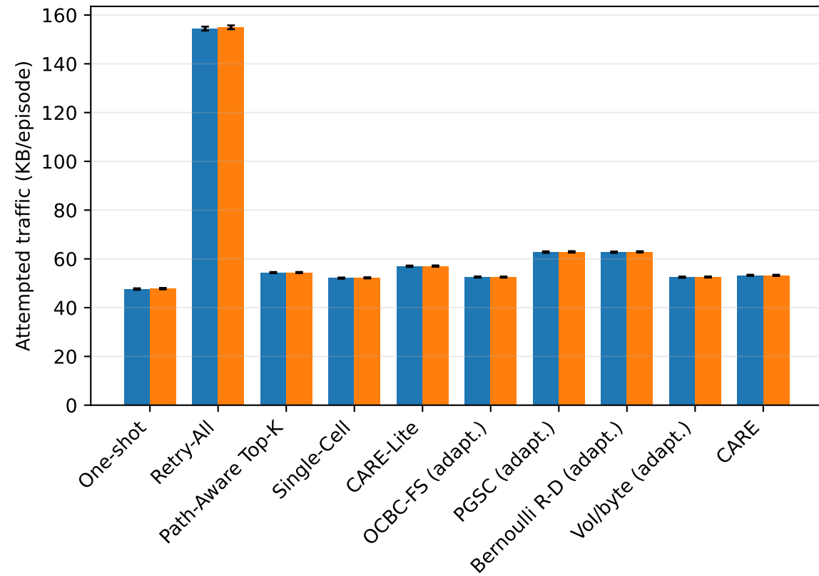
Closest-work controls under one explicit-map communication contract (95% map CIs)
