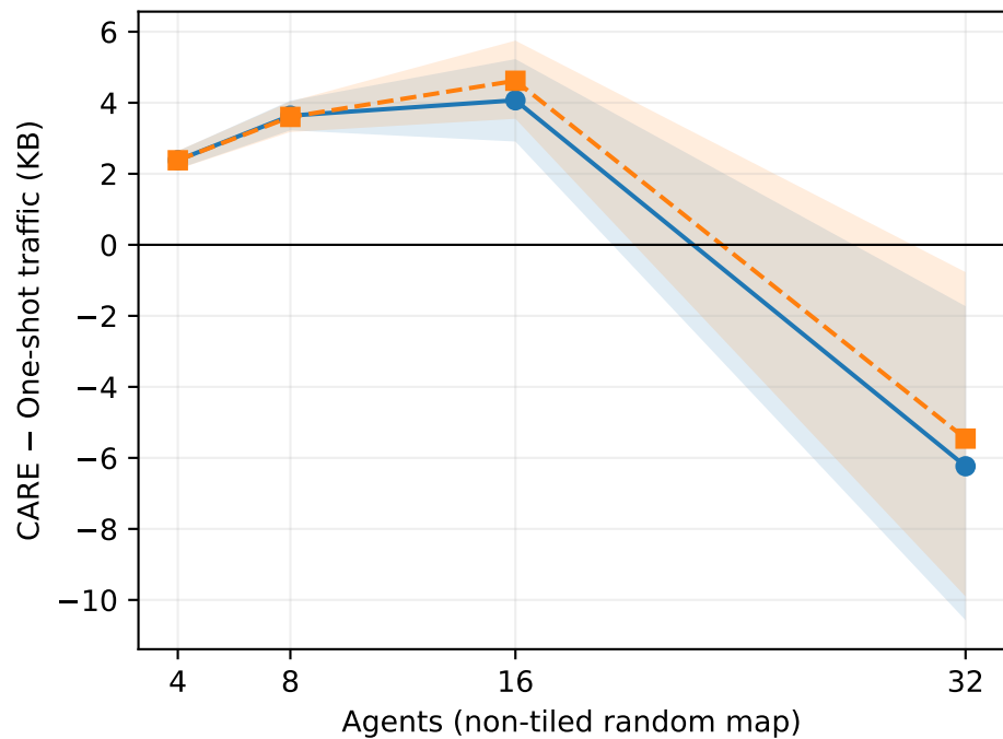
Natural decision-conflict scale study (paired 95% map CIs)
