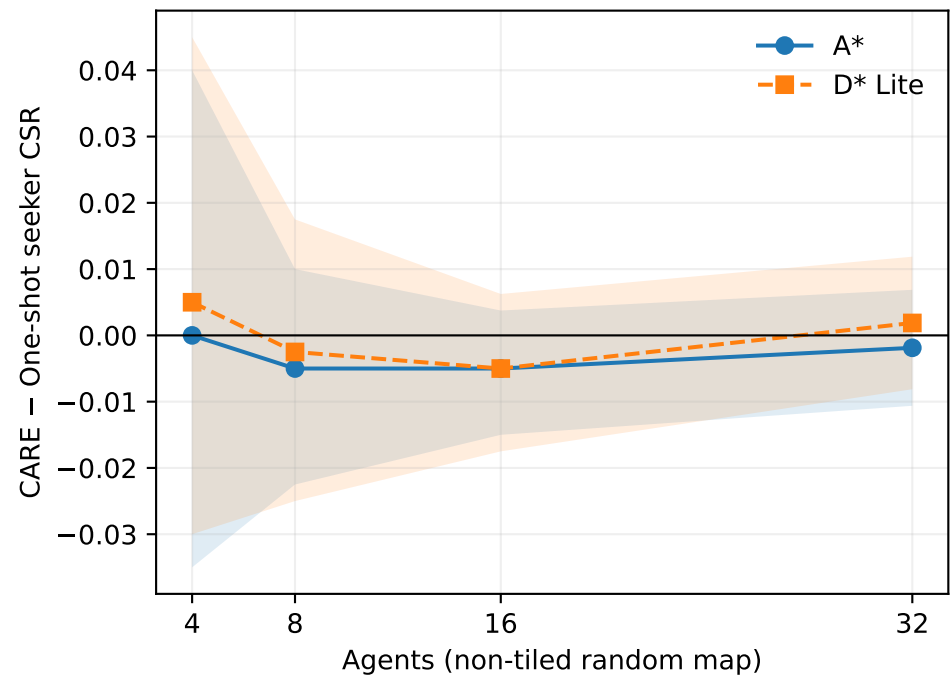
Natural decision-conflict scale study (paired 95% map CIs)
