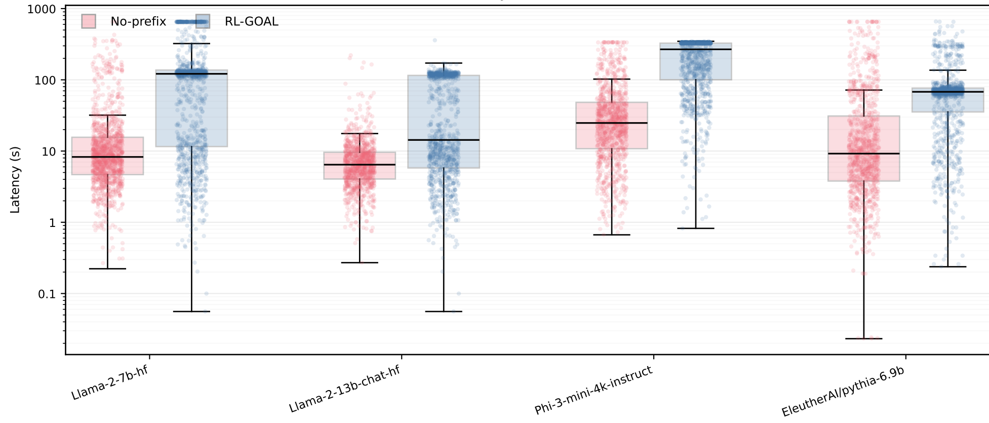
Latency distributions
