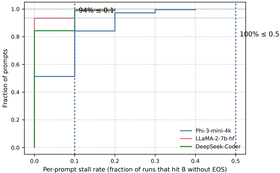
CDF of Per-prompt Stall Rates
