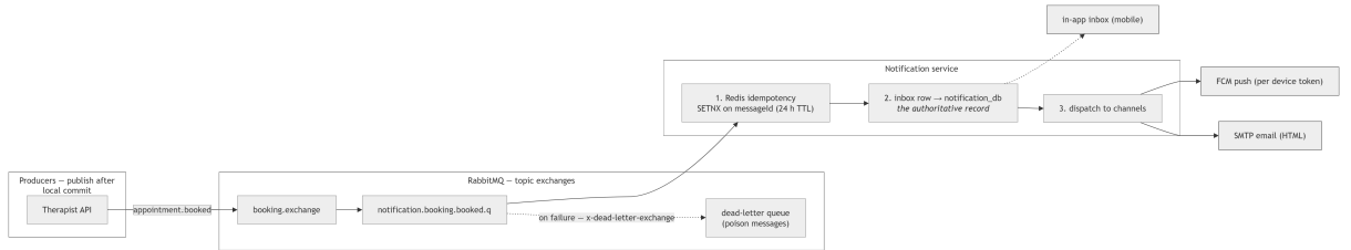
Figure 3.5: An event-flow diagram of domain event publication and consumption.
