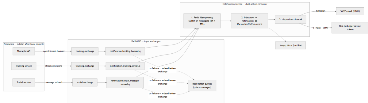
Figure 3.5: An event-flow diagram of domain event publication and consumption.
