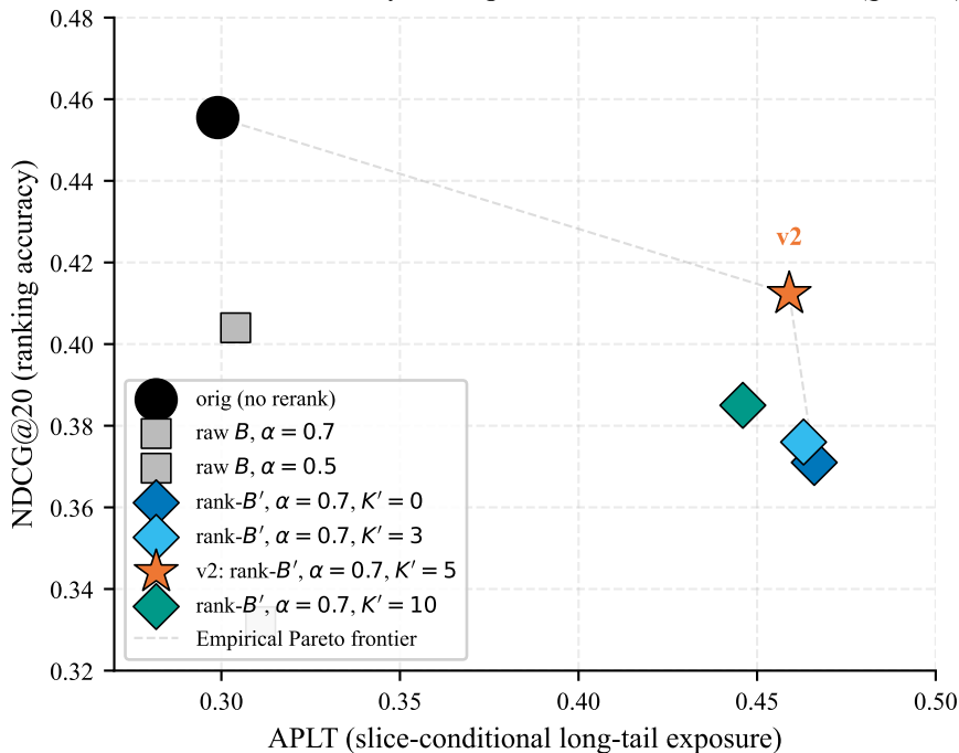
Pareto frontier: accuracy vs. exposure fairness on LFM-1K (gender)
