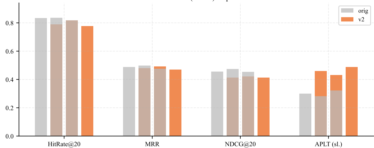
LastFM-1K track-level (n=600): exposure trade-off
