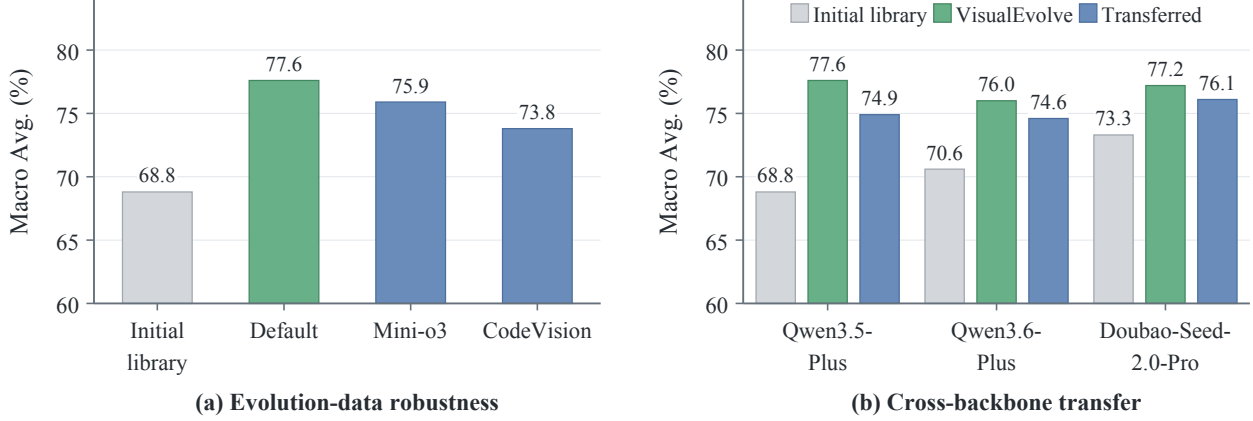
Figure 4 Generalization of VisualEvolve (RQ3). Macro-average Acc@1 (%) across six evaluation sets from the three benchmarks. In (b), VisualEvolve denotes results from backbone-specific evolution, where the skill library is evolved using the corresponding target backbone.
