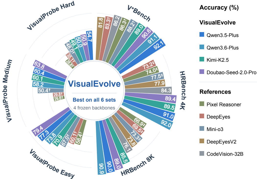
Figure 1 VisualEvolve versus training-based agents on six visual-reasoning evaluation sets. All four frozen-backbone configurations exceed the best reported reference accuracy (%) on each set (Table 1). VisualEvolve: Acc@1; †: Avg@32; ‡: Avg@8. Backbones and protocols differ; bar lengths are comparable only within sectors.
