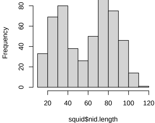
Histogram of squid$nid.length
