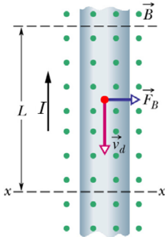
Halliday-Resnick-Walker (2003) Abb. 29.17
