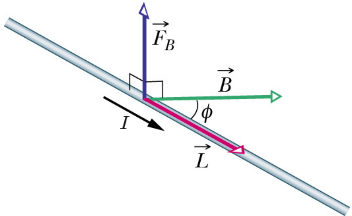
Halliday-Resnick-Walker (2003) Abb. 29.17
