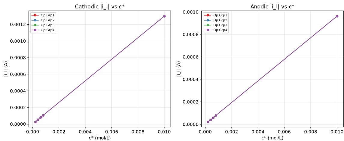
图 2: 浓度校准: |i_l| vs c^* @2000 rpm
