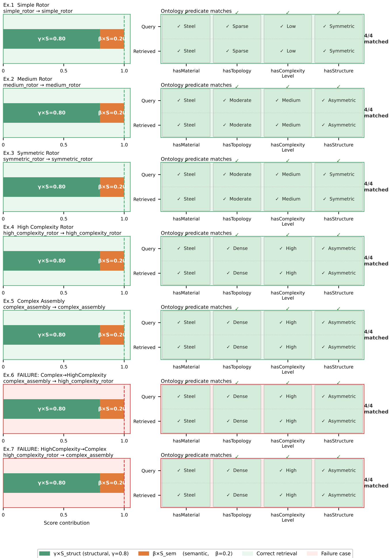
Fig. 5 Explainability traces: ontology-guided score decomposition per retrieval example
