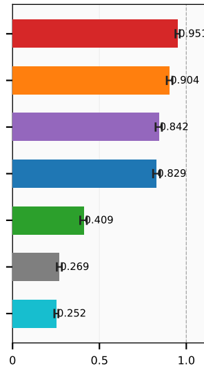
P@5
