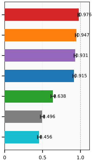
MRR
