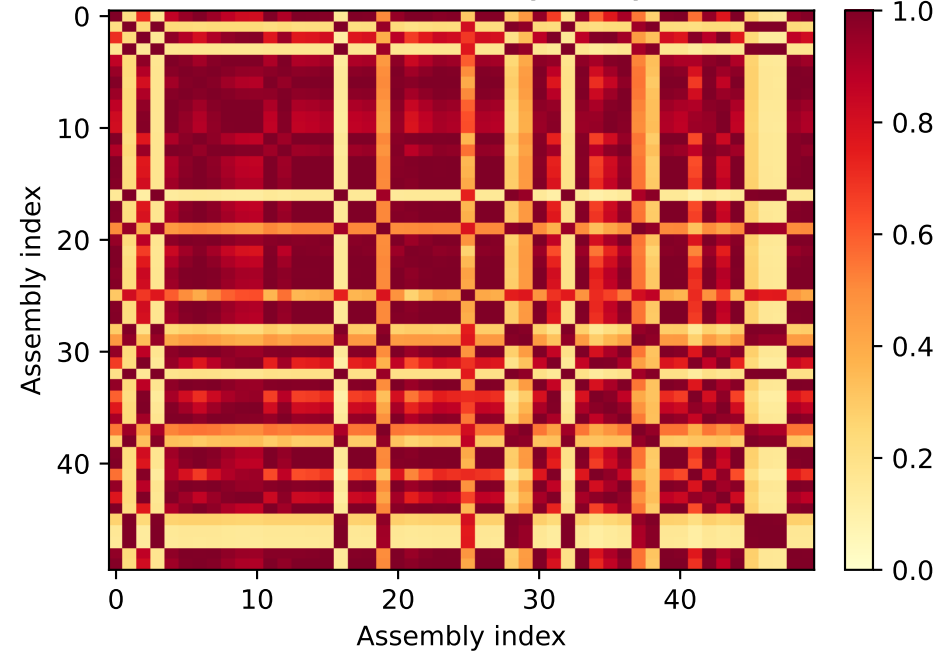
Structural Similarity (first 50, sorted by family)
