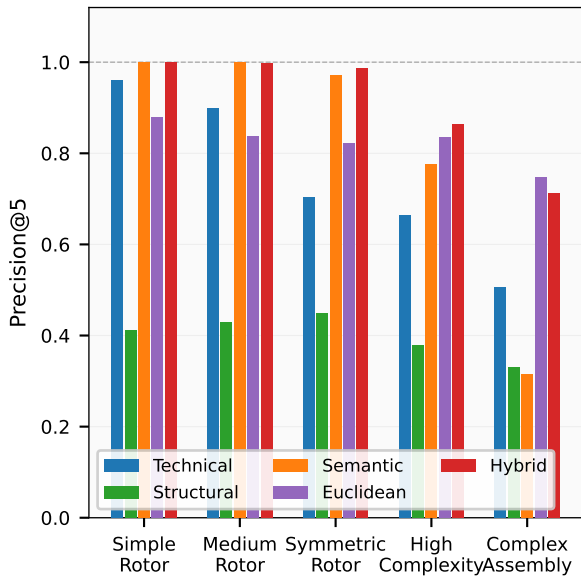
Per-Family P@5 by Method
