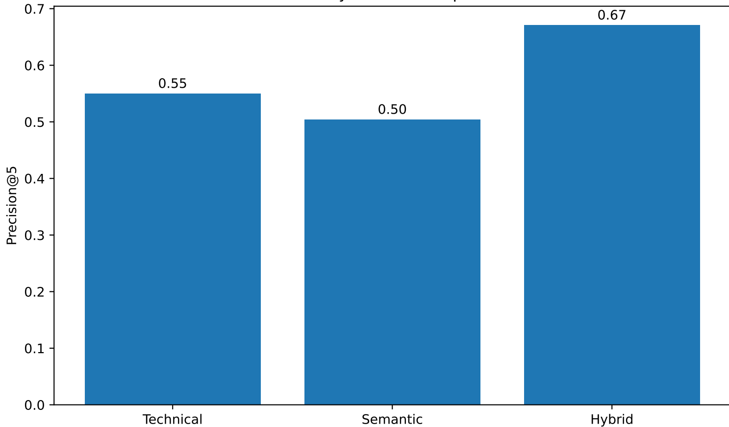
Similarity Method Comparison
