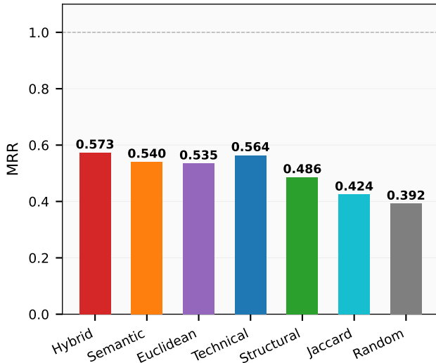
Mean Reciprocal Rank
