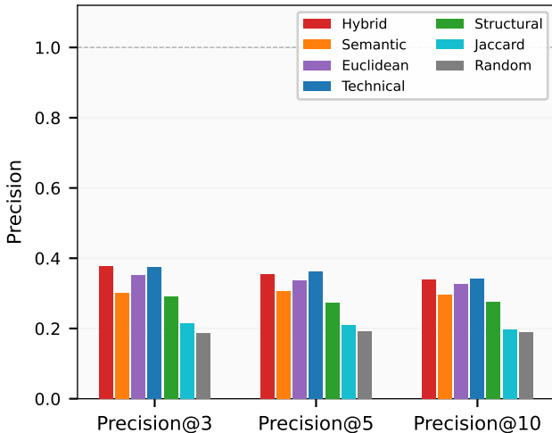
Precision@K Comparison
