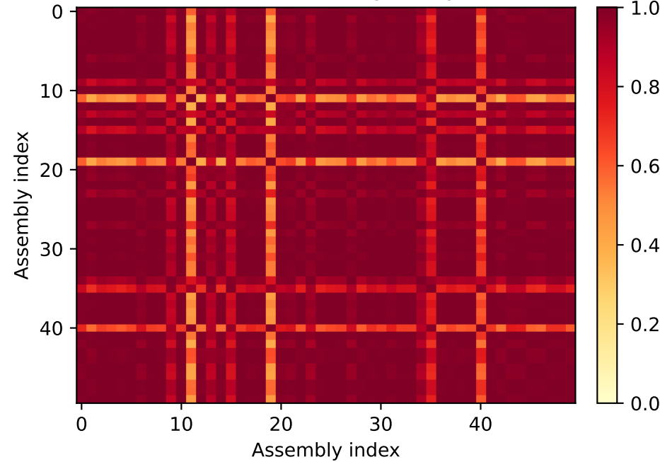
Technical Similarity (first 50, sorted by family)
