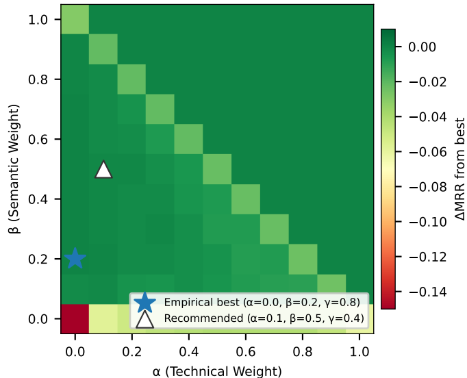
Hybrid Weight Grid Search — MRR
