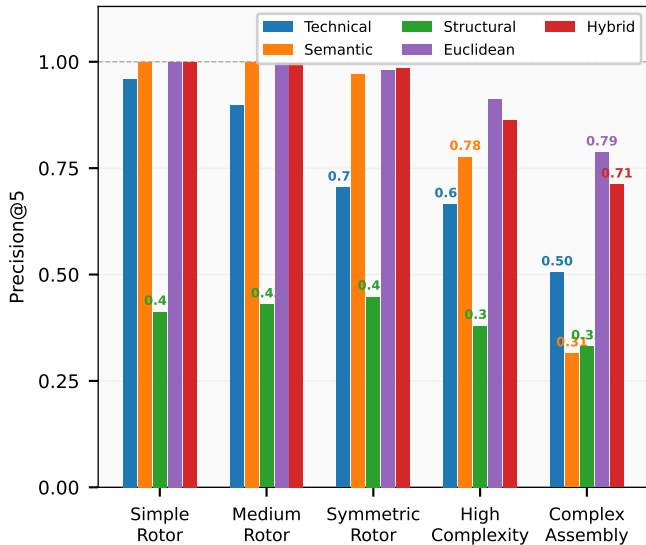
Per-Family Precision@5
