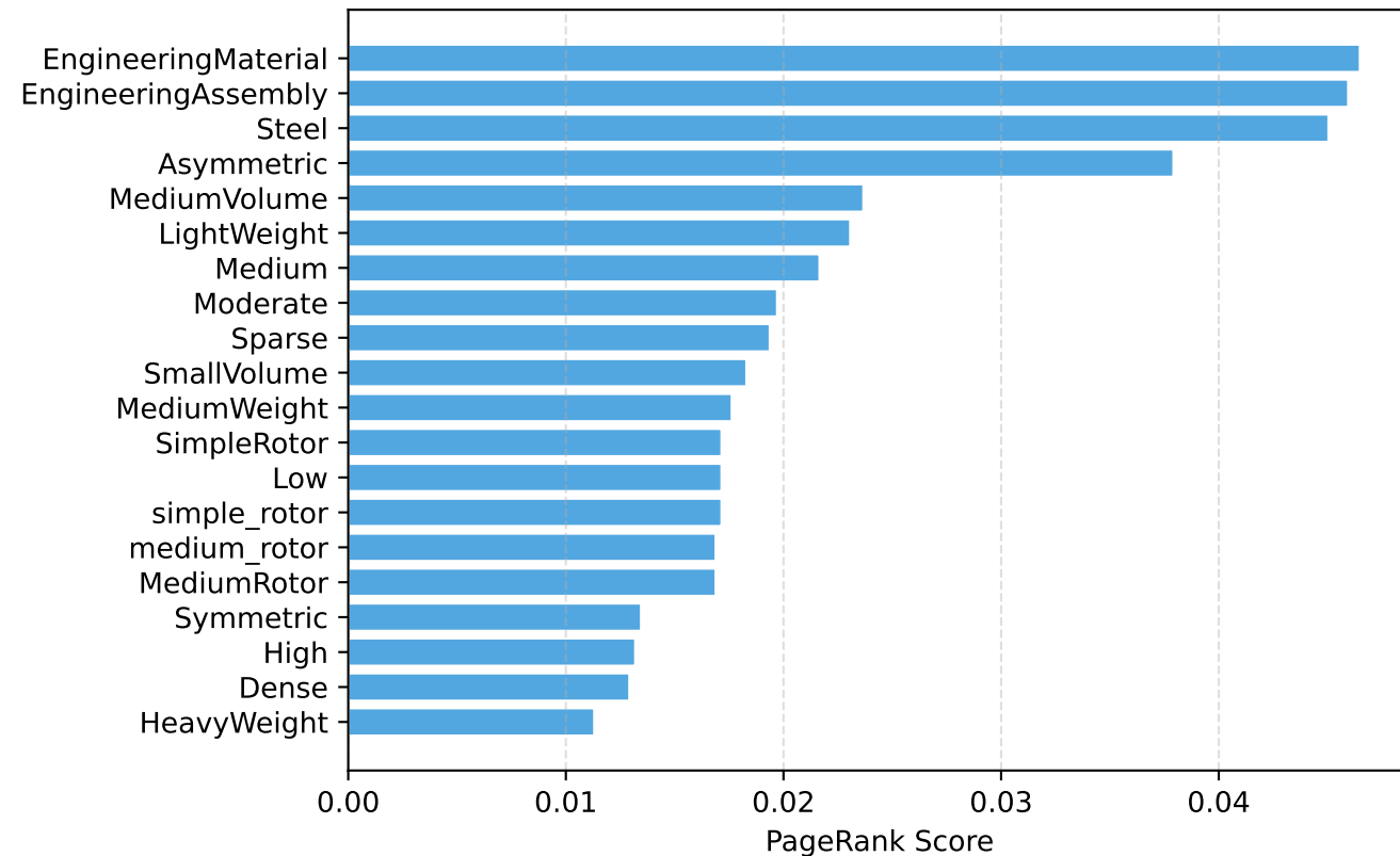
Top-20 Nodes by PageRank
