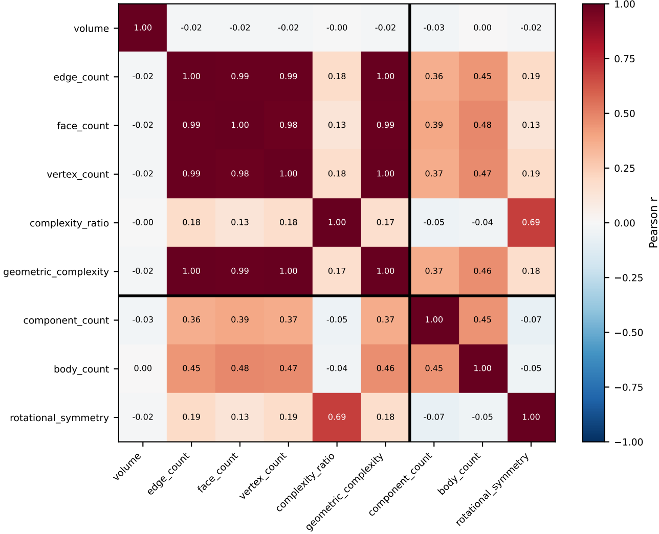
Feature Correlation Matrix (black line: Technical | Structural boundary)
