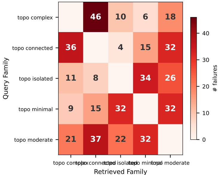
Hybrid Rank-1 Failure Confusion (446 total failures)
