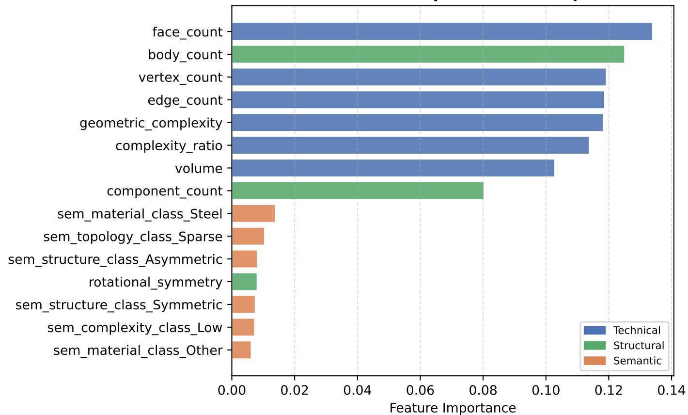
Random Forest — Top-15 Feature Importance
