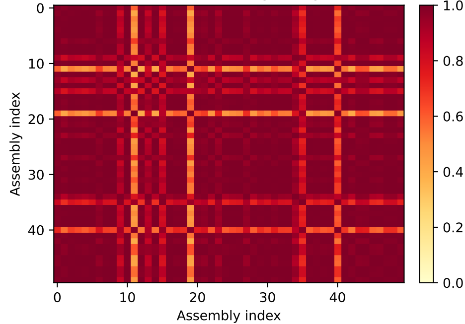
Technical Similarity (first 50, sorted by family)
