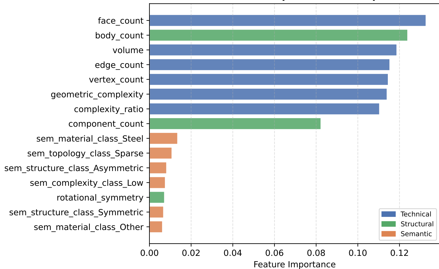
Random Forest — Top-15 Feature Importance
