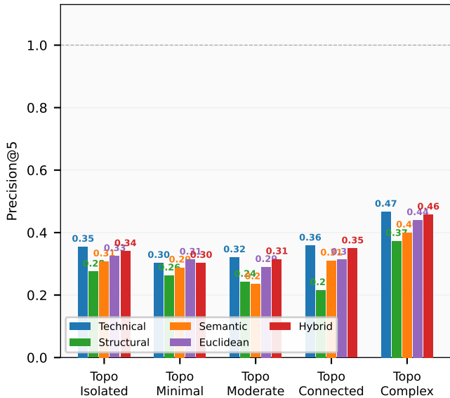
Per-Family Precision@5
