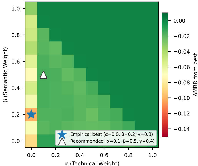
Hybrid Weight Grid Search — MRR
