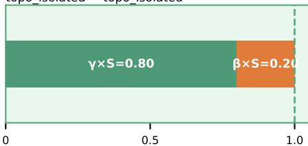
Fig. 5 Explainability traces: ontology-guided score decomposition per retrieval example
