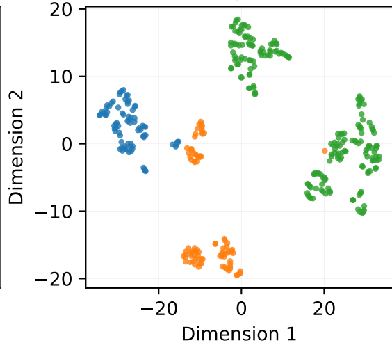
Inception
