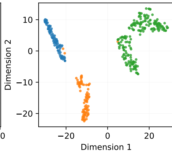
Transformer
