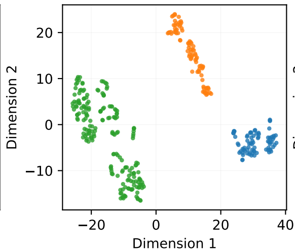
Inception
