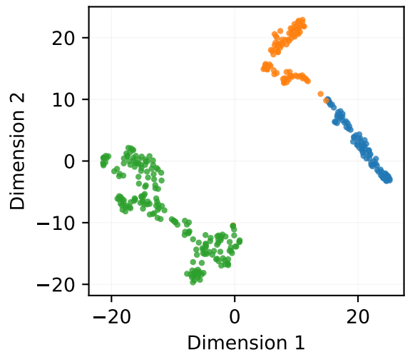
LSTM
