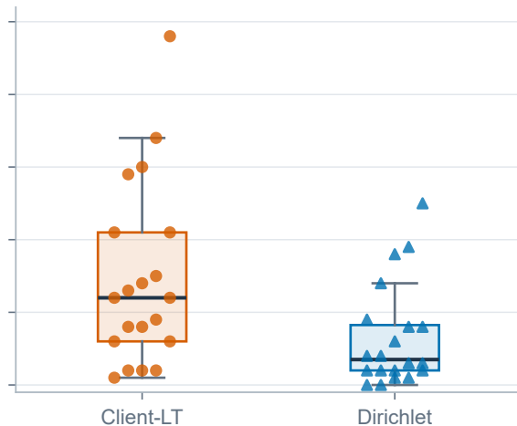
J: 20 individual tail classes
