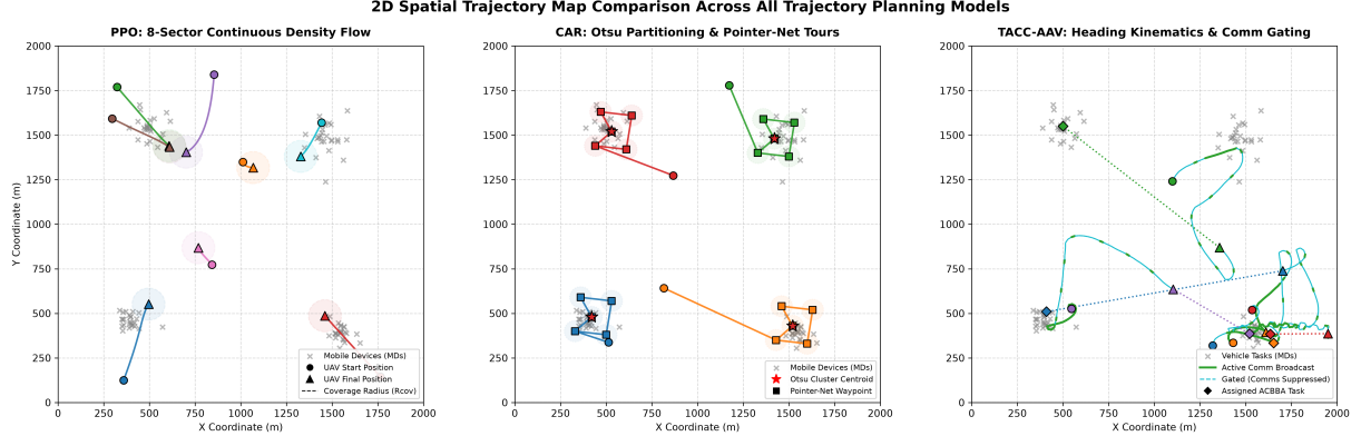
Fig. 2. 2D spatial flight trajectories across the 2000\text{ m} \times 2000\text{ m} simulation field: (a) PPO continuous density flow converging into central MD hot spots; (b) CAR Otsu region partitioning, cluster centroids ( \star ), square waypoints ( \blacksquare ), and Pointer-Net TSP tour routes; (c) TACC-AAV continuous heading kinematics with MOCPO communication gating (solid green = active broadcast, dashed cyan = gated/suppressed broadcast) and ACBBA task bundle links ( \blacklozenge ).
