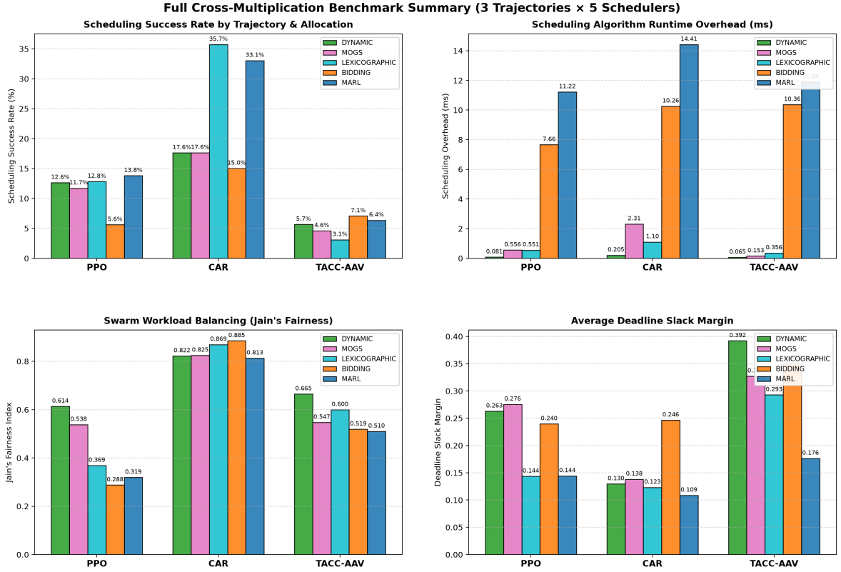
Fig. 1. Full Cartesian cross-product benchmark summary comparing all 15 combinations (3 Trajectory Models \times 5 Task Schedulers) across 100 simulation epochs on four primary KPIs: (a) Scheduling Success Rate (%), (b) Scheduling Algorithm Runtime Overhead (ms), (c) Swarm Workload Balancing via Jain's Fairness Index, and (d) Average Deadline Slack Margin.
