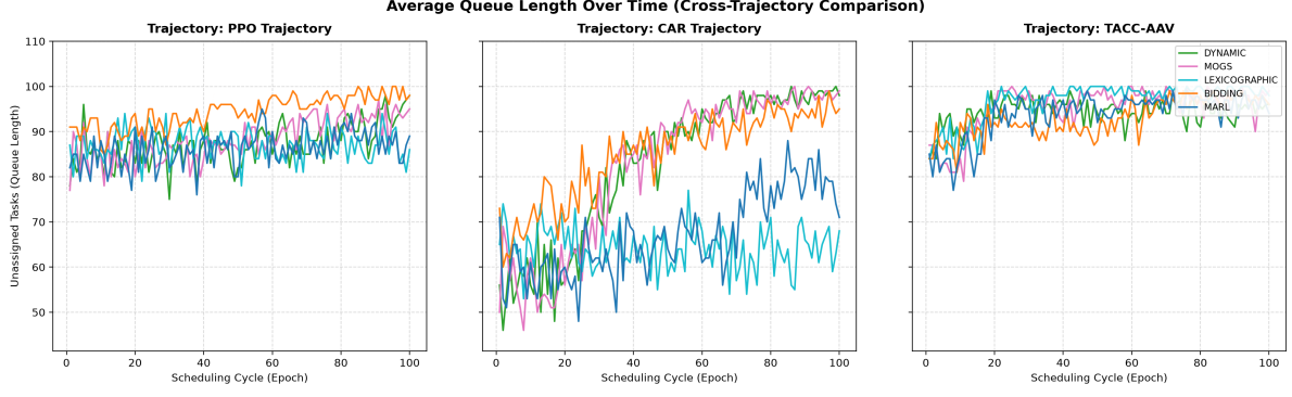
Fig. 8. Average queue length backlog over 100 cycles across PPO (left), CAR (center), and TACC-AAV (right). PPO experiences severe localized buffer overflow, whereas CAR balances queue occupancy across the fleet.
