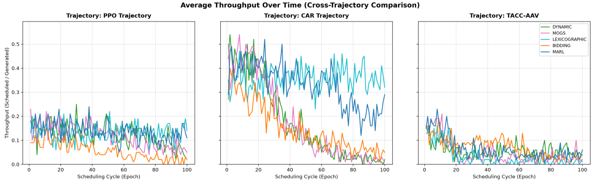
Fig. 3. Temporal throughput evolution (scheduled tasks / generated tasks) over 100 cycles across PPO (left), CAR (center), and TACC-AAV (right). CAR sustains significantly higher throughput due to global spatial coverage.
