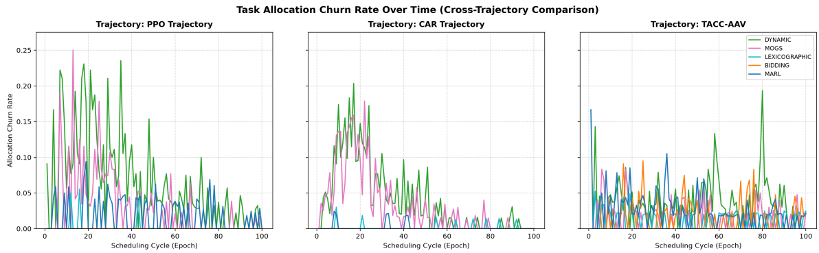
Fig. 7. Task allocation churn rate over 100 simulation epochs across PPO (left), CAR (center), and TACC-AAV (right). Dynamic matching isolates broken links without causing cascading network churn.
