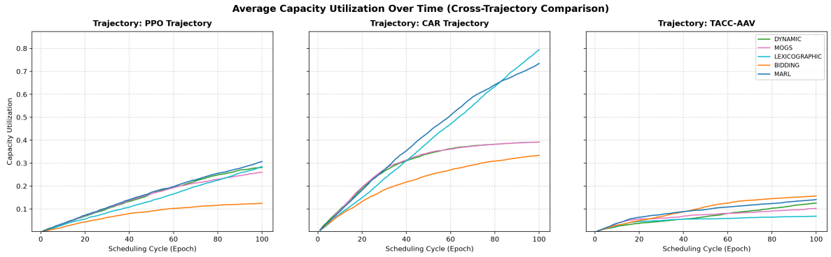
Fig. 9. Fleet capacity utilization over 100 simulation epochs across PPO (left), CAR (center), and TACC-AAV (right). CAR achieves the highest hardware capacity utilization.
