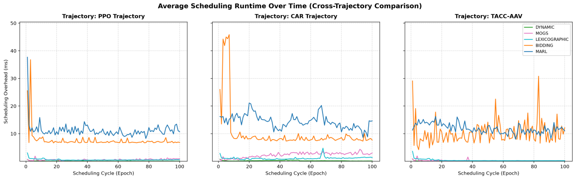
Fig. 4. Average scheduling runtime overhead (ms) per cycle over 100 epochs across PPO (left), CAR (center), and TACC-AAV (right). DYNAMIC achieves near-constant sub-millisecond execution, outperforming MARL and iterative auctions by over two orders of magnitude.
