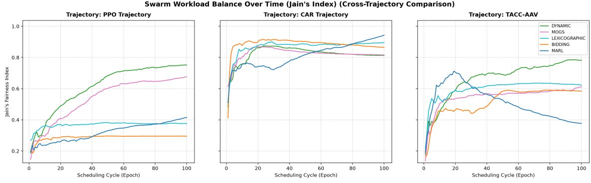
Fig. 5. Swarm workload balancing evaluated via Jain's Fairness Index ( \mathcal{J} ) across 100 simulation epochs for PPO (left), CAR (center), and TACC-AAV (right). CAR achieves the highest balance ( \mathcal{J} > 0.81 ) across all schedulers.
