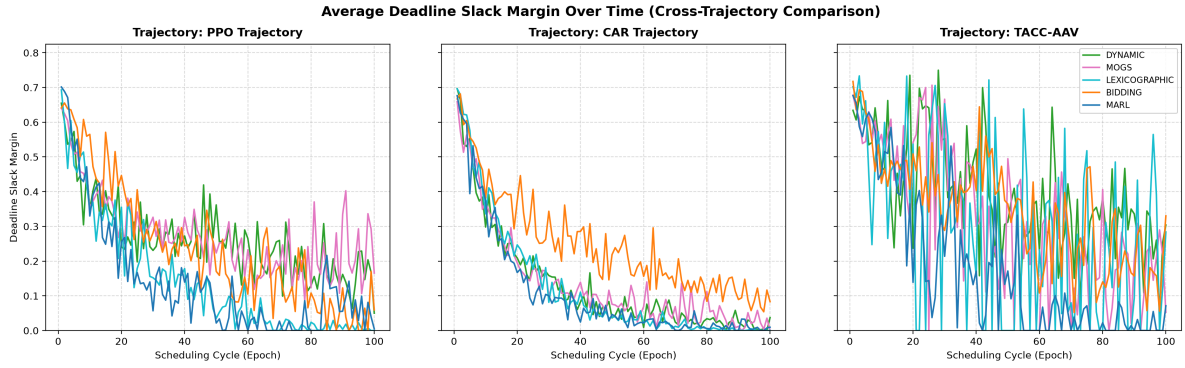
Fig. 6. Average deadline slack margin ( \bar{S} ) over 100 simulation epochs across PPO (left), CAR (center), and TACC-AAV (right). TACC-AAV maximizes safety slack by coupling dynamic battery headroom with admission gating.
